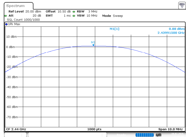
BLE_2M_Middle_Channel
