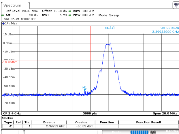
BLE_1M_Low_Channel
