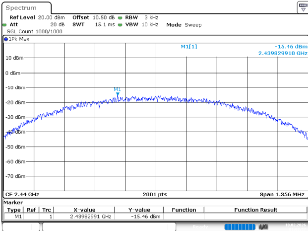
BLE_1M_Middle_Channel
