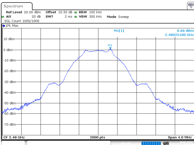
BLE_1M_High_Channel
