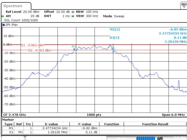
BLE_2M_High_Channel
