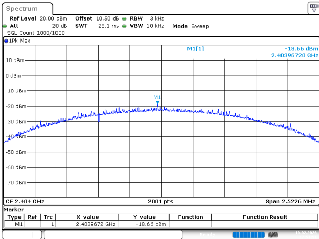
BLE_2M_Low_Channel
