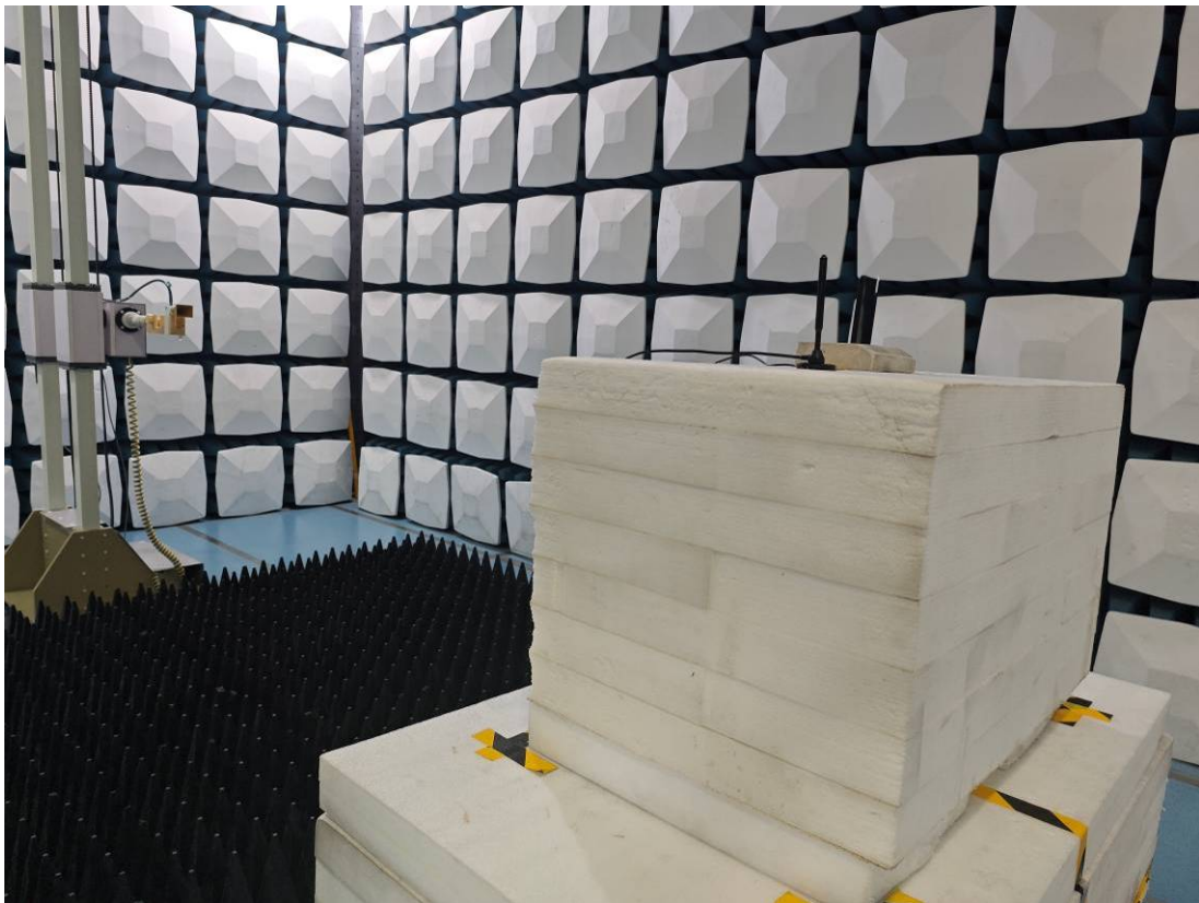
Radiated Emission 26.5-36GHz View
