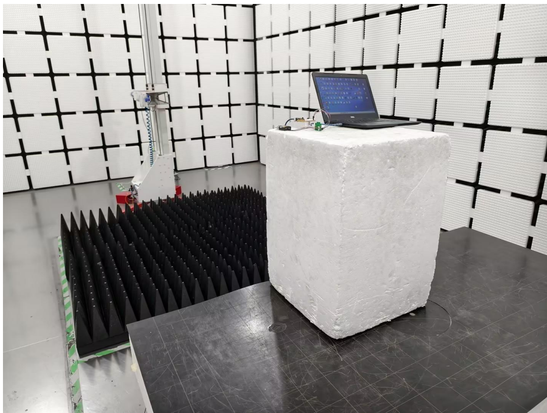
Spurious Emission above 1GHz test photo
