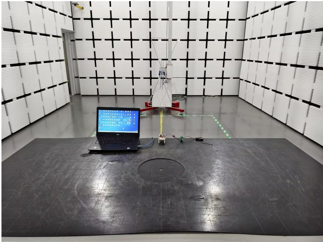
Spurious Emission below 1GHz test photo
