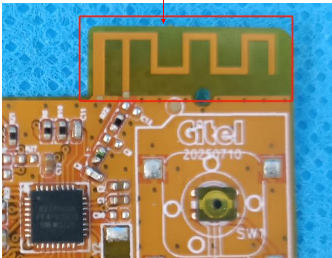
View of RF antenna
