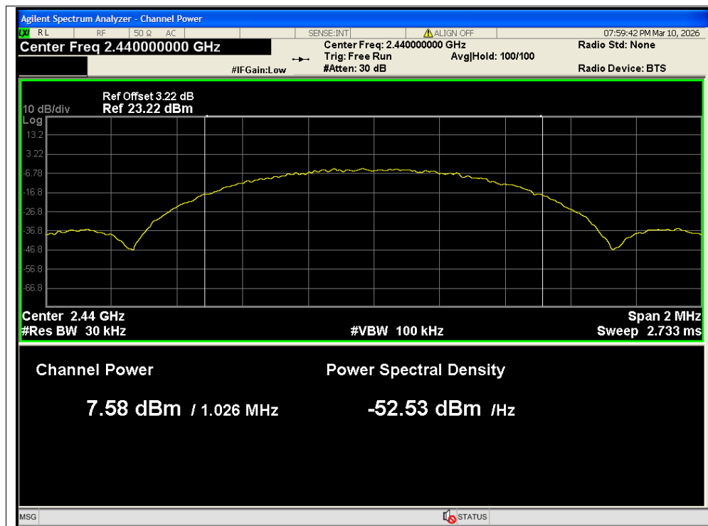
Average Power NVNT BLE 1M 2440MHz Ant2
