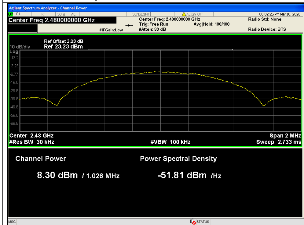
Average Power NVNT BLE 1M 2480MHz Ant2
