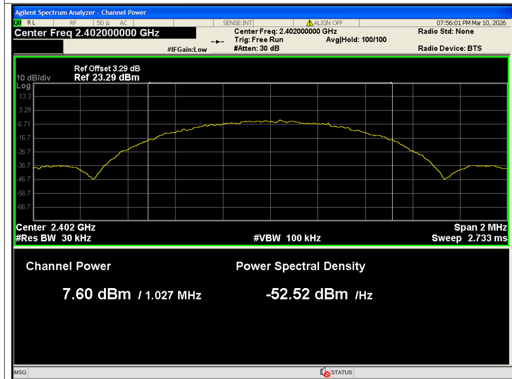
Average Power NVNT BLE 1M 2402MHz Ant2
