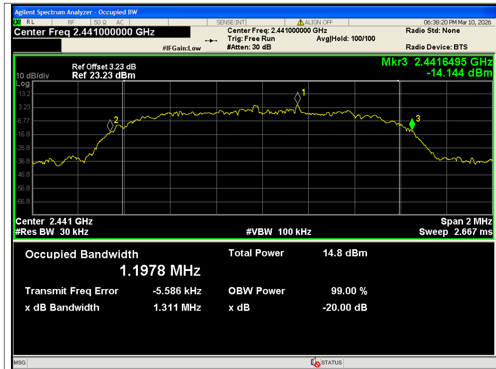
-20dB Bandwidth NVNT 3-DH5 2441MHz Ant2
