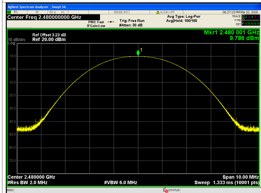
Peak Power NVNT 1-DH5 2480MHz Ant2
