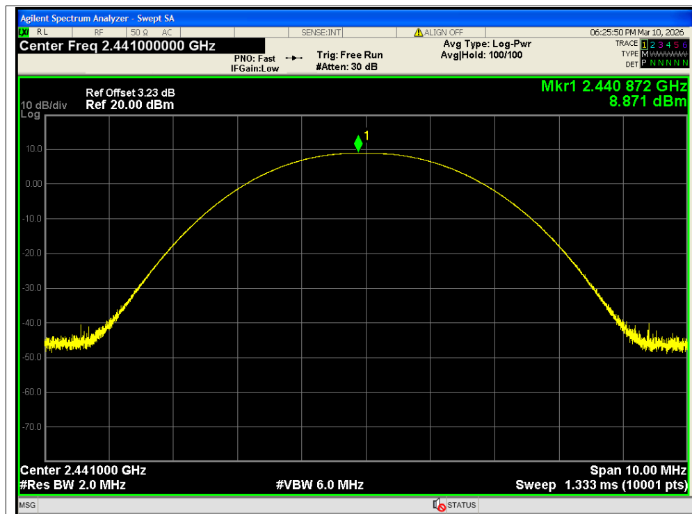
Peak Power NVNT 1-DH5 2441MHz Ant2
