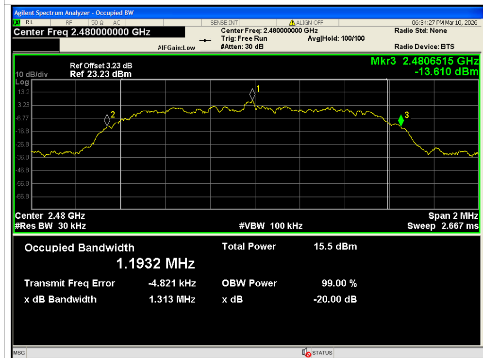
-20dB Bandwidth NVNT 2-DH5 2480MHz Ant2
