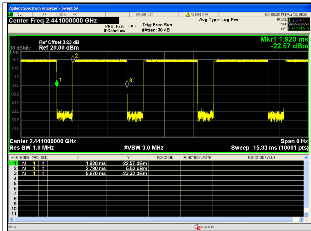
Duty Cycle NVNT 3-DH5 2441MHz Ant2
