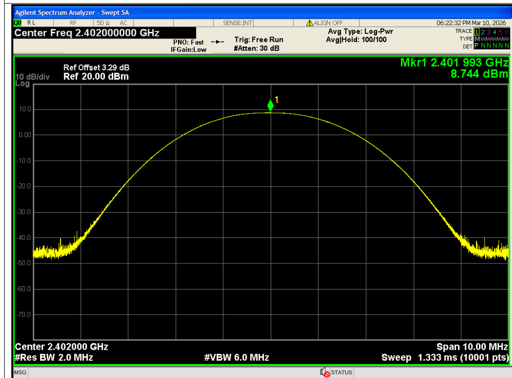
Peak Power NVNT 1-DH5 2402MHz Ant2
