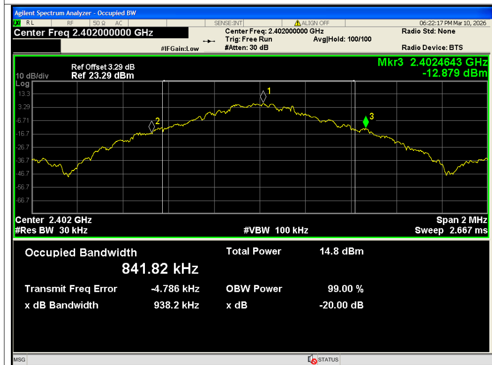
-20dB Bandwidth NVNT 1-DH5 2402MHz Ant2
