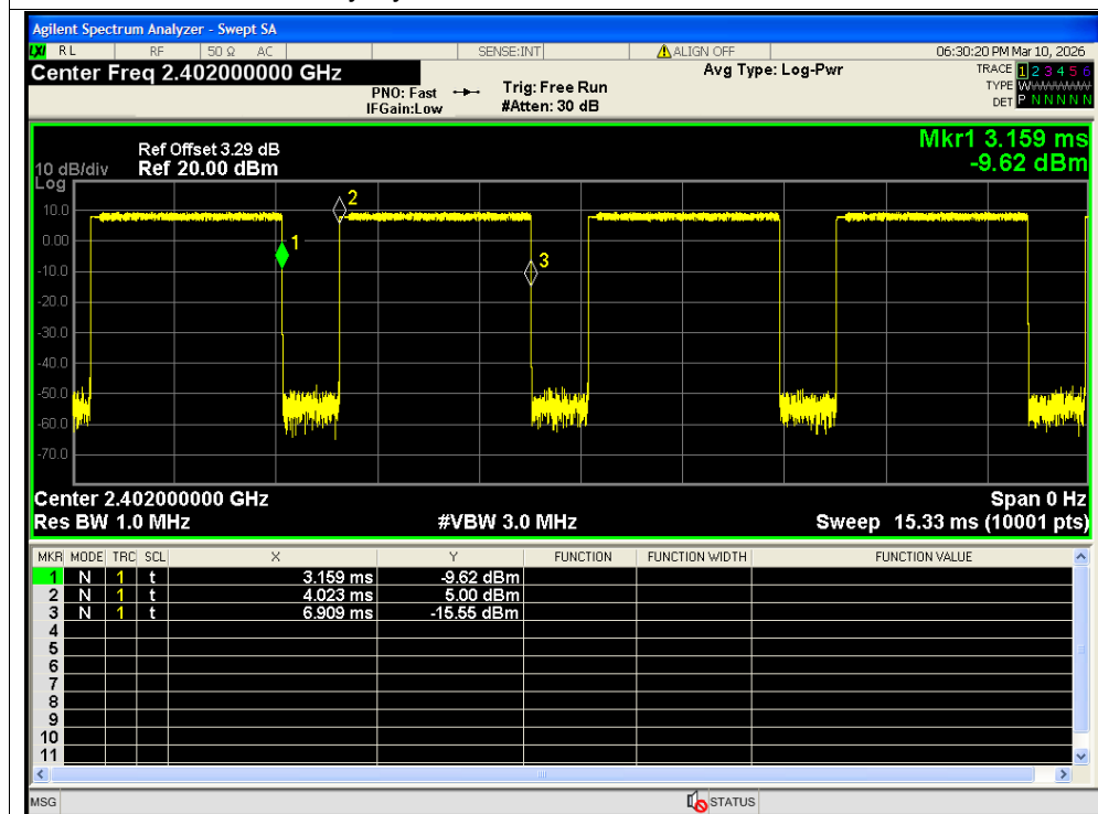
Duty Cycle NVNT 2-DH5 2402MHz Ant2
