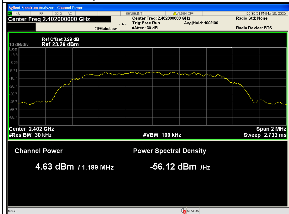
Average Power NVNT 2-DH5 2402MHz Ant2
