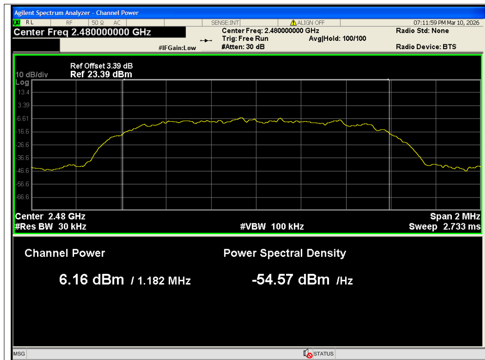
Average Power NVNT 3-DH5 2480MHz Ant1
