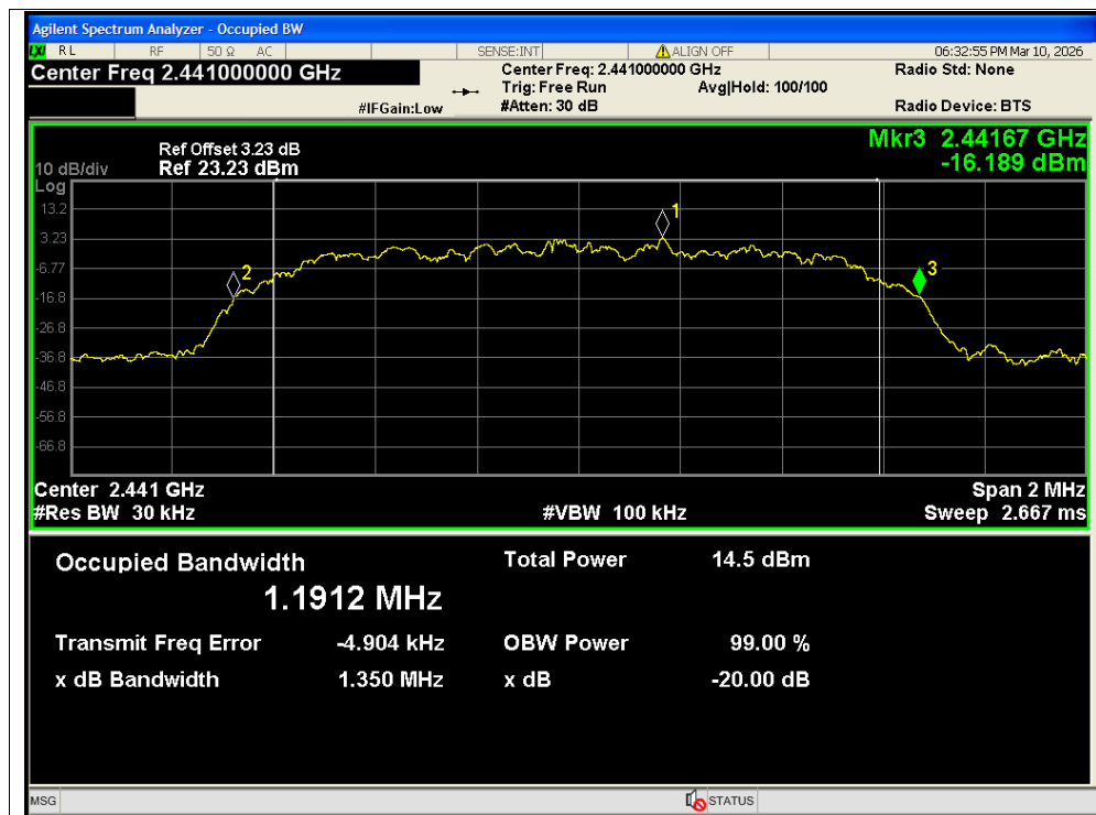
-20dB Bandwidth NVNT 2-DH5 2441MHz Ant2
