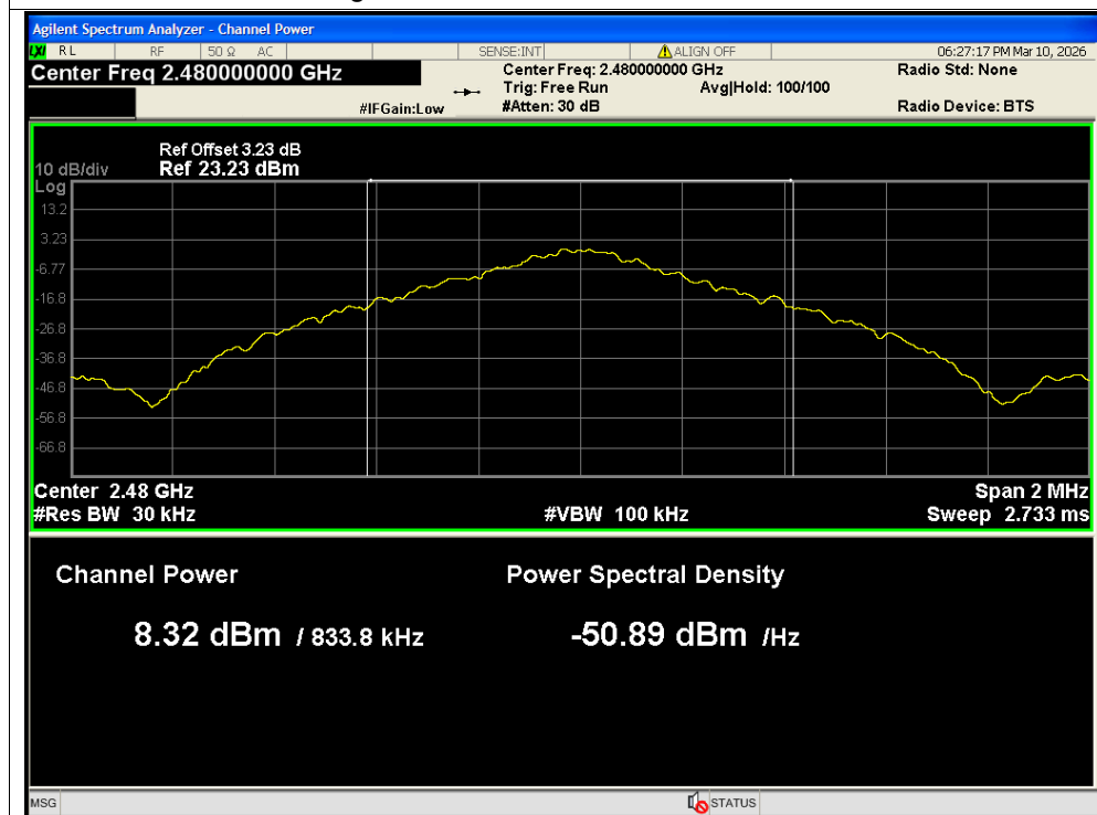
Average Power NVNT 1-DH5 2480MHz Ant2
