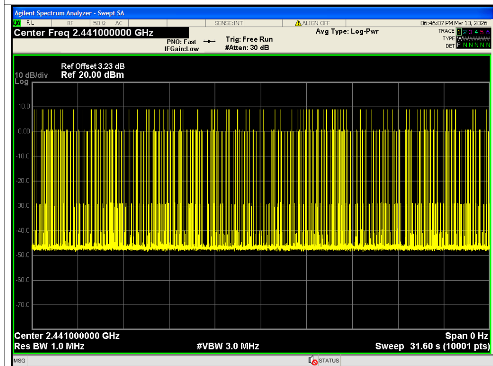
Dwell NVNT 1-DH5 2441MHz Ant2 Accumulated
