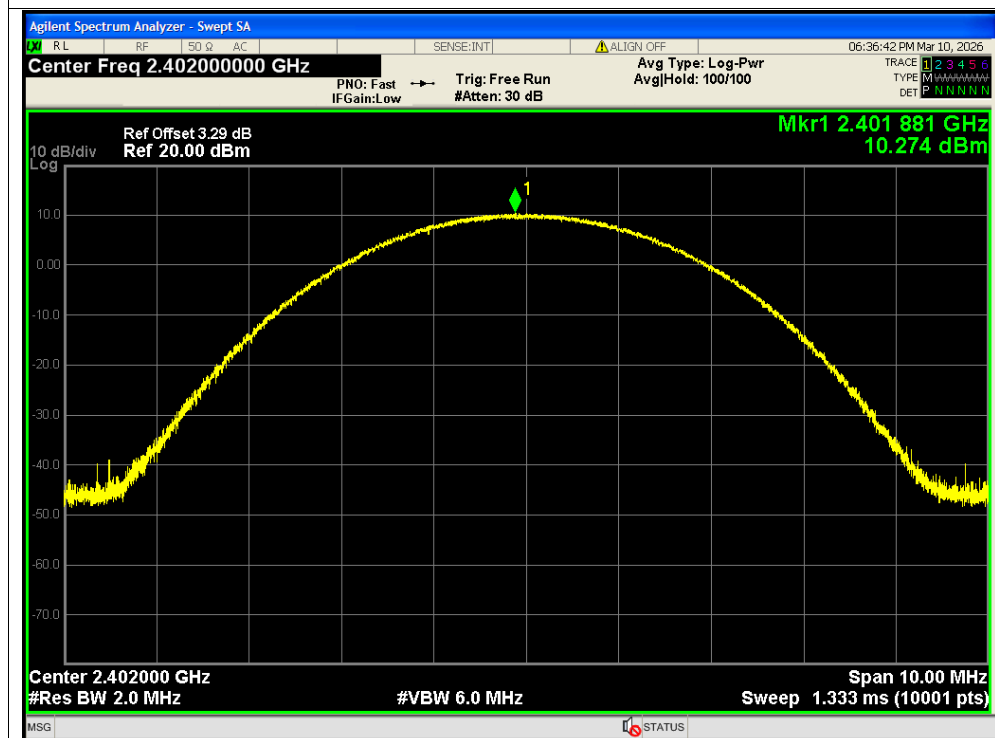
Peak Power NVNT 3-DH5 2402MHz Ant2
