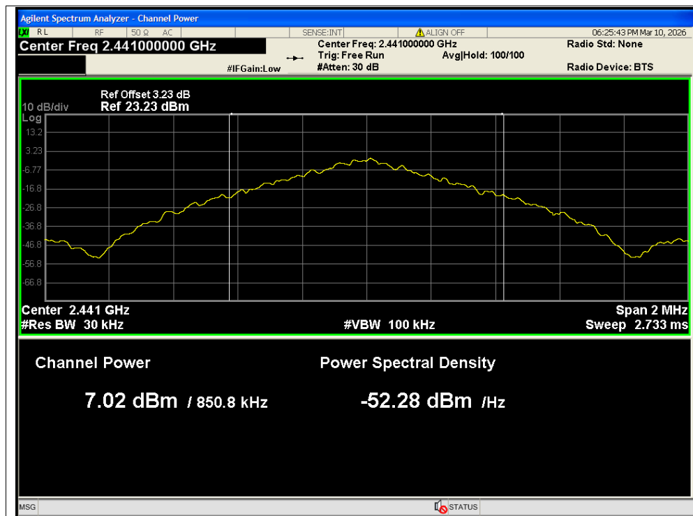
Average Power NVNT 1-DH5 2441MHz Ant2
