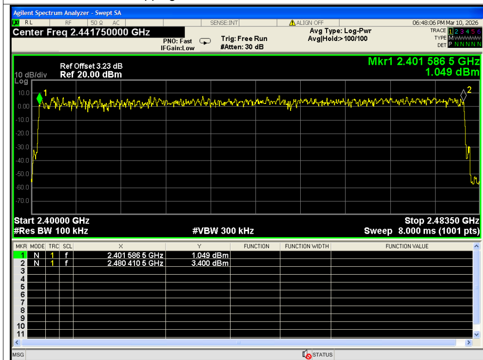
Hopping No. NVNT 2-DH5 2441MHz Ant2
