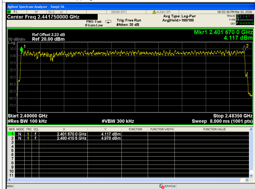
Hopping No. NVNT 3-DH5 2441MHz Ant2
