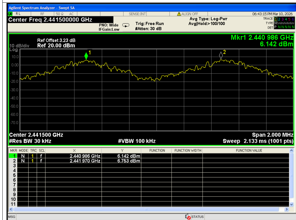
CFS NVNT 1-DH5 2441MHz Ant2
