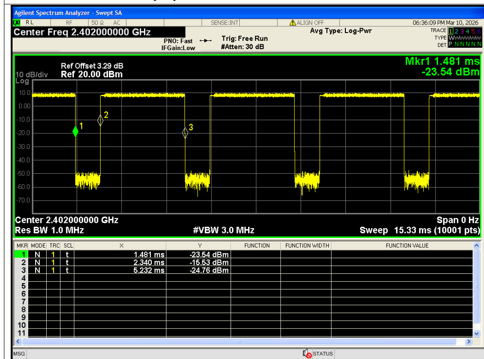
Duty Cycle NVNT 3-DH5 2402MHz Ant2
