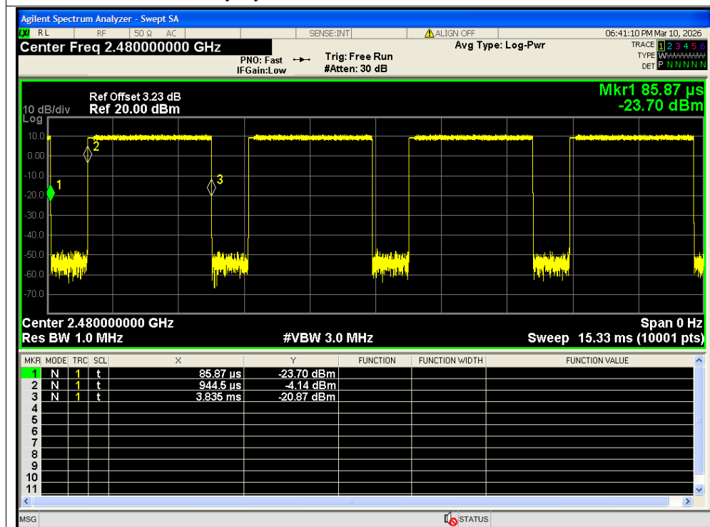
Duty Cycle NVNT 3-DH5 2480MHz Ant2
