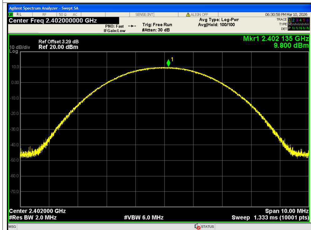
Peak Power NVNT 2-DH5 2402MHz Ant2
