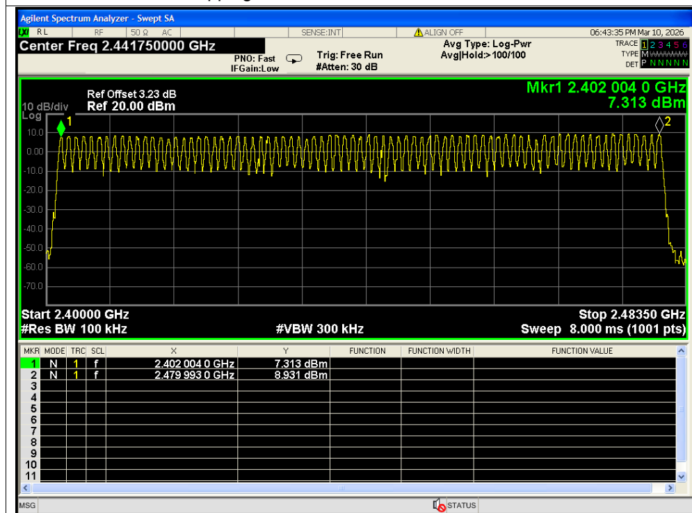
Hopping No. NVNT 1-DH5 2441MHz Ant2
