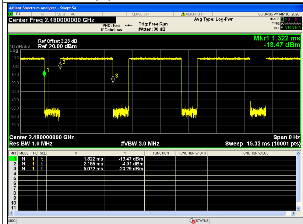
Duty Cycle NVNT 2-DH5 2480MHz Ant2
