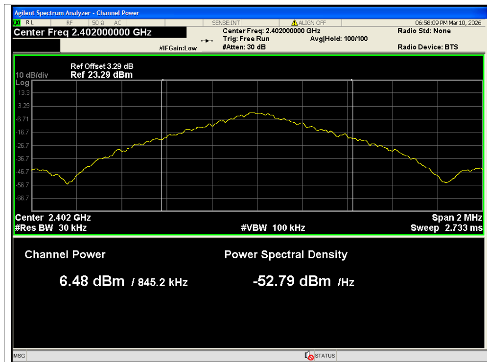
Average Power NVNT 1-DH5 2402MHz Ant1
