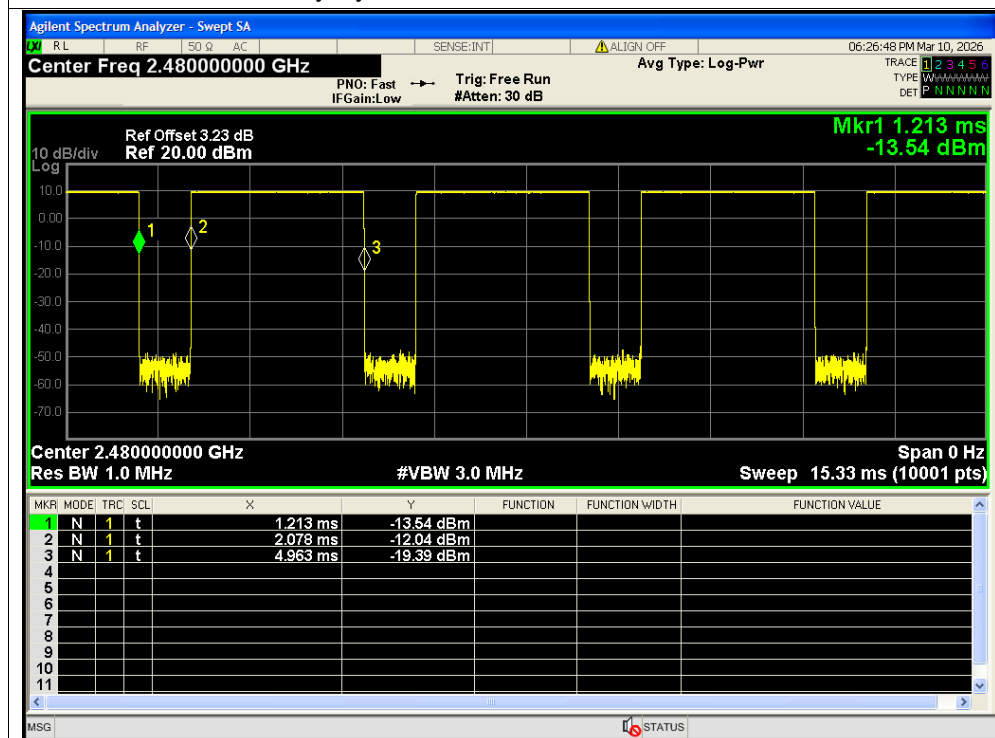
Duty Cycle NVNT 1-DH5 2480MHz Ant2
