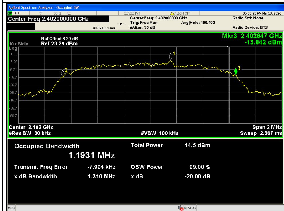
-20dB Bandwidth NVNT 3-DH5 2402MHz Ant2
