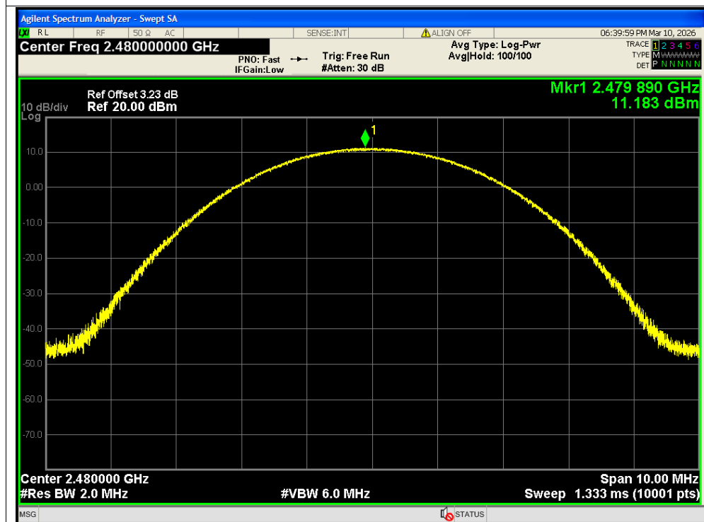
Peak Power NVNT 3-DH5 2480MHz Ant2
