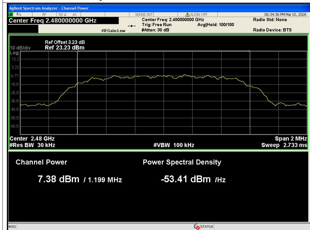
Average Power NVNT 2-DH5 2480MHz Ant2
