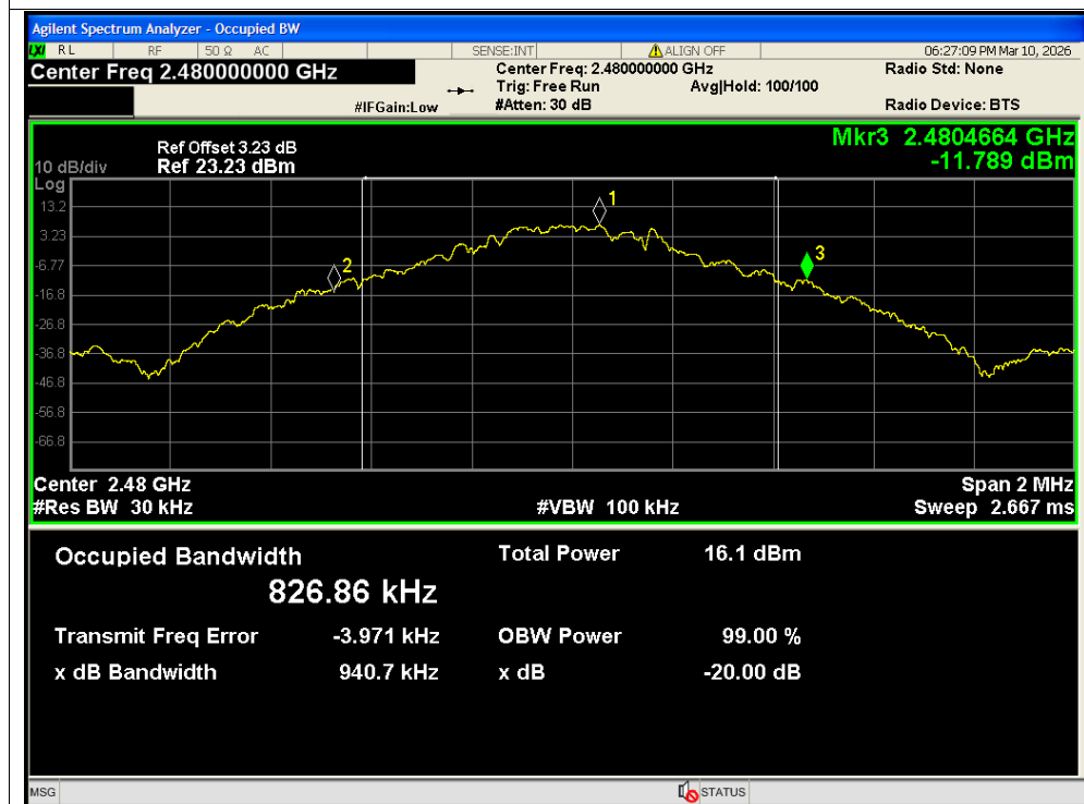
-20dB Bandwidth NVNT 1-DH5 2480MHz Ant2
