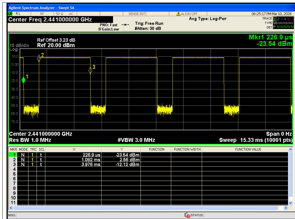
Duty Cycle NVNT 1-DH5 2441MHz Ant2
