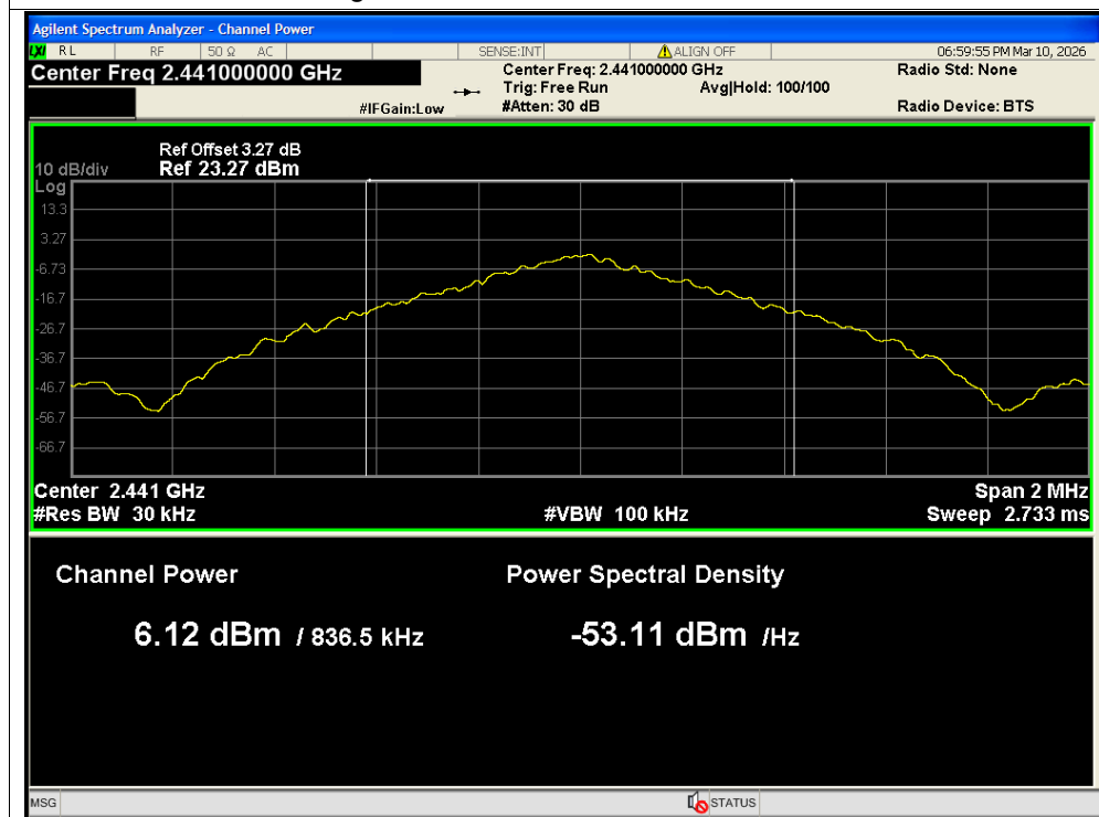
Average Power NVNT 1-DH5 2441MHz Ant1
