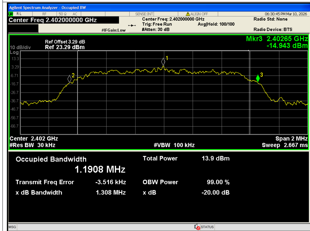
-20dB Bandwidth NVNT 2-DH5 2402MHz Ant2
