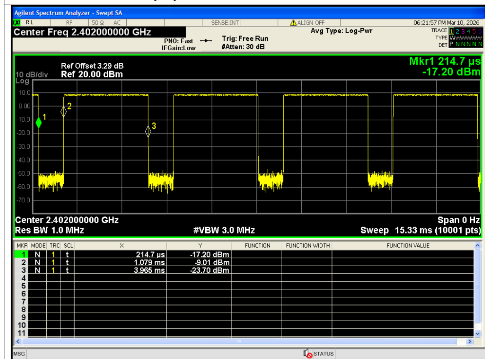
Duty Cycle NVNT 1-DH5 2402MHz Ant2
