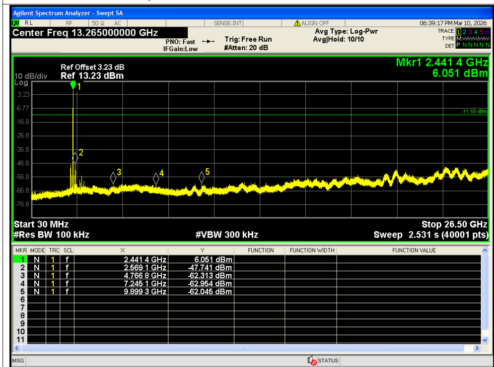
Tx. Spurious NVNT 3-DH5 2441MHz Ant2 Emission
