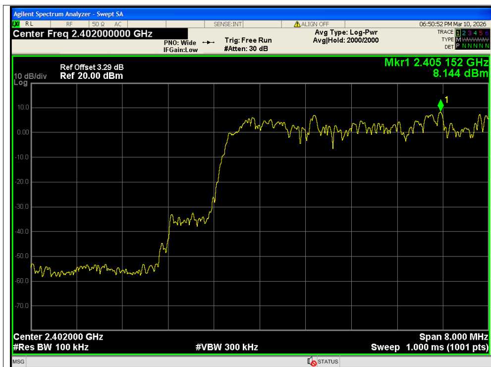
Band Edge(Hopping) NVNT 3-DH5 2402MHz Ant2 Hopping Ref
