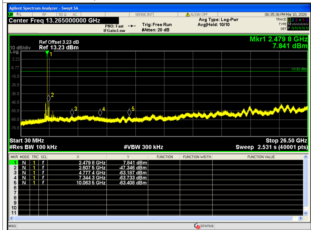
Tx. Spurious NVNT 2-DH5 2480MHz Ant2 Emission
