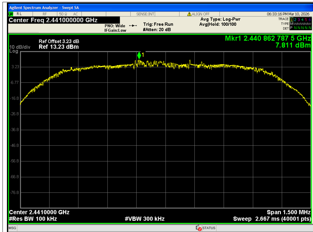
Tx. Spurious NVNT 2-DH5 2441MHz Ant2 Ref
