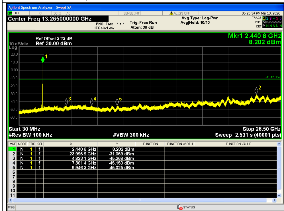
Tx. Spurious NVNT 1-DH5 2441MHz Ant2 Emission
