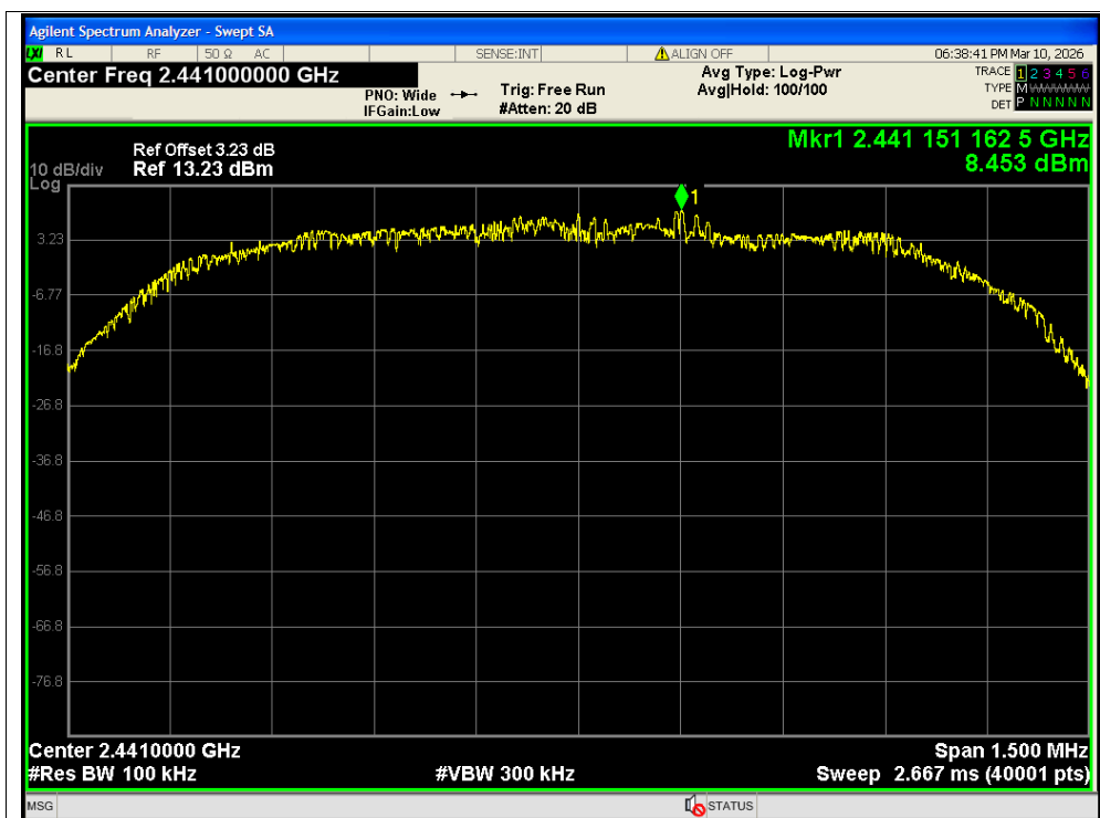
Tx. Spurious NVNT 3-DH5 2441MHz Ant2 Ref
