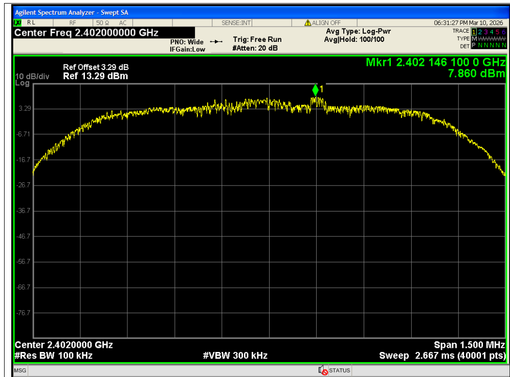
Tx. Spurious NVNT 2-DH5 2402MHz Ant2 Ref
