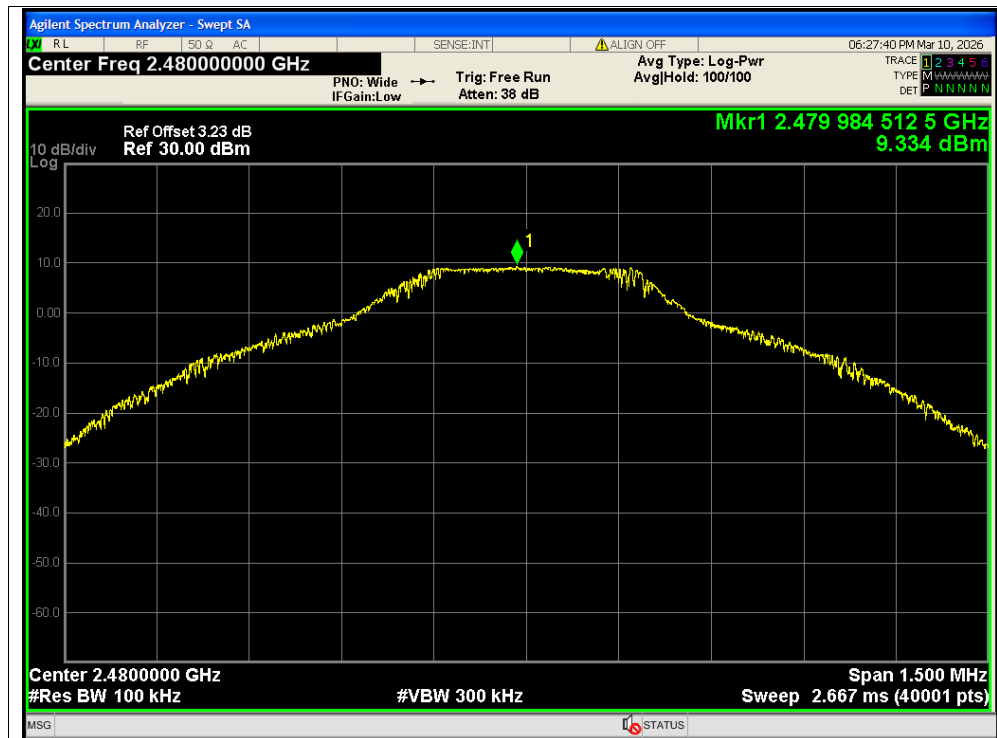
Tx. Spurious NVNT 1-DH5 2480MHz Ant2 Ref
