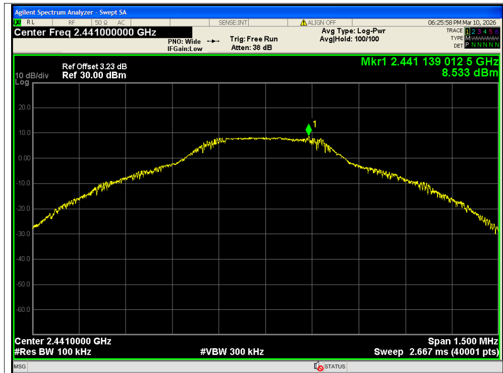
Tx. Spurious NVNT 1-DH5 2441MHz Ant2 Ref
