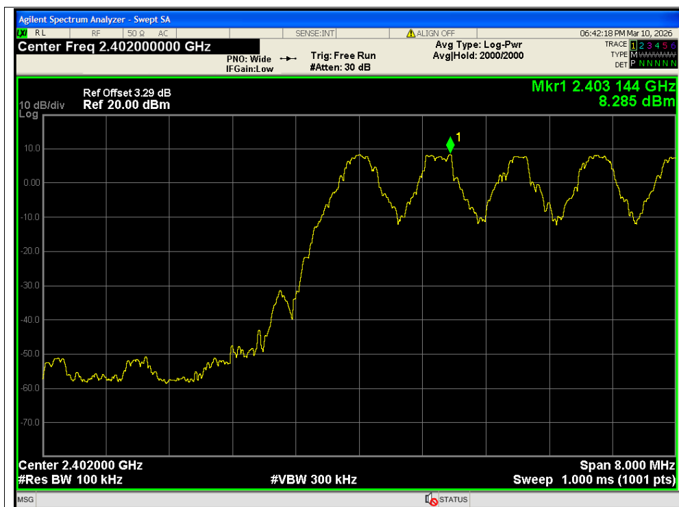
Band Edge(Hopping) NVNT 1-DH5 2402MHz Ant2 Hopping Ref
