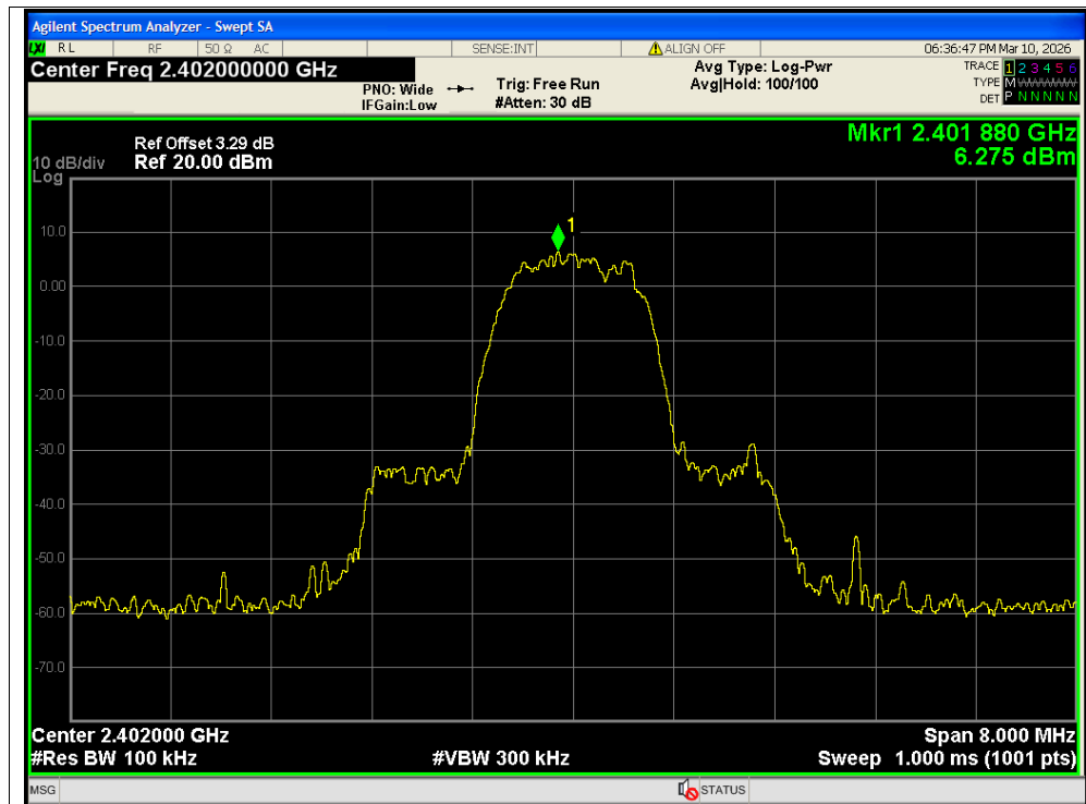
Band Edge NVNT 3-DH5 2402MHz Ant2 No-Hopping Ref
