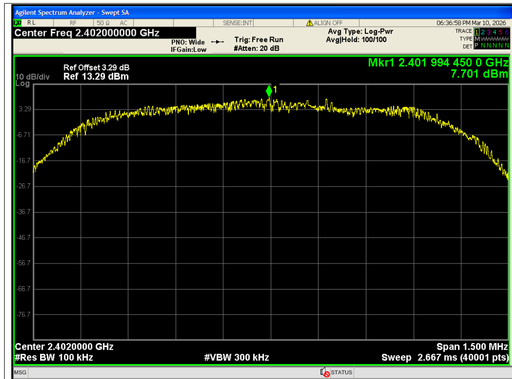
Tx. Spurious NVNT 3-DH5 2402MHz Ant2 Ref
