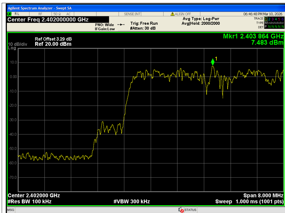
Band Edge(Hopping) NVNT 2-DH5 2402MHz Ant2 Hopping Ref
