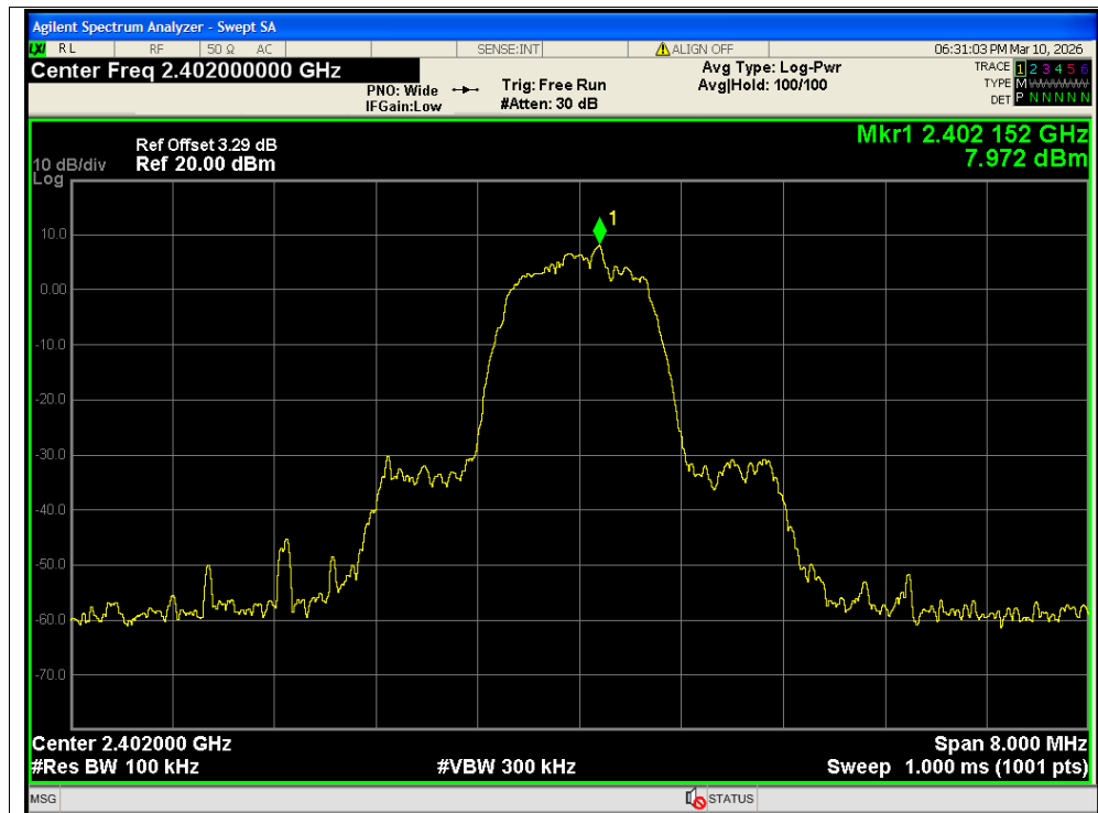
Band Edge NVNT 2-DH5 2402MHz Ant2 No-Hopping Ref
