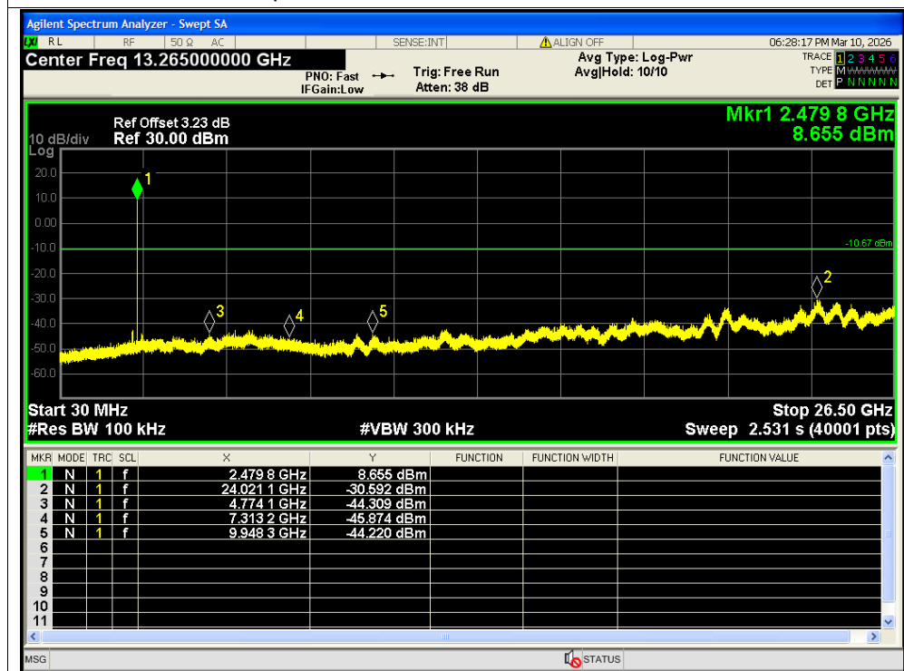
Tx. Spurious NVNT 1-DH5 2480MHz Ant2 Emission
