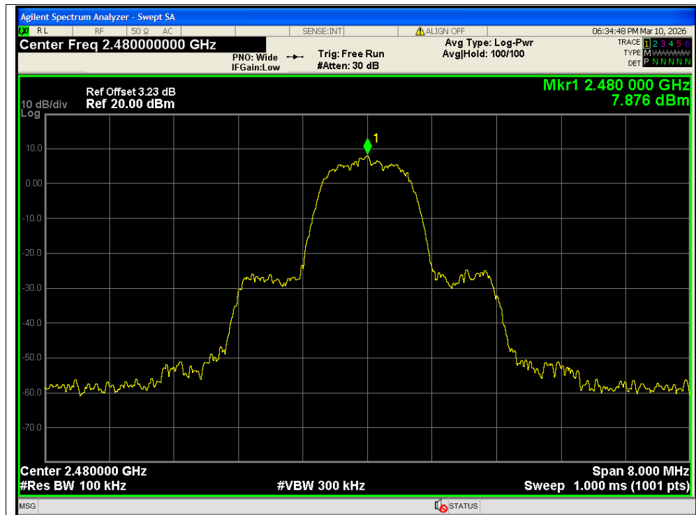
Band Edge NVNT 2-DH5 2480MHz Ant2 No-Hopping Ref
