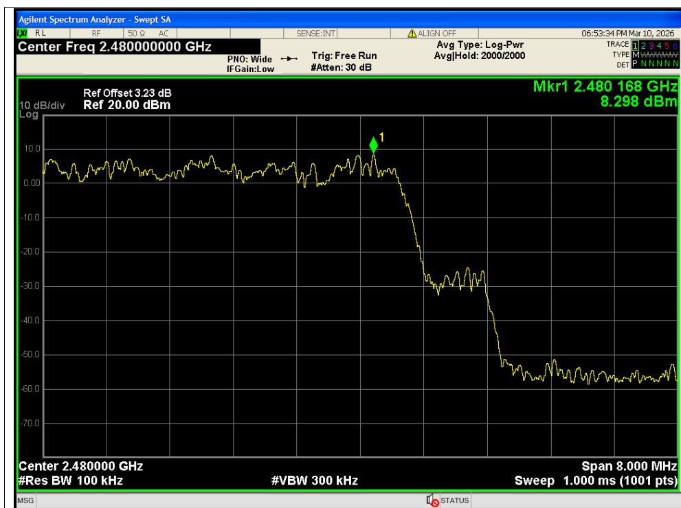
Band Edge(Hopping) NVNT 3-DH5 2480MHz Ant2 Hopping Ref
