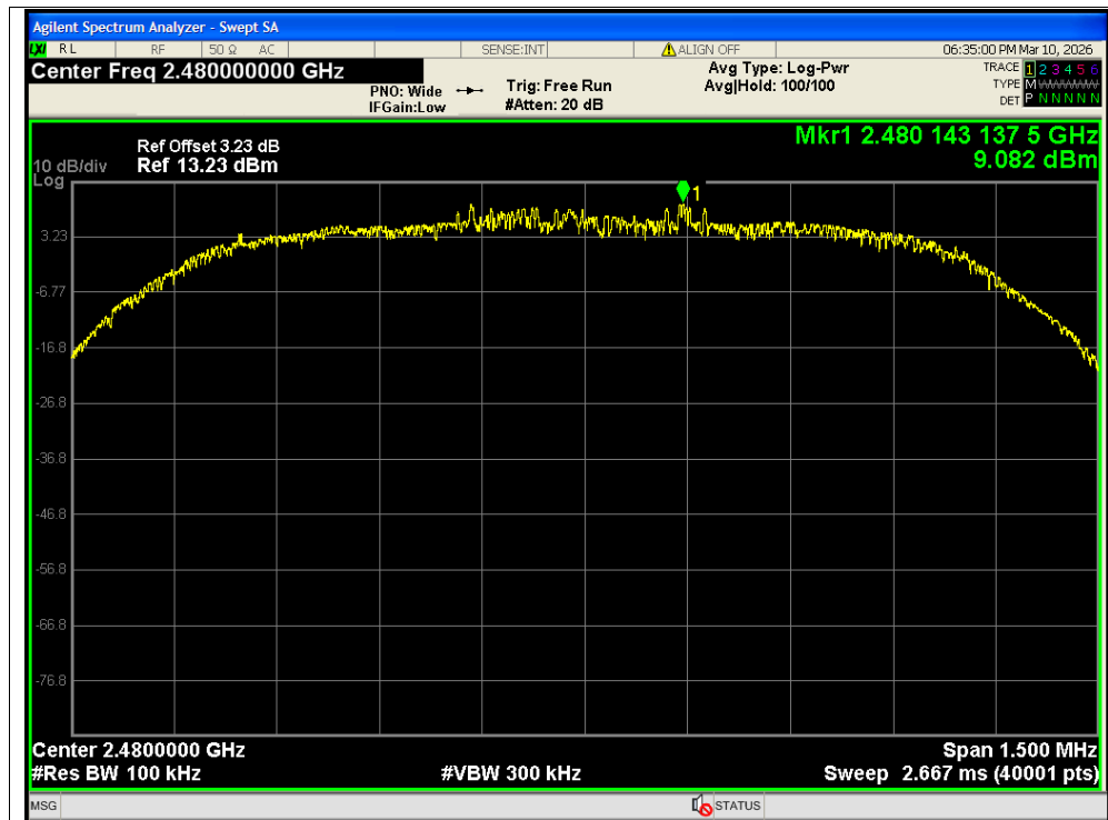
Tx. Spurious NVNT 2-DH5 2480MHz Ant2 Ref
