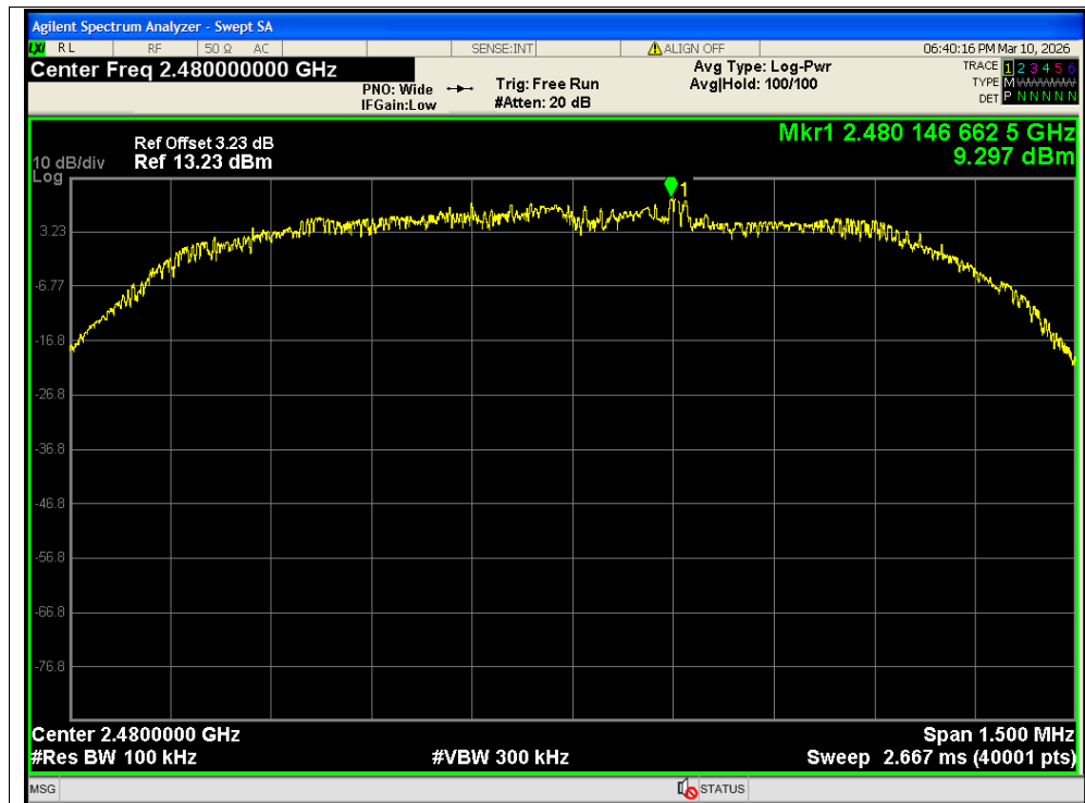
Tx. Spurious NVNT 3-DH5 2480MHz Ant2 Ref
