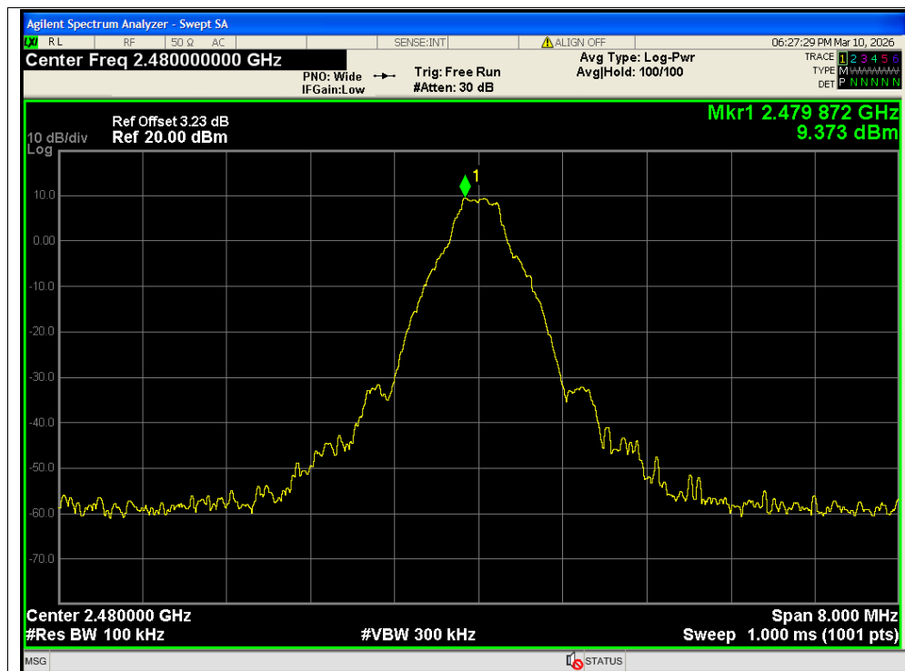
Band Edge NVNT 1-DH5 2480MHz Ant2 No-Hopping Ref
