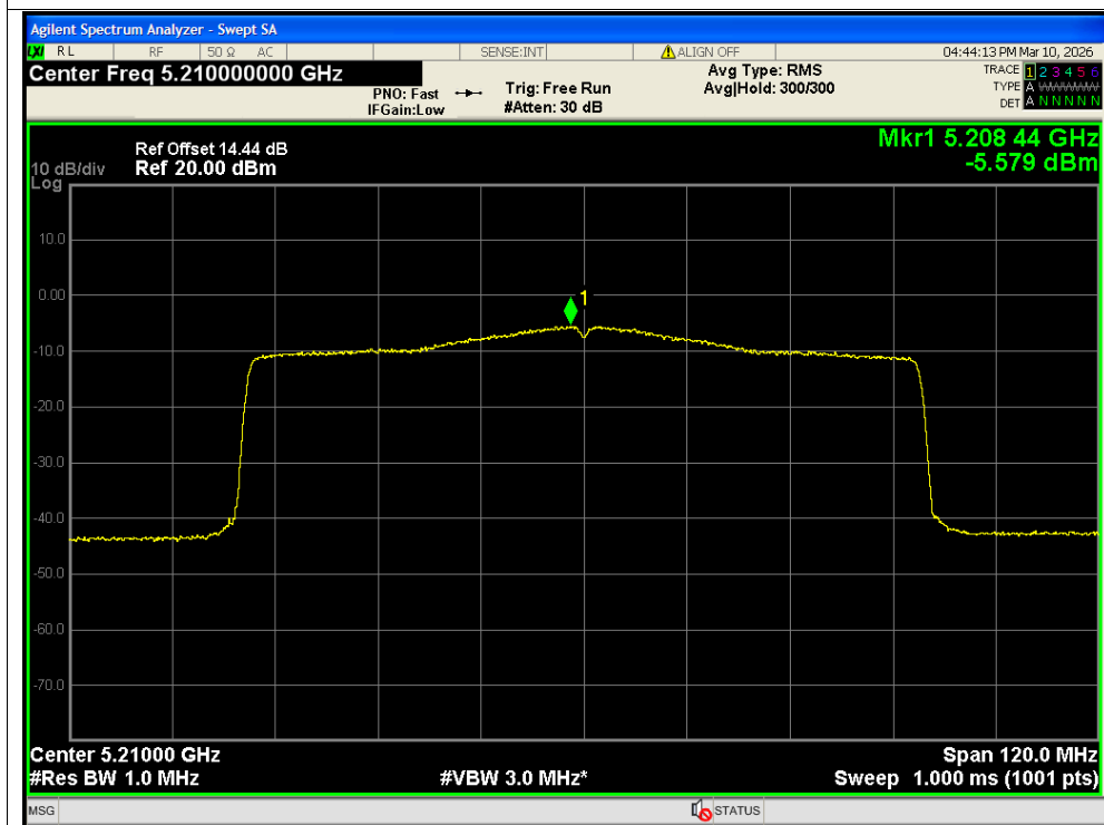
PSD NVNT ax80 5210MHz Ant2 MIMO
