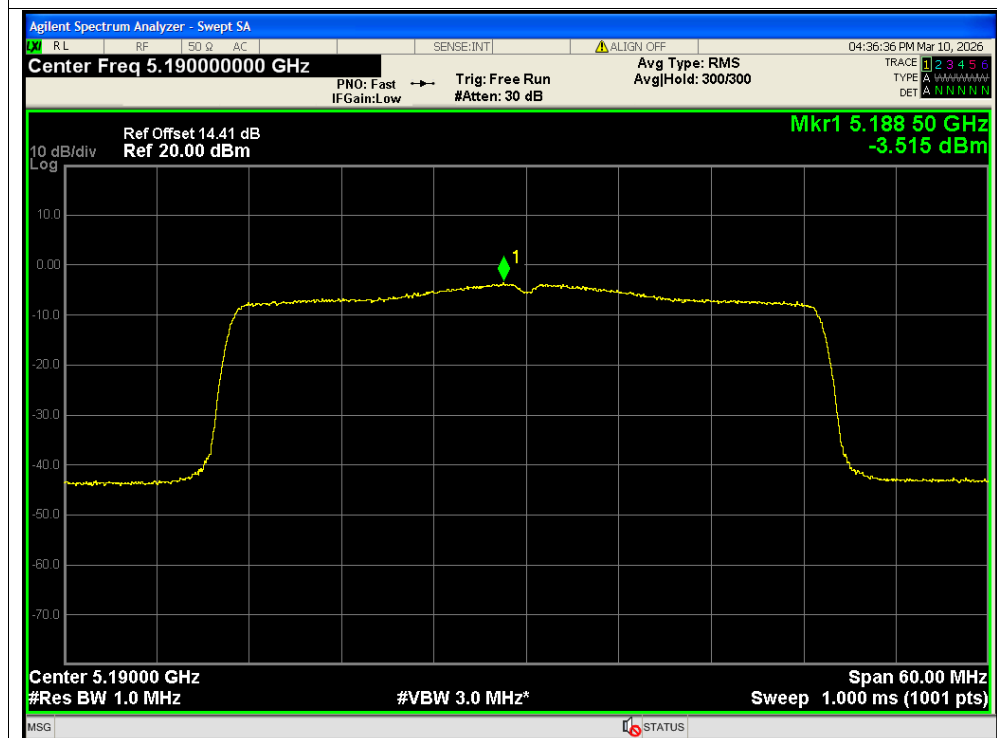
PSD NVNT ax40 5190MHz Ant2 MIMO
