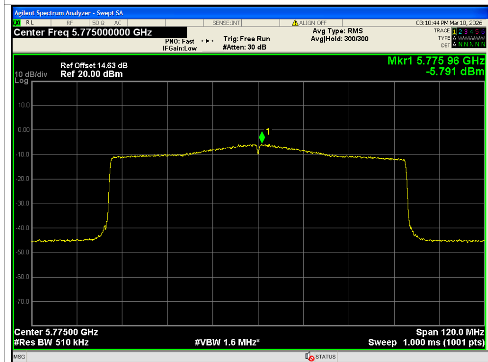
PSD NVNT ax80 5775MHz Ant2 SISO
