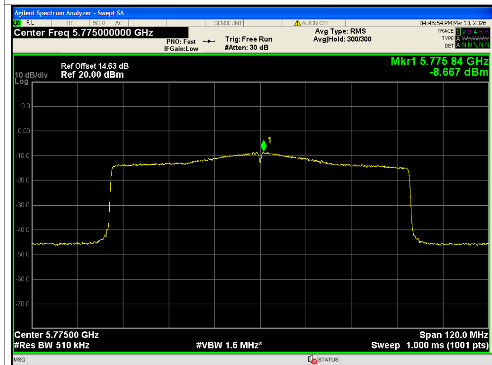
PSD NVNT ax80 5775MHz Ant2 MIMO
