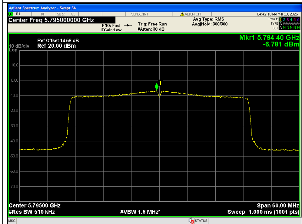
PSD NVNT ax40 5795MHz Ant2 MIMO
