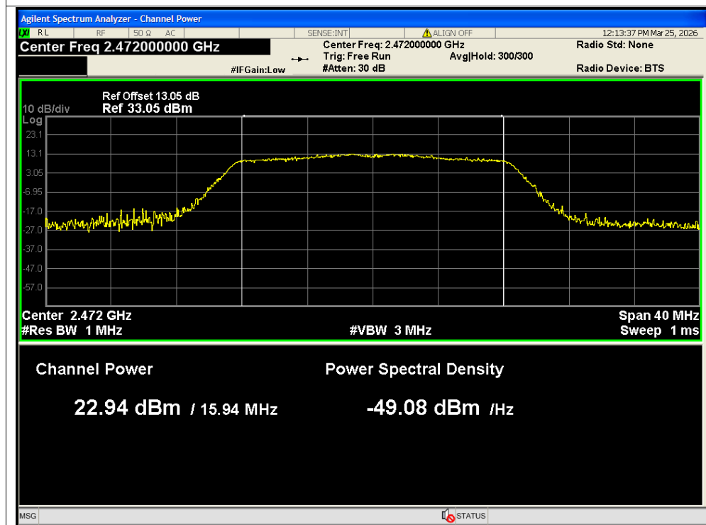
Peak Power NVNT n20 2472MHz Ant2 SISO
