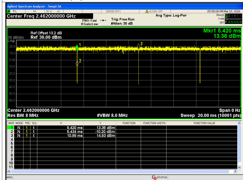
Duty Cycle NVNT ax40 2462MHz Ant1 SISO
