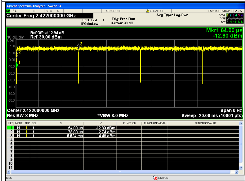
Duty Cycle NVNT ax40 2422MHz Ant1 SISO
