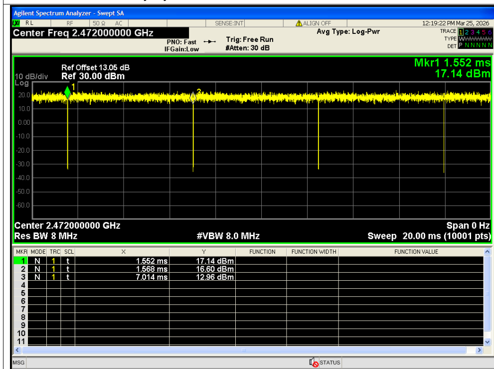
Duty Cycle NVNT ax20 2472MHz Ant2 SISO
