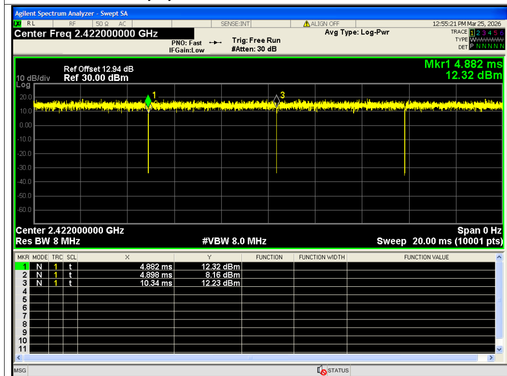
Duty Cycle NVNT ax40 2422MHz Sum MIMO
