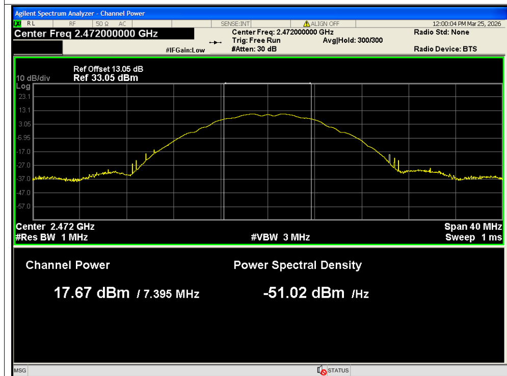
Peak Power NVNT b 2472MHz Ant2 SISO
