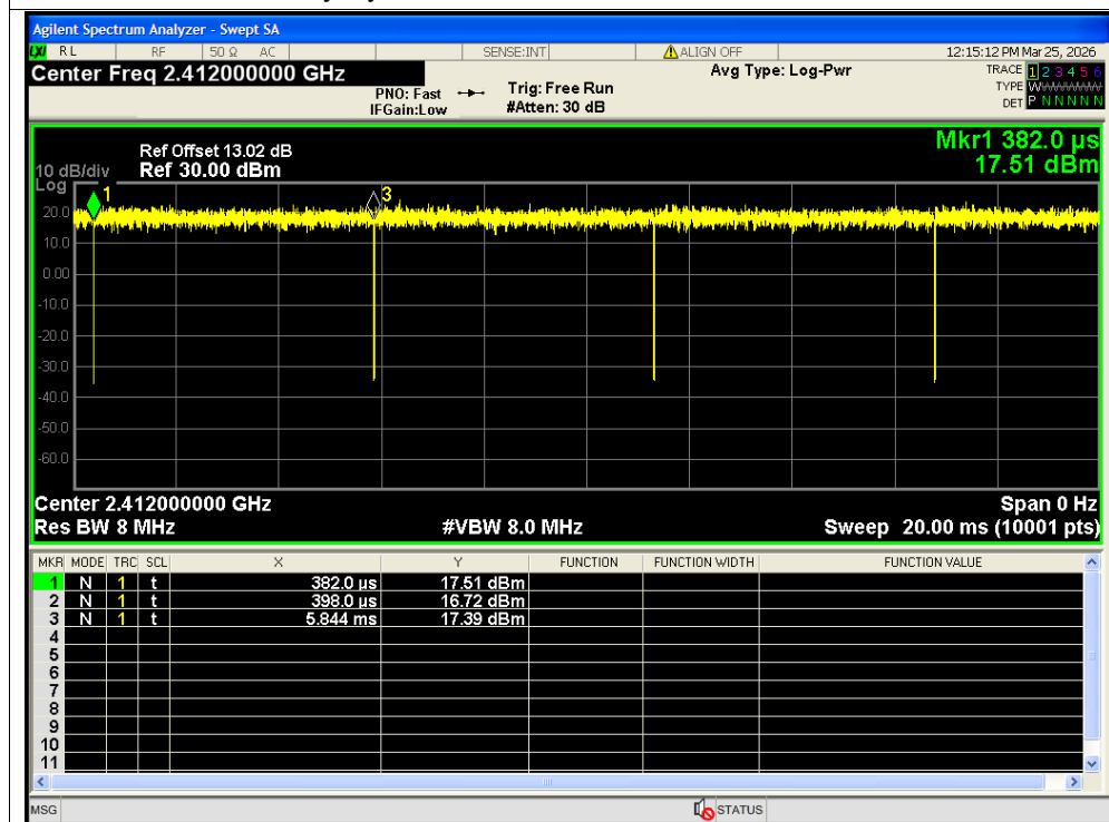
Duty Cycle NVNT ax20 2412MHz Ant2 SISO
