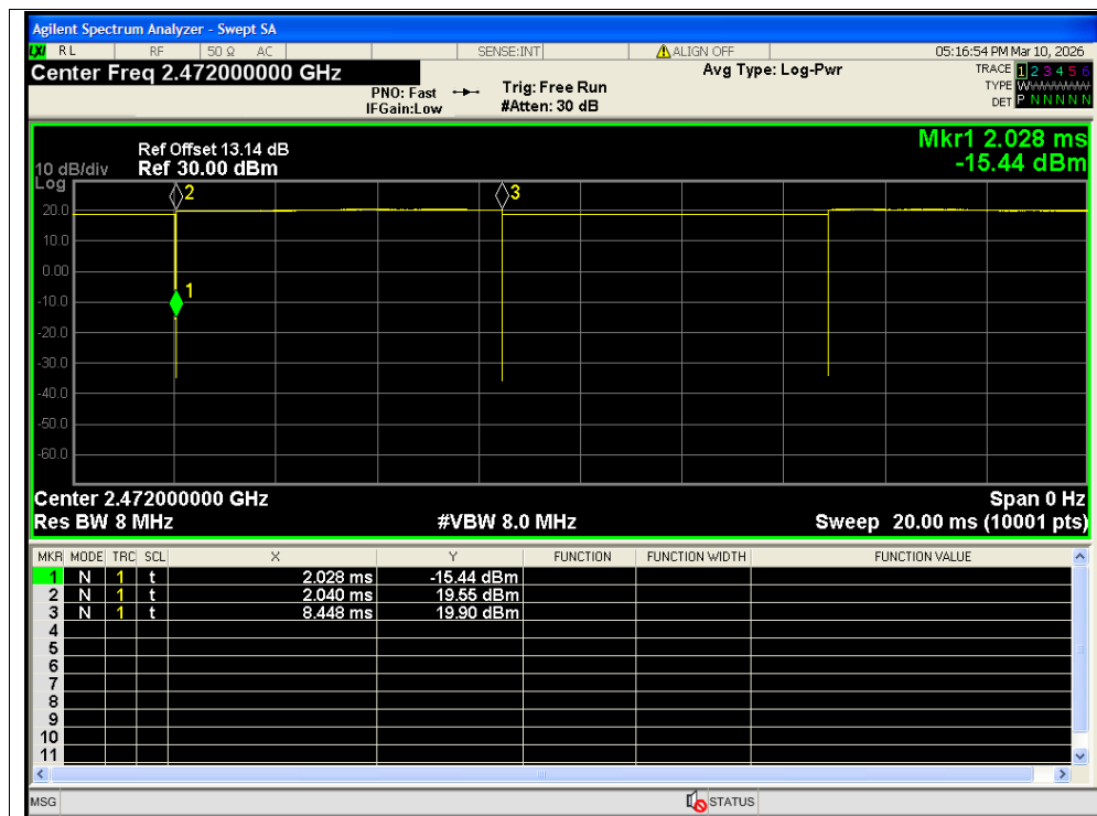
Duty Cycle NVNT b 2472MHz Ant1 SISO
