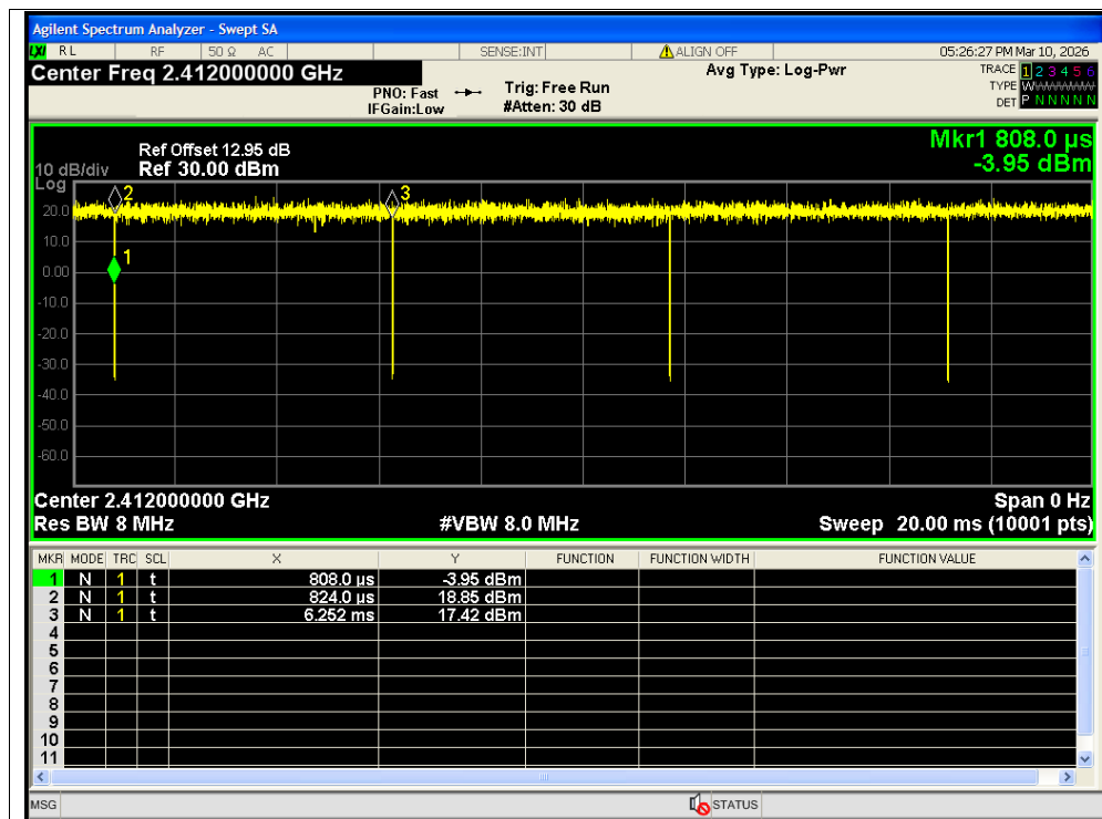
Duty Cycle NVNT n20 2412MHz Ant1 SISO
