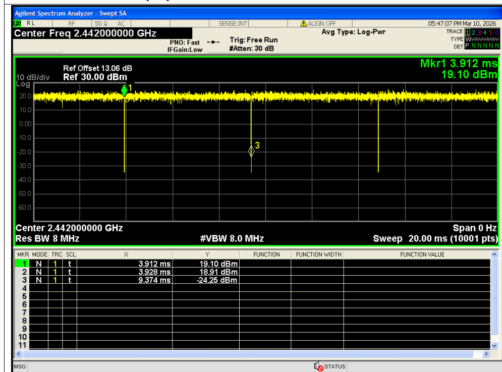
Duty Cycle NVNT ax20 2442MHz Ant1 SISO
