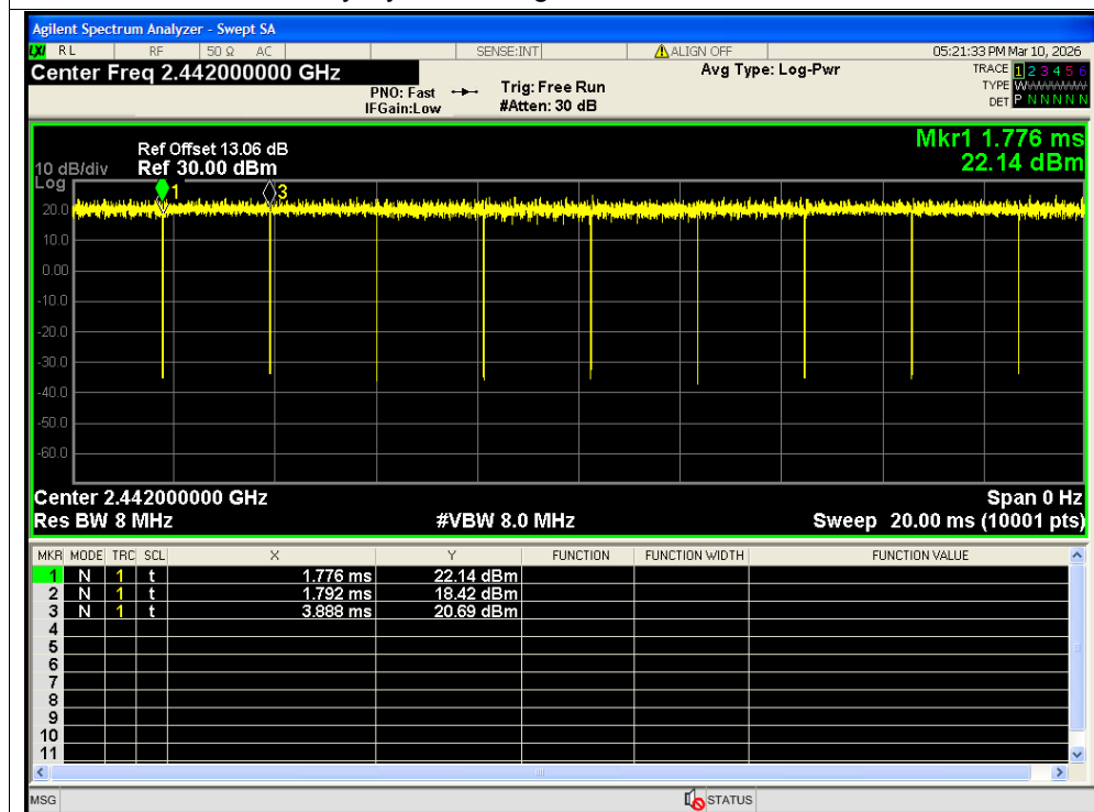
Duty Cycle NVNT g 2442MHz Ant1 SISO
