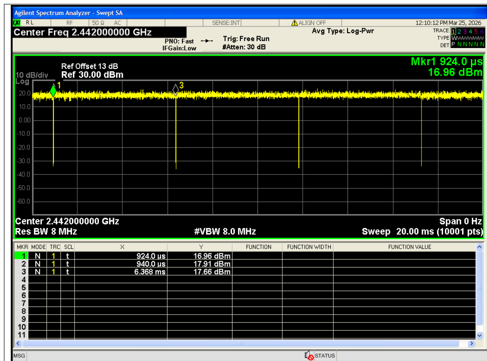
Duty Cycle NVNT n20 2442MHz Ant2 SISO
