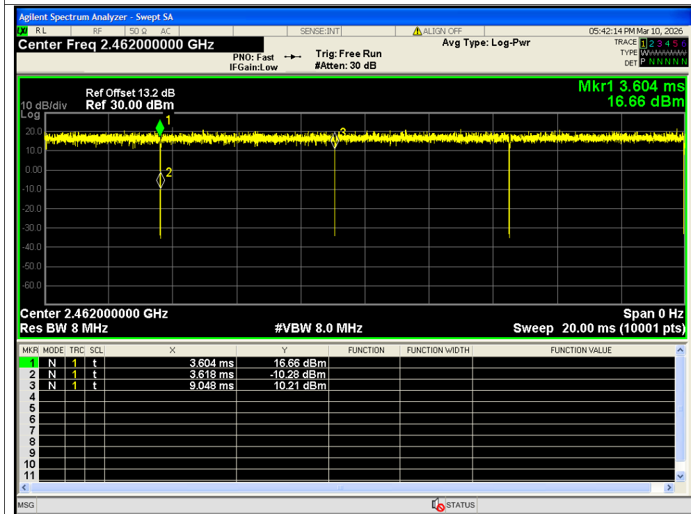
Duty Cycle NVNT n40 2462MHz Ant1 SISO
