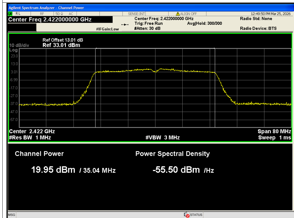
Peak Power NVNT n40 2422MHz Ant2 MIMO
