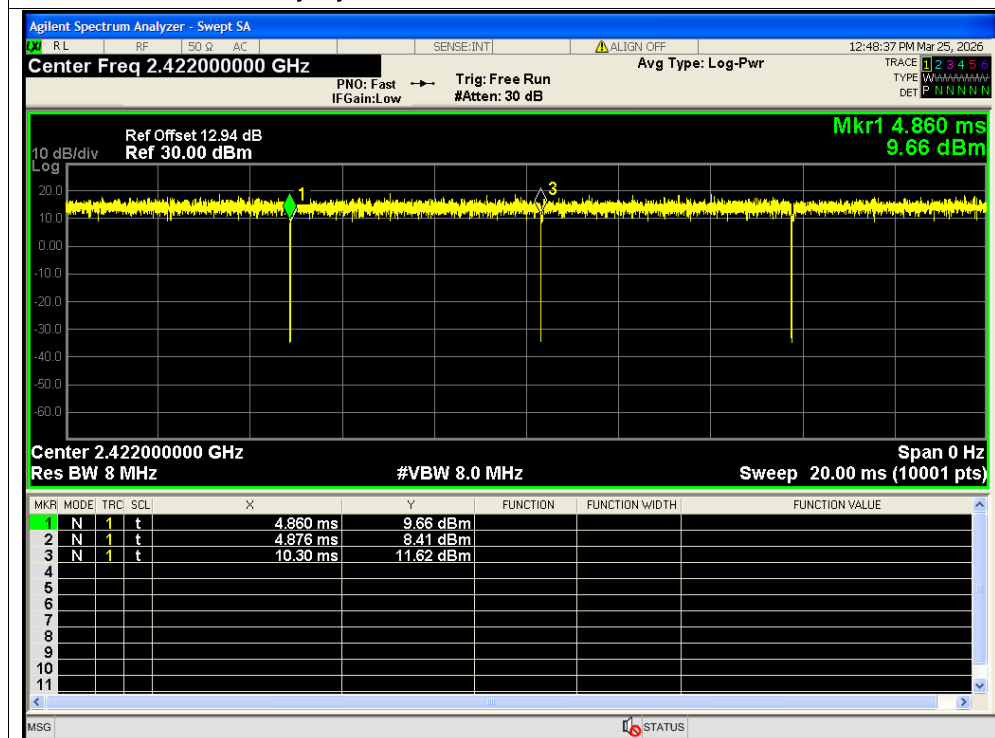
Duty Cycle NVNT n40 2422MHz Sum MIMO
