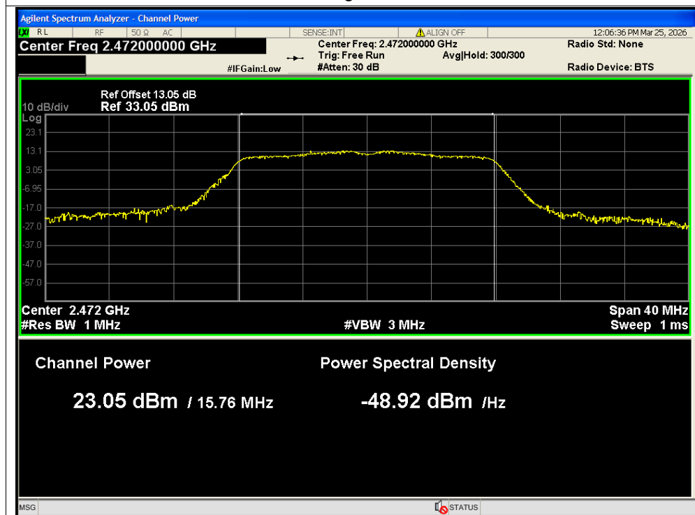
Peak Power NVNT g 2472MHz Ant2 SISO
