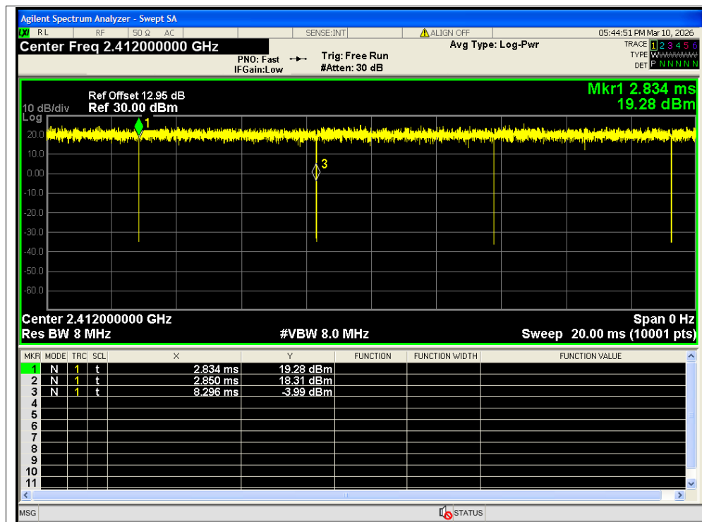
Duty Cycle NVNT ax20 2412MHz Ant1 SISO
