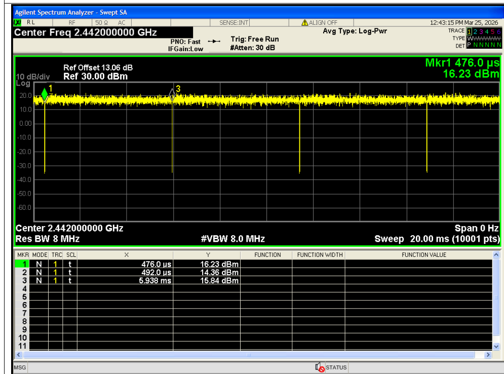
Duty Cycle NVNT ax20 2442MHz Sum MIMO
