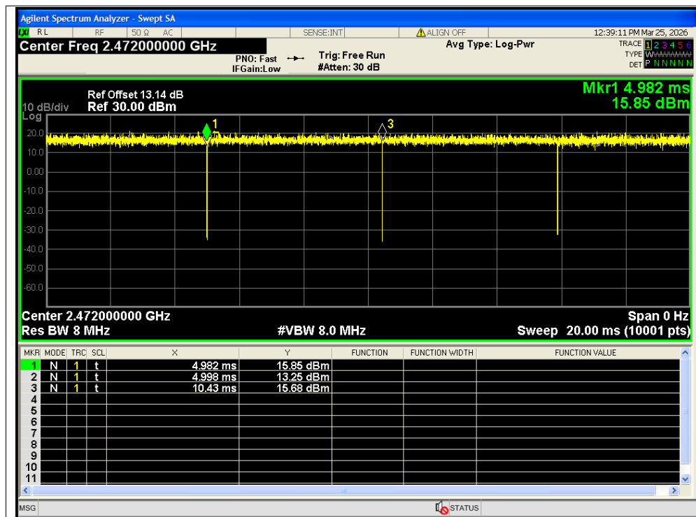
Duty Cycle NVNT n20 2472MHz Sum MIMO
