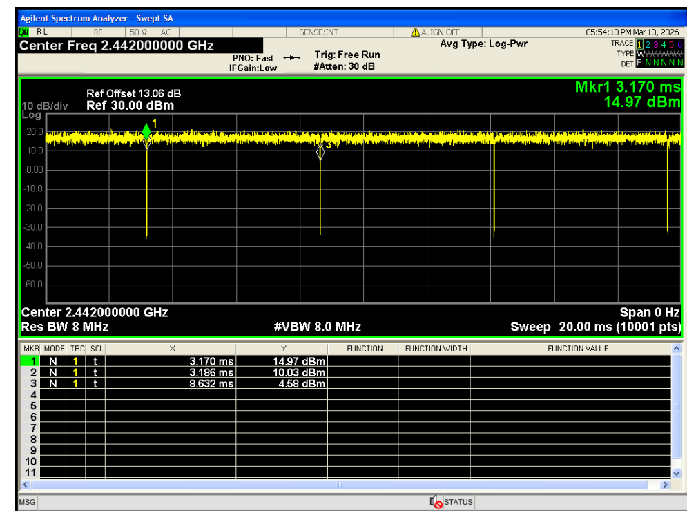
Duty Cycle NVNT ax40 2442MHz Ant1 SISO
