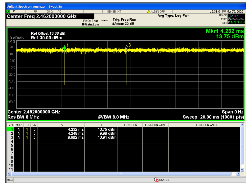
Duty Cycle NVNT ax40 2462MHz Ant2 SISO
