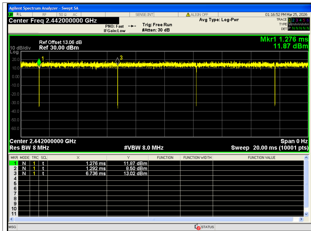
Duty Cycle NVNT ax40 2442MHz Sum MIMO
