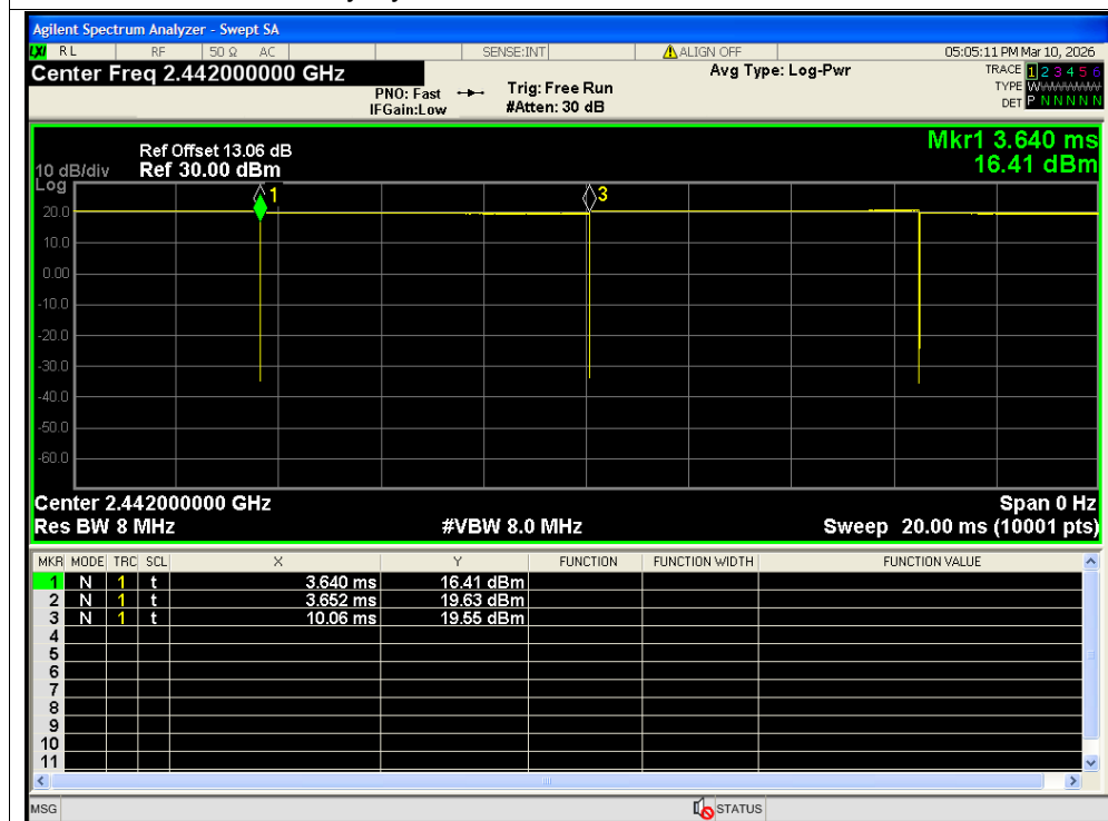
Duty Cycle NVNT b 2442MHz Ant1 SISO
