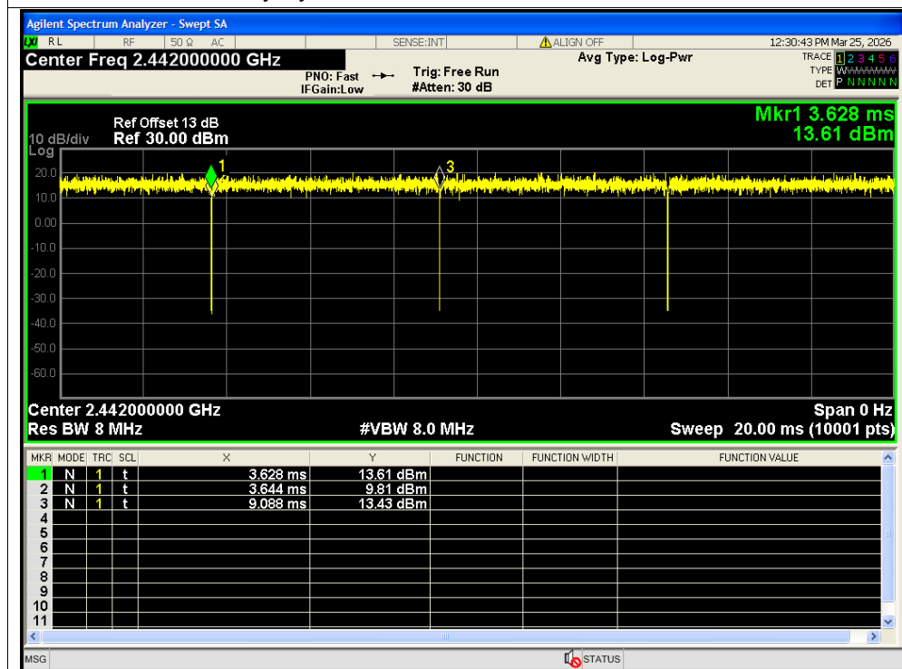
Duty Cycle NVNT ax40 2442MHz Ant2 SISO
