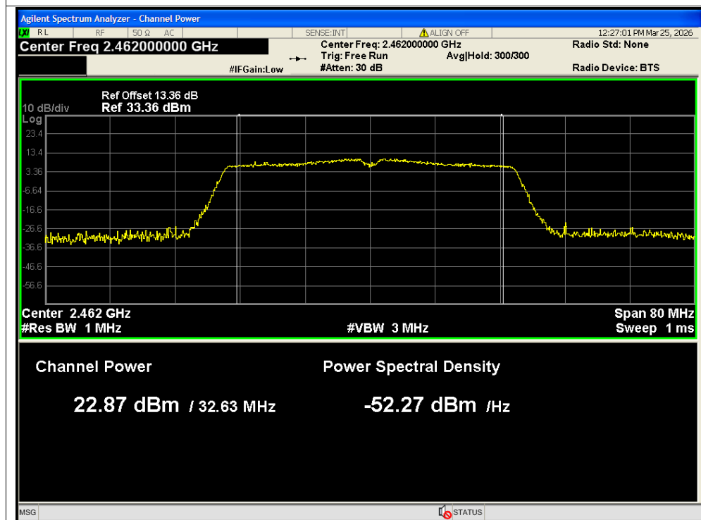
Peak Power NVNT n40 2462MHz Ant2 SISO
