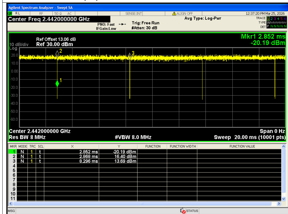
Duty Cycle NVNT n20 2442MHz Sum MIMO
