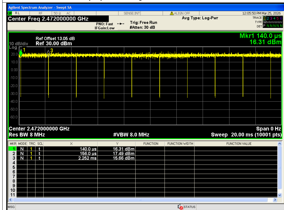
Duty Cycle NVNT g 2472MHz Ant2 SISO
