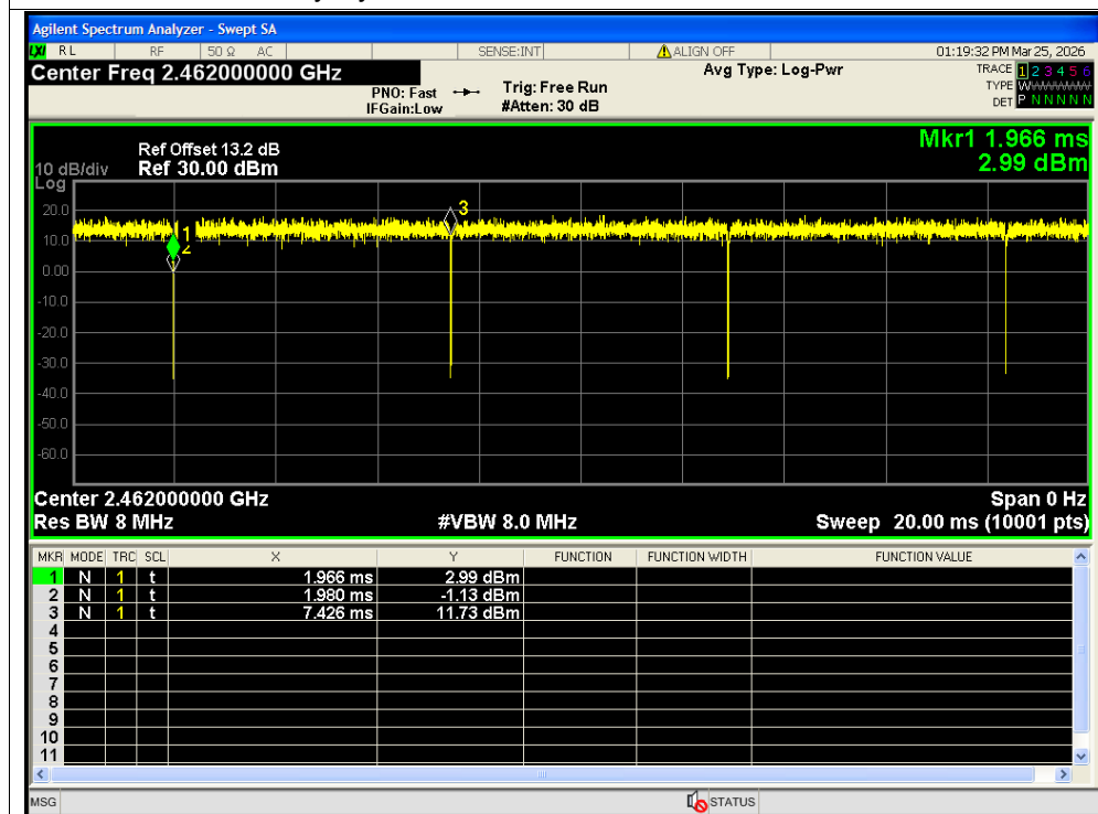
Duty Cycle NVNT ax40 2462MHz Sum MIMO
