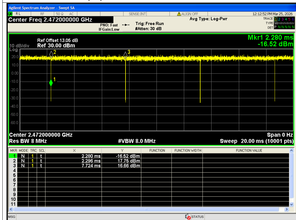
Duty Cycle NVNT n20 2472MHz Ant2 SISO
