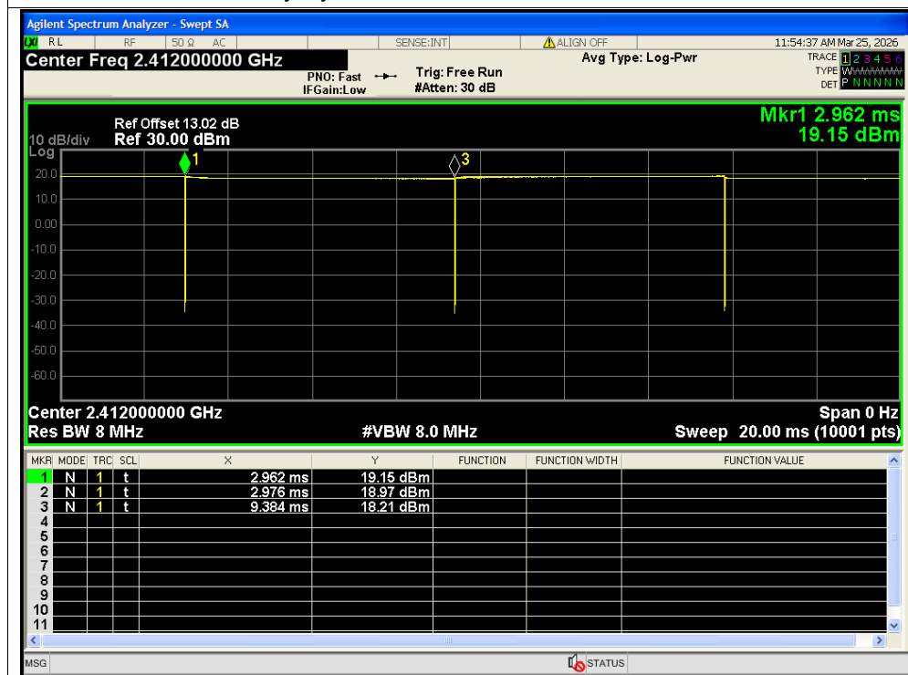
Duty Cycle NVNT b 2412MHz Ant2 SISO
