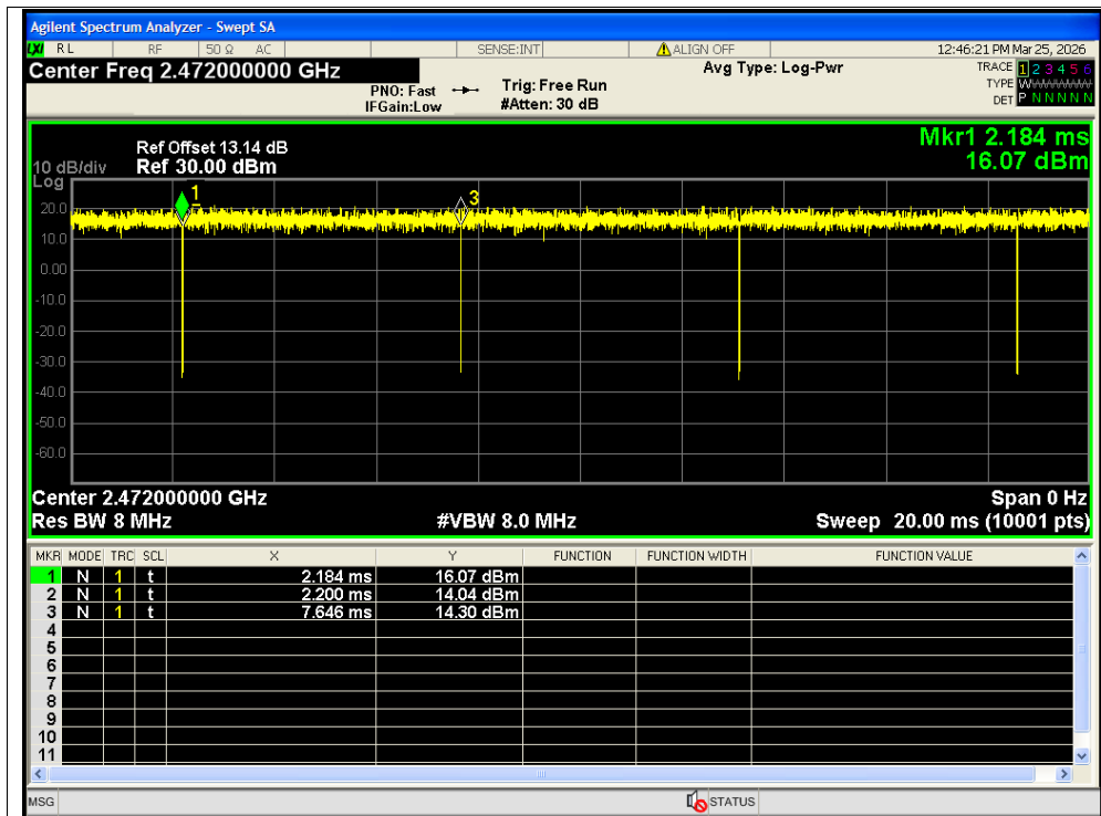
Duty Cycle NVNT ax20 2472MHz Sum MIMO
