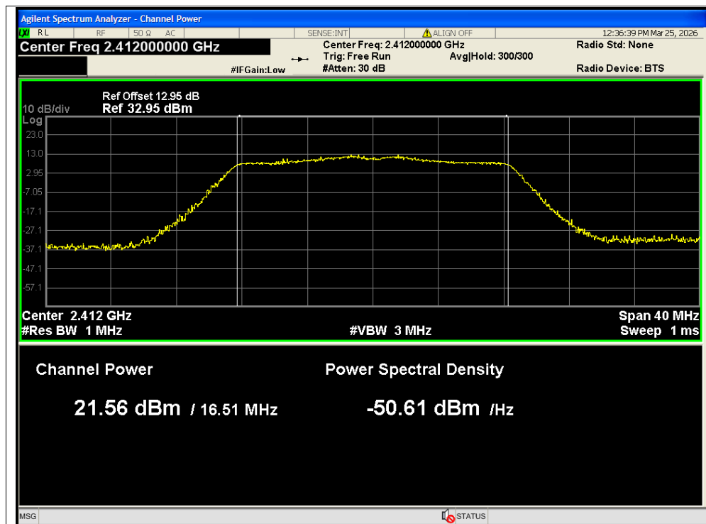
Peak Power NVNT n20 2412MHz Ant1 MIMO
