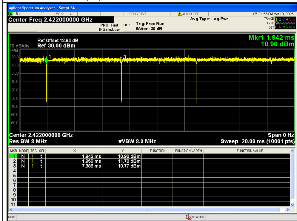
Duty Cycle NVNT n40 2422MHz Ant1 SISO
