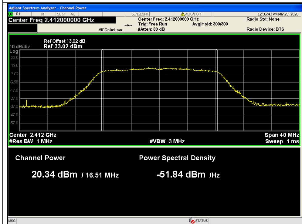
Peak Power NVNT n20 2412MHz Ant2 MIMO
