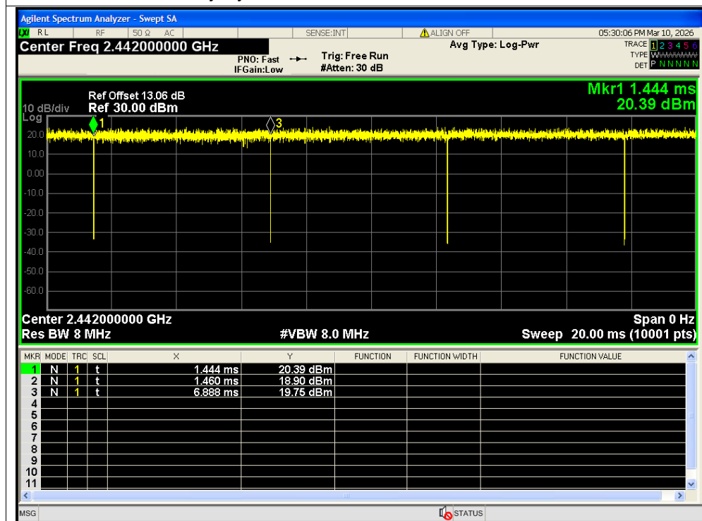
Duty Cycle NVNT n20 2442MHz Ant1 SISO
