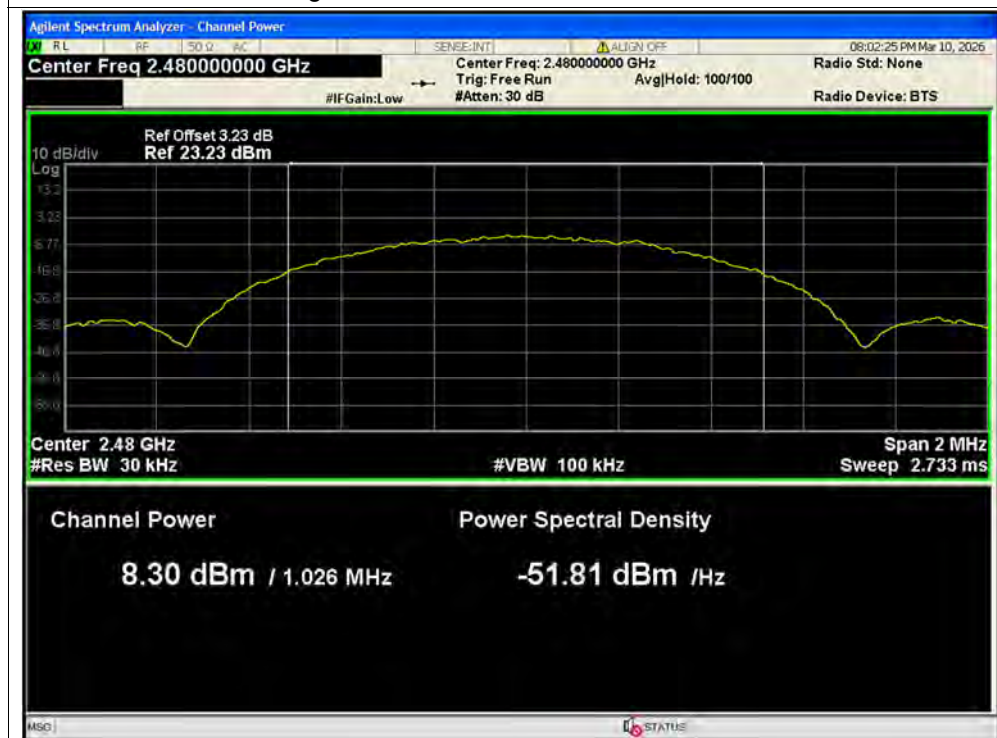
Average Power NVNT BLE 1M 2480MHz Ant2
