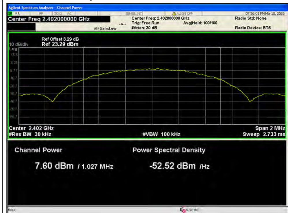
Average Power NVNT BLE 1M 2402MHz Ant2
