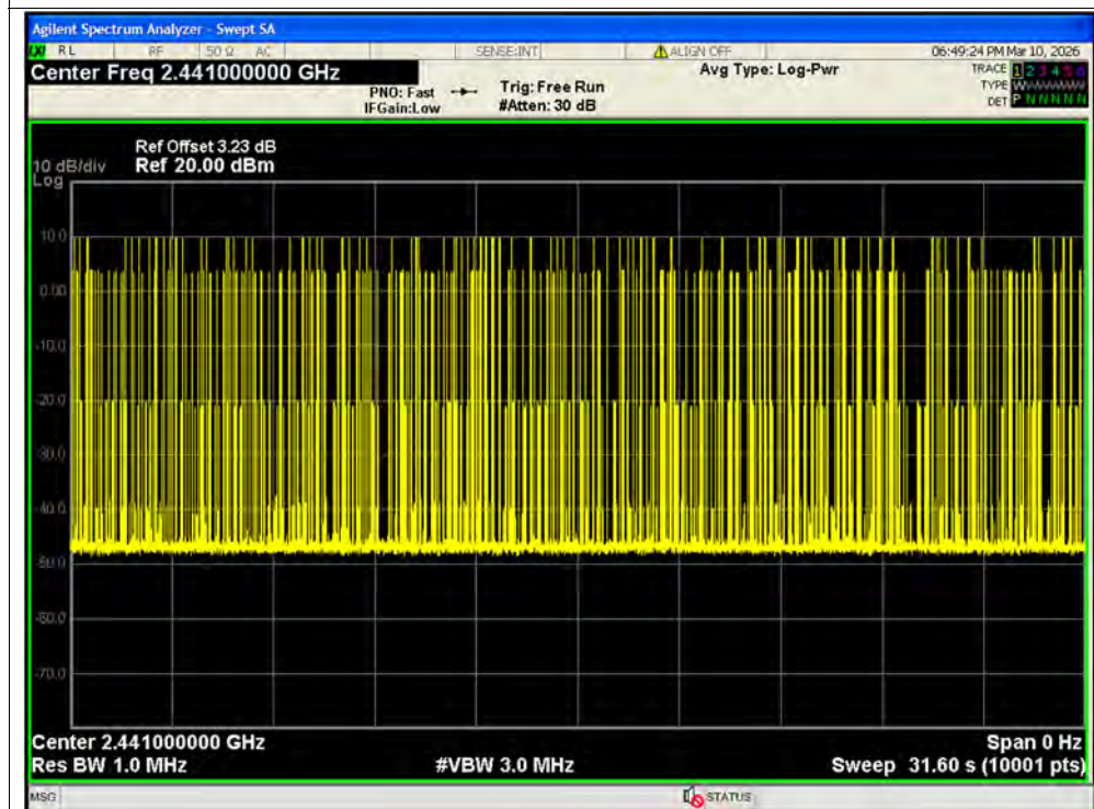
Dwell NVNT 2-DH5 2441MHz Ant2 Accumulated
