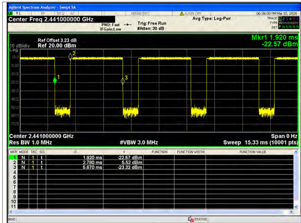
Duty Cycle NVNT 3-DH5 2441MHz Ant2
