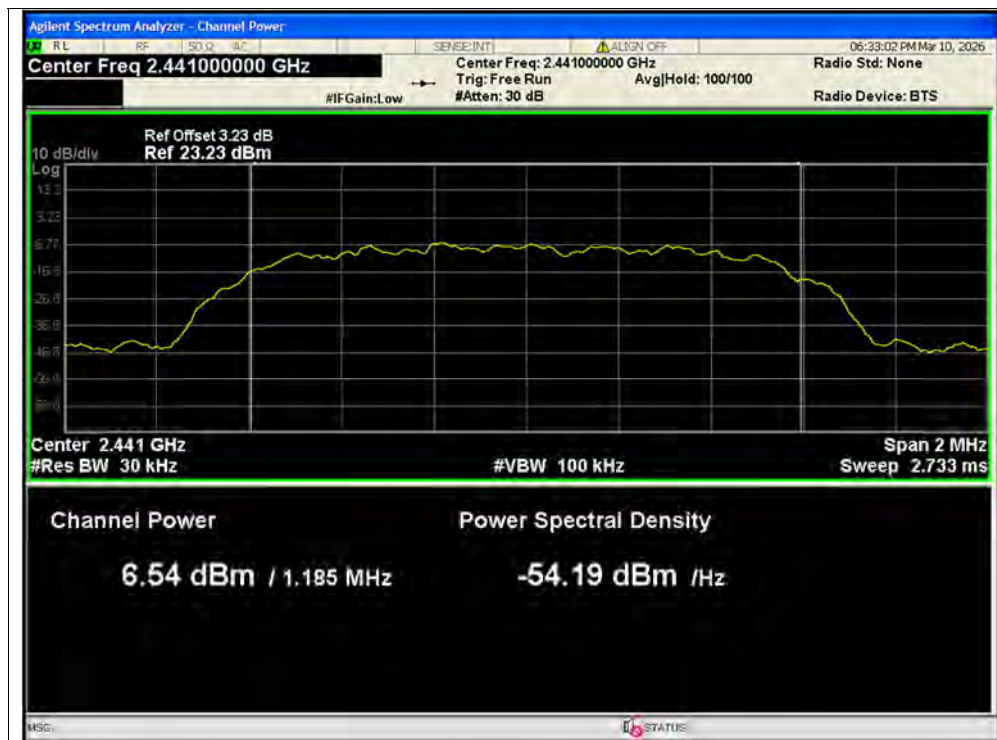
Average Power NVNT 2-DH5 2441MHz Ant2
