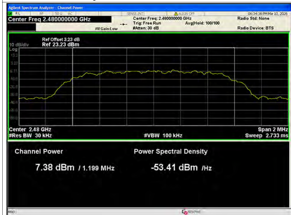
Average Power NVNT 2-DH5 2480MHz Ant2
