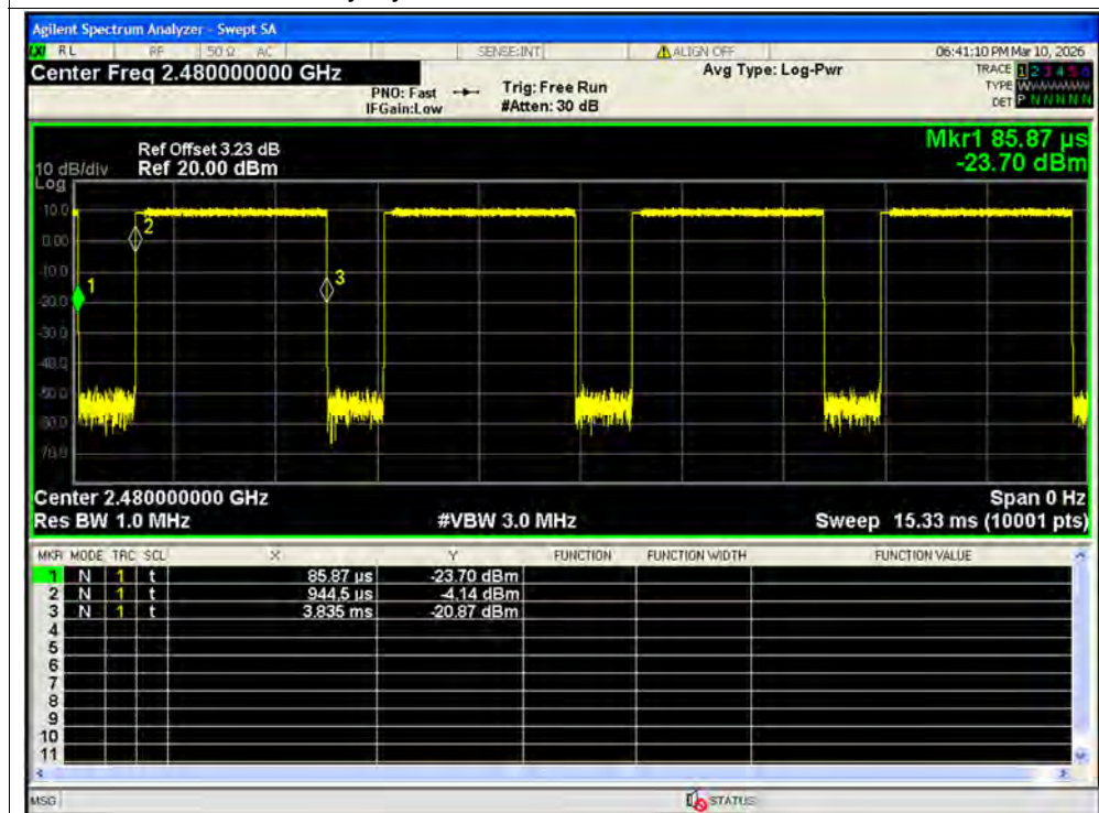
Duty Cycle NVNT 3-DH5 2480MHz Ant2
