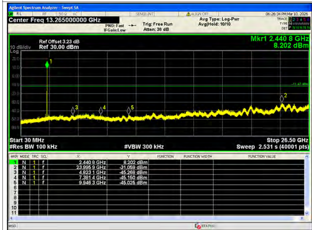
Tx. Spurious NVNT 1-DH5 2441MHz Ant2 Emission
