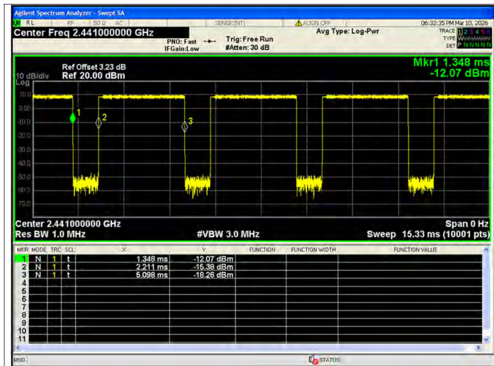
Duty Cycle NVNT 2-DH5 2441MHz Ant2
