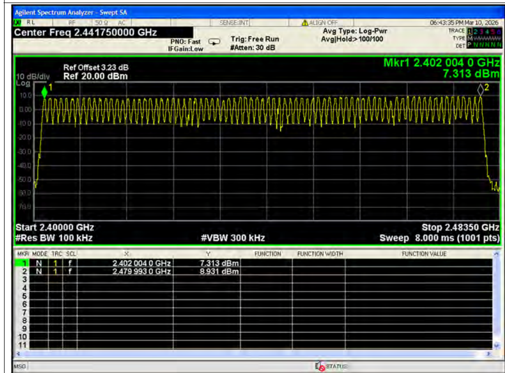
Hopping No. NVNT 1-DH5 2441MHz Ant2
