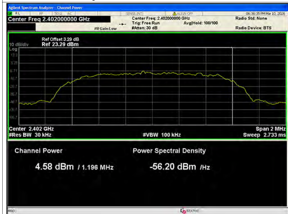
Average Power NVNT 3-DH5 2402MHz Ant2
