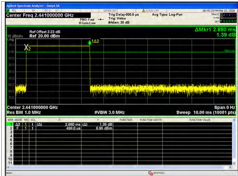
Dwell NVNT 1-DH5 2441MHz Ant2 One Burst
