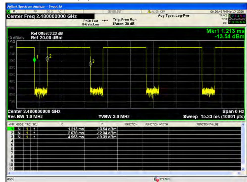
Duty Cycle NVNT 1-DH5 2480MHz Ant2
