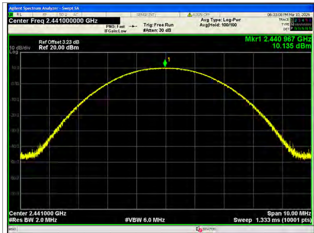
Peak Power NVNT 2-DH5 2441MHz Ant2
