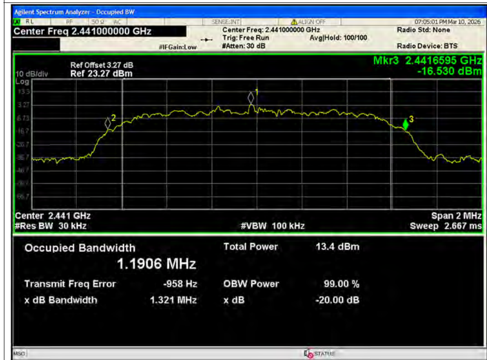
-20dB Bandwidth NVNT 2-DH5 2441MHz Ant1
