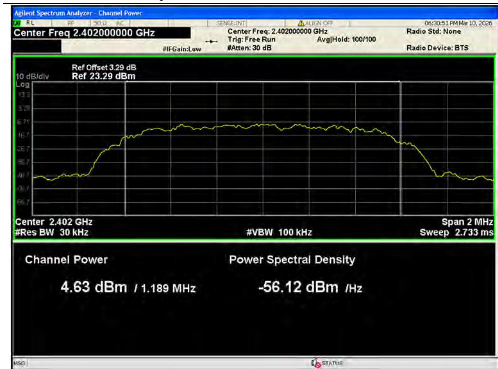
Average Power NVNT 2-DH5 2402MHz Ant2
