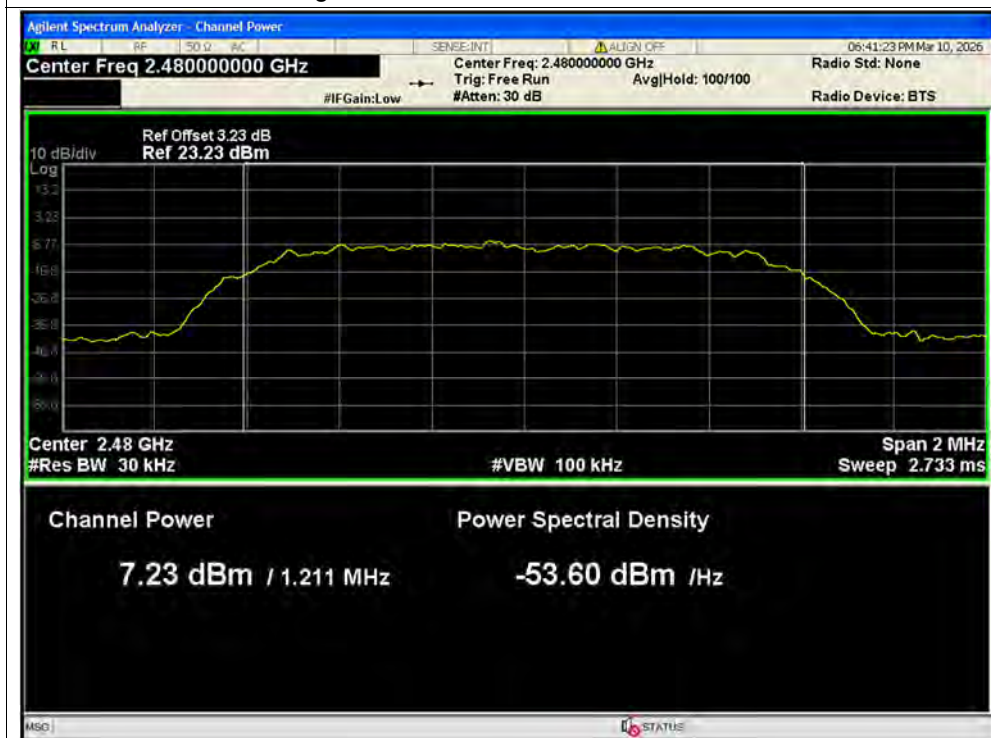
Average Power NVNT 3-DH5 2480MHz Ant2
