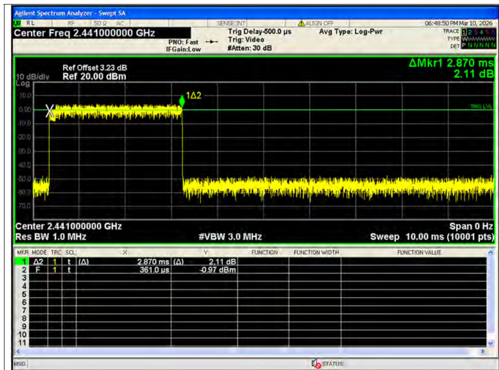
Dwell NVNT 2-DH5 2441MHz Ant2 One Burst
