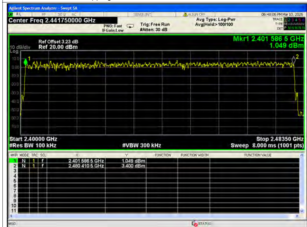
Hopping No. NVNT 2-DH5 2441MHz Ant2
