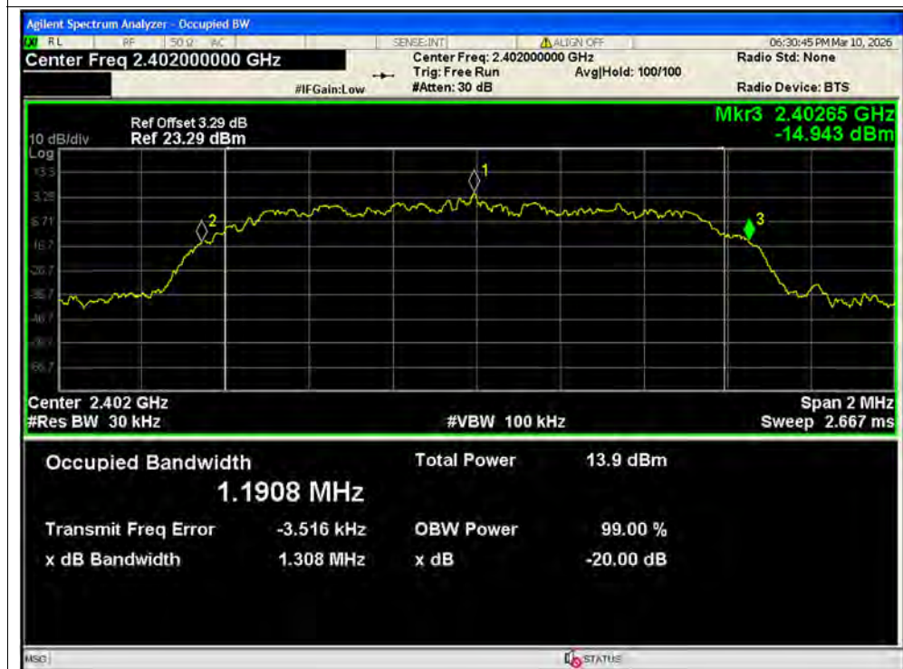
-20dB Bandwidth NVNT 2-DH5 2402MHz Ant2
