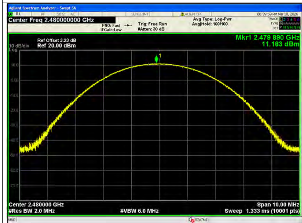
Peak Power NVNT 3-DH5 2480MHz Ant2
