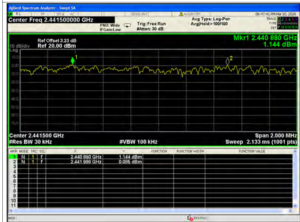
CFS NVNT 2-DH5 2441MHz Ant2
