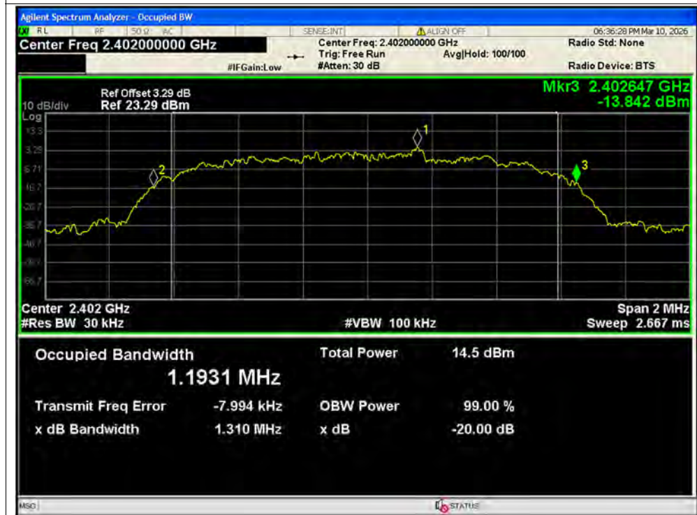
-20dB Bandwidth NVNT 3-DH5 2402MHz Ant2
