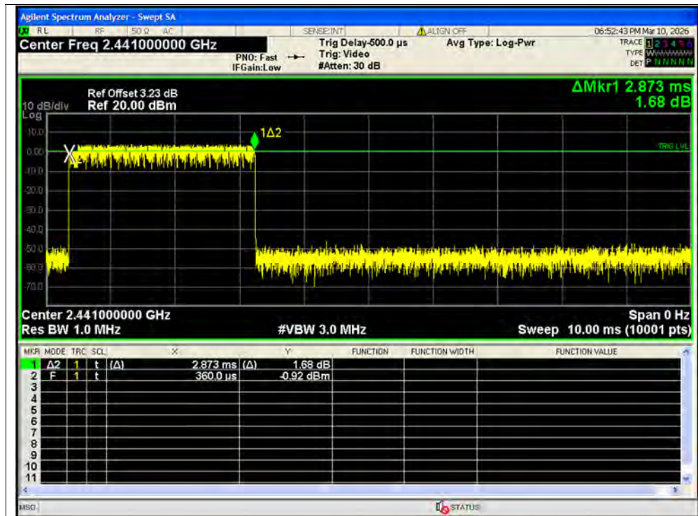
Dwell NVNT 3-DH5 2441MHz Ant2 One Burst
