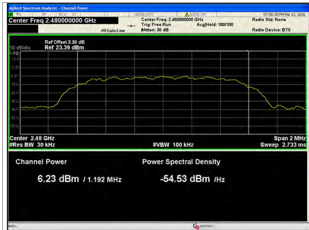
Average Power NVNT 2-DH5 2480MHz Ant1
