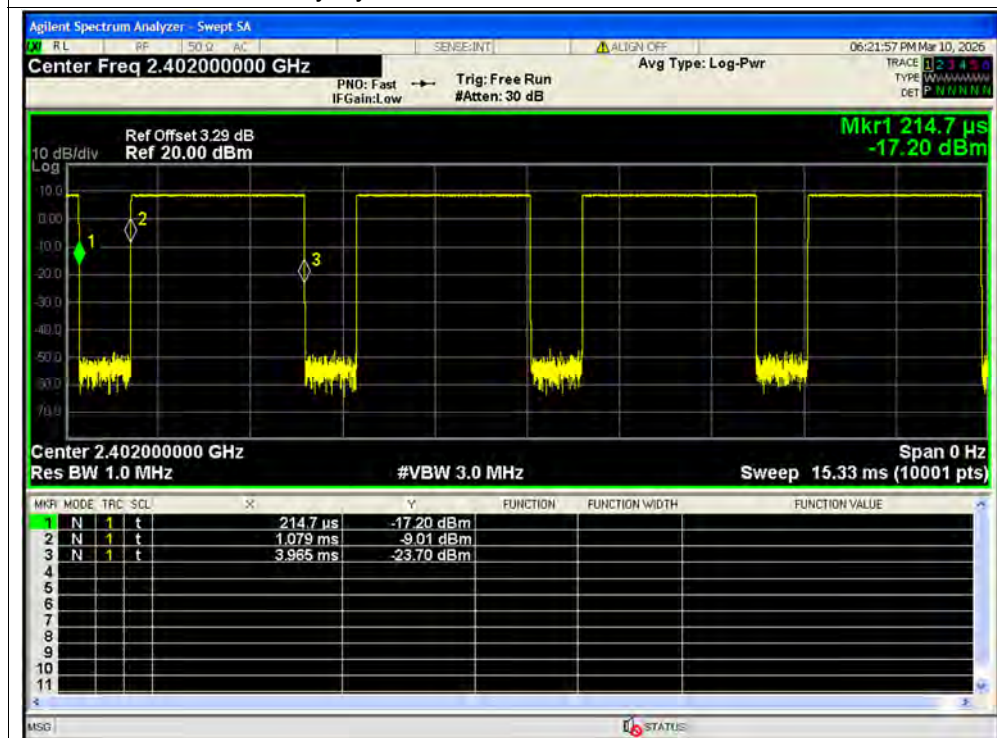
Duty Cycle NVNT 1-DH5 2402MHz Ant2
