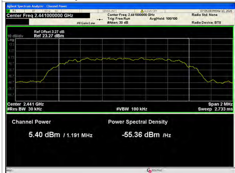
Average Power NVNT 2-DH5 2441MHz Ant1
