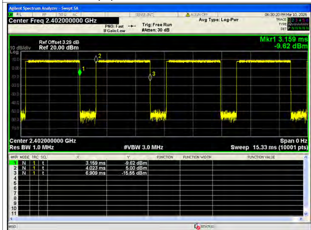
Duty Cycle NVNT 2-DH5 2402MHz Ant2
