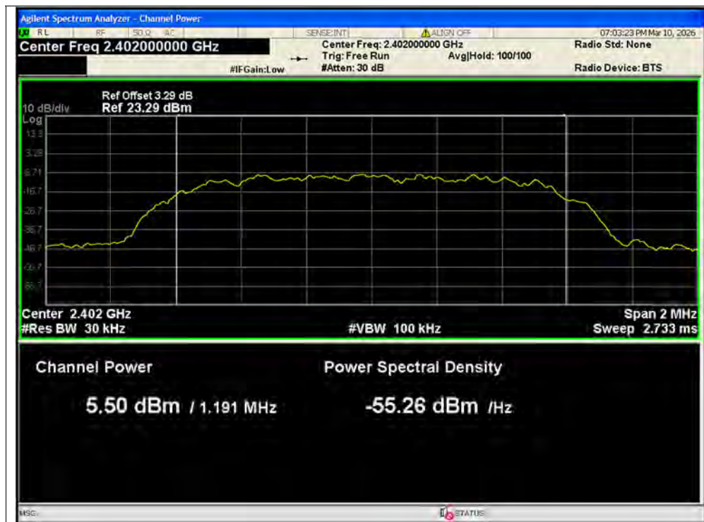
Average Power NVNT 2-DH5 2402MHz Ant1
