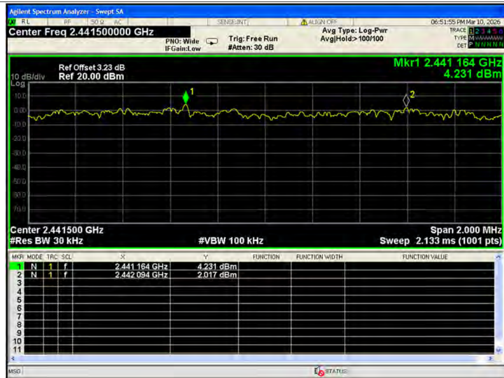
CFS NVNT 3-DH5 2441MHz Ant2
