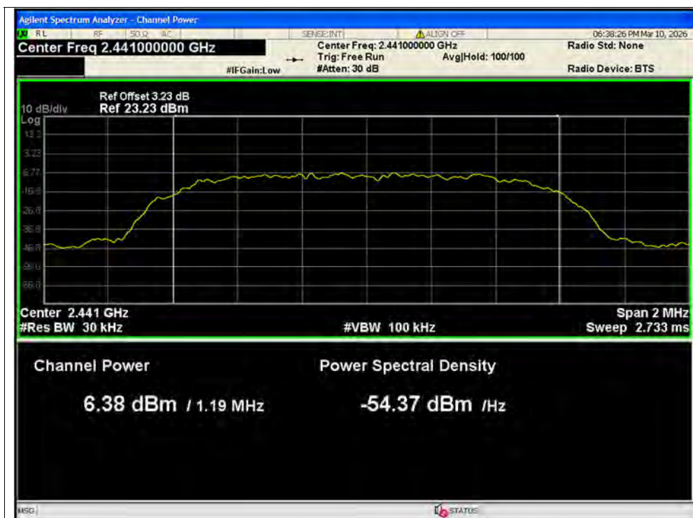
Average Power NVNT 3-DH5 2441MHz Ant2
