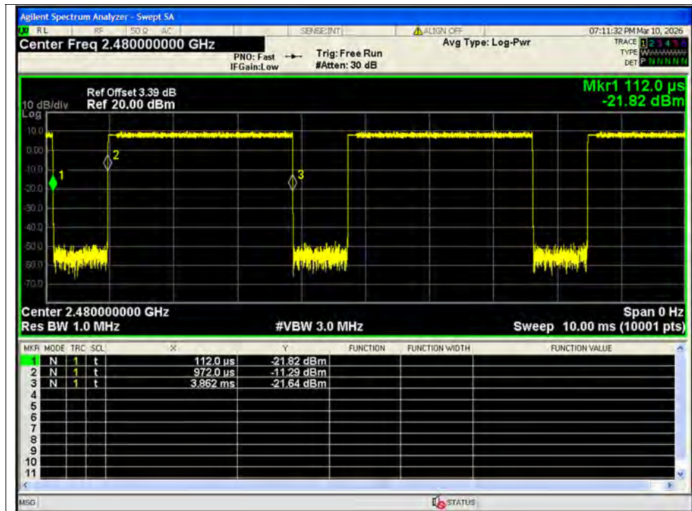
Duty Cycle NVNT 3-DH5 2480MHz Ant1
