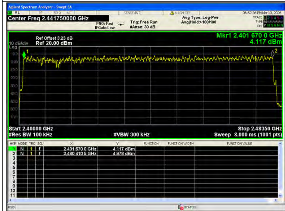
Hopping No. NVNT 3-DH5 2441MHz Ant2
