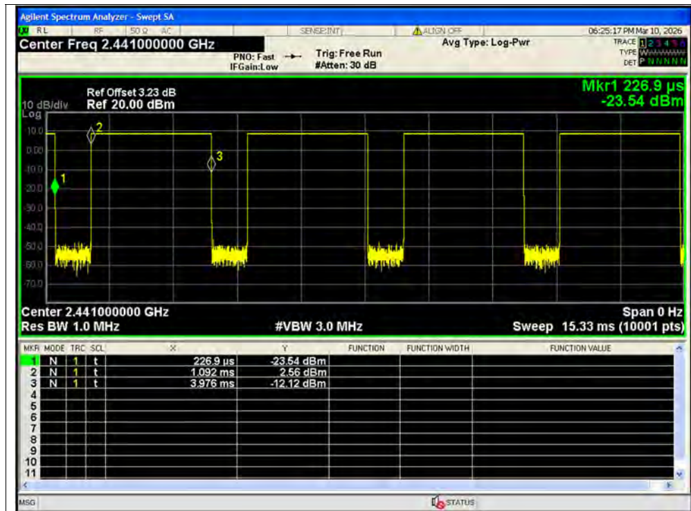
Duty Cycle NVNT 1-DH5 2441MHz Ant2
