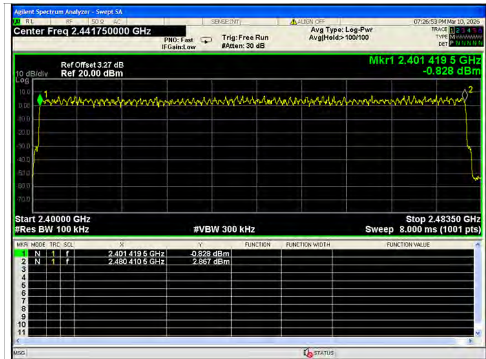
Hopping No. NVNT 3-DH5 2441MHz Ant1
