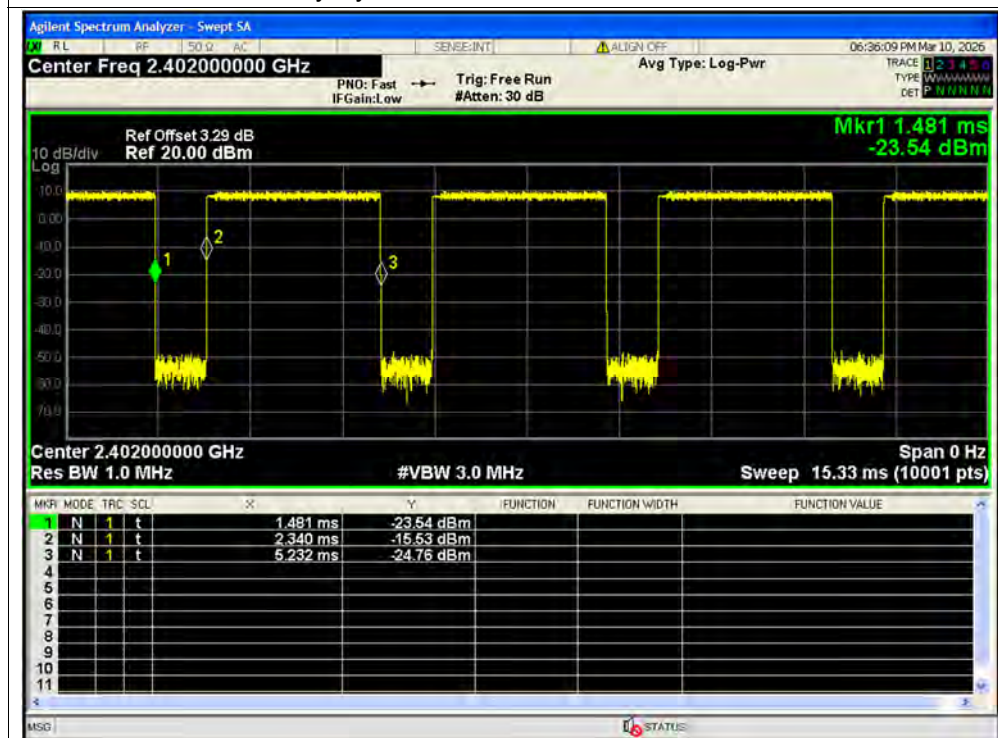
Duty Cycle NVNT 3-DH5 2402MHz Ant2
