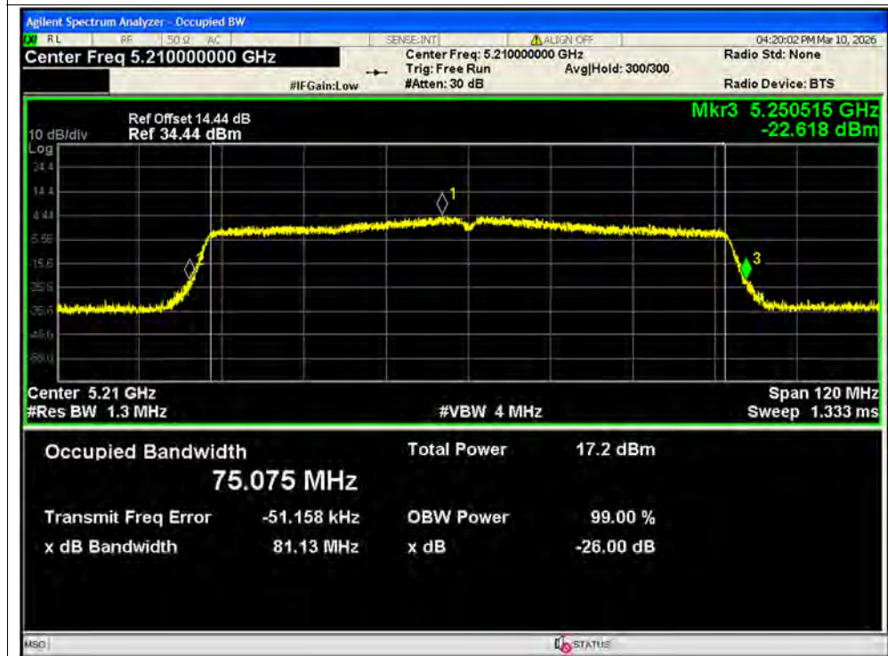
-26dB Bandwidth NVNT ac80 5210MHz Ant2 MIMO
