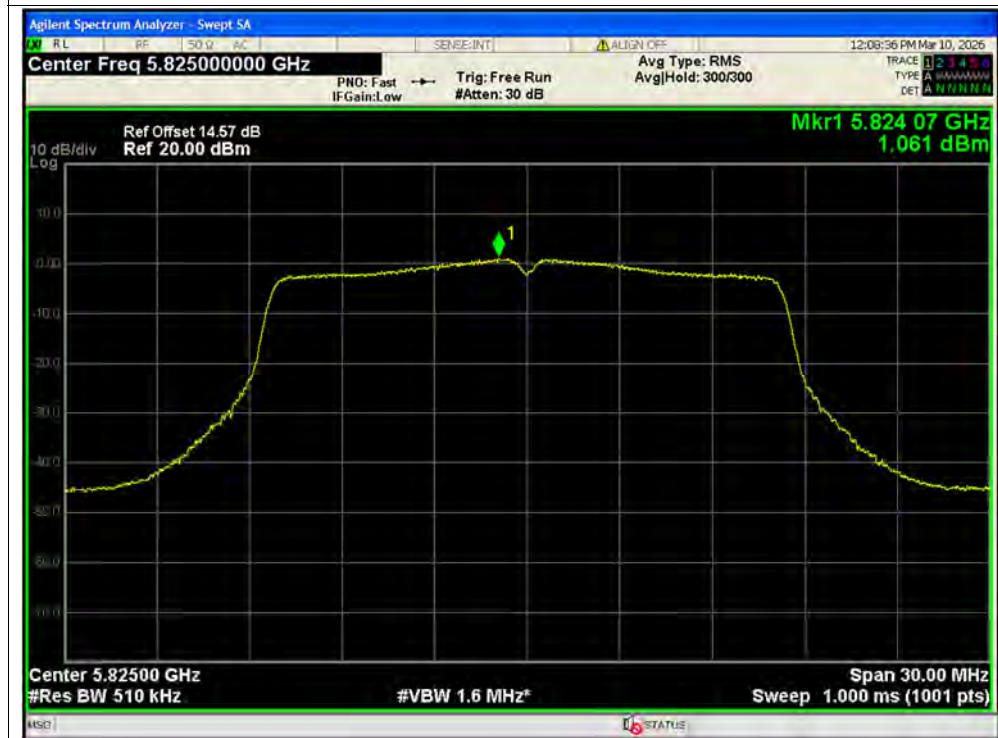
PSD NVNT a 5825MHz Ant1 SISO
