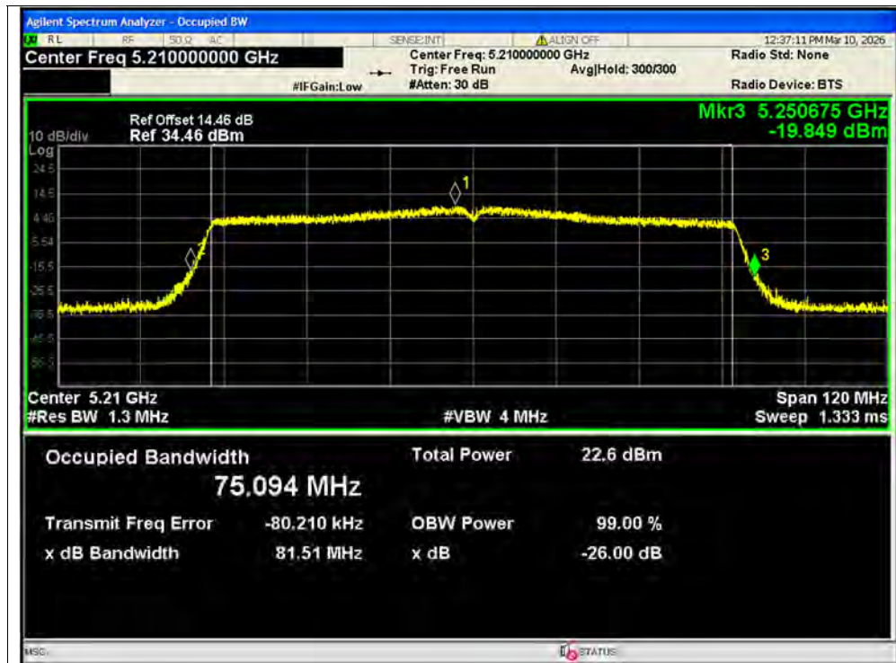
-26dB Bandwidth NVNT ac80 5210MHz Ant1 SISO
