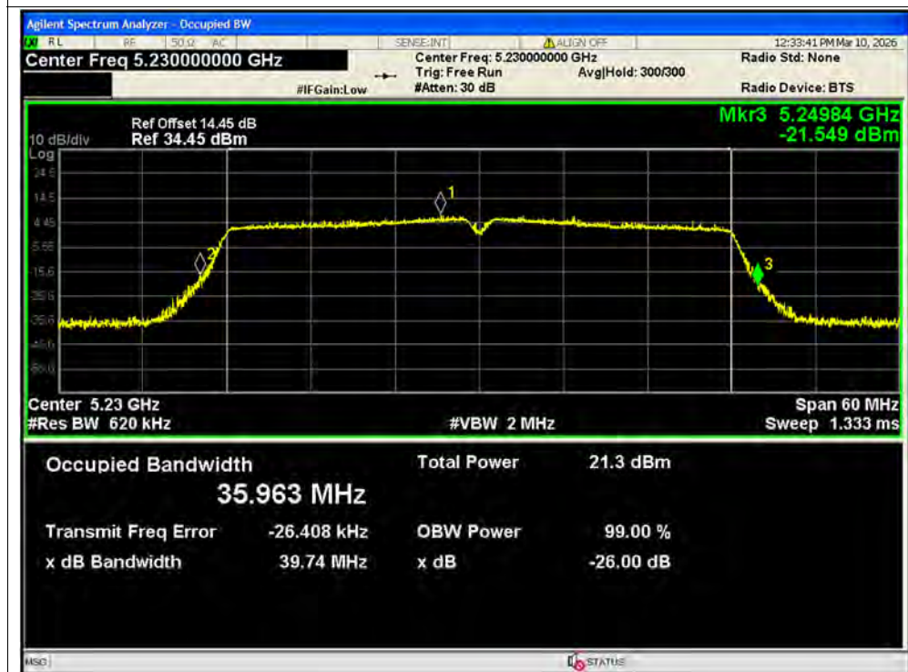
-26dB Bandwidth NVNT ac40 5230MHz Ant1 SISO
