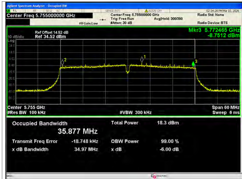
-6dB Bandwidth NVNT n40 5755MHz Ant2 SISO
