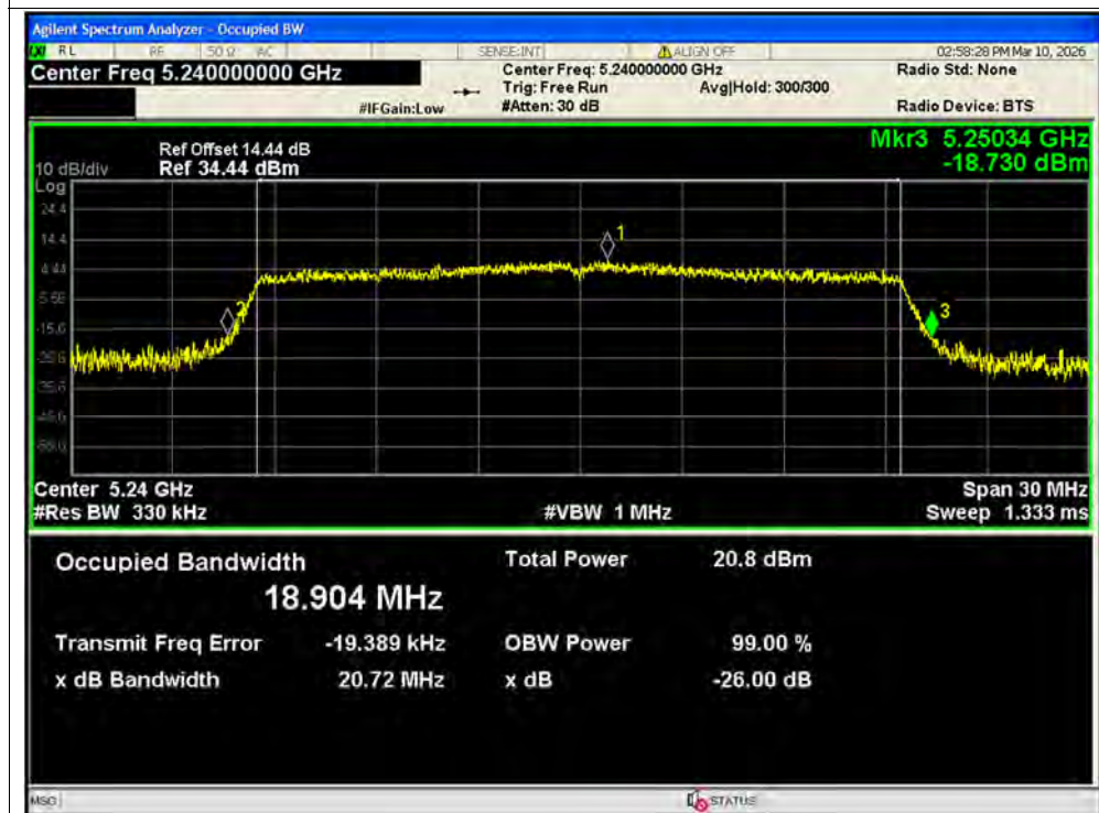
-26dB Bandwidth NVNT ax20 5240MHz Ant2 SISO
