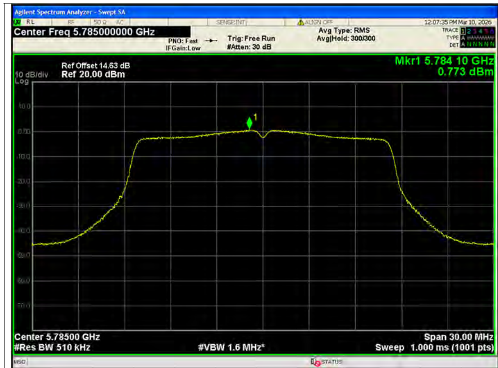
PSD NVNT a 5785MHz Ant1 SISO
