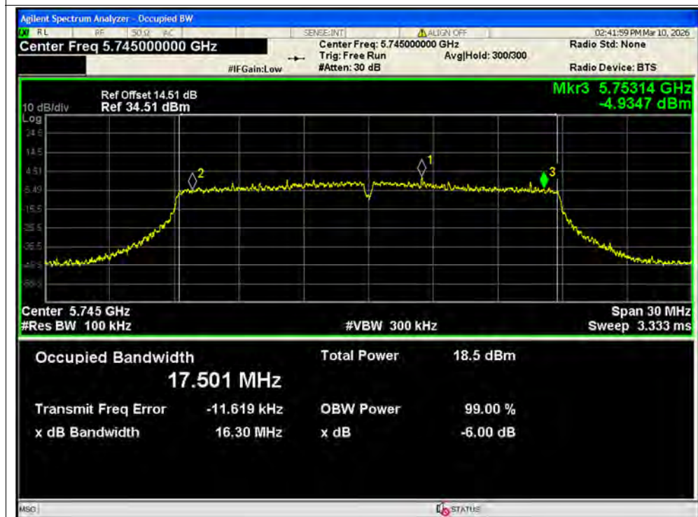
-6dB Bandwidth NVNT ac20 5745MHz Ant2 SISO
