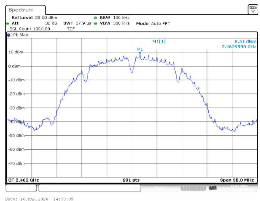
Tx. Spurious NVNT b 2462MHz Ant1 Ref
