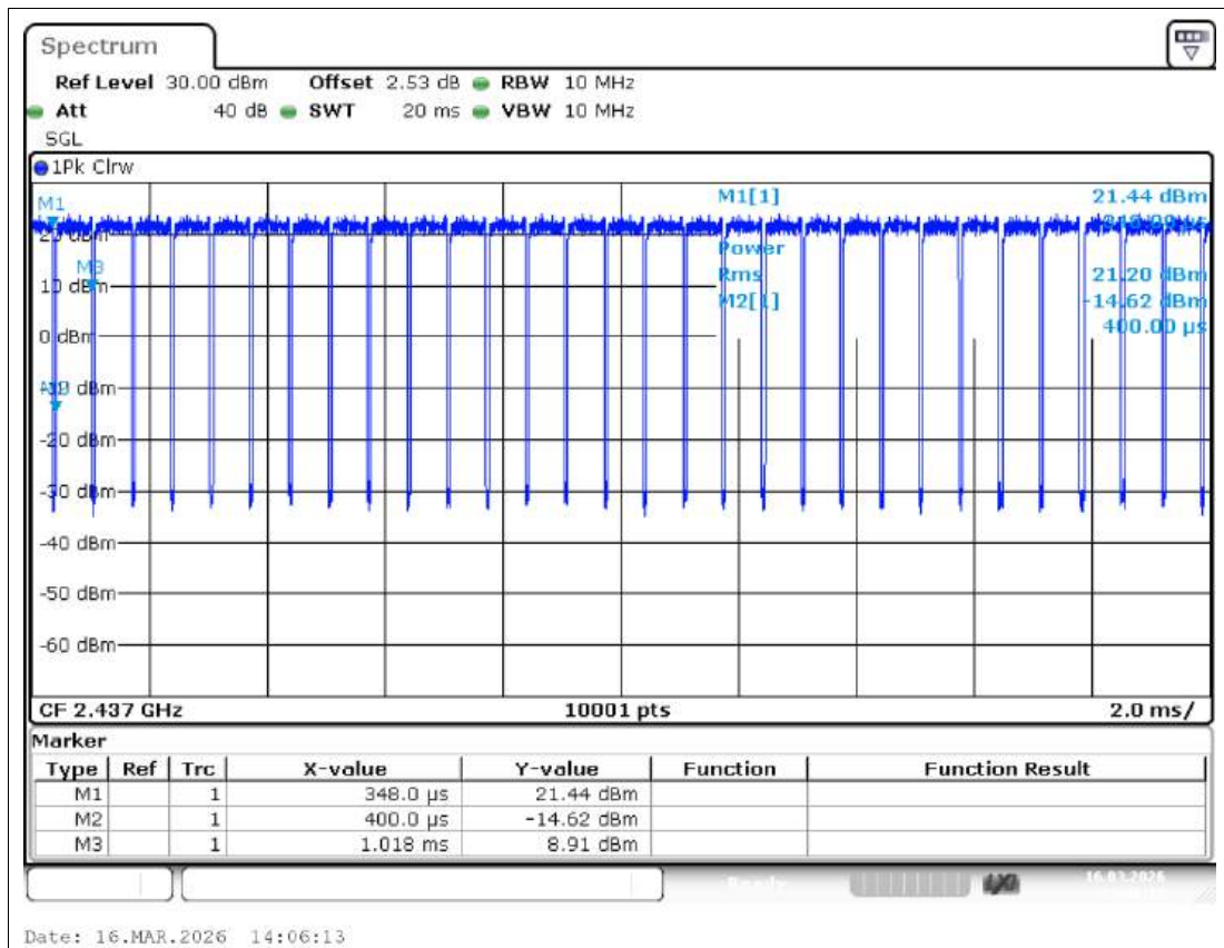
Duty Cycle NVNT g 2437MHz Ant1
