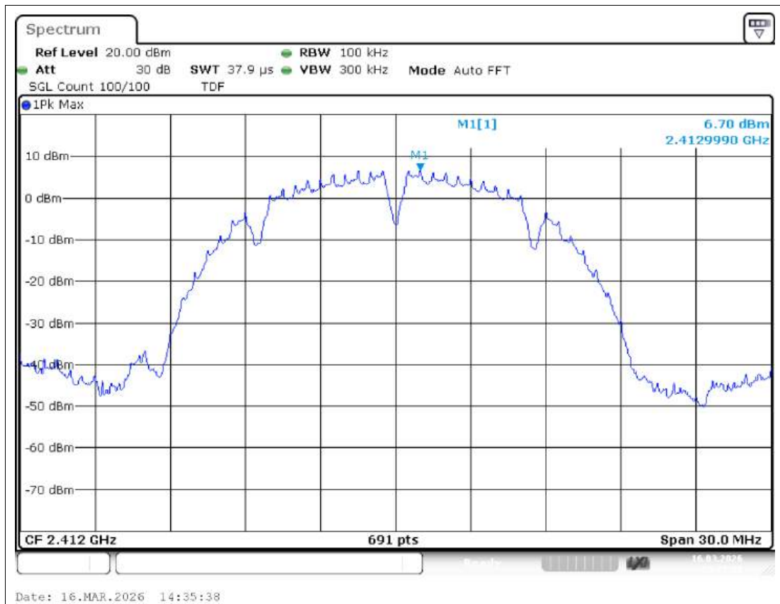
Tx. Spurious NVNT b 2412MHz Ant1 Ref
