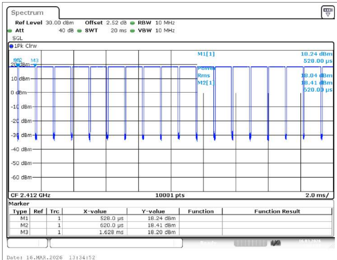
Duty Cycle NVNT b 2412MHz Ant1
