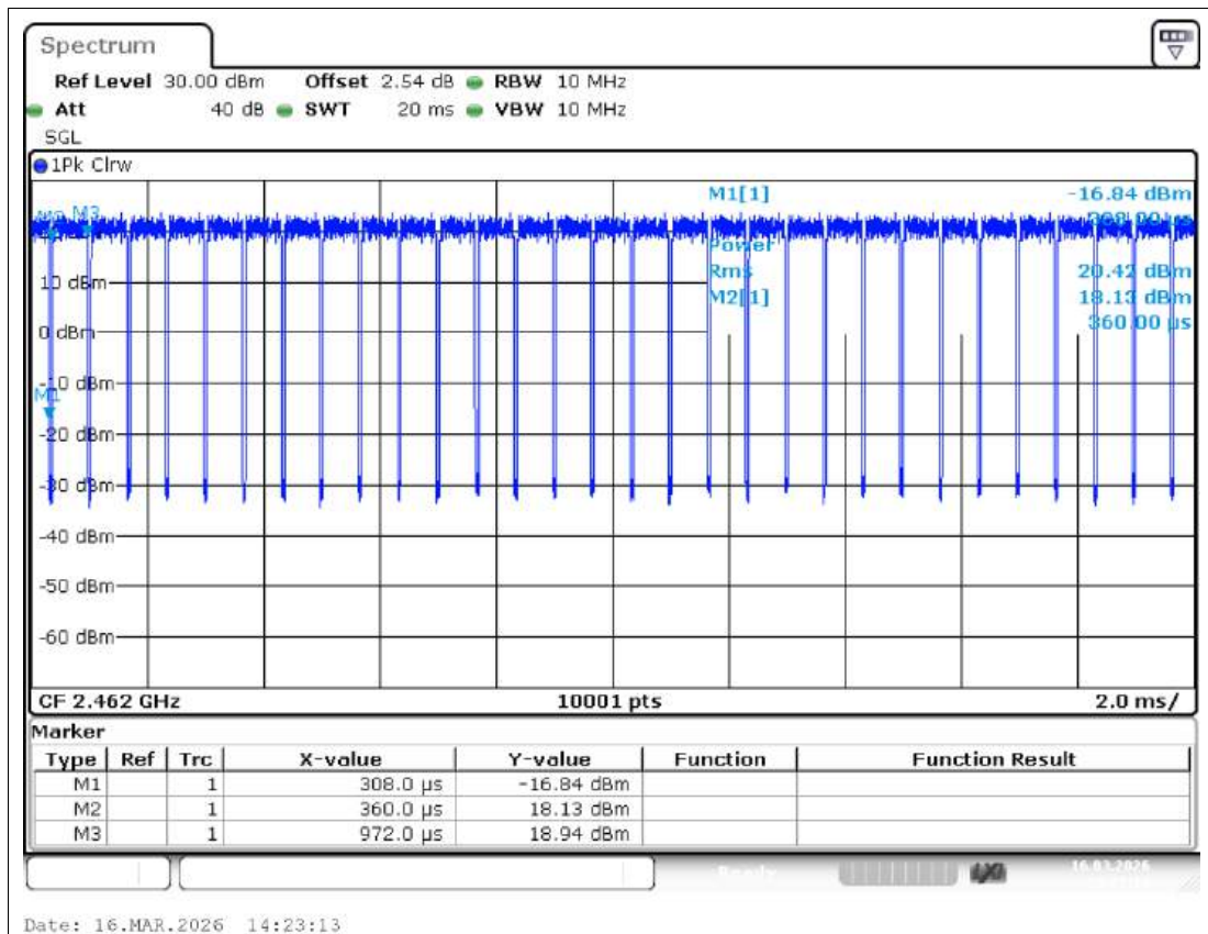
Duty Cycle NVNT n20 2462MHz Ant1
