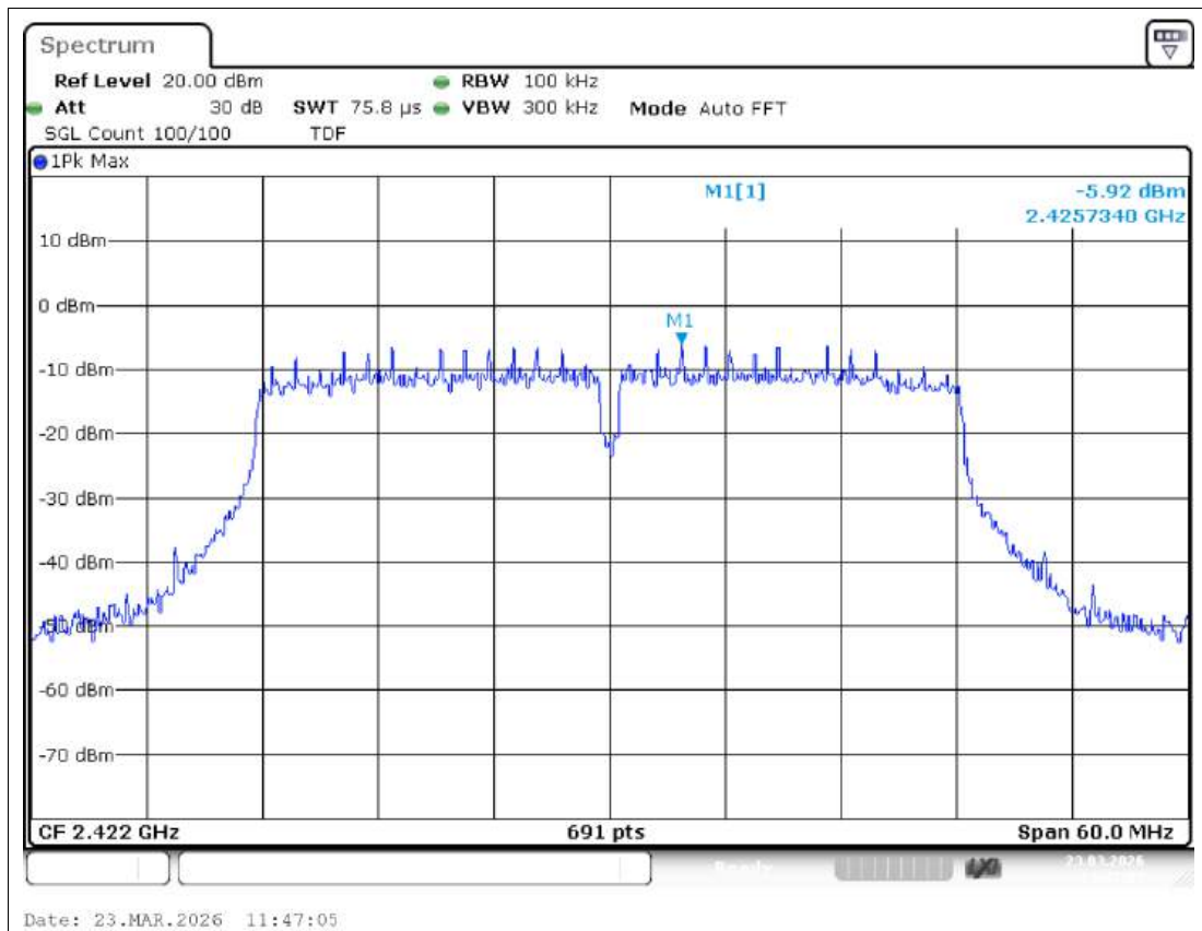
Tx. Spurious NVNT n40 2422MHz Ant1 Ref
