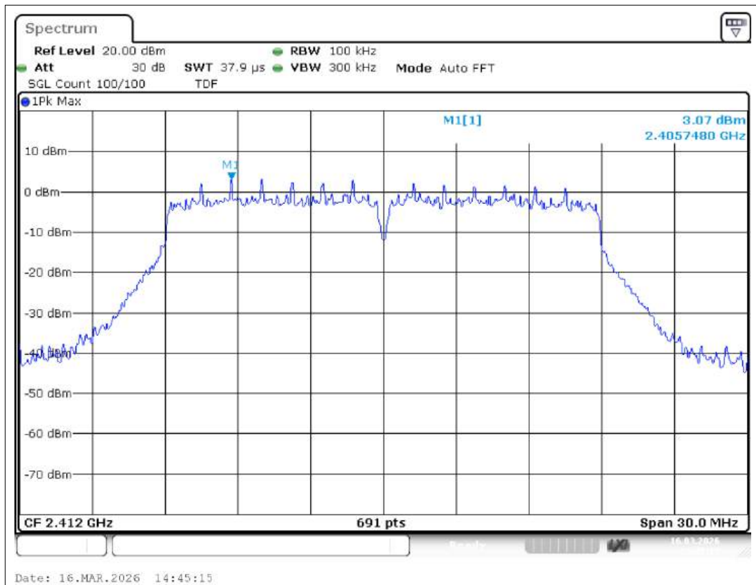
Tx. Spurious NVNT n20 2412MHz Ant1 Ref
