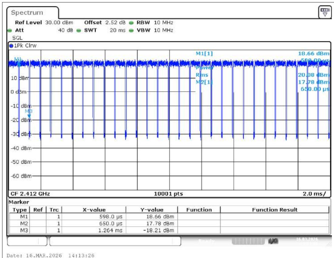
Duty Cycle NVNT n20 2412MHz Ant1
