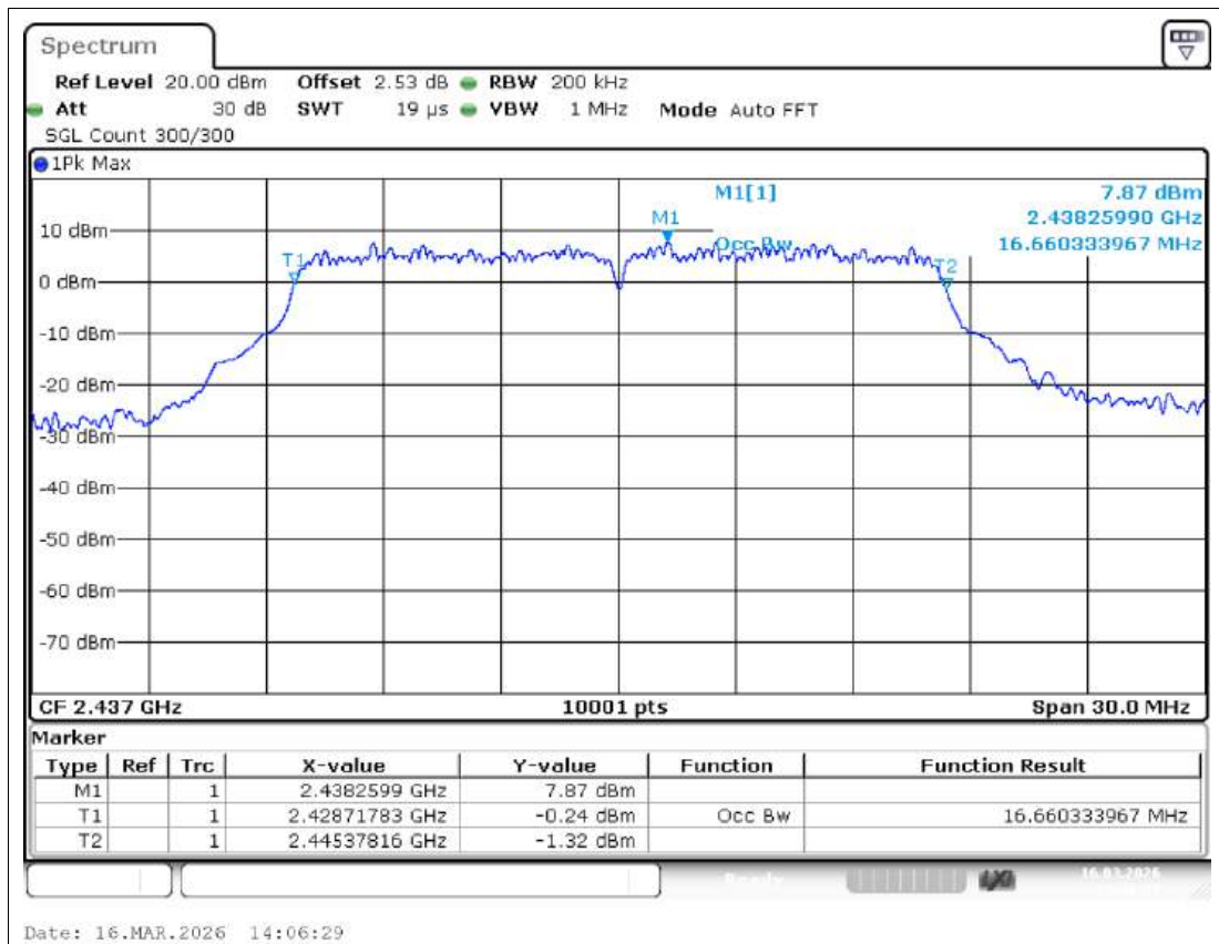
OBW NVNT g 2437MHz Ant1
