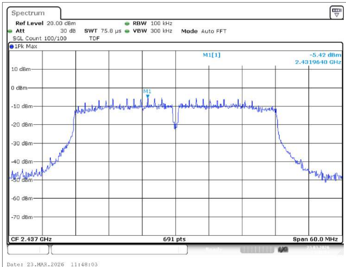
Tx. Spurious NVNT n40 2437MHz Ant1 Ref
