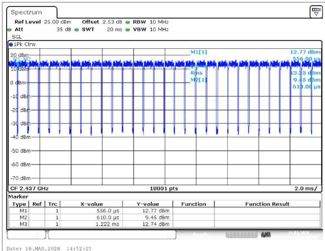
Duty Cycle NVNT n40 2437MHz Ant1
