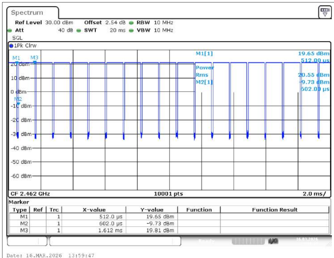
Duty Cycle NVNT b 2462MHz Ant1
