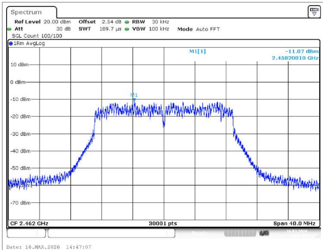
PSD NVNT n20 2462MHz Ant1
