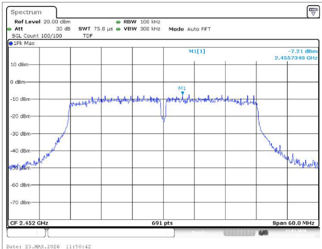
Tx. Spurious NVNT n40 2452MHz Ant1 Ref
