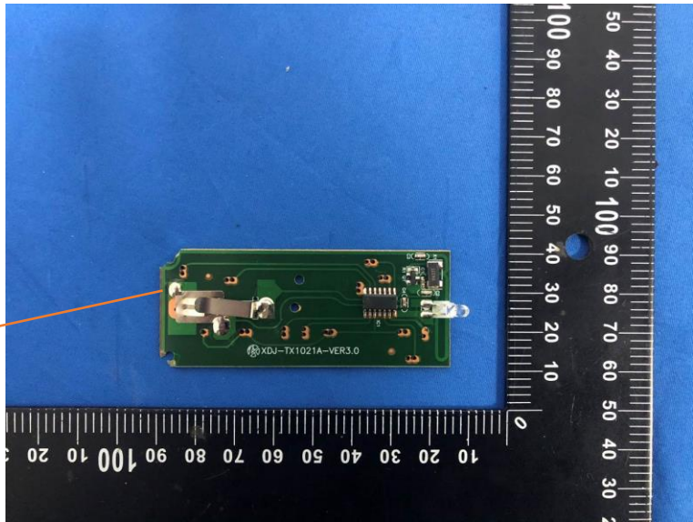
433MHz ANT
