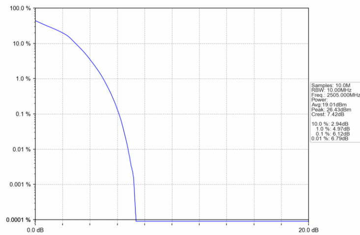
Band7_10MHz_16QAM_LCH_2505MHz_RB_50_0_NTNV
