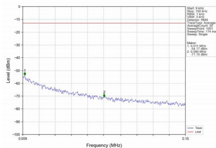
Band2_15MHz_16QAM_HCH_1902.5MHz_RB_1_0_NTNV
