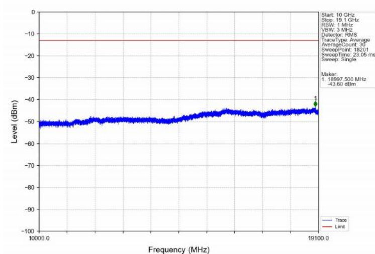
Band2_15MHz_16QAM_HCH_1902.5MHz_RB_1_0_NTNV
