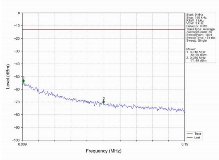
Band2_15MHz_16QAM_LCH_1857.5MHz_RB_1_0_NTNV
