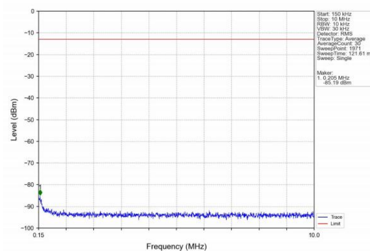
Band2_15MHz_16QAM_MCH_1880MHz_RB_1_0_NTNV
