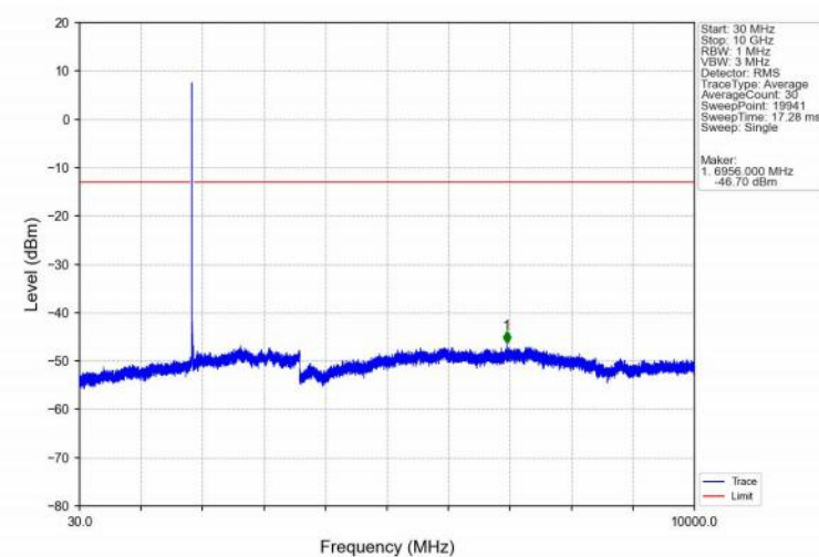
Band2_15MHz_16QAM_LCH_1857.5MHz_RB_1_0_NTNV
