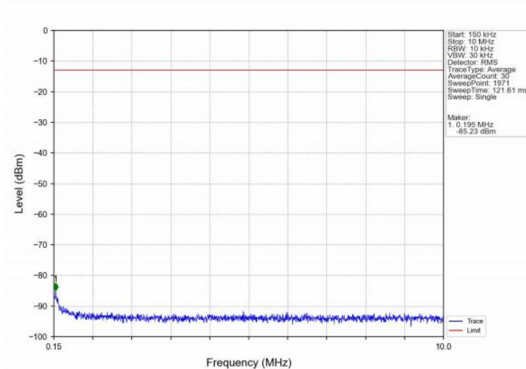
Band2_15MHz_16QAM_LCH_1857.5MHz_RB_1_0_NTNV
