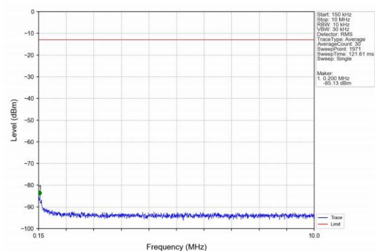
Band2_15MHz_16QAM_HCH_1902.5MHz_RB_1_0_NTNV
