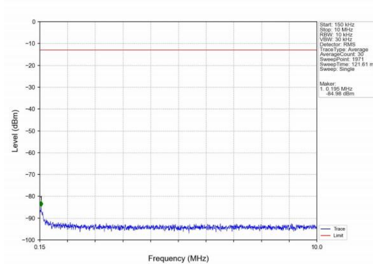
Band4_10MHz_16QAM_LCH_1715MHz_RB_1_0_NTNV
