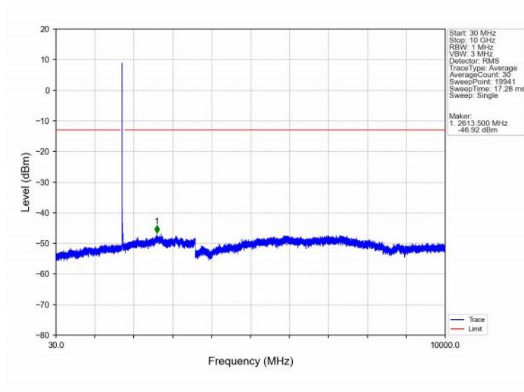
Band4_15MHz_QPSK_MCH_1732.5MHz_RB_1_0_NTNV
