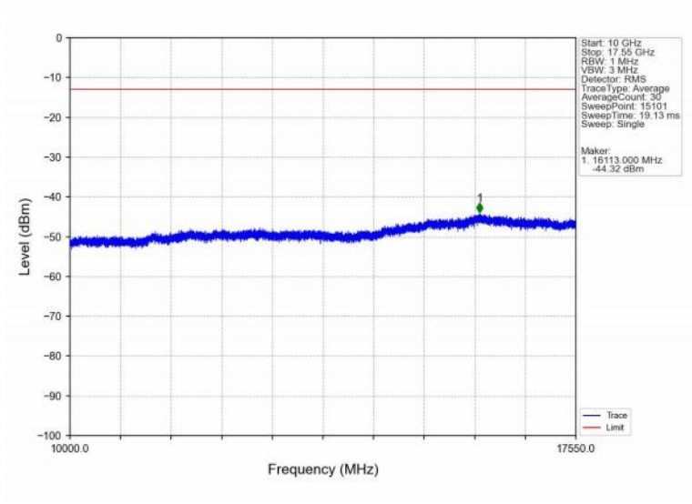
Band4_15MHz_16QAM_LCH_1717.5MHz_RB_75_0_NTNV
