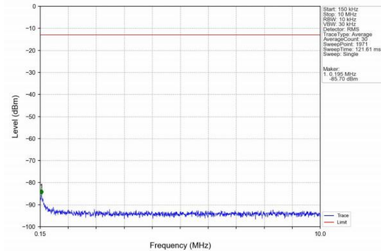
Band4_15MHz_16QAM_MCH_1732.5MHz_RB_1_0_NTNV
