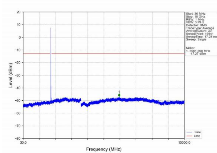
Band4_15MHz_16QAM_HCH_1747.5MHz_RB_1_0_NTNV
