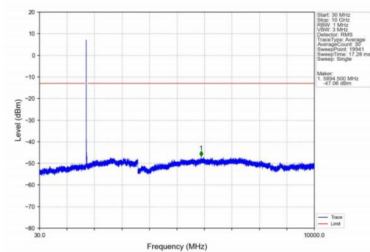
Band4_15MHz_16QAM_MCH_1732.5MHz_RB_1_0_NTNV
