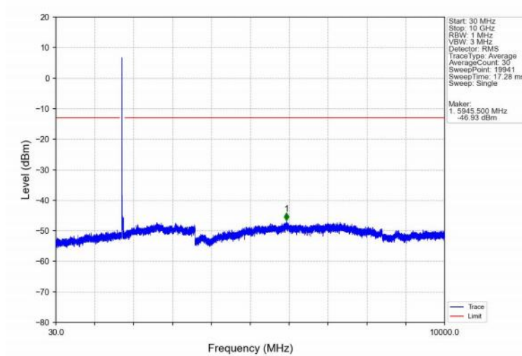
Band4_20MHz_16QAM_MCH_1732.5MHz_RB_1_0_NTNV
