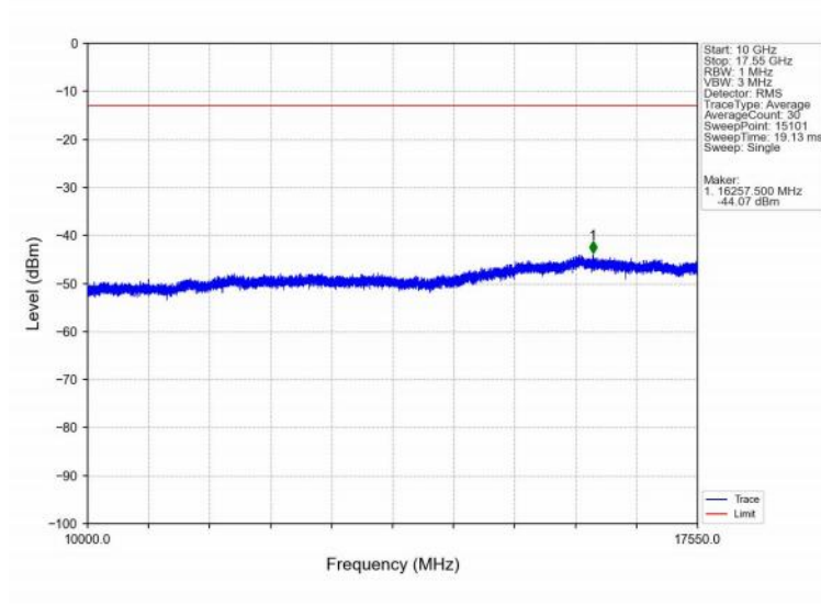
Band4_10MHz_16QAM_HCH_1750MHz_RB_1_0_NTNV
