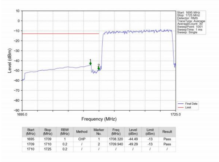
Band4_15MHz_16QAM_LCH_1717.5MHz_RB_75_0_NTNV
