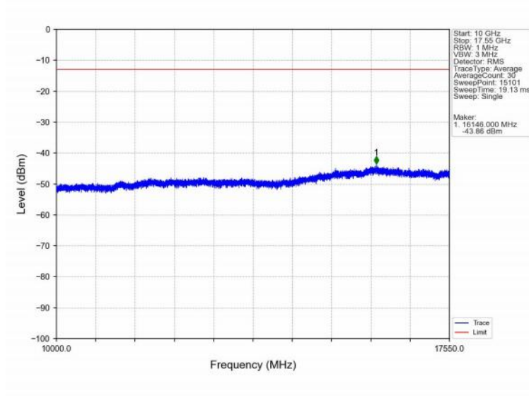
Band4_10MHz_QPSK_MCH_1732.5MHz_RB_1_0_NTNV
