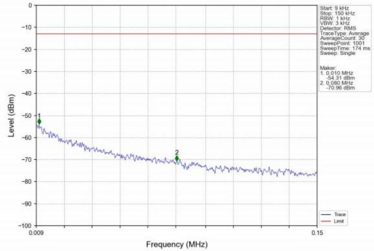
Band4_15MHz_QPSK_HCH_1747.5MHz_RB_1_0_NTNV
