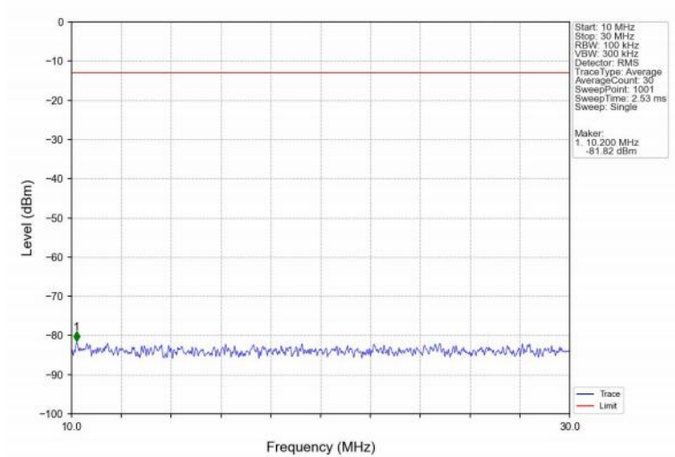
Band4_15MHz_QPSK_MCH_1732.5MHz_RB_1_0_NTNV
