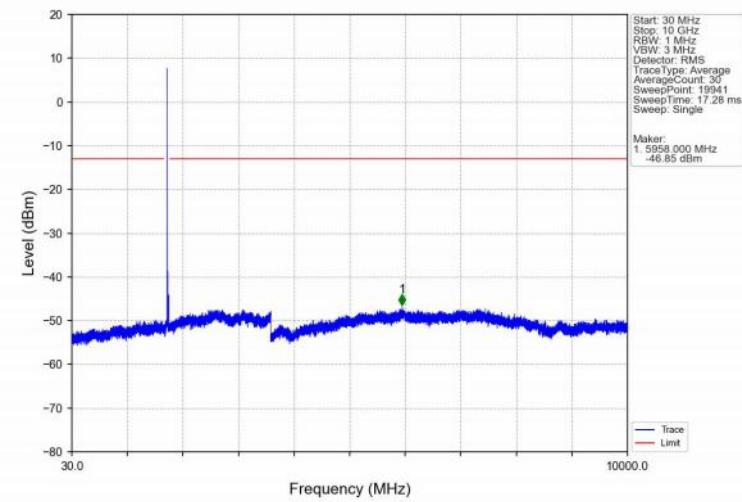
Band4_15MHz_QPSK_HCH_1747.5MHz_RB_1_0_NTNV
