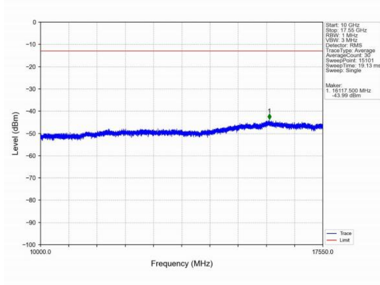
Band4_10MHz_QPSK_LCH_1715MHz_RB_1_0_NTNV
