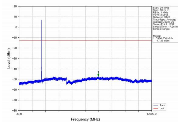
Band4_10MHz_16QAM_LCH_1715MHz_RB_1_0_NTNV
