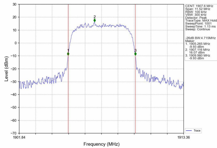
Band2_HSUPA_HCH_1907.6MHz_Subtest 1_NTNV
