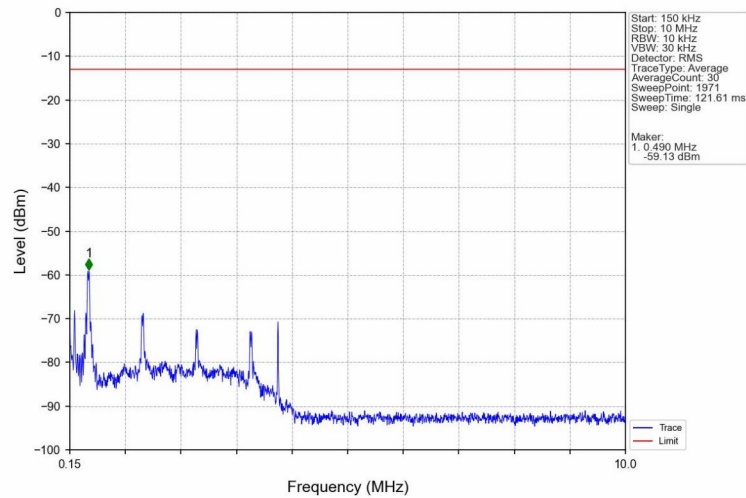
Band2_HSUPA_HCH_1907.6MHz_Subtest 1_NTNV
