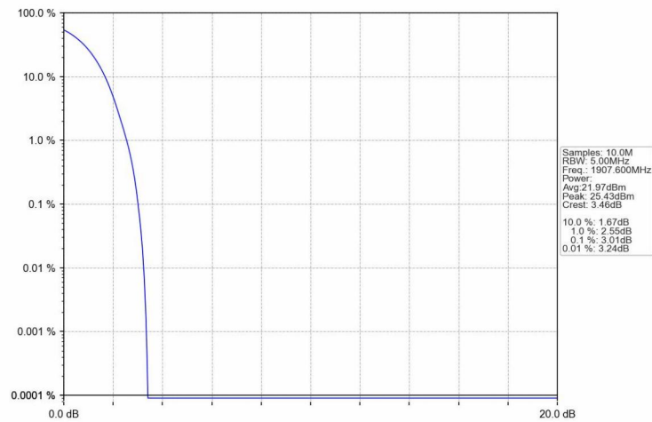
Band2_RMC_HCH_1907.6MHz_12.2kbps RMC_NTNV
