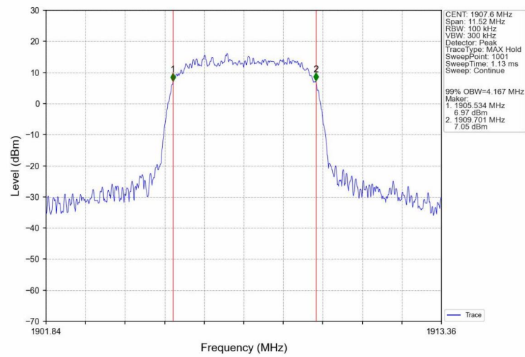
Band2_HSUPA_HCH_1907.6MHz_Subtest 1_NTNV
