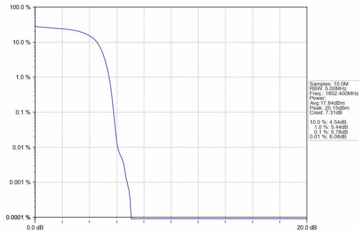
Band2_HSDPA_LCH_1852.4MHz_Subtest 1_NTNV
