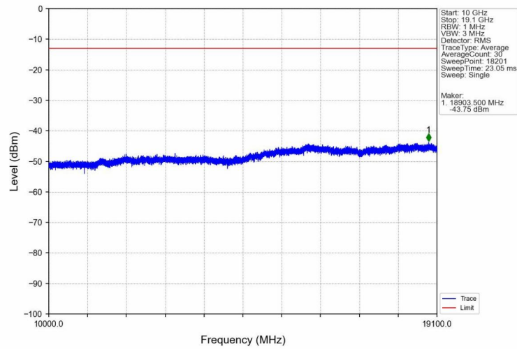
Band2_HSDPA_MCH_1880MHz_Subtest 1_NTNV
