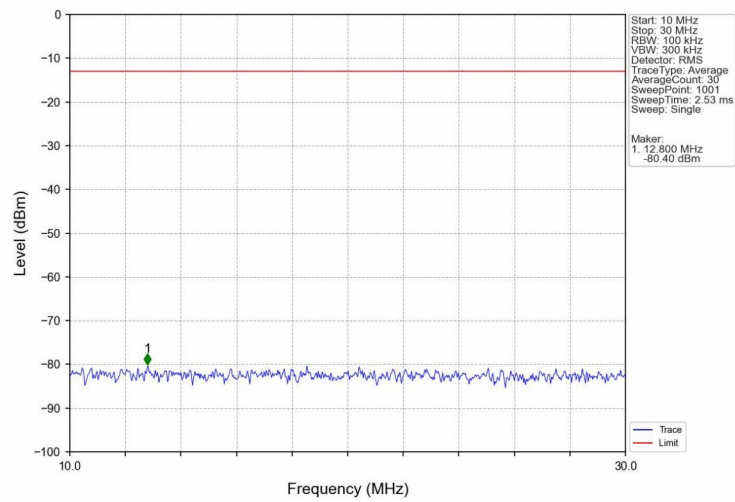
Band2_HSUPA_HCH_1907.6MHz_Subtest 1_NTNV
