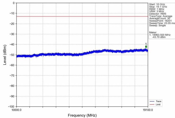
Band2_HSUPA_LCH_1852.4MHz_Subtest 1_NTNV
