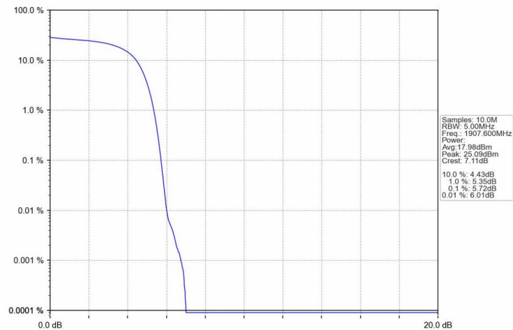
Band2_HSDPA_HCH_1907.6MHz_Subtest 1_NTNV
