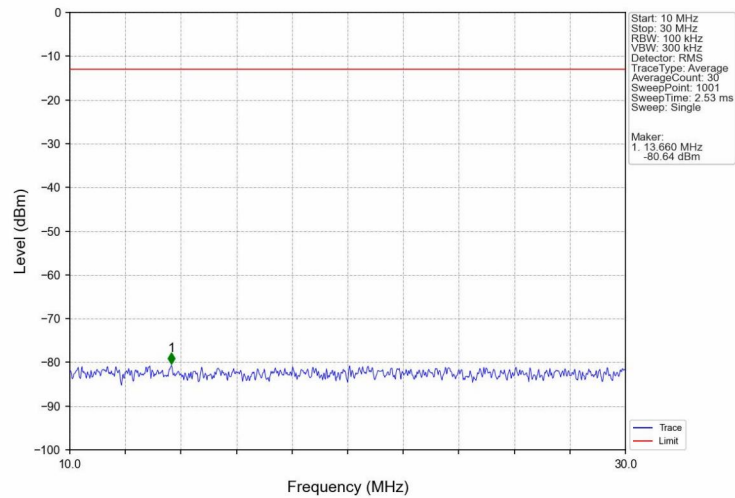
Band2_HSDPA_MCH_1880MHz_Subtest 1_NTNV
