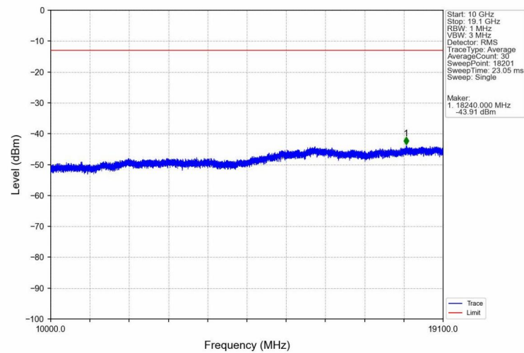
Band2_HSDPA_MCH_1880MHz_Subtest 1_NTNV
