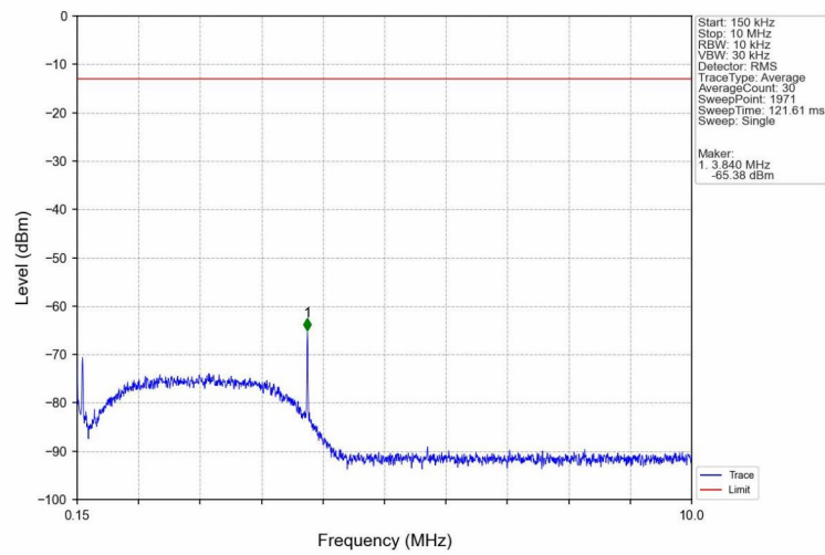
Band2_RMC_LCH_1852.4MHz_12.2kbps RMC_NTNV
