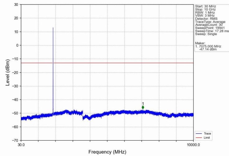
Band2_HSDPA_MCH_1880MHz_Subtest 1_NTNV
