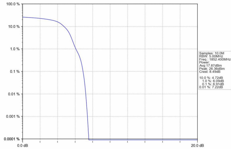
Band2_HSUPA_LCH_1852.4MHz_Subtest 1_NTNV
