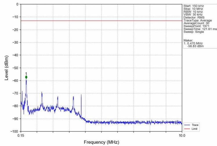
Band2_HSUPA_LCH_1852.4MHz_Subtest 1_NTNV
