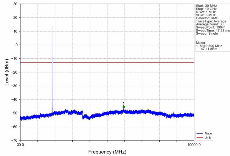
Band2_HSUPA_LCH_1852.4MHz_Subtest 1_NTNV
