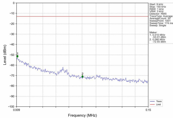
Band2_HSDPA_MCH_1880MHz_Subtest 1_NTNV
