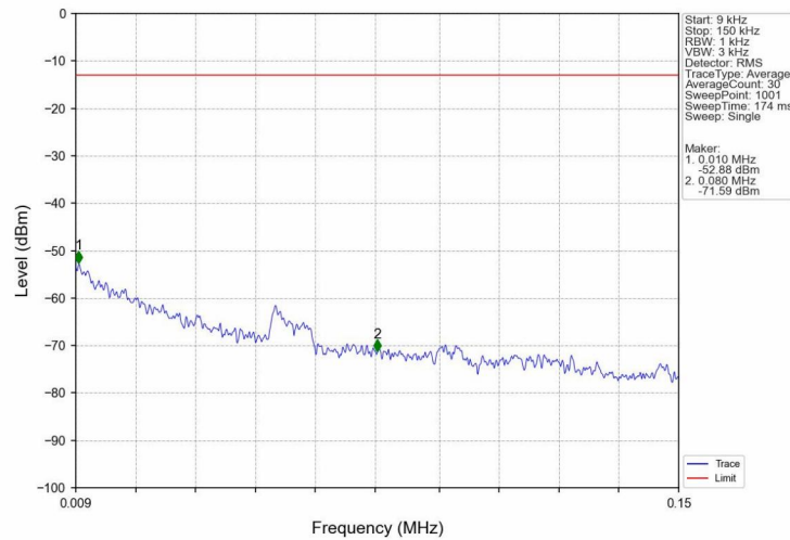
Band2_HSDPA_HCH_1907.6MHz_Subtest 1_NTNV
