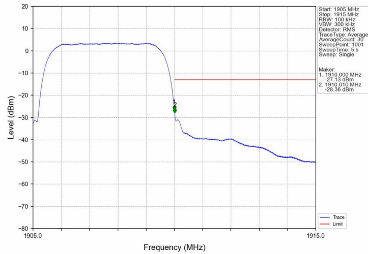
Band2_HSDPA_HCH_1907.6MHz_Subtest 1_NTNV
