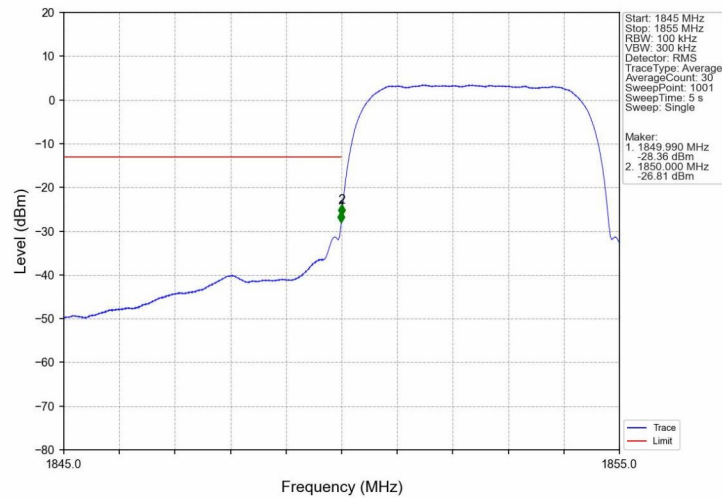
Band2_HSDPA_LCH_1852.4MHz_Subtest 1_NTNV
