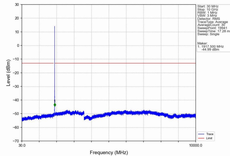
Band2_HSUPA_HCH_1907.6MHz_Subtest 1_NTNV
