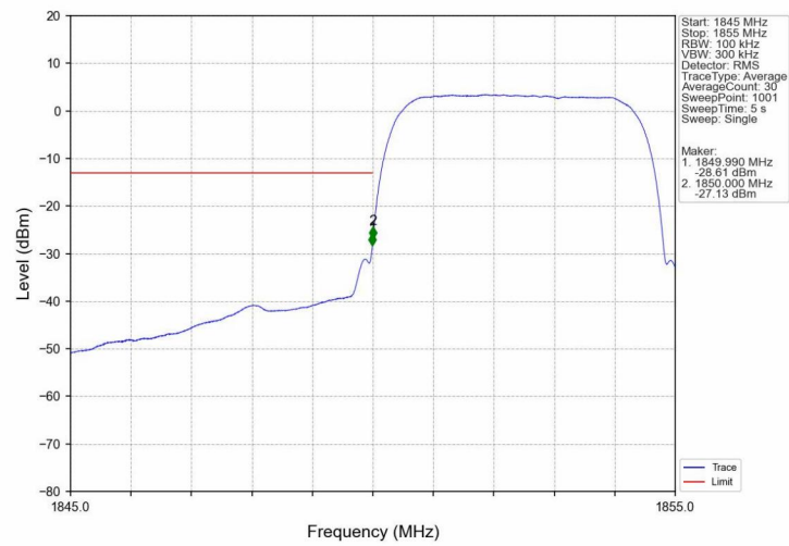
Band2_HSUPA_LCH_1852.4MHz_Subtest 1_NTNV
