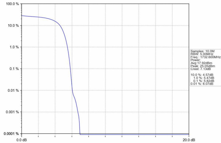
Band4_HSDPA_MCH_1732.6MHz_Subtest 1_NTNV
