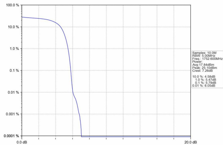
Band4_HSDPA_HCH_1752.6MHz_Subtest 1_NTNV
