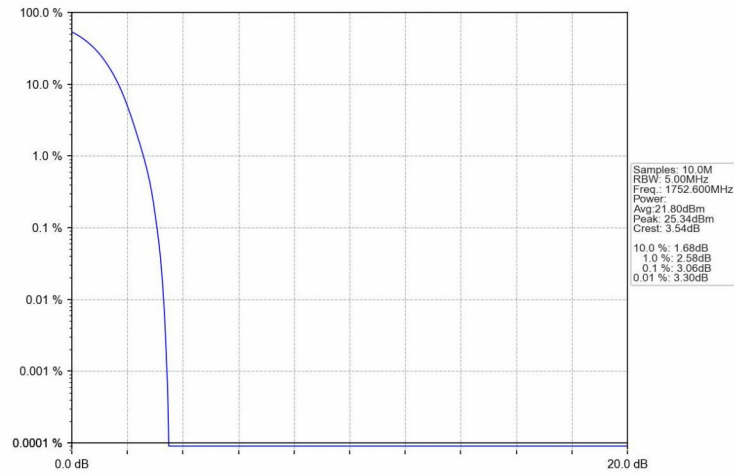
Band4_RMC_HCH_1752.6MHz_12.2kbps RMC_NTNV
