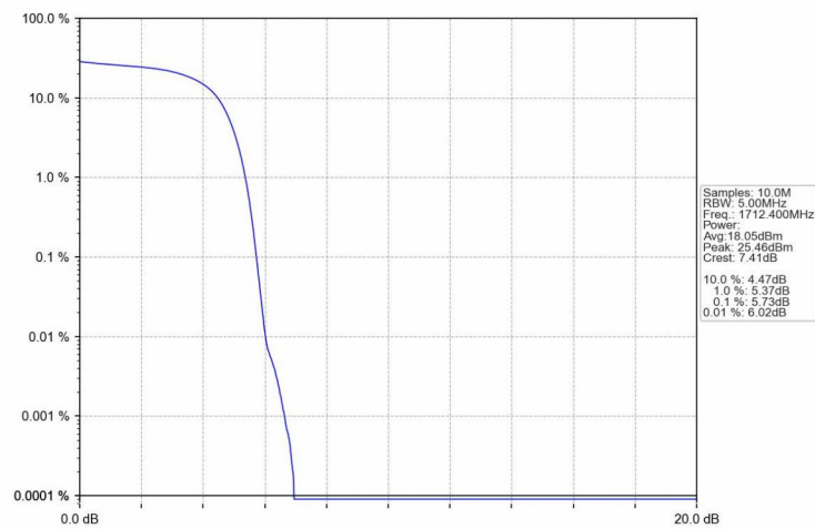
Band4_HSDPA_LCH_1712.4MHz_Subtest 1_NTNV
