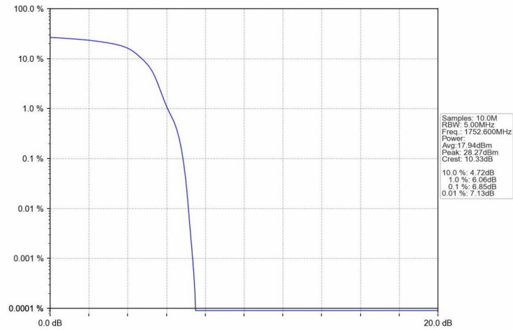
Band4_HSUPA_HCH_1752.6MHz_Subtest 1_NTNV
