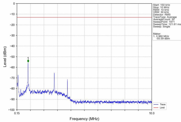
Band5_HSDPA_MCH_836.6MHz_Subtest 1_NTNV
