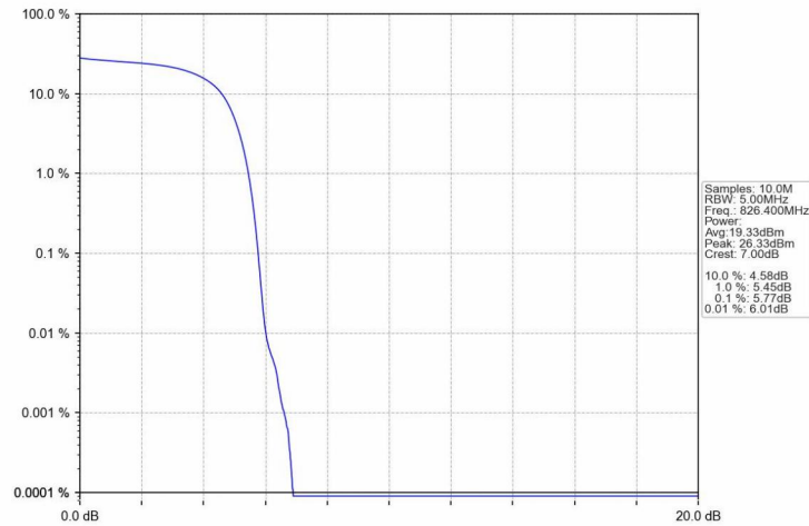
Band5_HSDPA_LCH_826.4MHz_Subtest 1_NTNV
