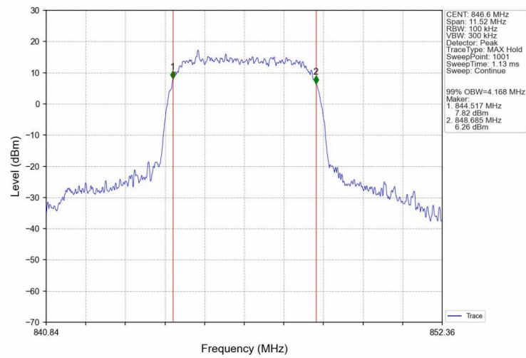
Band5_HSUPA_HCH_846.6MHz_Subtest 1_NTNV
