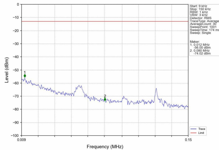
Band5_HSUPA_LCH_826.4MHz_Subtest 1_NTNV
