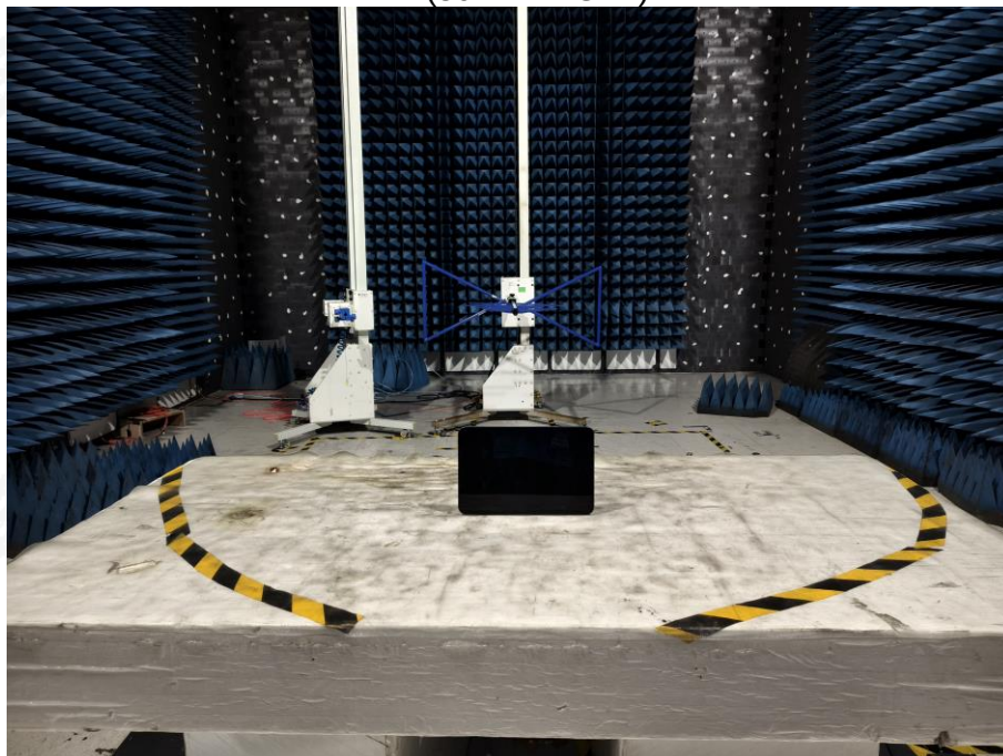
RE (30 MHz-1GHz)
