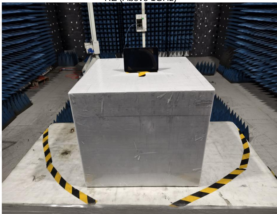
RE (Above 1GHz)
