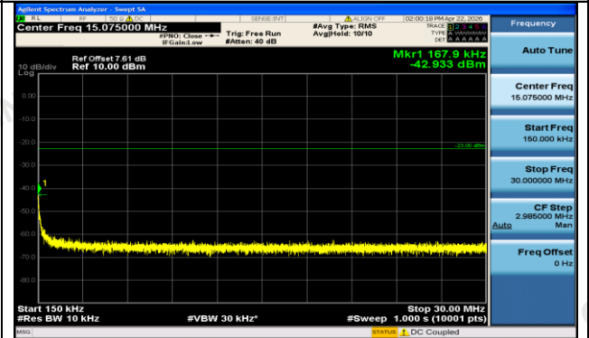
EGPRS850-190-8-0.15~30MHz-PASS
