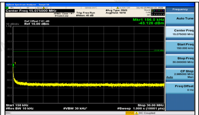
GPRS850-190-5-0.15~30MHz-PASS
