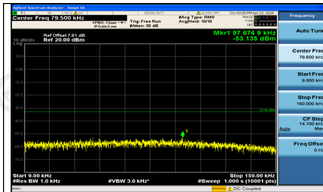
GPRS850-190-5-0.009~0.15MHz-PASS
