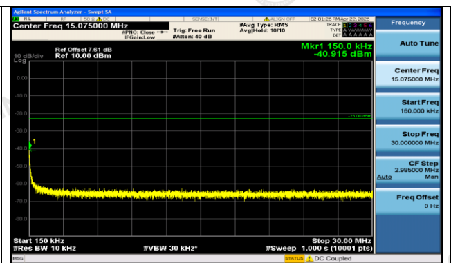
EGPRS850-251-8-0.15~30MHz-PASS
