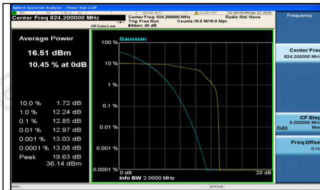
EGPRS850-128-8-PASS
