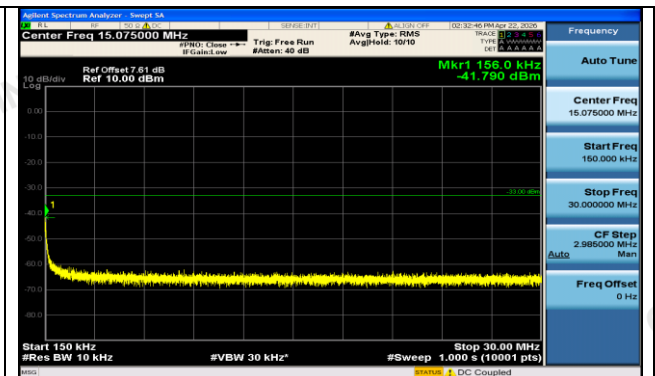
EGPRS1900-512-2-0.15~30MHz-PASS
