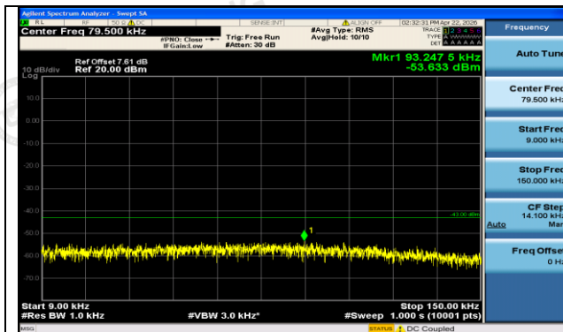
EGPRS1900-512-2-0.009~0.15MHz-PASS
