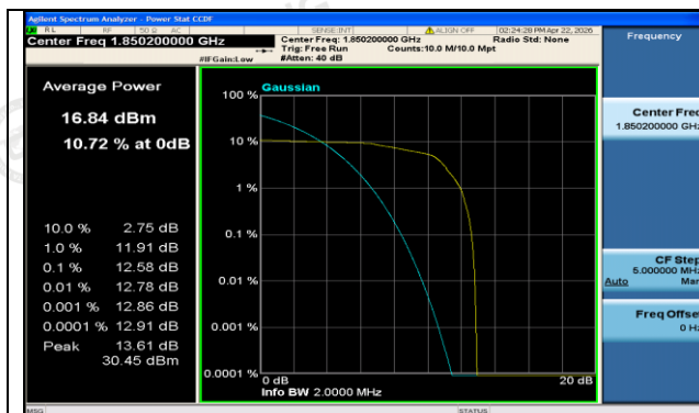
EGPRS1900-512-2-PASS
