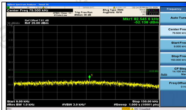
GPRS1900-512-0-0.009~0.15MHz-PASS
