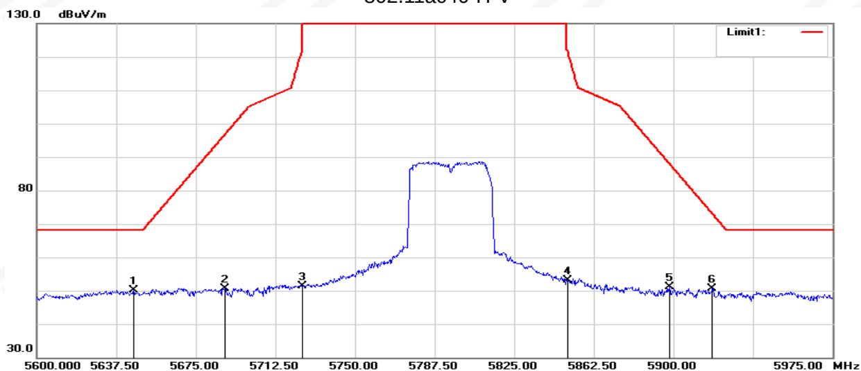
802.11ac40-H-V
