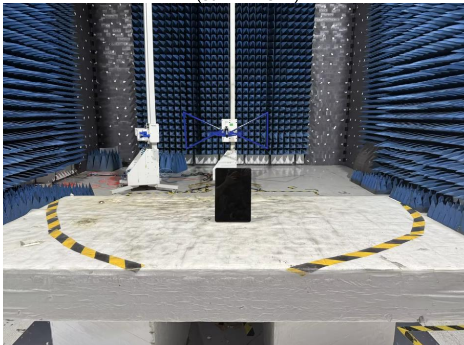
RE (30 MHz-1GHz)
