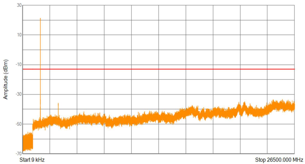
Band66 16QAM BW=3MHz Channel=132322 RB Size=15 Position=#0
