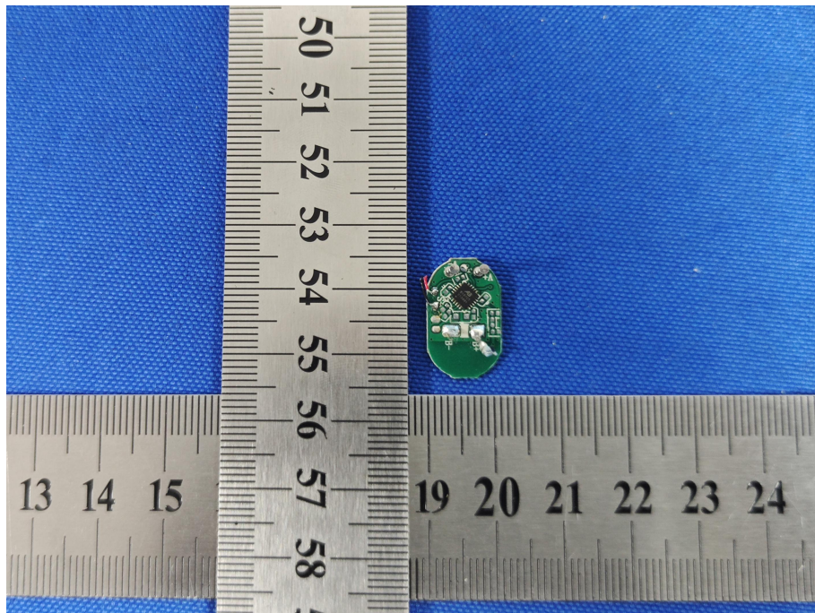
INTERNAL PHOTO OF SAMPLE PCB (RIGHT)
