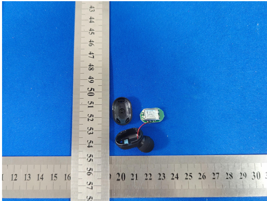
INTERNAL PHOTO OF SAMPLE (RIGHT)
