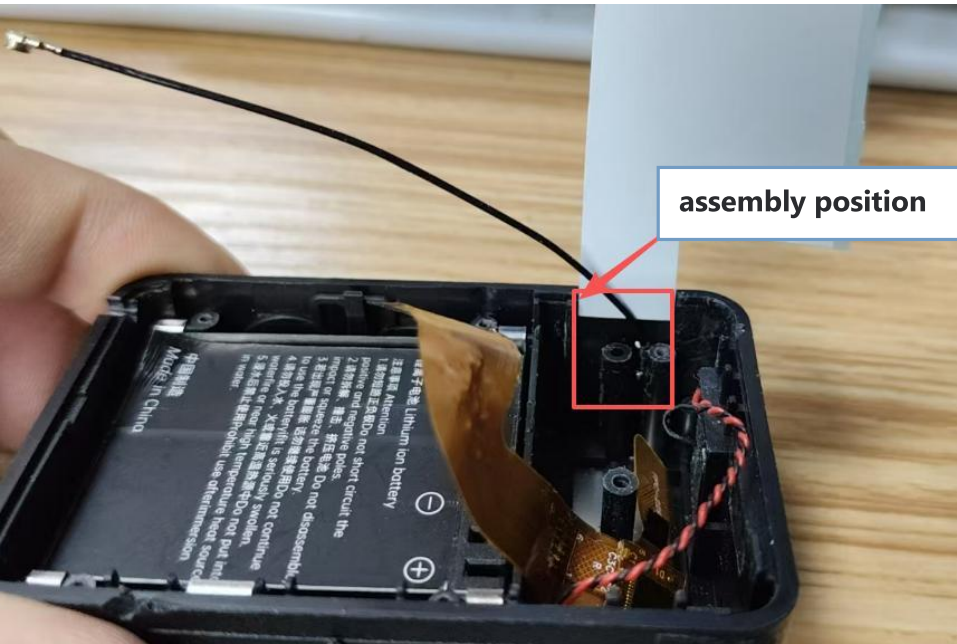
assembly position
