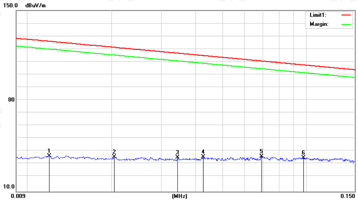
RSE-9KHz-150KHz-Coaxial
