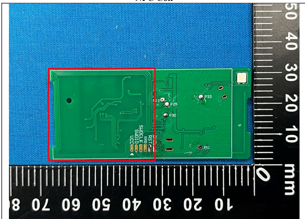
NFC Coil
