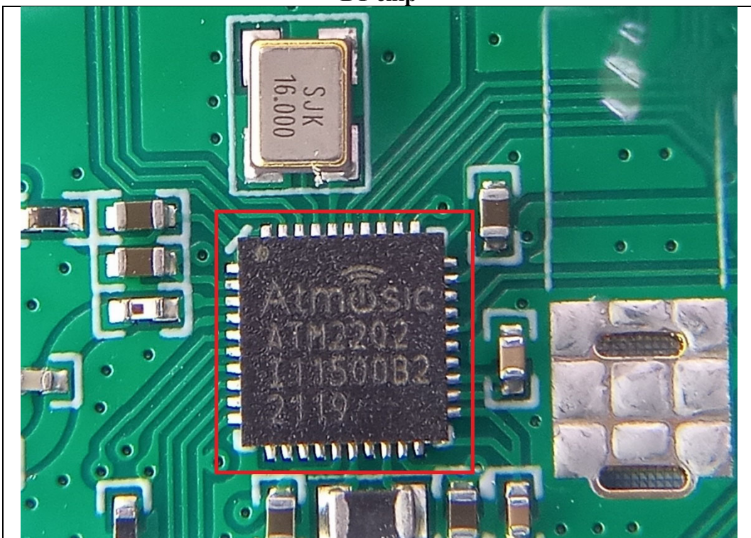
BT chip
