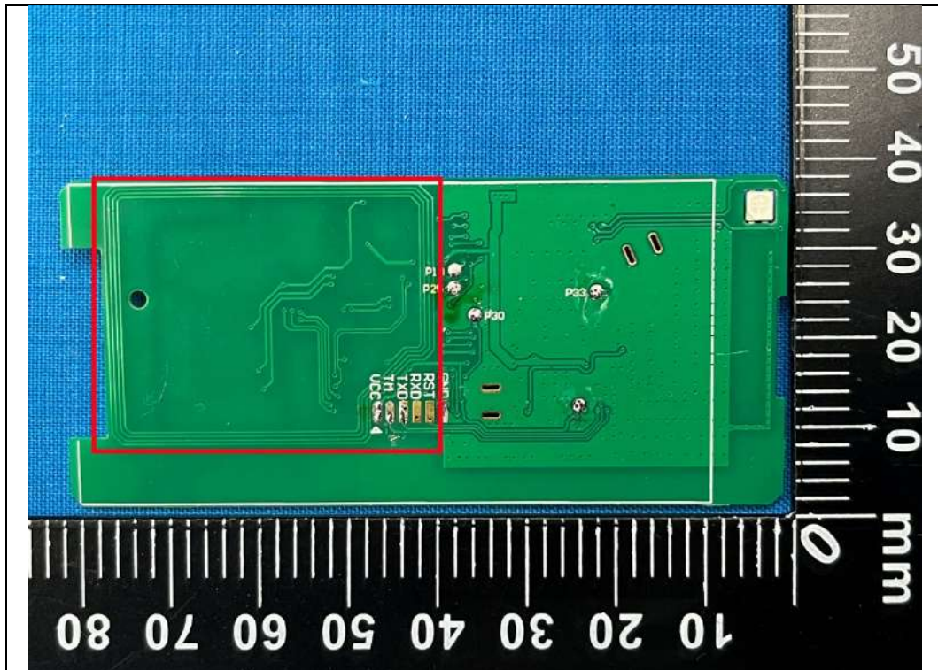
NFC Coil
