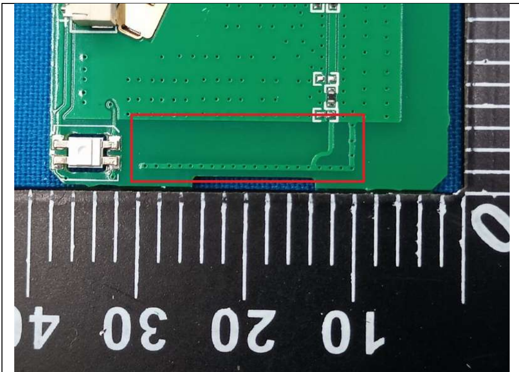
BT Antenna
