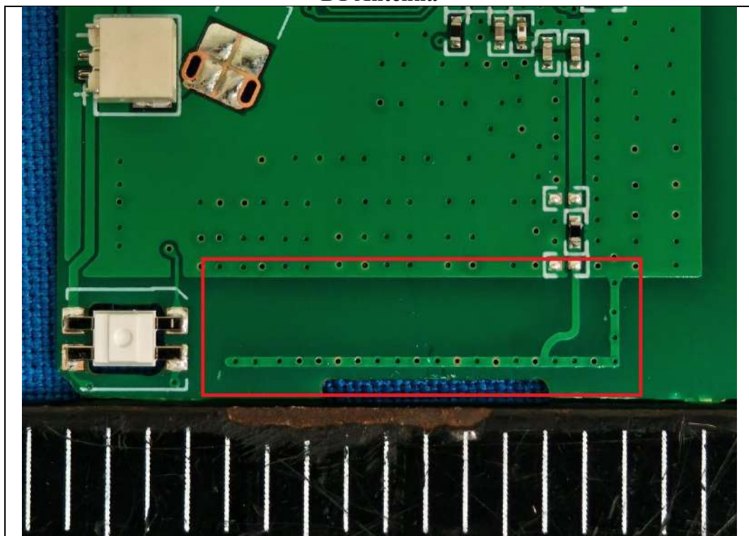
BT Antenna
