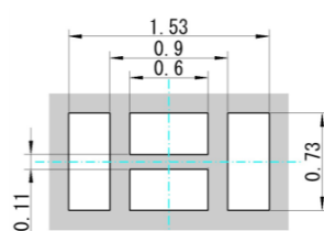
&lt; Solder resist pattern &gt;
