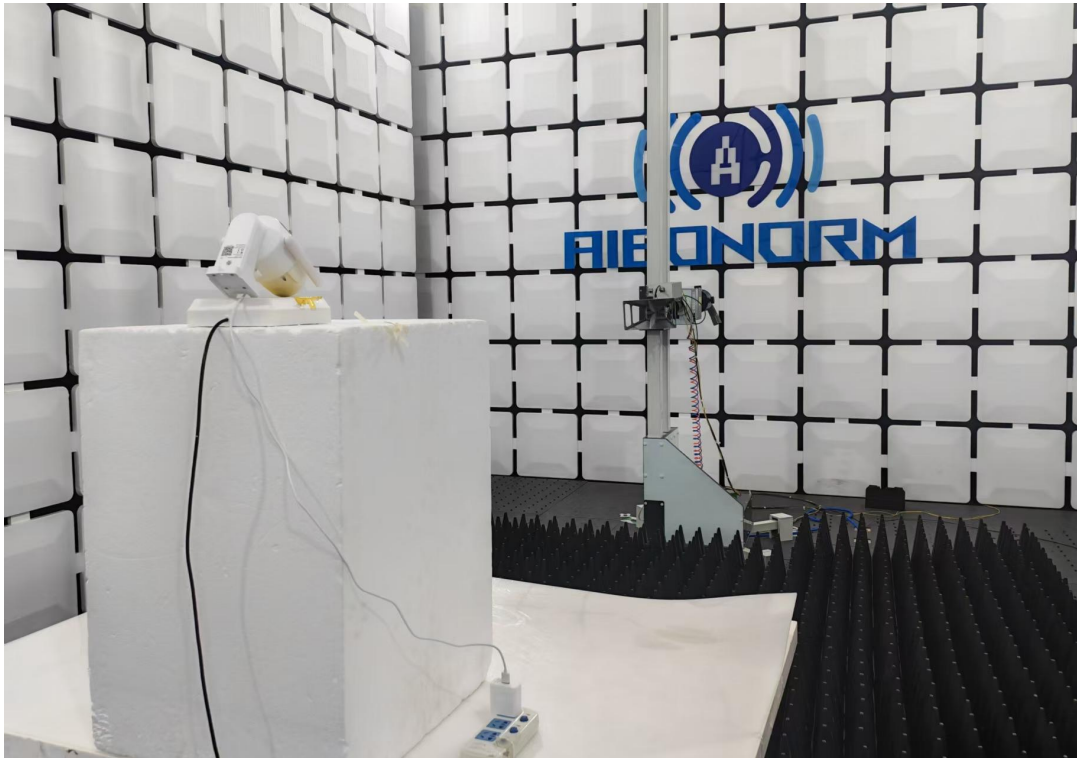
Radiated Spurious Emission Test View 1
