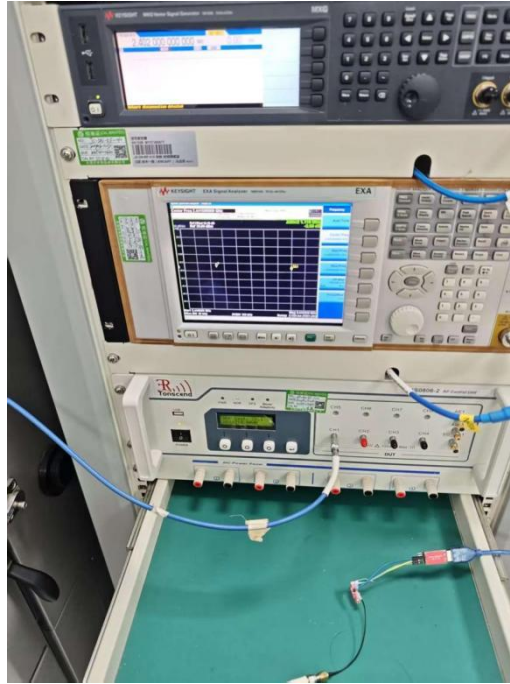
Conducted Emission Test View
