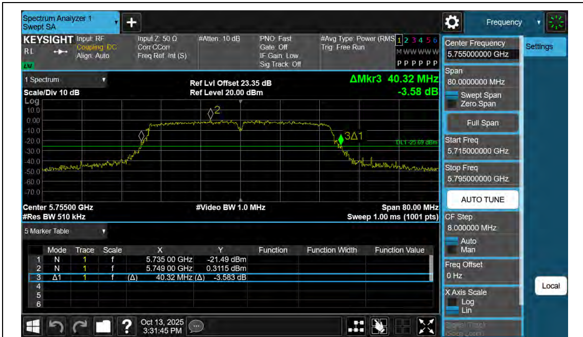
11AC40MIMO-Ant2-5755
