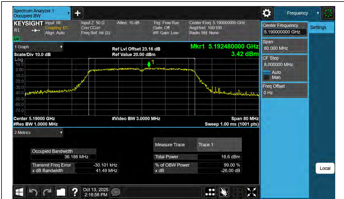
11N40MIMO-Ant2-5190
