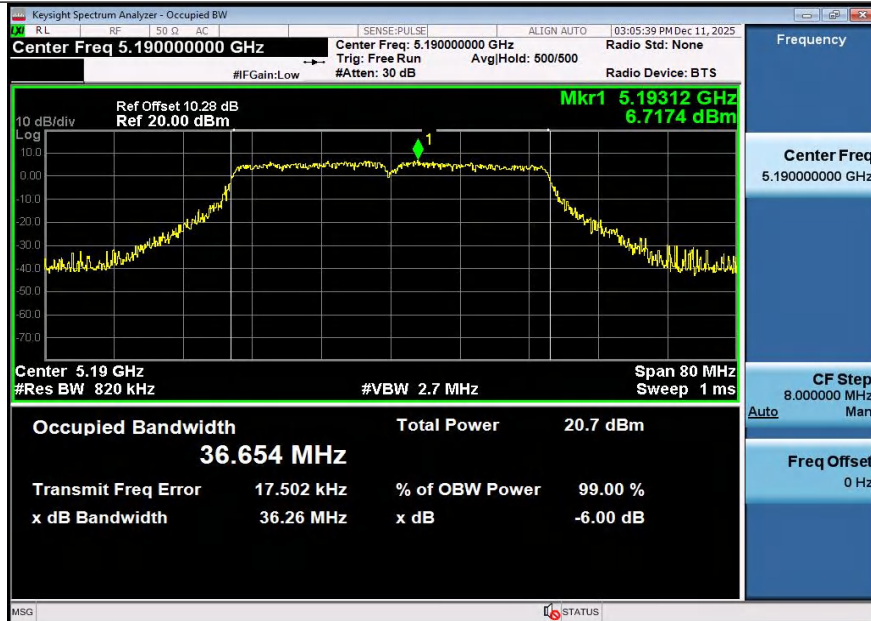
11N40SISO-Ant1-5190
