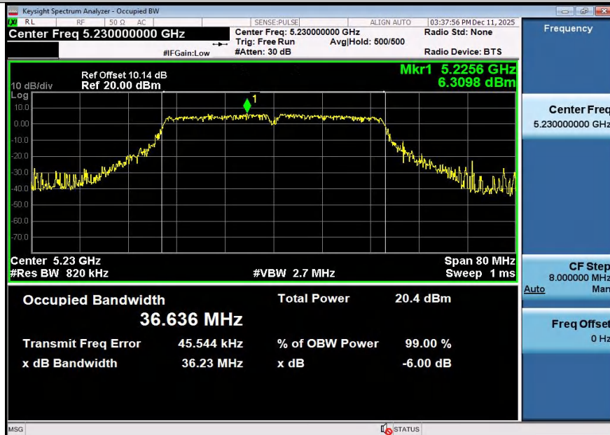
11AC40SISO-Ant1-5230
