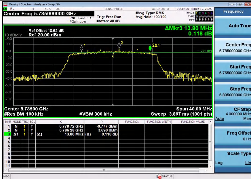
11N20SISO-Ant2-5785-PASS
