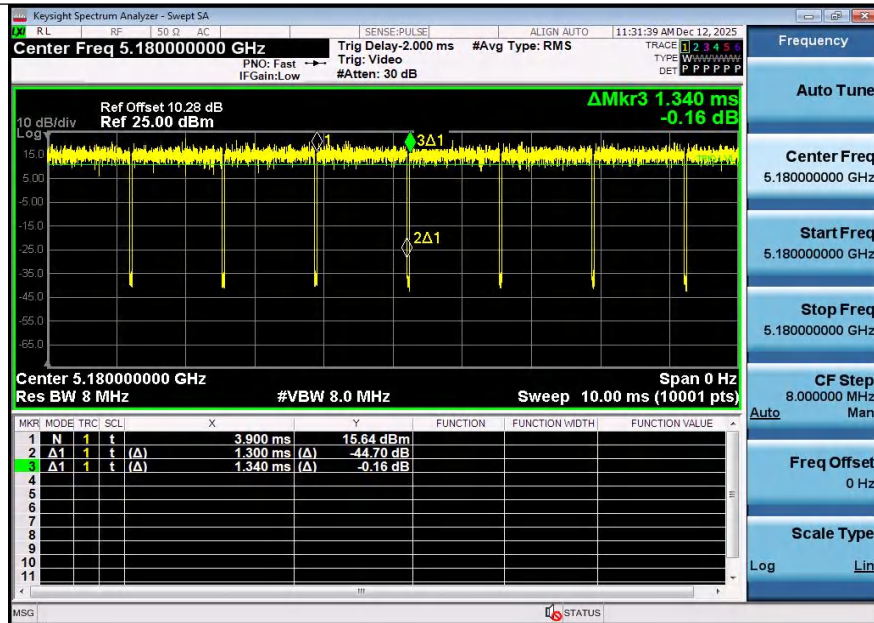
NTNV-11N20SISO-Ant1-5180
