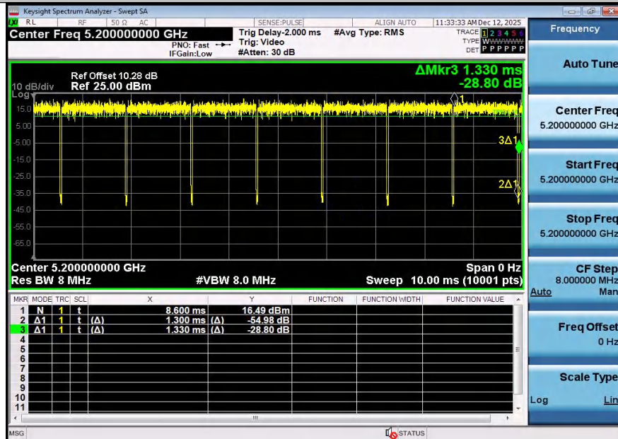
NTNV-11N20SISO-Ant1-5200
