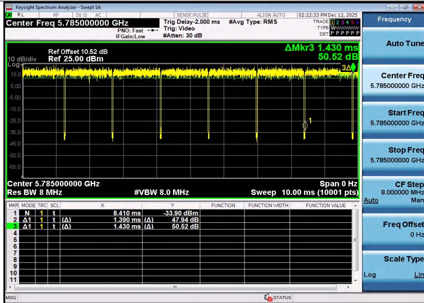
NTNV-11A-Ant2-5785
