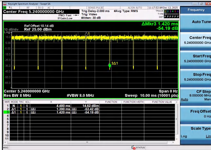
NTNV-11A-Ant1-5240
