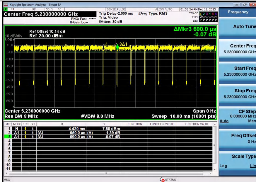
NTNV-11AC40SISO-Ant1-5230
