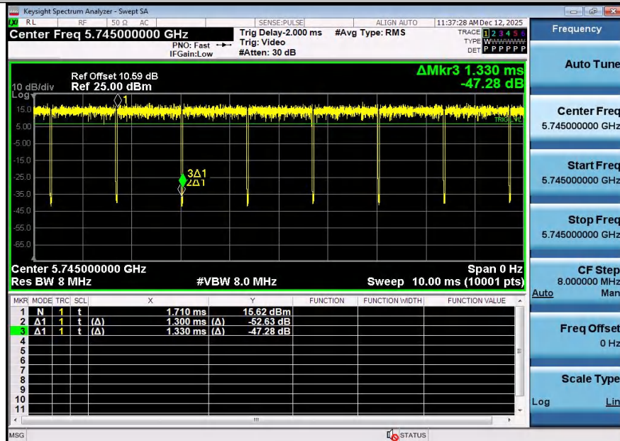
NTNV-11N20SISO-Ant1-5745
