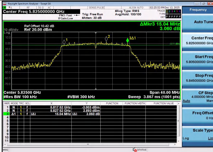
11A-Ant2-5825-PASS
