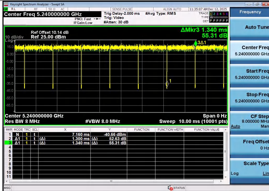
NTNV-11N20SISO-Ant1-5240
