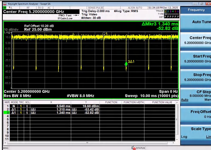
NTNV-11AC20SISO-Ant1-5200
