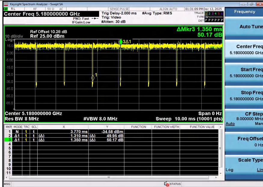
NTNV-11AC20SISO-Ant1-5180
