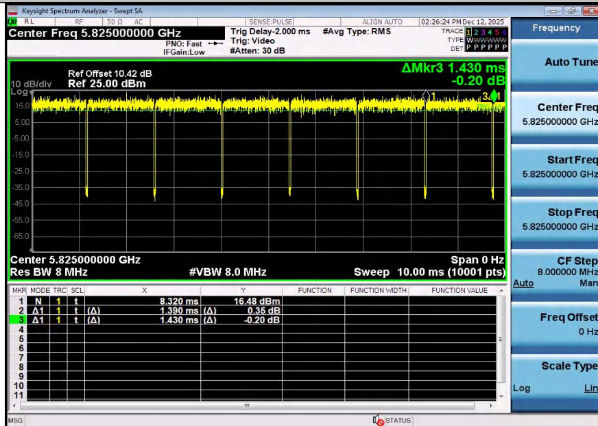
NTNV-11A-Ant2-5825
