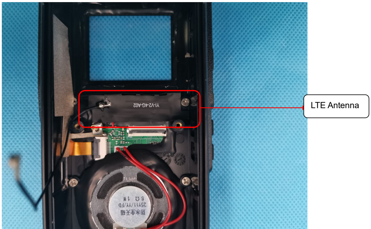
Internal View-1 of EUT
