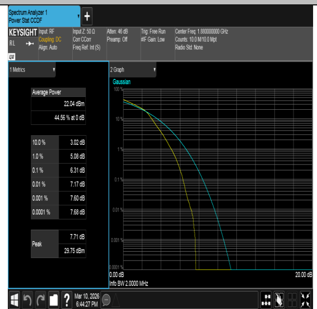
Band2-1.4MHz-16QAM-18900-6RB#0-PASS
