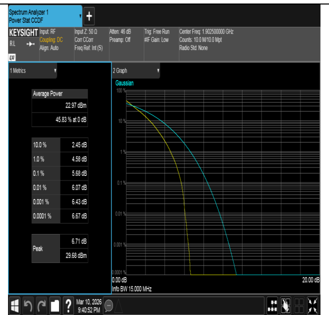
Band2-15MHz-QPSK-19125-75RB#0-PASS
