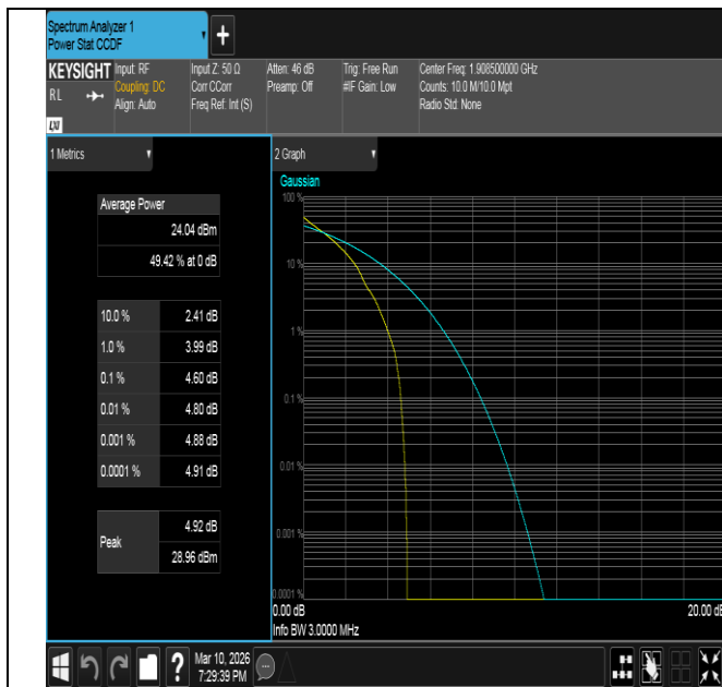
Band2-3MHz-QPSK-19185-1RB#0-PASS
