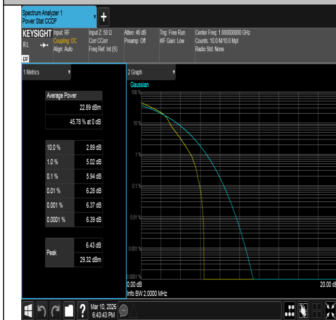
Band2-1.4MHz-16QAM-18900-1RB#0-PASS
