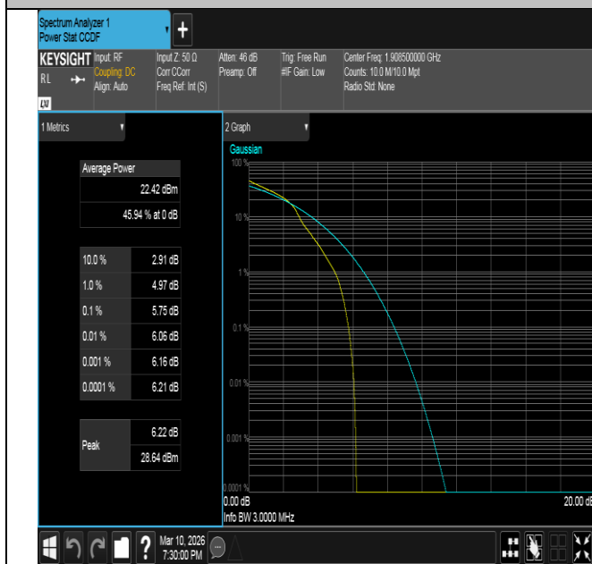
Band2-3MHz-16QAM-19185-1RB#0-PASS
