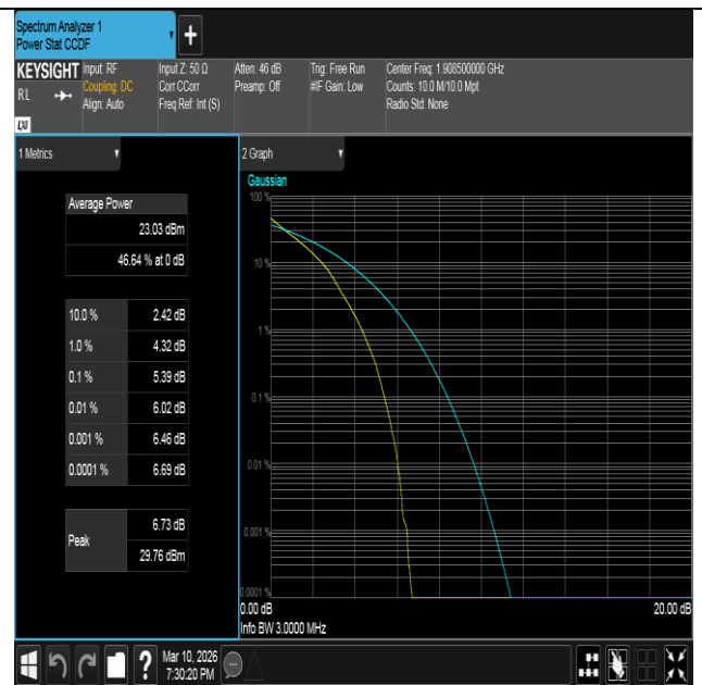
Band2-3MHz-QPSK-19185-15RB#0-PASS
