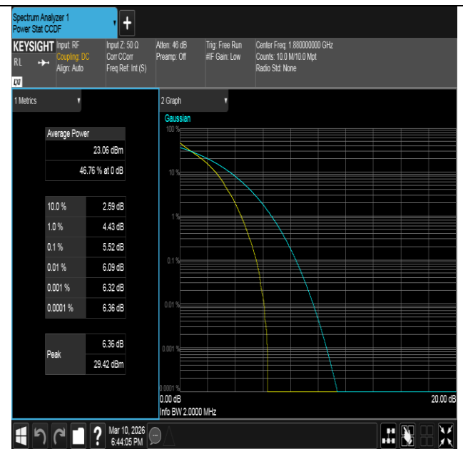
Band2-1.4MHz-QPSK-18900-6RB#0-PASS
