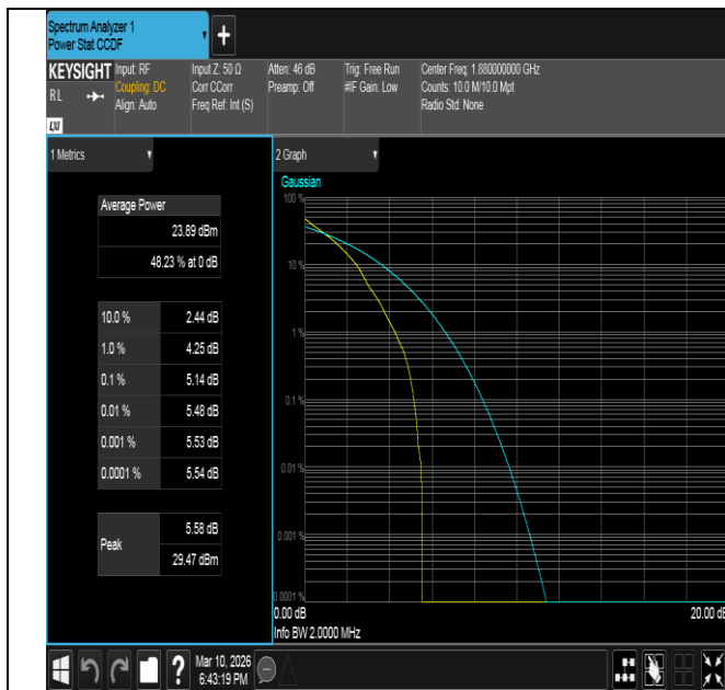
Band2-1.4MHz-QPSK-18900-1RB#0-PASS
