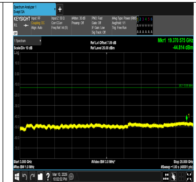
Band2-20MHz-16QAM-19100-1RB#0-3000~20000-PASS
