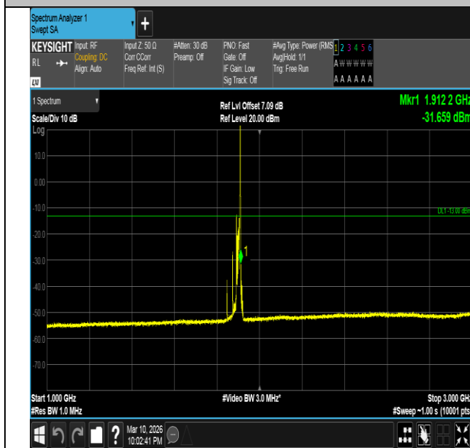
Band2-20MHz-QPSK-19100-1RB#99-1000~3000-PASS
