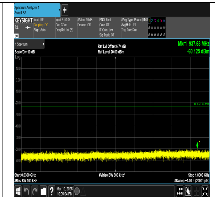
Band2-20MHz-16QAM-19100-100RB#0-30~1000-PASS
