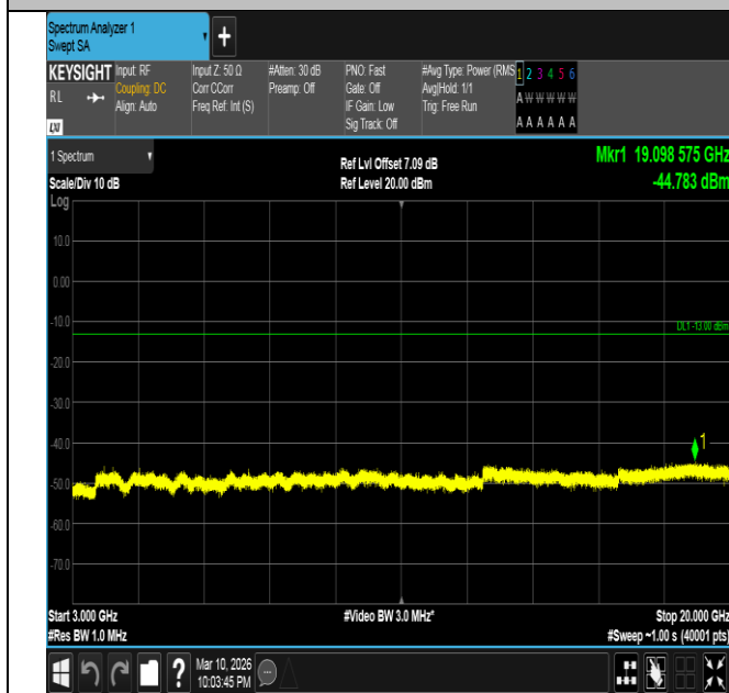
Band2-20MHz-16QAM-19100-1RB#99-3000~20000-PASS
