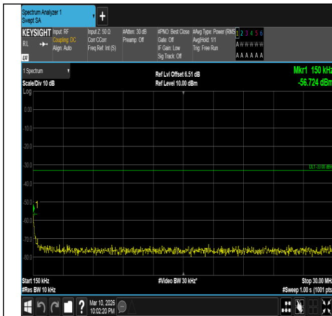
Band2-20MHz-QPSK-19100-1RB#99-0.15~30-PASS
