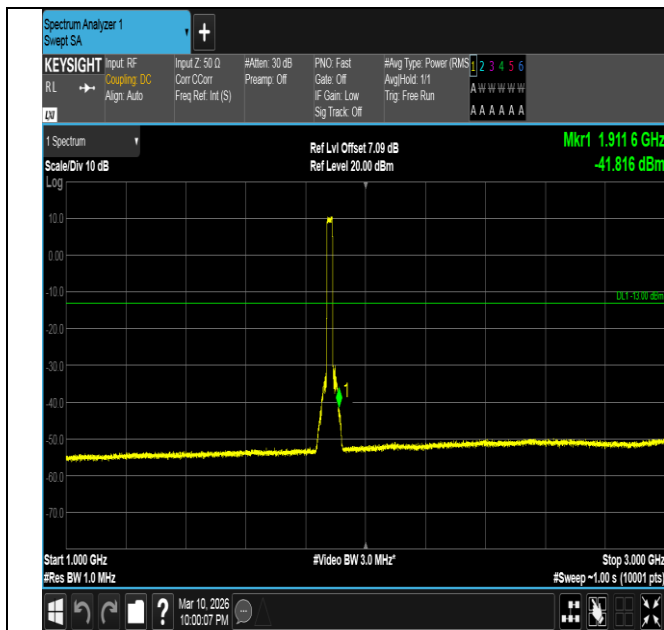
Band2-20MHz-16QAM-18900-100RB#0-1000~3000-PASS
