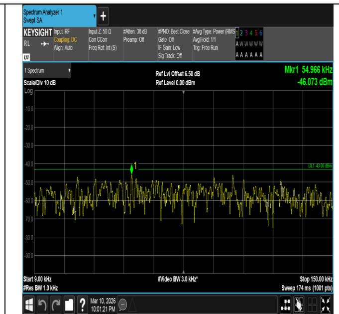
Band2-20MHz-16QAM-19100-1RB#0-0.009~0.15-PASS
