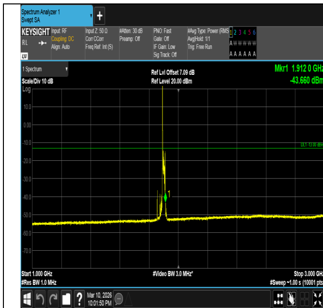
Band2-20MHz-16QAM-19100-1RB#0-1000~3000-PASS
