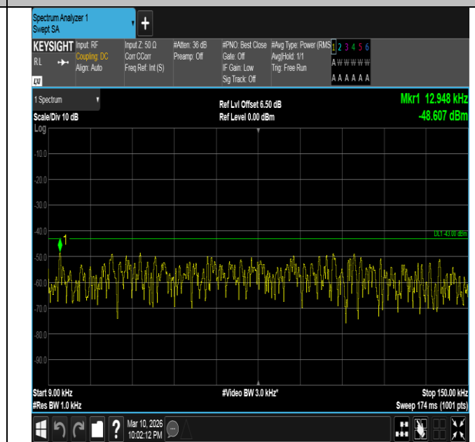
Band2-20MHz-QPSK-19100-1RB#99-0.009~0.15-PASS
