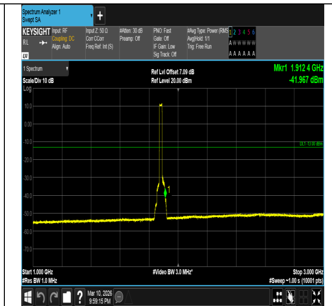
Band2-20MHz-QPSK-18900-100RB#0-1000~3000-PASS
