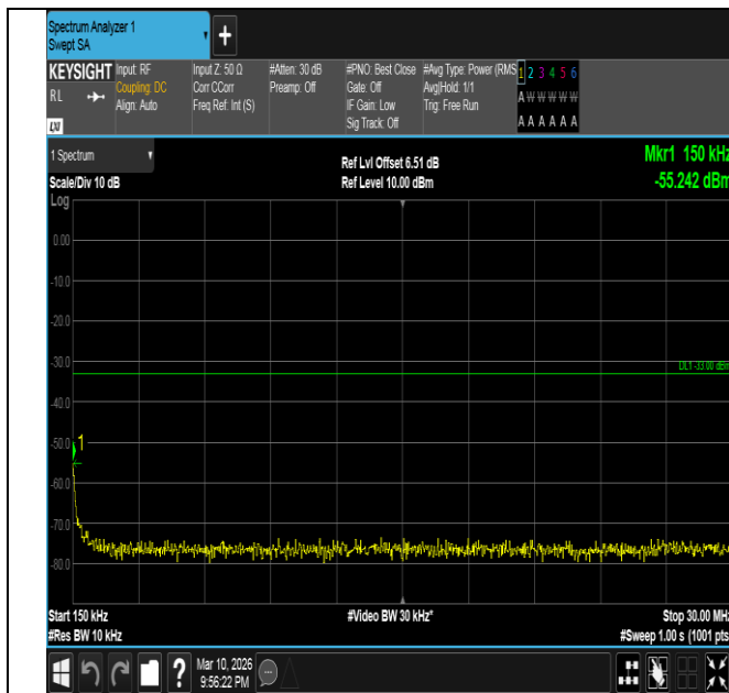
Band2-20MHz-16QAM-18900-1RB#0-0.15~30-PASS
