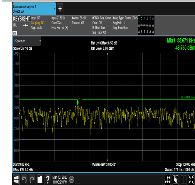
Band2-20MHz-QPSK-19100-1RB#0-0.009~0.15-PASS
