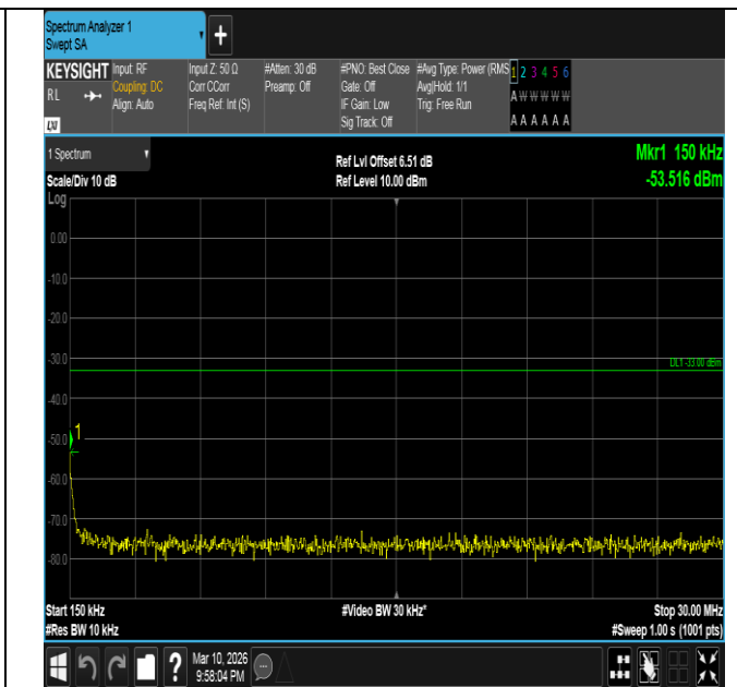
Band2-20MHz-16QAM-18900-1RB#99-0.15~30-PASS
