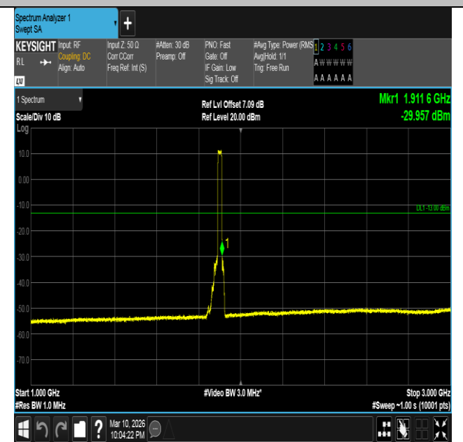
Band2-20MHz-QPSK-19100-100RB#0-1000~3000-PASS
