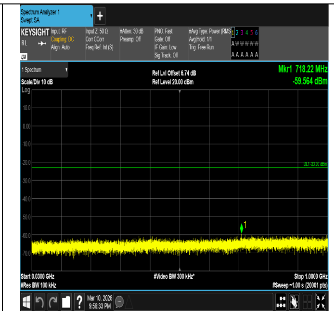
Band2-20MHz-16QAM-18900-1RB#0-30~1000-PASS
