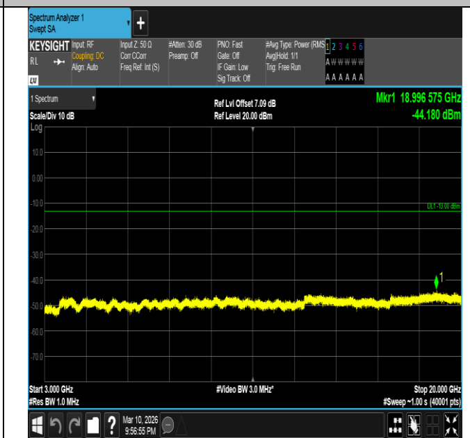
Band2-20MHz-16QAM-18900-1RB#0-3000~20000-PASS
