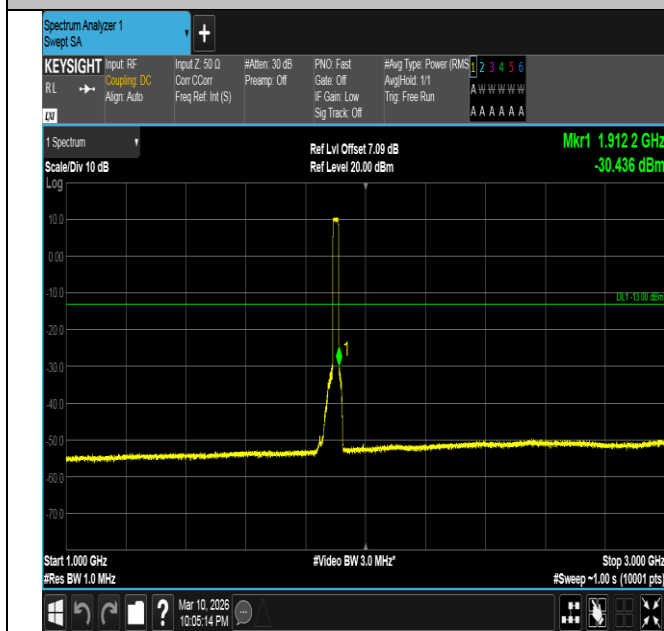
Band2-20MHz-16QAM-19100-100RB#0-1000~3000-PASS
