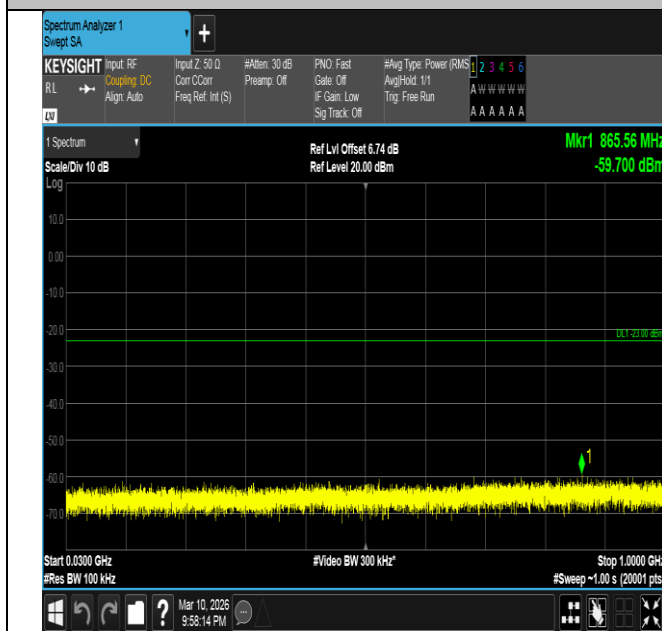
Band2-20MHz-16QAM-18900-1RB#99-30~1000-PASS
