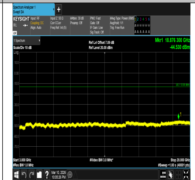
Band2-20MHz-16QAM-19100-100RB#0-3000~20000-PASS
