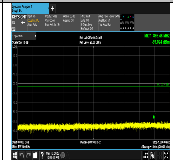
Band2-20MHz-16QAM-19100-1RB#0-30~1000-PASS
