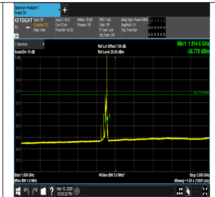
Band2-20MHz-16QAM-19100-1RB#99-1000~3000-PASS
