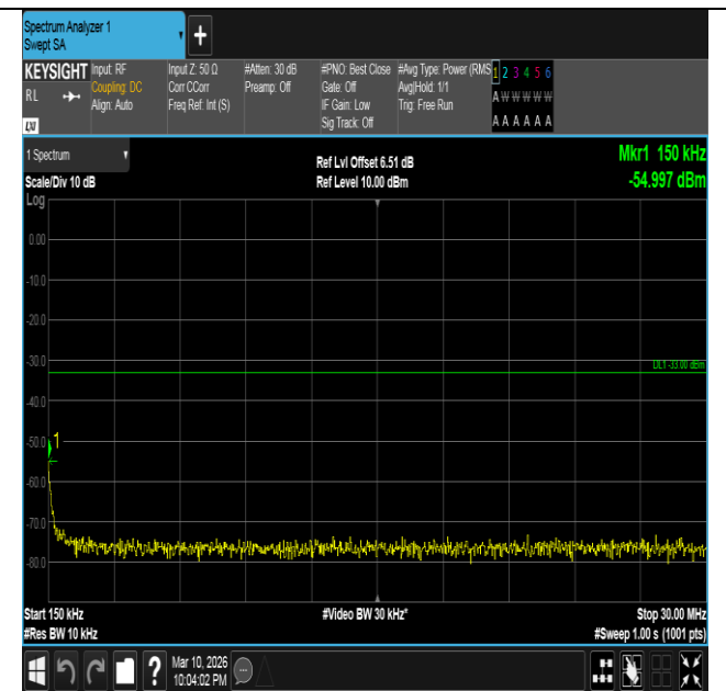
Band2-20MHz-QPSK-19100-100RB#0-0.15~30-PASS
