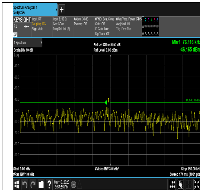
Band2-20MHz-16QAM-18900-1RB#99-0.009~0.15-PASS
