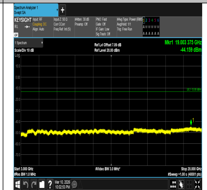
Band2-20MHz-QPSK-19100-1RB#99-3000~20000-PASS
