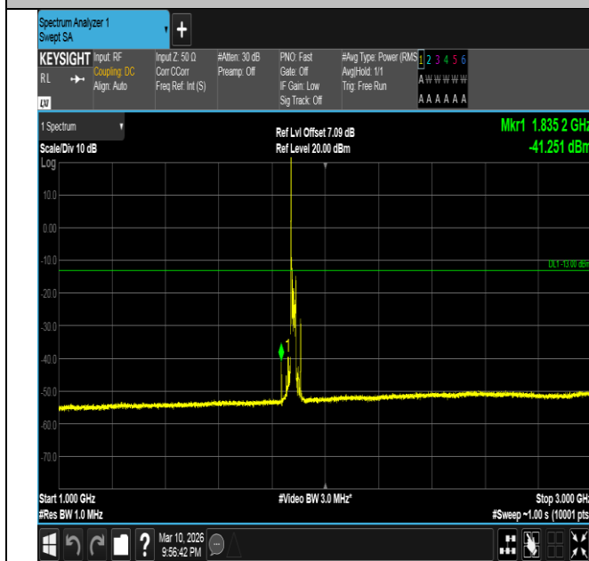
Band2-20MHz-16QAM-18900-1RB#0-1000~3000-PASS
