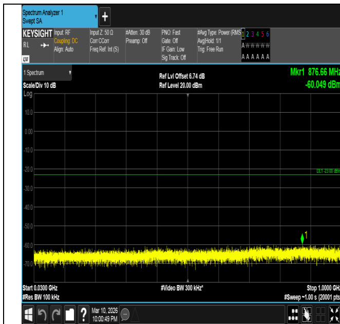
Band2-20MHz-QPSK-19100-1RB#0-30~1000-PASS
