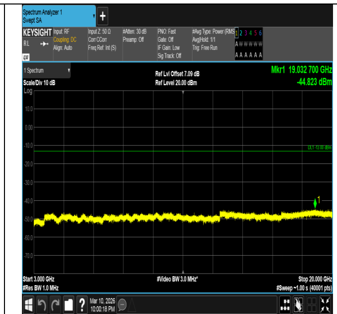
Band2-20MHz-16QAM-18900-100RB#0-3000~20000-PASS
