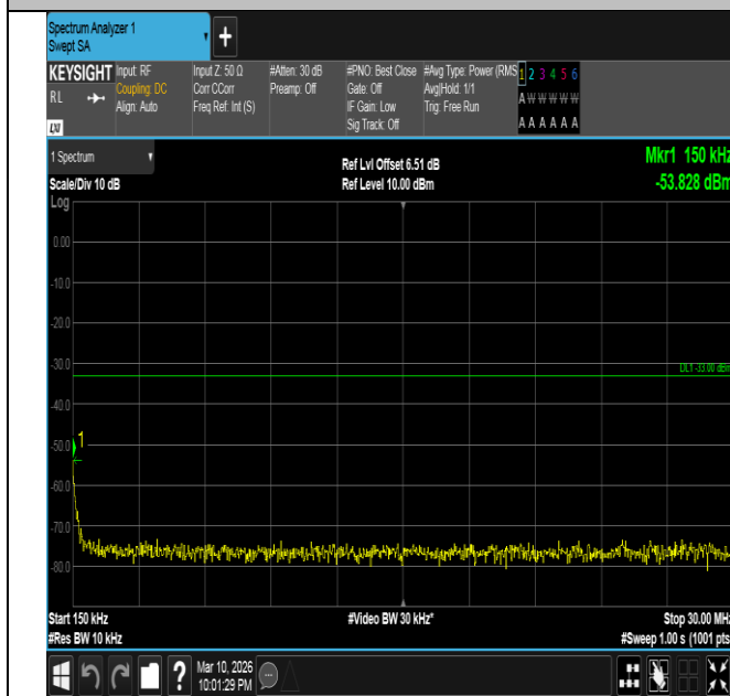
Band2-20MHz-16QAM-19100-1RB#0-0.15~30-PASS
