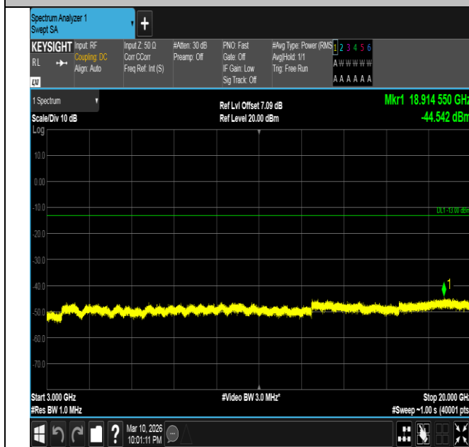
Band2-20MHz-QPSK-19100-1RB#0-3000~20000-PASS
