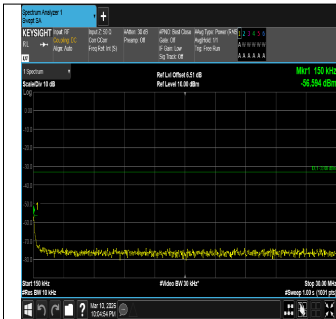
Band2-20MHz-16QAM-19100-100RB#0-0.15~30-PASS
