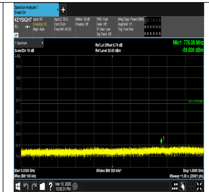
Band2-20MHz-QPSK-19100-1RB#99-30~1000-PASS
