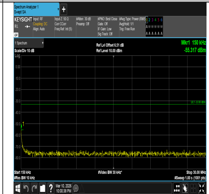
Band2-20MHz-QPSK-19100-1RB#0-0.15~30-PASS
