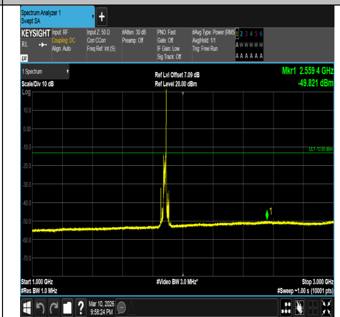
Band2-20MHz-16QAM-18900-1RB#99-1000~3000-PASS
