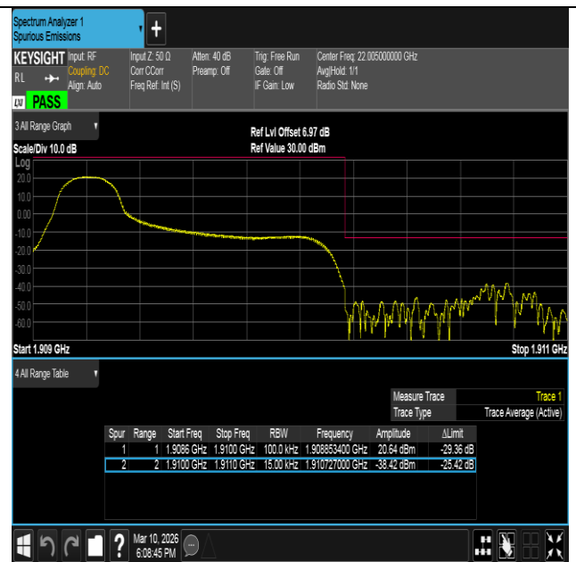
Band2-1.4MHz-16QAM-19193-1RB#0-PASS
