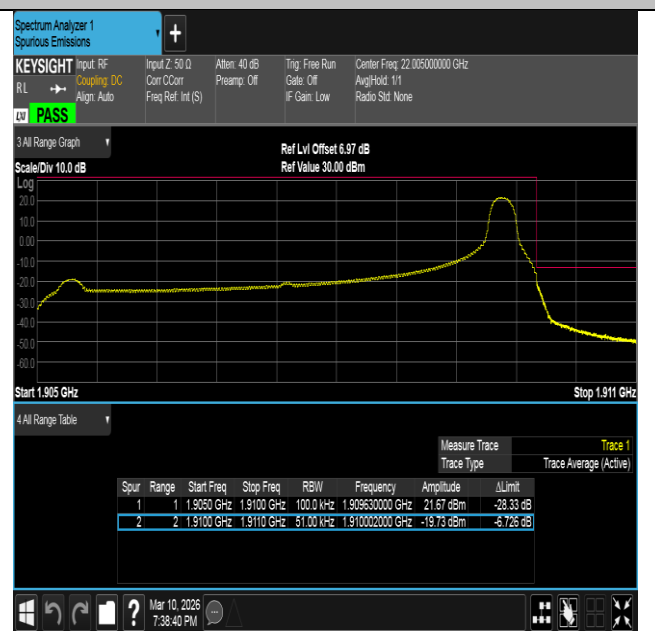
Band2-5MHz-QPSK-19175-1RB#24-PASS
