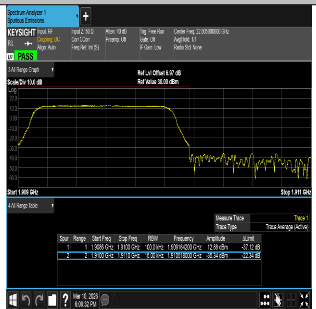
Band2-1.4MHz-16QAM-19193-6RB#0-PASS
