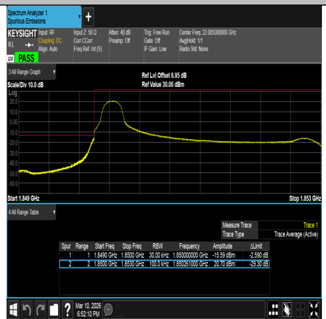
Band2-3MHz-16QAM-18615-1RB#0-PASS
