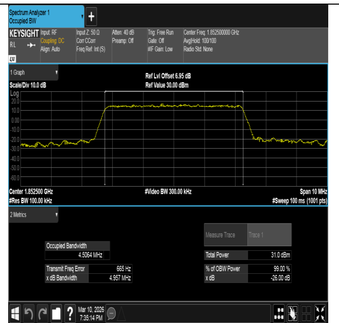
Band2-5MHz-16QAM-18625-25RB#0-PASS
