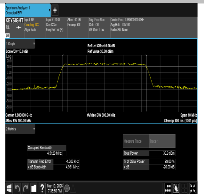
Band2-5MHz-16QAM-18900-25RB#0-PASS
