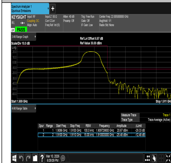
Band2-1.4MHz-16QAM-19193-1RB#5-PASS
