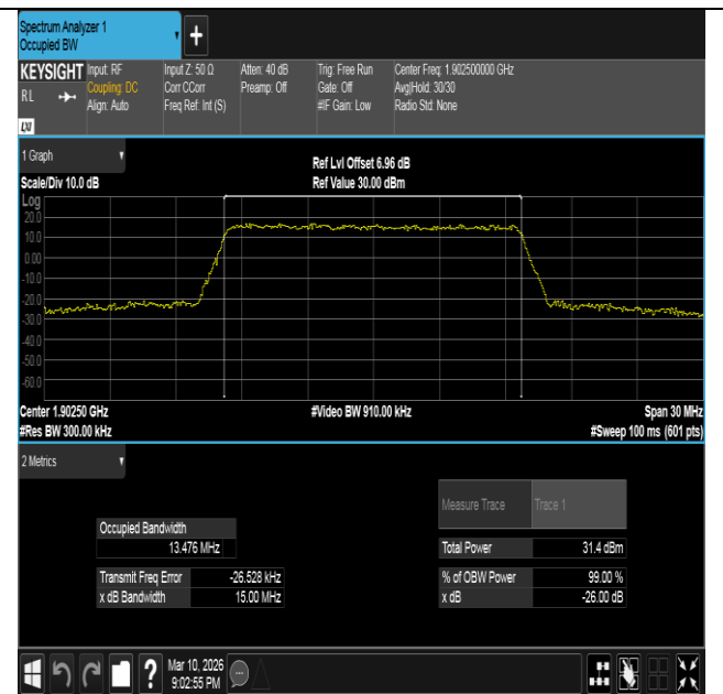
Band2-15MHz-16QAM-19125-75RB#0-PASS
