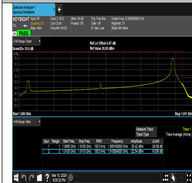
Band2-15MHz-16QAM-19125-1RB#74-PASS
