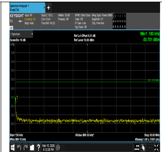
Band2-1.4MHz-16QAM-18607-1RB#5-0.15~30-PASS
