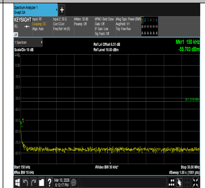
Band2-1.4MHz-QPSK-18607-6RB#0-0.15~30-PASS
