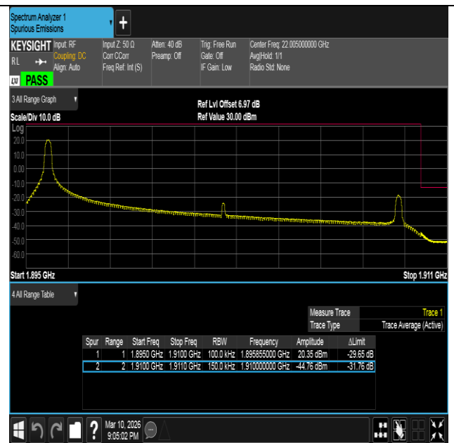
Band2-15MHz-16QAM-19125-1RB#0-PASS
