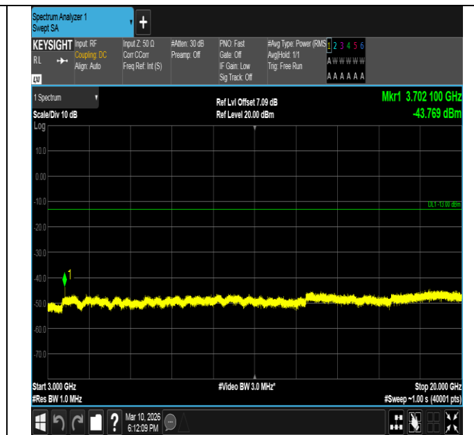
Band2-1.4MHz-QPSK-18607-1RB#5-3000~20000-PASS
