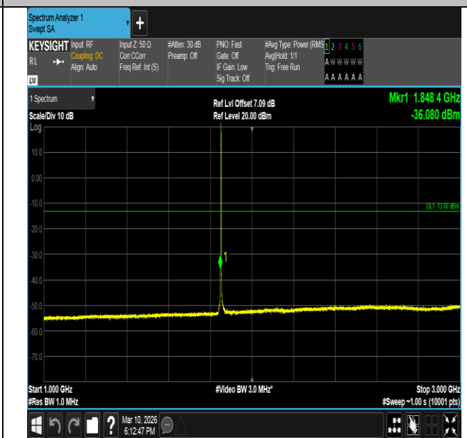
Band2-1.4MHz-16QAM-18607-1RB#5-1000~3000-PASS
