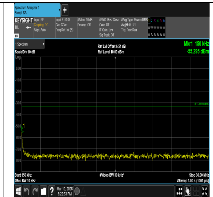
Band2-1.4MHz-16QAM-19193-1RB#5-0.15~30-PASS
