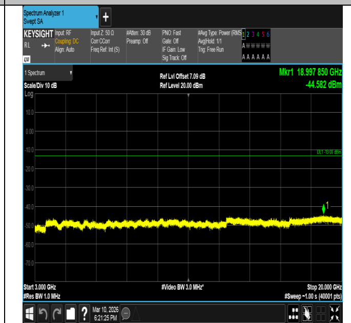
Band2-1.4MHz-16QAM-19193-1RB#0-3000~20000-PASS
