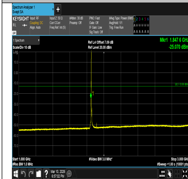
Band2-3MHz-QPSK-18615-1RB#14-1000~3000-PASS
