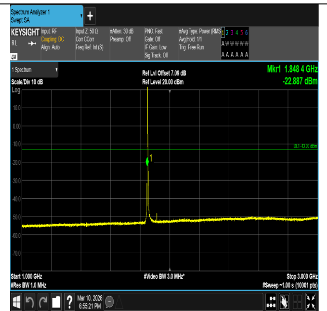
Band2-3MHz-QPSK-18615-1RB#0-1000~3000-PASS
