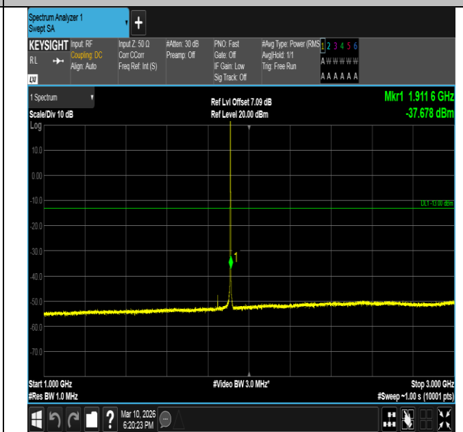
Band2-1.4MHz-QPSK-19193-1RB#0-1000~3000-PASS
