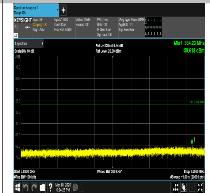
Band2-1.4MHz-16QAM-19193-6RB#0-30~1000-PASS
