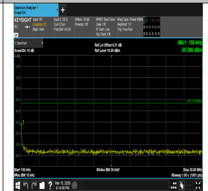
Band2-1.4MHz-QPSK-18900-1RB#0-0.15~30-PASS
