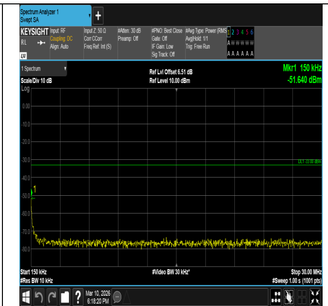
Band2-1.4MHz-QPSK-18900-6RB#0-0.15~30-PASS
