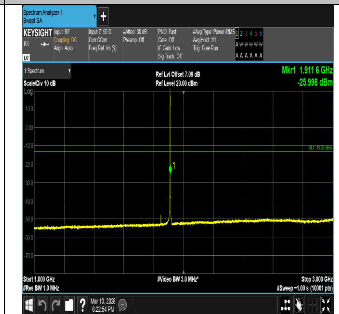
Band2-1.4MHz-16QAM-19193-1RB#5-1000~3000-PASS
