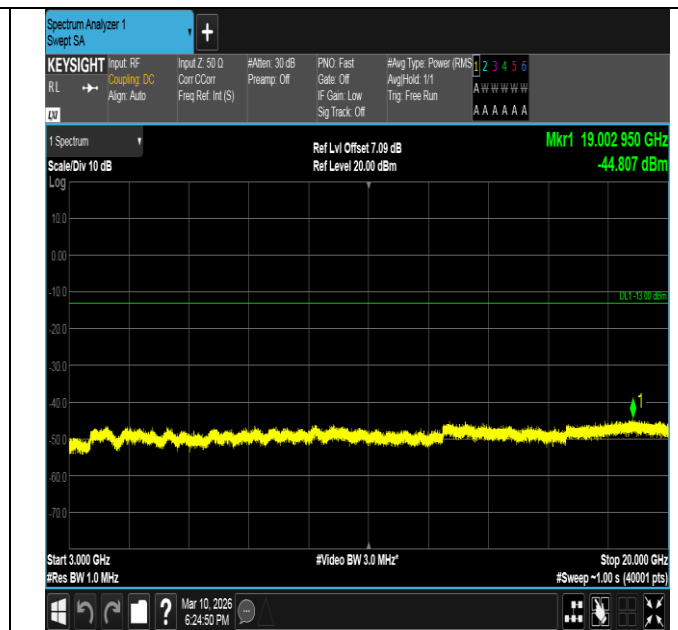
Band2-1.4MHz-16QAM-19193-6RB#0-3000~20000-PASS
