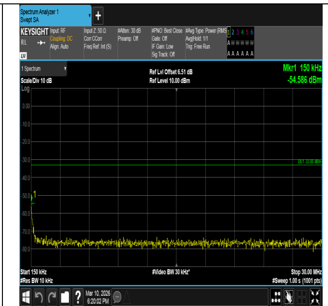
Band2-1.4MHz-QPSK-19193-1RB#0-0.15~30-PASS
