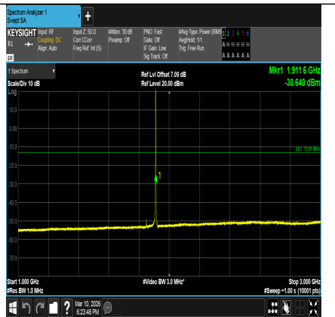
Band2-1.4MHz-QPSK-19193-6RB#0-1000~3000-PASS
