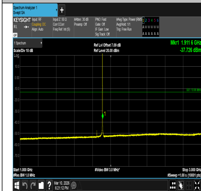
Band2-1.4MHz-16QAM-19193-1RB#0-1000~3000-PASS
