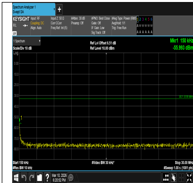
Band2-1.4MHz-16QAM-19193-1RB#0-0.15~30-PASS
