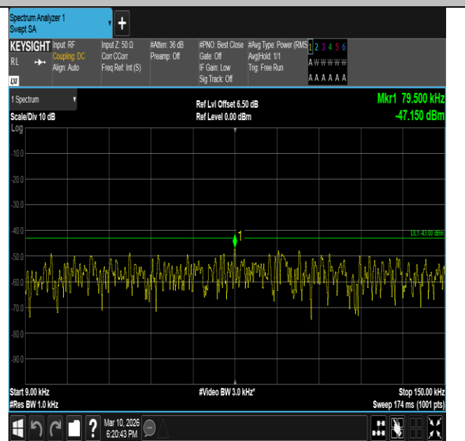
Band2-1.4MHz-16QAM-19193-1RB#0-0.009~0.15-PASS
