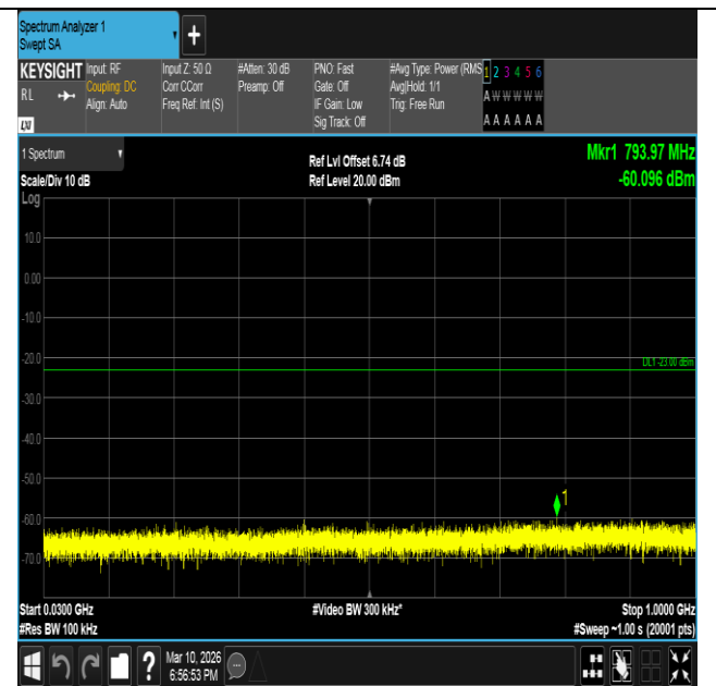
Band2-3MHz-QPSK-18615-1RB#14-30~1000-PASS
