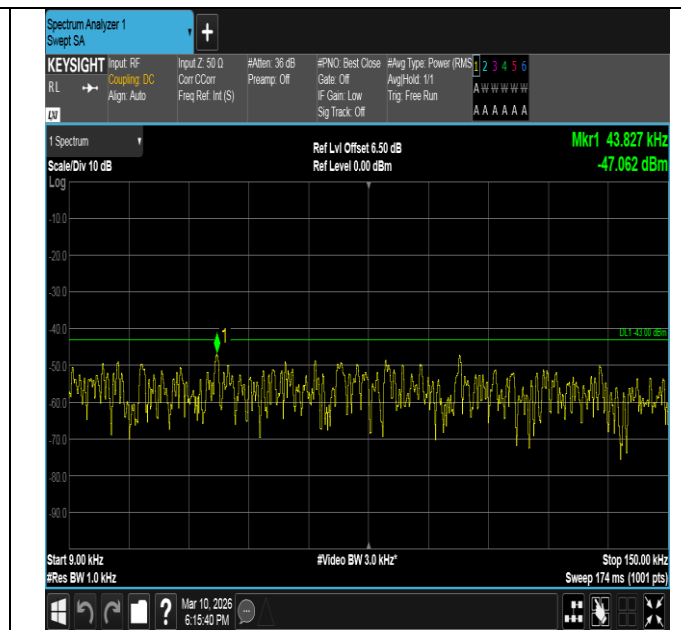
Band2-1.4MHz-16QAM-18900-1RB#0-0.009~0.15-PASS
