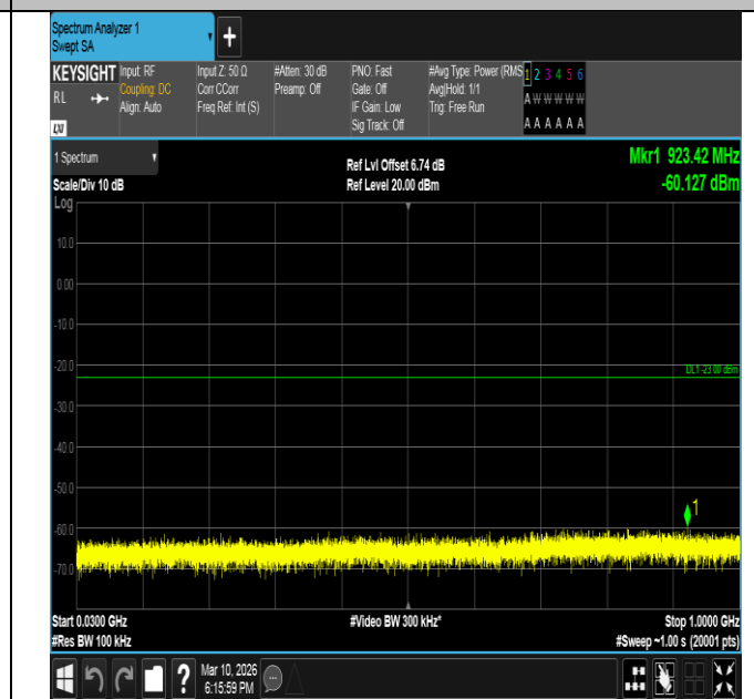
Band2-1.4MHz-16QAM-18900-1RB#0-30~1000-PASS
