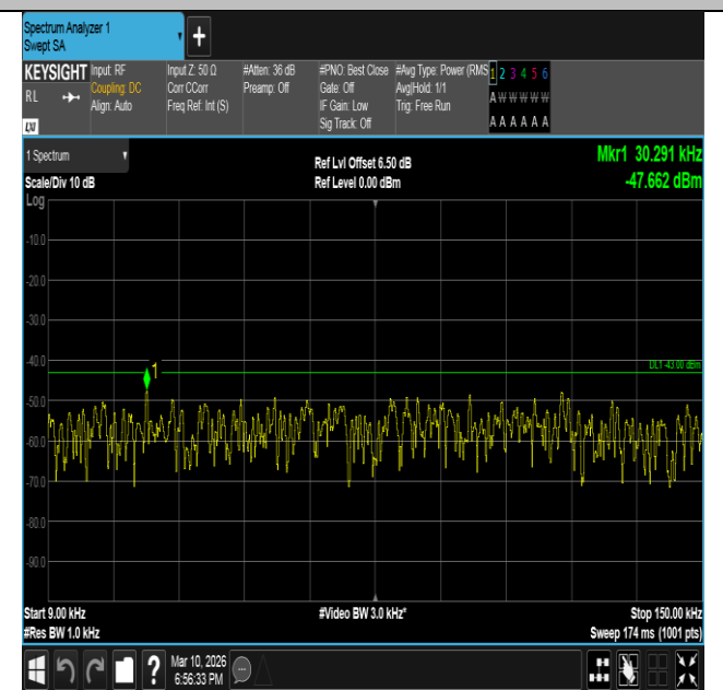
Band2-3MHz-QPSK-18615-1RB#14-0.009~0.15-PASS
