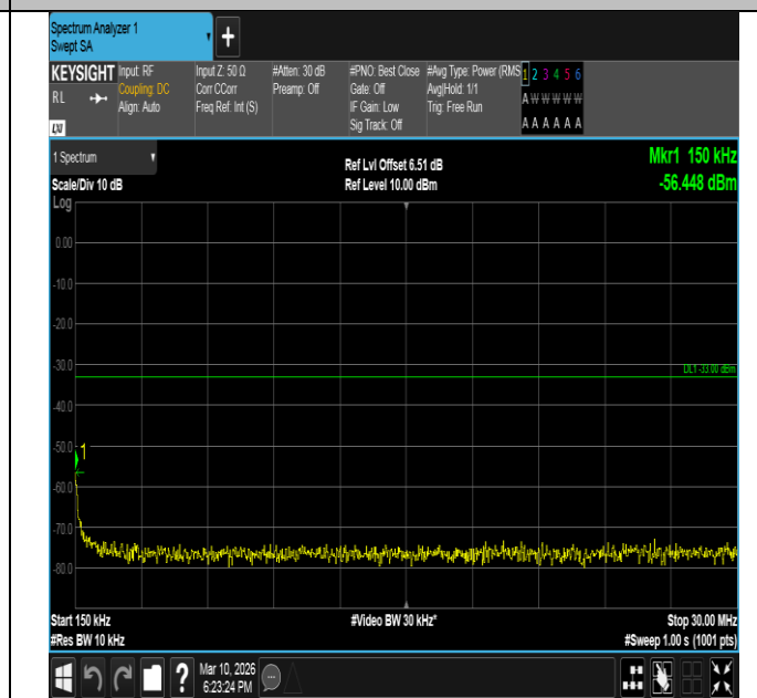
Band2-1.4MHz-QPSK-19193-6RB#0-0.15~30-PASS
