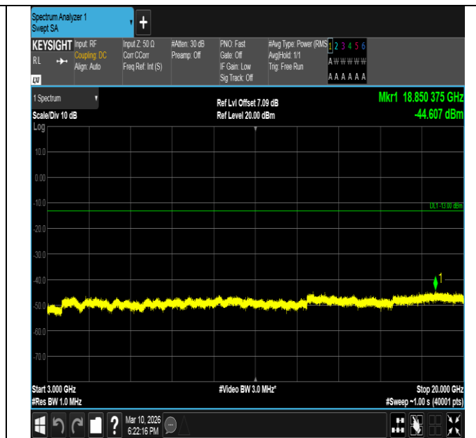
Band2-1.4MHz-QPSK-19193-1RB#5-3000~20000-PASS
