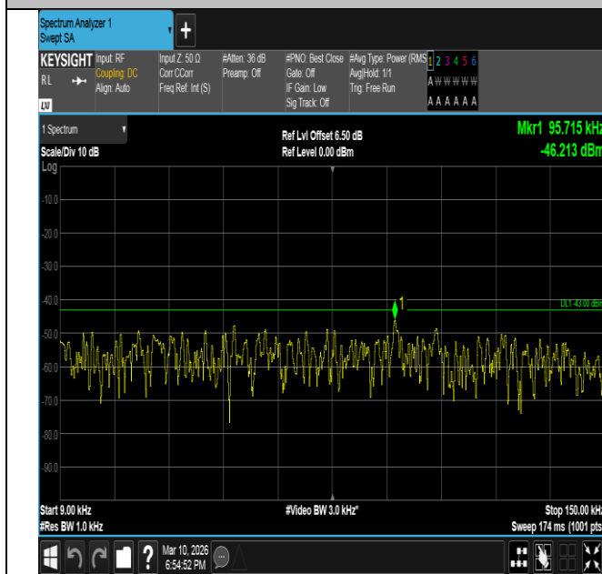
Band2-3MHz-QPSK-18615-1RB#0-0.009~0.15-PASS
