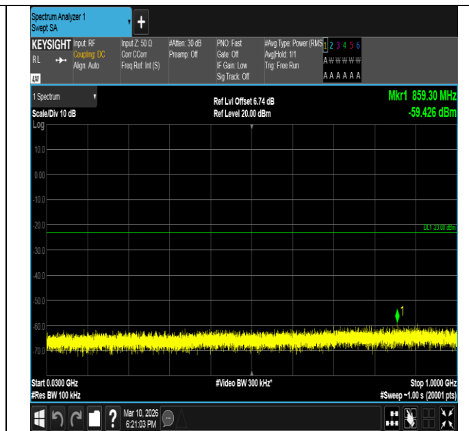
Band2-1.4MHz-16QAM-19193-1RB#0-30~1000-PASS
