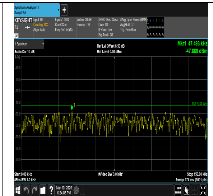
Band2-1.4MHz-16QAM-19193-6RB#0-0.009~0.15-PASS
