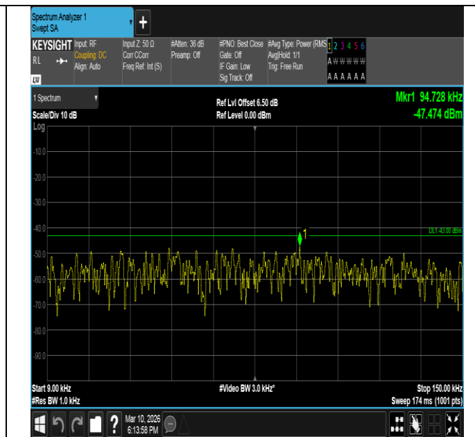
Band2-1.4MHz-16QAM-18607-6RB#0-0.009~0.15-PASS
