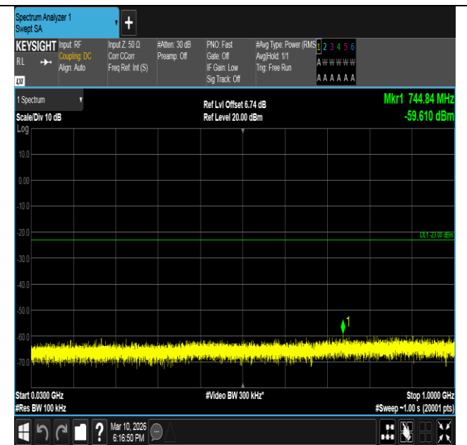
Band2-1.4MHz-QPSK-18900-1RB#5-30~1000-PASS
