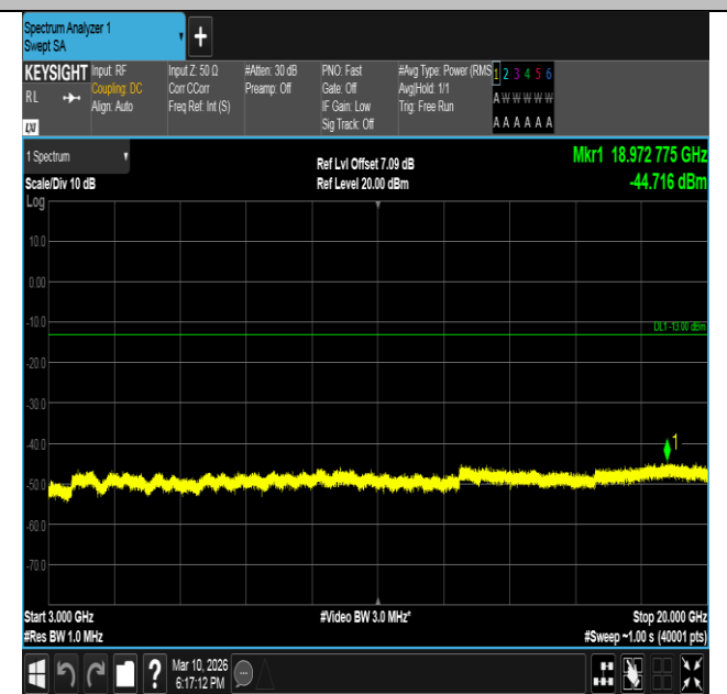
Band2-1.4MHz-QPSK-18900-1RB#5-3000~20000-PASS
