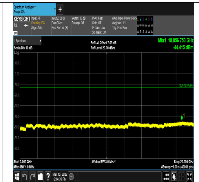
Band2-1.4MHz-16QAM-18607-6RB#0-3000~20000-PASS
