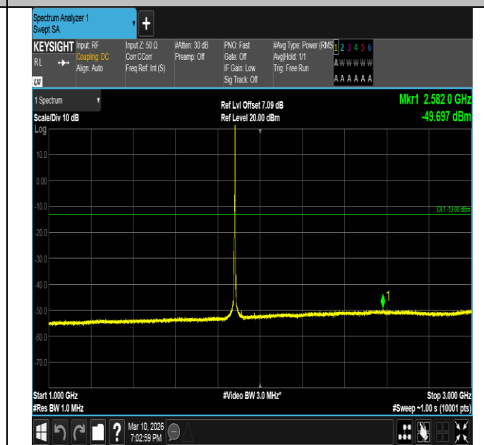
Band2-3MHz-16QAM-18900-1RB#14-1000~3000-PASS
