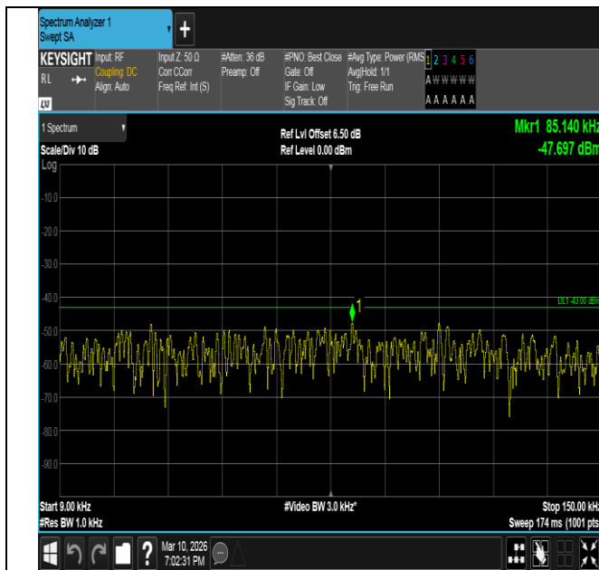
Band2-3MHz-16QAM-18900-1RB#14-0.009~0.15-PASS
