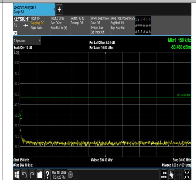
Band2-3MHz-QPSK-18900-15RB#0-0.15~30-PASS
