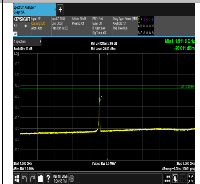
Band2-3MHz-QPSK-19185-15RB#0-1000~3000-PASS
