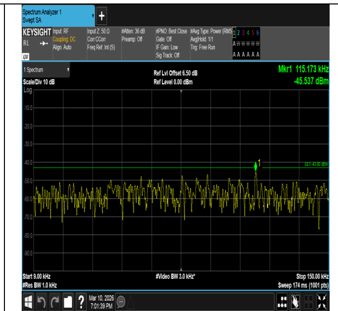
Band2-3MHz-QPSK-18900-1RB#14-0.009~0.15-PASS
