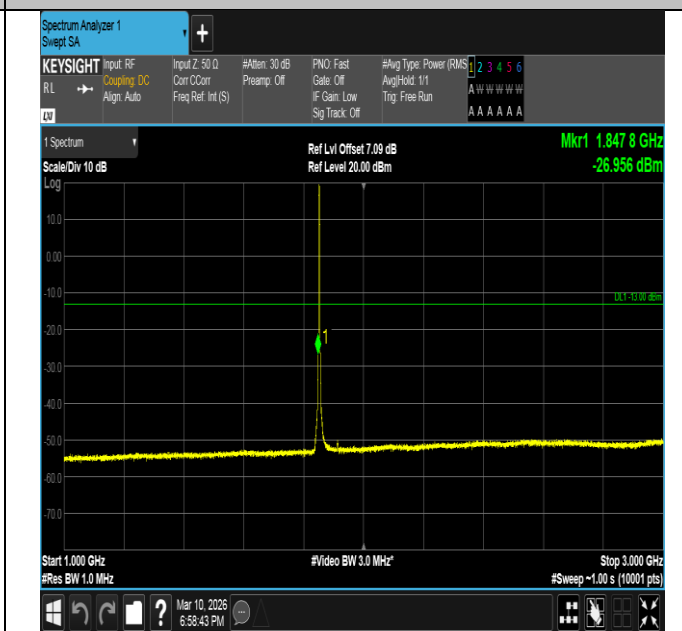
Band2-3MHz-QPSK-18615-15RB#0-1000~3000-PASS
