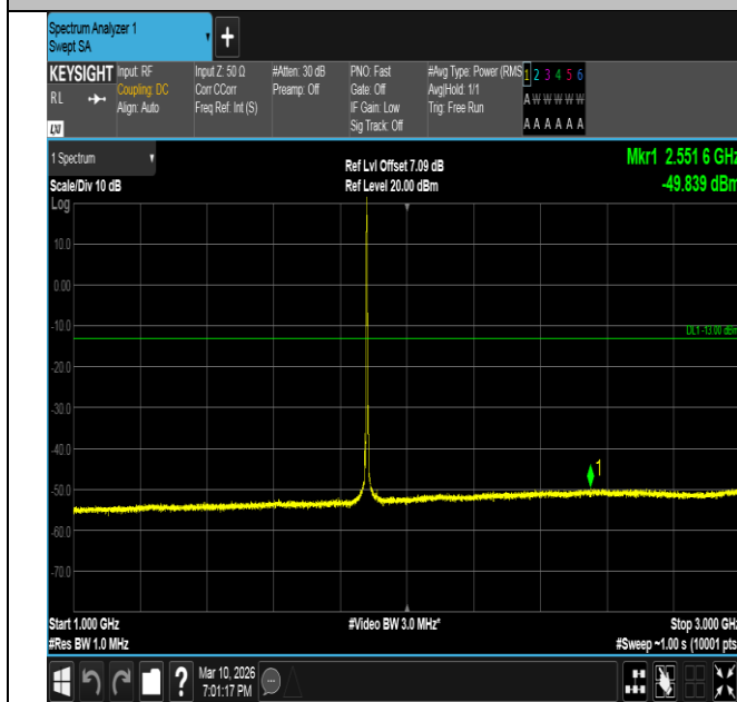
Band2-3MHz-16QAM-18900-1RB#0-1000~3000-PASS
