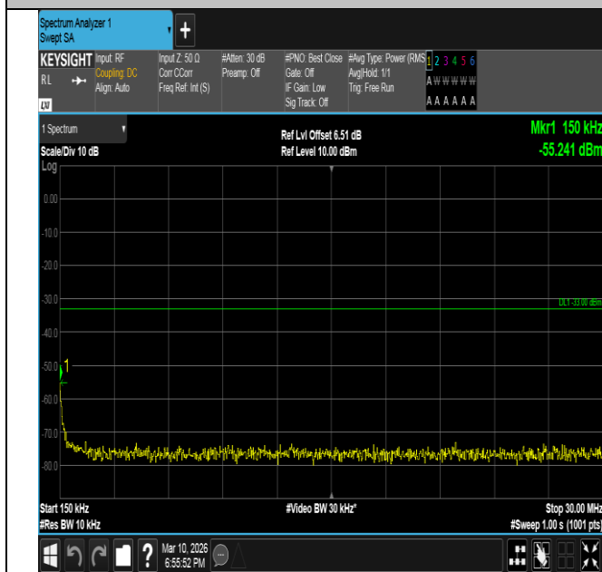
Band2-3MHz-16QAM-18615-1RB#0-0.15~30-PASS
