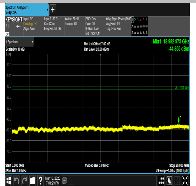
Band2-3MHz-16QAM-18900-1RB#0-3000~20000-PASS
