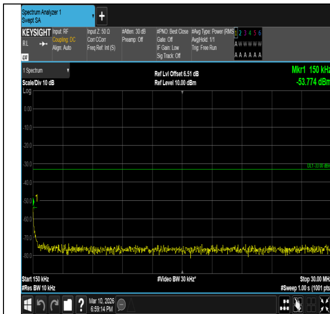
Band2-3MHz-16QAM-18615-15RB#0-0.15~30-PASS
