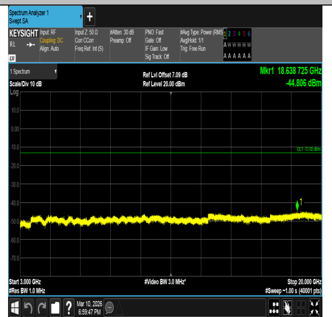
Band2-3MHz-16QAM-18615-15RB#0-3000~20000-PASS
