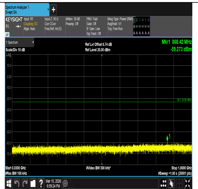
Band2-3MHz-16QAM-18615-15RB#0-30~1000-PASS
