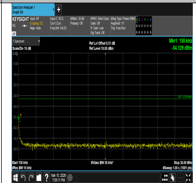
Band2-3MHz-QPSK-19185-1RB#0-0.15~30-PASS
