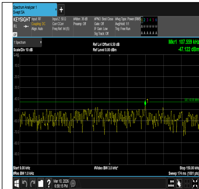
Band2-3MHz-QPSK-18615-15RB#0-0.009~0.15-PASS
