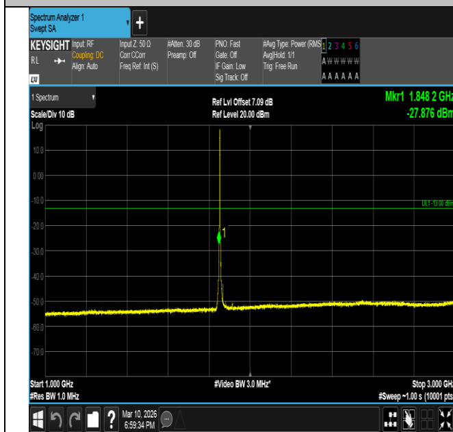
Band2-3MHz-16QAM-18615-15RB#0-1000~3000-PASS
