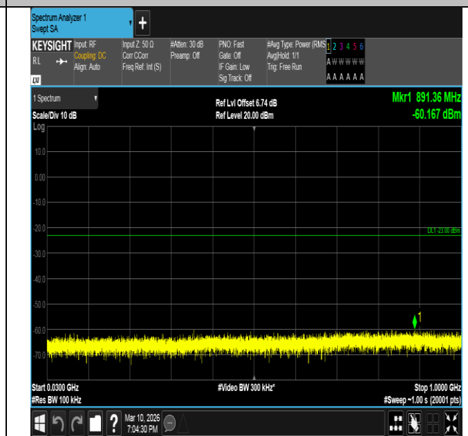
Band2-3MHz-16QAM-18900-15RB#0-30~1000-PASS
