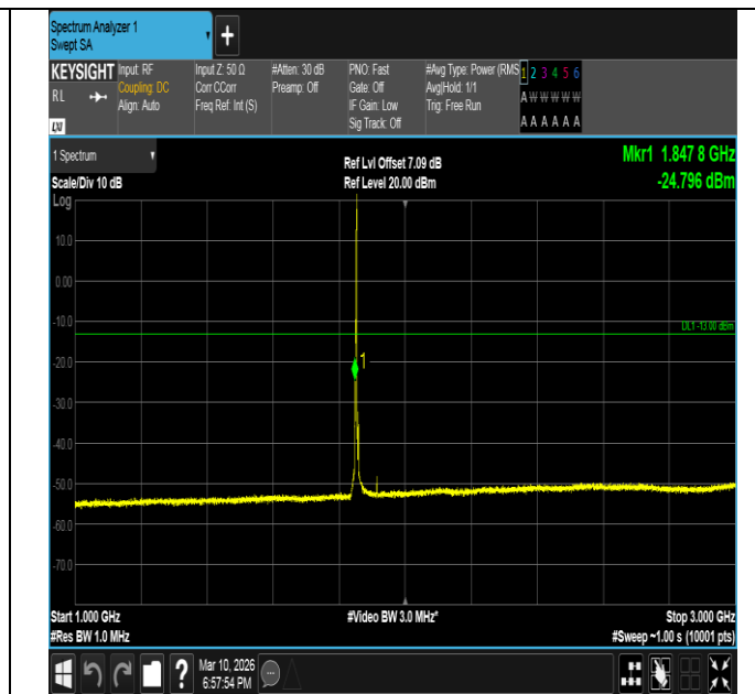
Band2-3MHz-16QAM-18615-1RB#14-1000~3000-PASS
