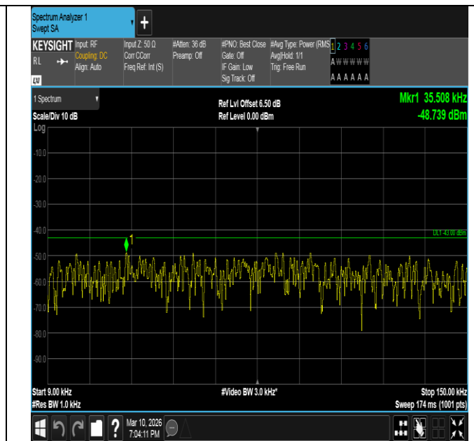
Band2-3MHz-16QAM-18900-15RB#0-0.009~0.15-PASS
