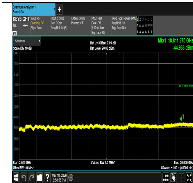
Band2-3MHz-QPSK-18615-15RB#0-3000~20000-PASS
