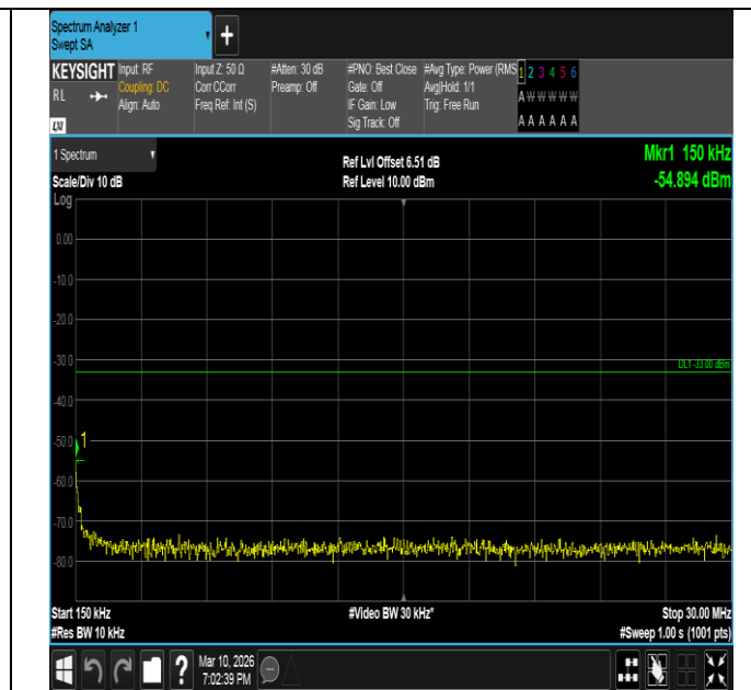
Band2-3MHz-16QAM-18900-1RB#14-0.15~30-PASS
