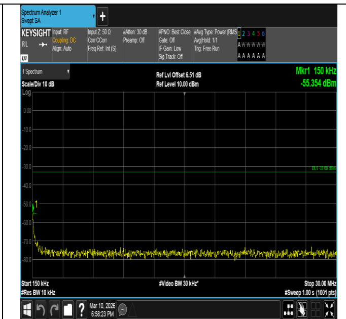
Band2-3MHz-QPSK-18615-15RB#0-0.15~30-PASS
