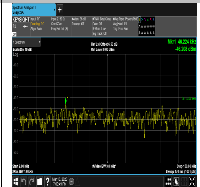
Band2-3MHz-16QAM-18900-1RB#0-0.009~0.15-PASS
