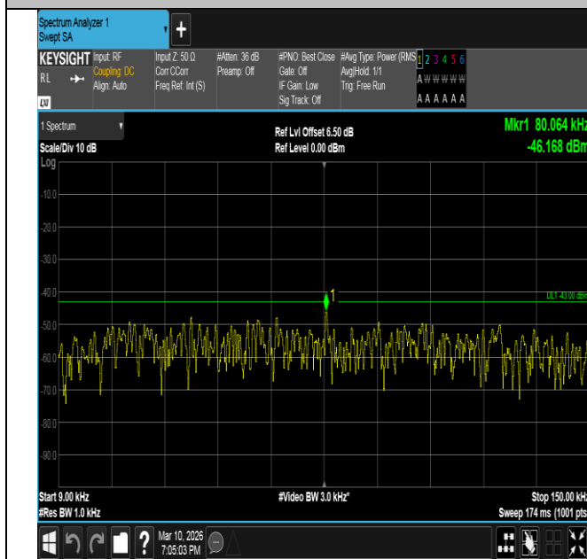
Band2-3MHz-QPSK-19185-1RB#0-0.009~0.15-PASS
