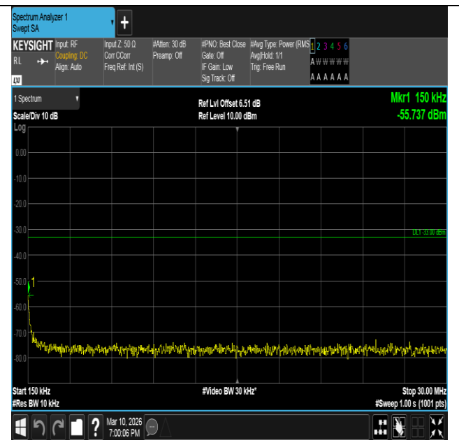
Band2-3MHz-QPSK-18900-1RB#0-0.15~30-PASS
