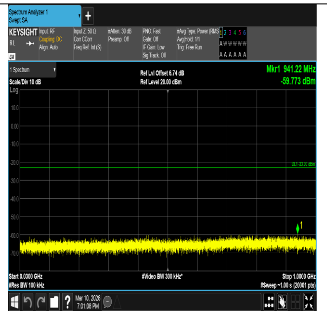
Band2-3MHz-16QAM-18900-1RB#0-30~1000-PASS
