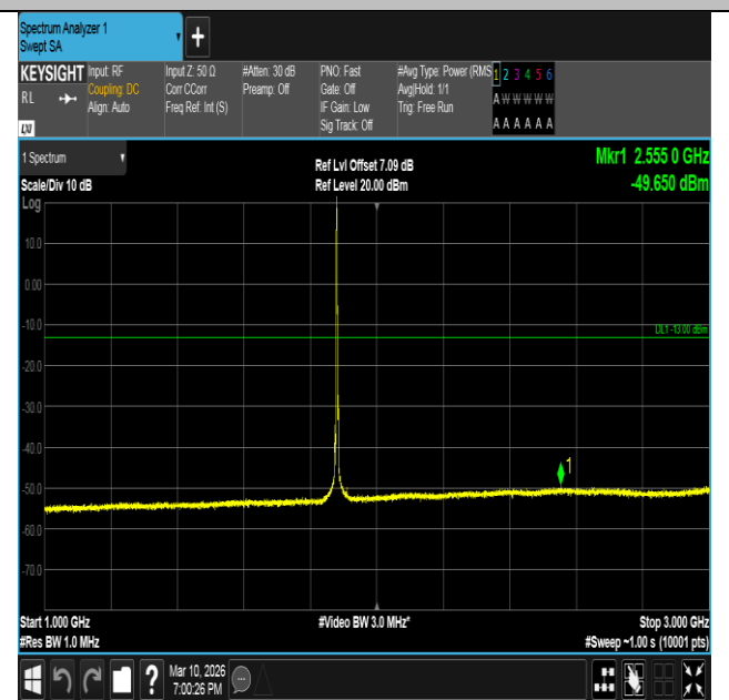
Band2-3MHz-QPSK-18900-1RB#0-1000~3000-PASS
