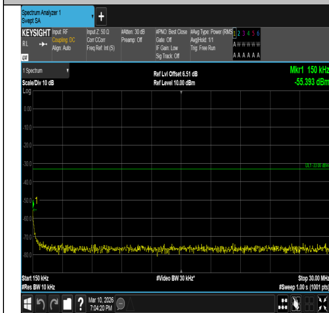
Band2-3MHz-16QAM-18900-15RB#0-0.15~30-PASS
