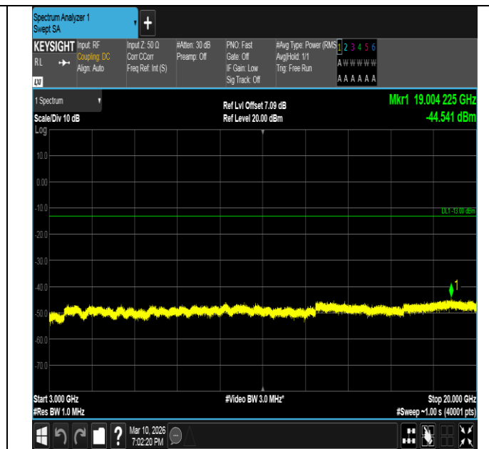
Band2-3MHz-QPSK-18900-1RB#14-3000~20000-PASS
