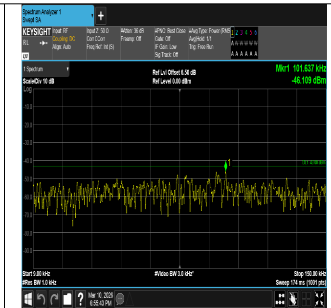
Band2-3MHz-16QAM-18615-1RB#0-0.009~0.15-PASS
