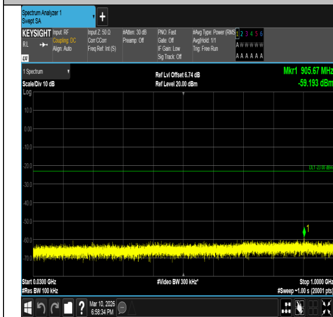
Band2-3MHz-QPSK-18615-15RB#0-30~1000-PASS
