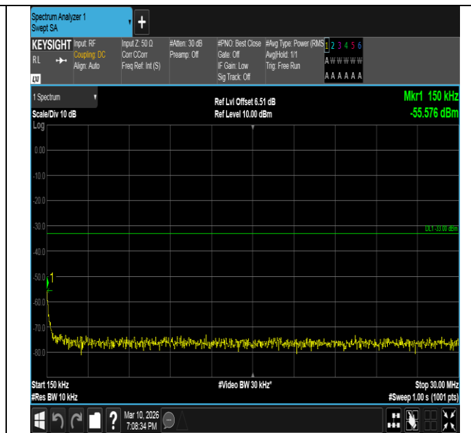
Band2-3MHz-QPSK-19185-15RB#0-0.15~30-PASS
