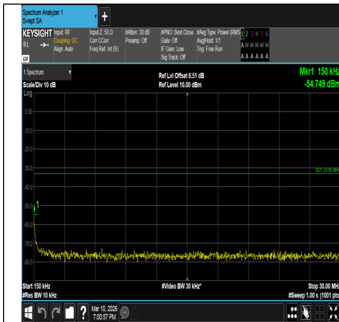
Band2-3MHz-16QAM-18900-1RB#0-0.15~30-PASS
