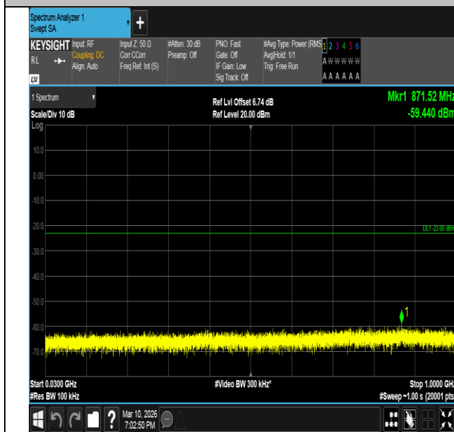
Band2-3MHz-16QAM-18900-1RB#14-30~1000-PASS
