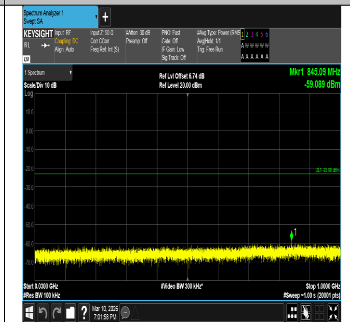
Band2-3MHz-QPSK-18900-1RB#14-30~1000-PASS
