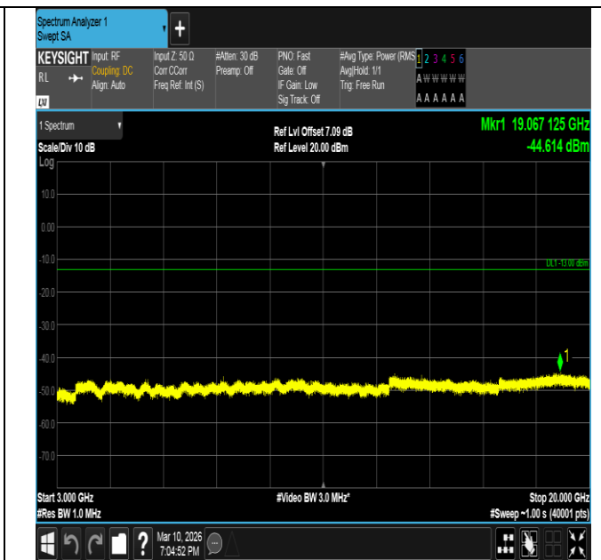
Band2-3MHz-16QAM-18900-15RB#0-3000~20000-PASS
