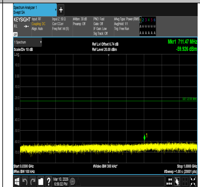
Band2-3MHz-16QAM-18615-1RB#0-30~1000-PASS
