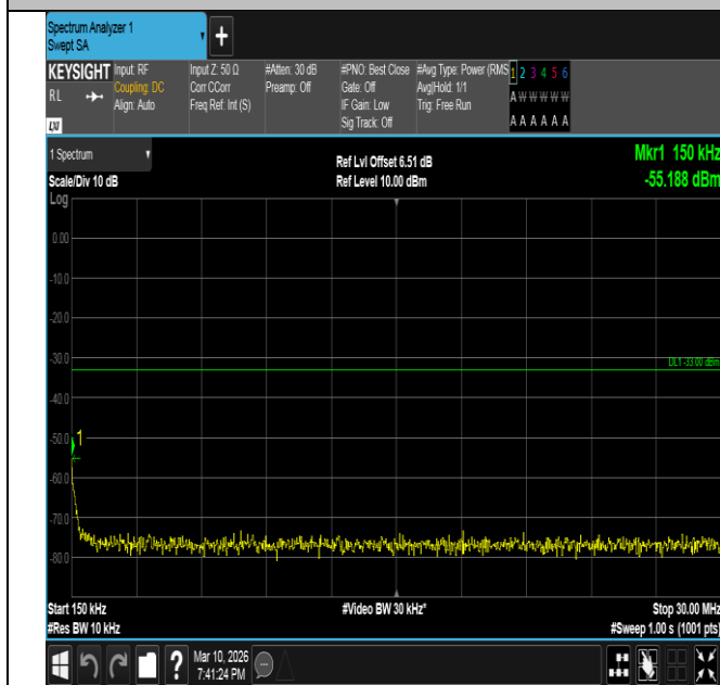
Band2-5MHz-QPSK-18625-1RB#24-0.15~30-PASS
