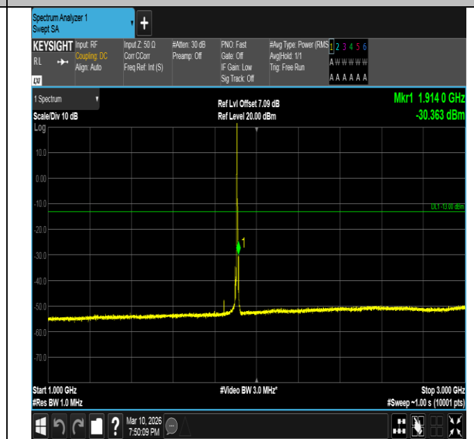
Band2-5MHz-QPSK-19175-1RB#0-1000~3000-PASS
