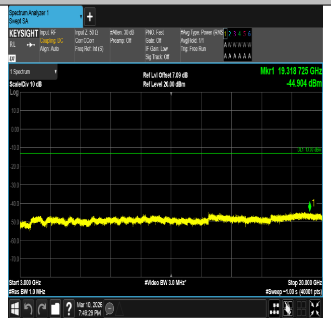
Band2-5MHz-16QAM-18900-25RB#0-3000~20000-PASS
