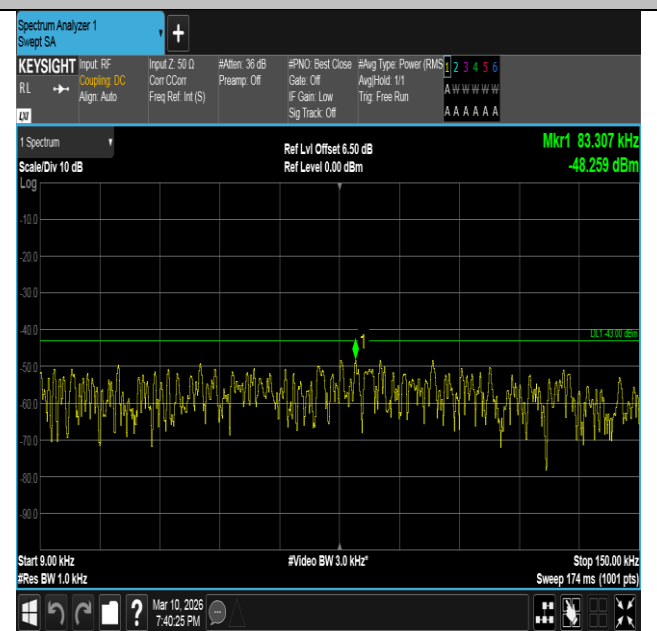
Band2-5MHz-16QAM-18625-1RB#0-0.009~0.15-PASS
