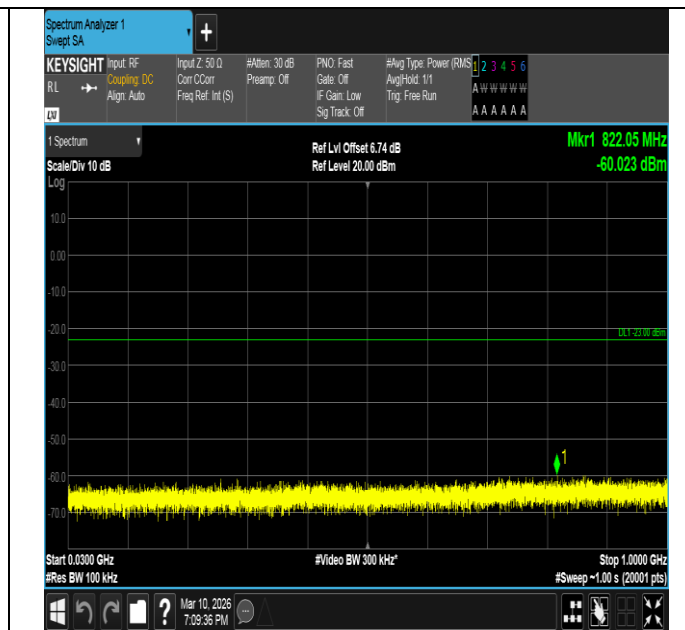
Band2-3MHz-16QAM-19185-15RB#0-30~1000-PASS
