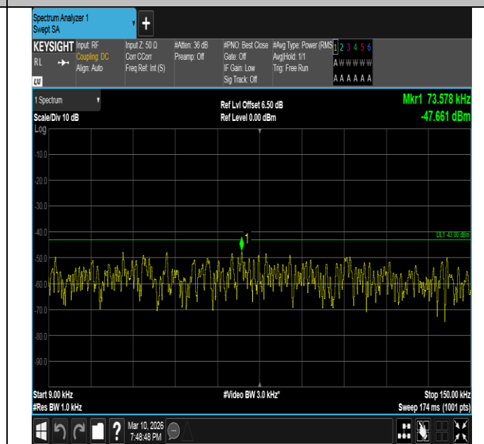
Band2-5MHz-16QAM-18900-25RB#0-0.009~0.15-PASS
