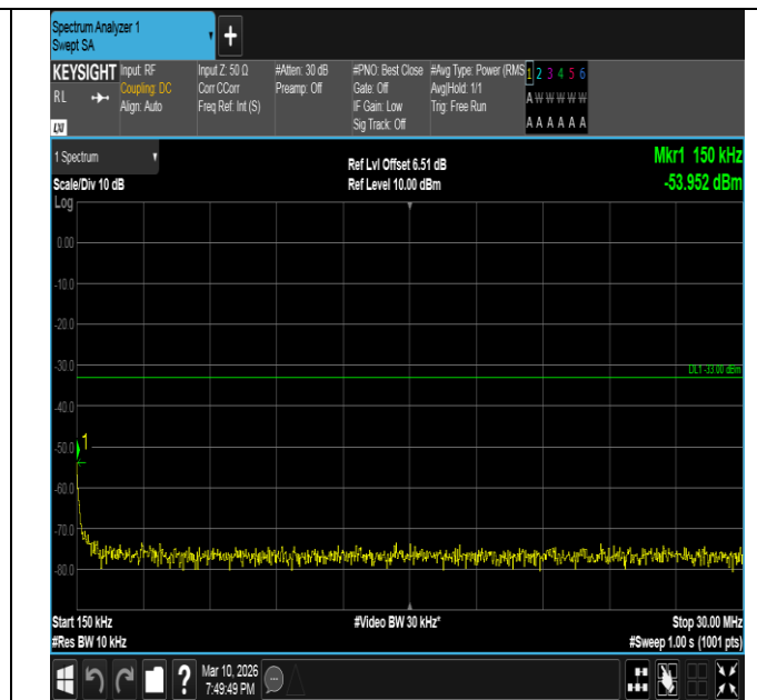
Band2-5MHz-QPSK-19175-1RB#0-0.15~30-PASS
