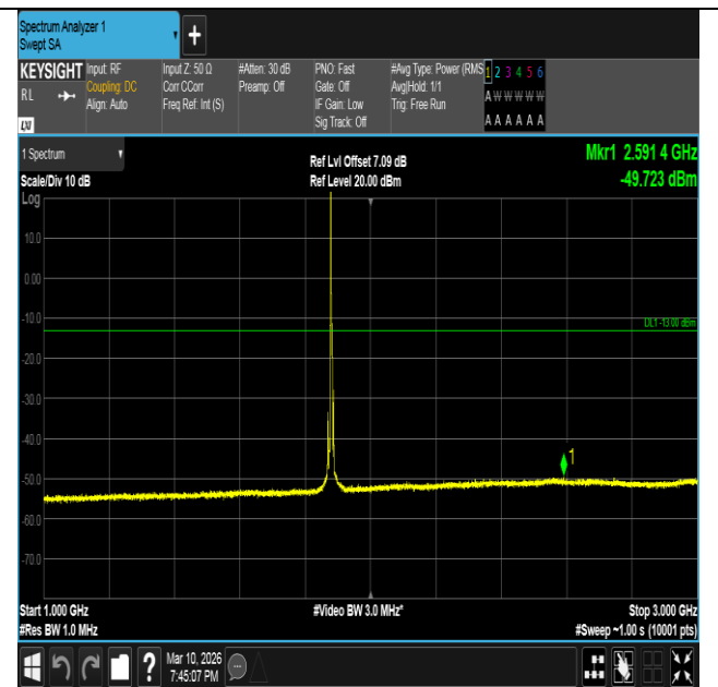
Band2-5MHz-QPSK-18900-1RB#0-1000~3000-PASS
