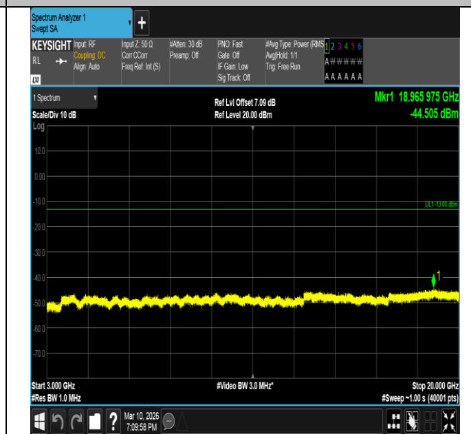
Band2-3MHz-16QAM-19185-15RB#0-3000~20000-PASS
