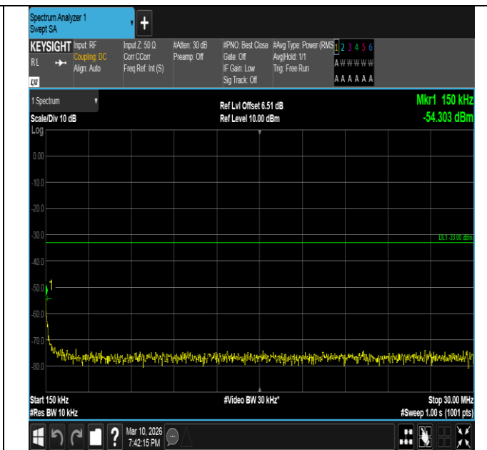
Band2-5MHz-16QAM-18625-1RB#24-0.15~30-PASS
