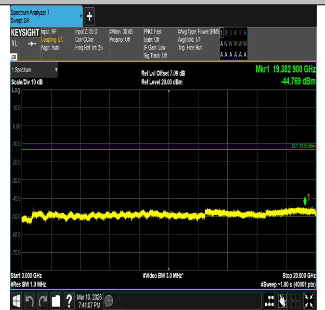
Band2-5MHz-16QAM-18625-1RB#0-3000~20000-PASS
