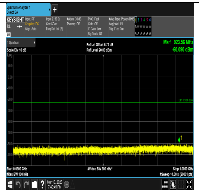
Band2-5MHz-16QAM-18625-1RB#0-30~1000-PASS
