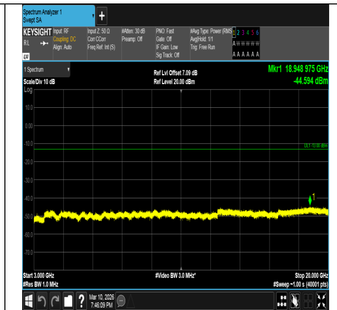
Band2-5MHz-16QAM-18900-1RB#0-3000~20000-PASS
