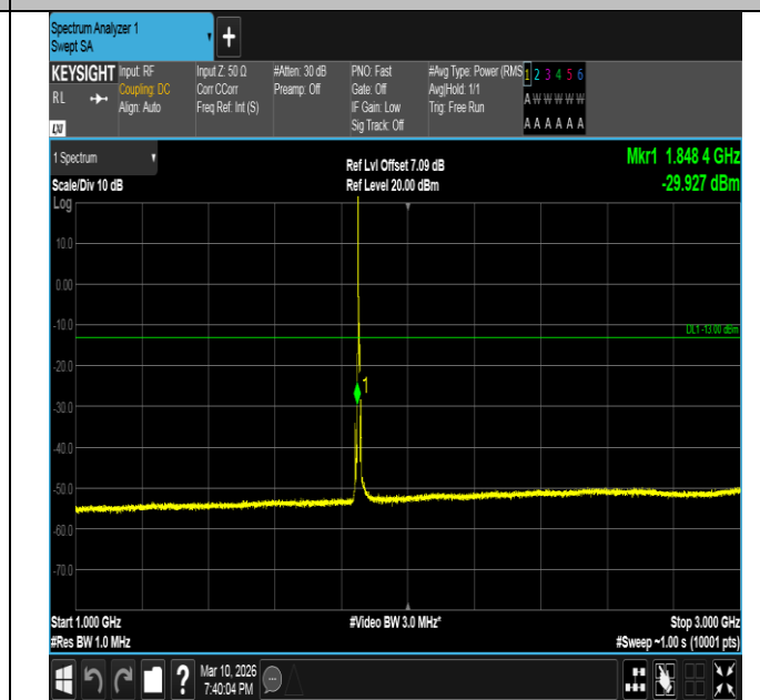
Band2-5MHz-QPSK-18625-1RB#0-1000~3000-PASS
