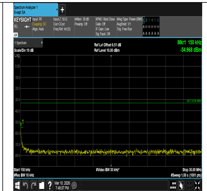
Band2-5MHz-QPSK-18900-25RB#0-0.15~30-PASS
