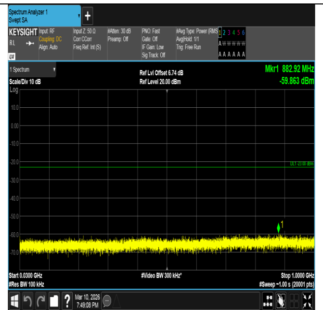
Band2-5MHz-16QAM-18900-25RB#0-30~1000-PASS
