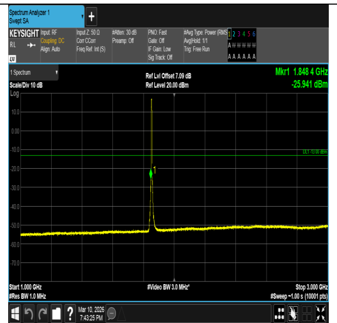
Band2-5MHz-QPSK-18625-25RB#0-1000~3000-PASS
