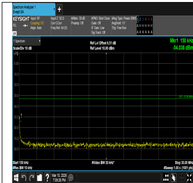
Band2-3MHz-16QAM-19185-15RB#0-0.15~30-PASS
