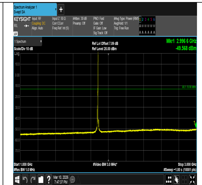
Band2-5MHz-16QAM-18900-1RB#24-1000~3000-PASS
