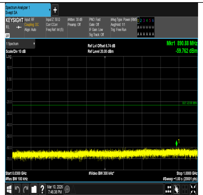
Band2-5MHz-QPSK-18900-1RB#24-30~1000-PASS
