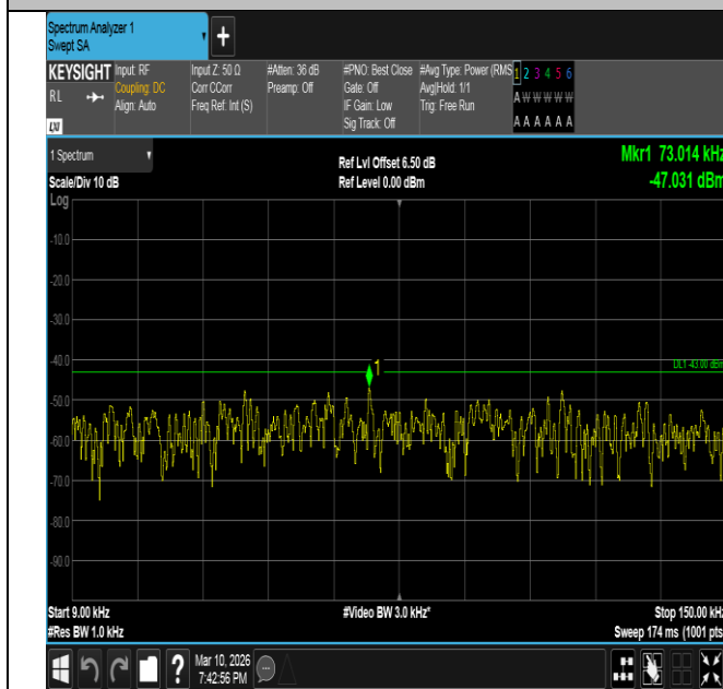
Band2-5MHz-QPSK-18625-25RB#0-0.009~0.15-PASS
