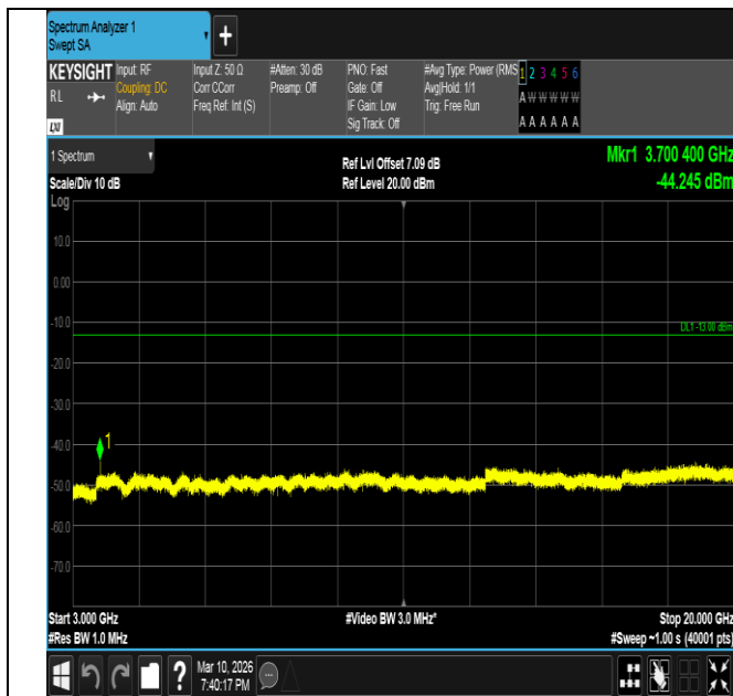
Band2-5MHz-QPSK-18625-1RB#0-3000~20000-PASS
