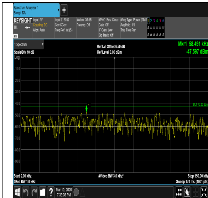
Band2-5MHz-QPSK-18625-1RB#0-0.009~0.15-PASS
