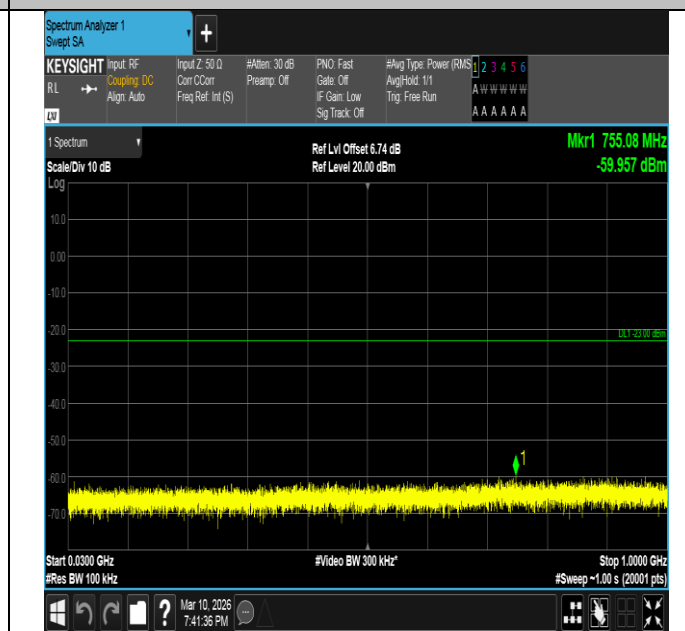
Band2-5MHz-QPSK-18625-1RB#24-30~1000-PASS
