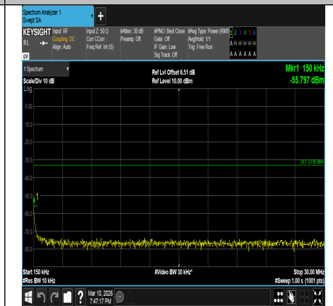
Band2-5MHz-16QAM-18900-1RB#24-0.15~30-PASS
