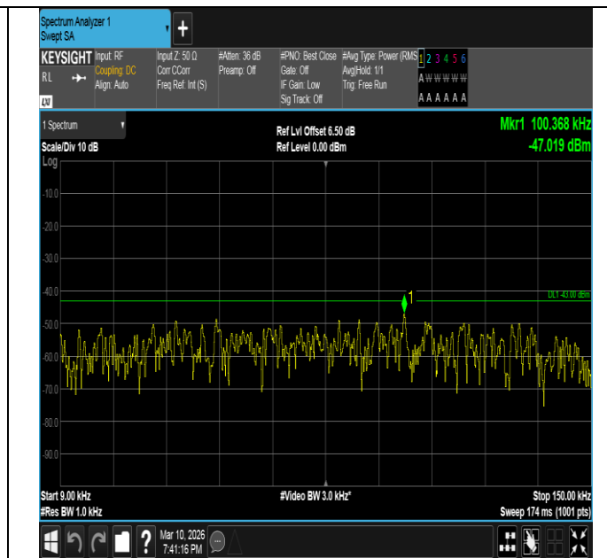
Band2-5MHz-QPSK-18625-1RB#24-0.009~0.15-PASS
