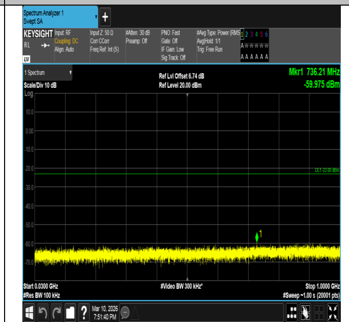
Band2-5MHz-QPSK-19175-1RB#24-30~1000-PASS
