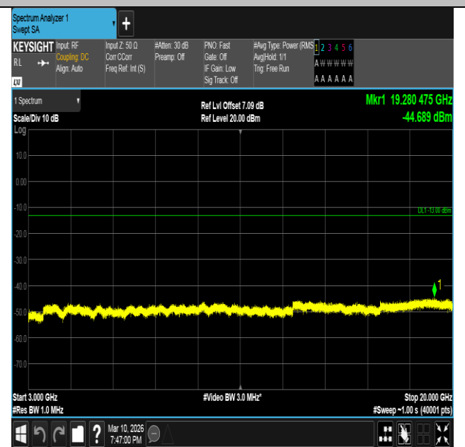
Band2-5MHz-QPSK-18900-1RB#24-3000~20000-PASS
