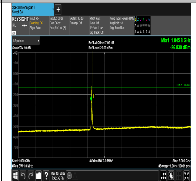
Band2-5MHz-16QAM-18625-1RB#24-1000~3000-PASS
