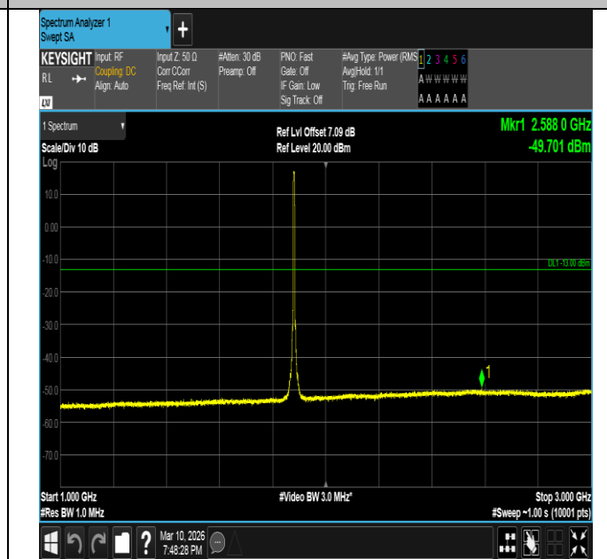
Band2-5MHz-QPSK-18900-25RB#0-1000~3000-PASS
