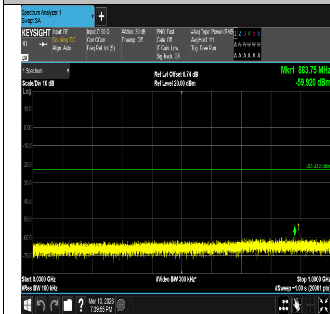
Band2-5MHz-QPSK-18625-1RB#0-30~1000-PASS
