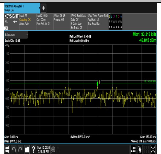
Band2-5MHz-QPSK-18900-1RB#24-0.009~0.15-PASS
