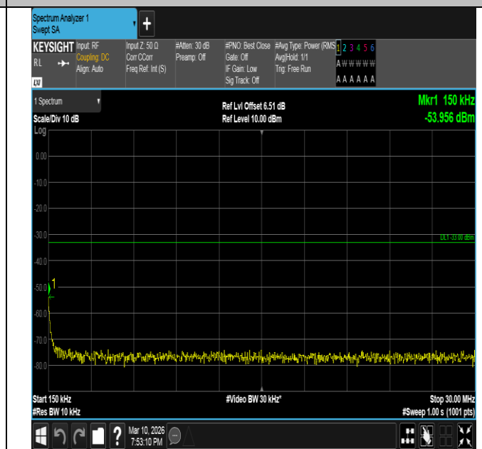
Band2-5MHz-QPSK-19175-25RB#0-0.15~30-PASS
