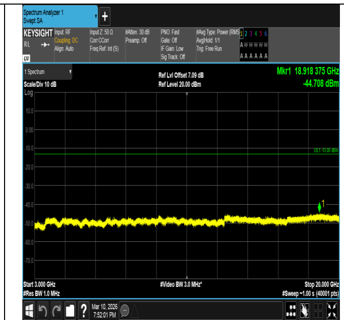
Band2-5MHz-QPSK-19175-1RB#24-3000~20000-PASS
