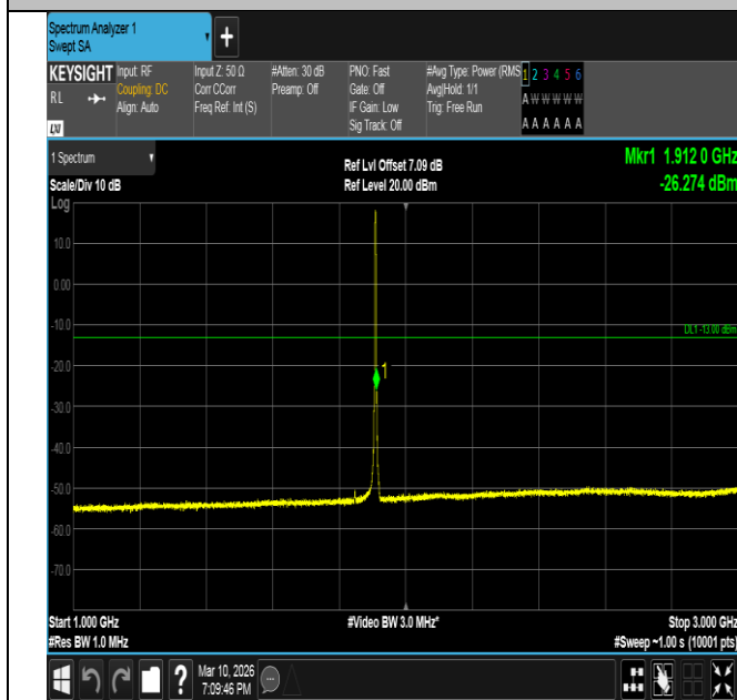
Band2-3MHz-16QAM-19185-15RB#0-1000~3000-PASS
