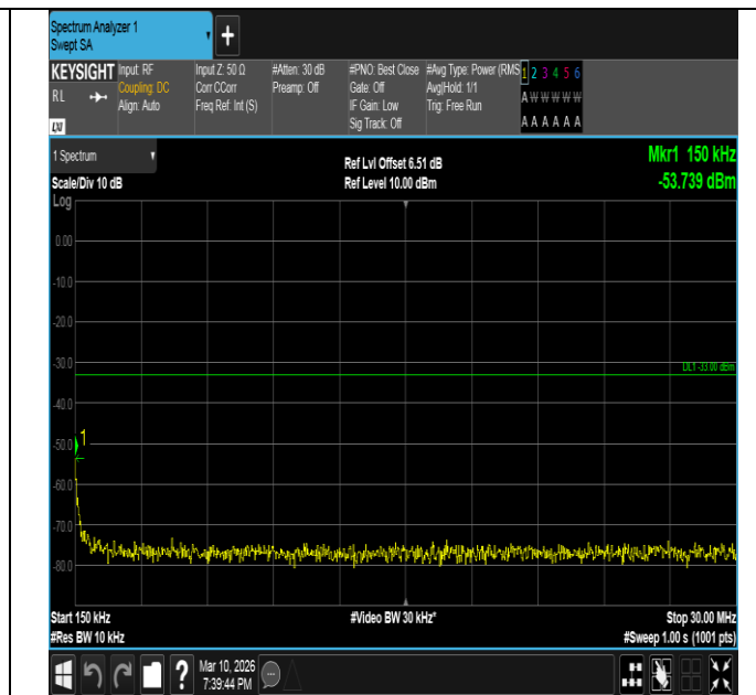
Band2-5MHz-QPSK-18625-1RB#0-0.15~30-PASS
