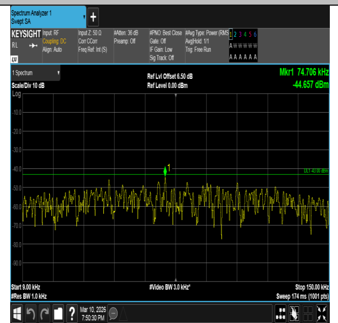
Band2-5MHz-16QAM-19175-1RB#0-0.009~0.15-PASS
