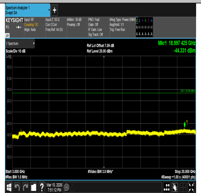
Band2-5MHz-16QAM-19175-1RB#0-3000~20000-PASS
