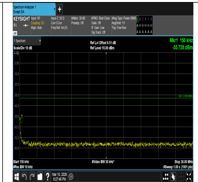
Band2-10MHz-QPSK-18900-1RB#0-0.15~30-PASS
