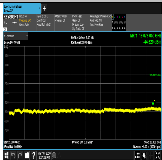
Band2-10MHz-16QAM-18650-50RB#0-3000~20000-PASS
