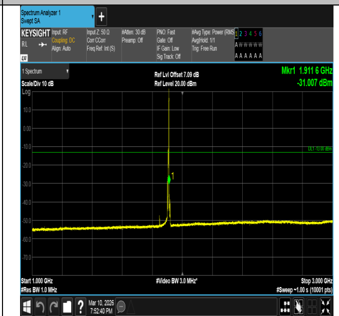
Band2-5MHz-16QAM-19175-1RB#24-1000~3000-PASS
