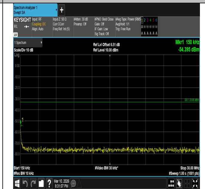
Band2-10MHz-QPSK-18900-50RB#0-0.15~30-PASS
