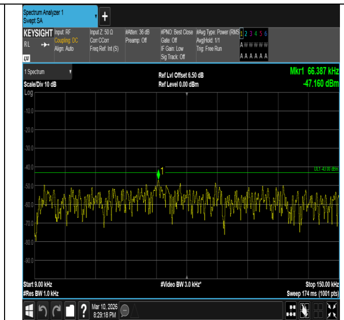
Band2-10MHz-QPSK-18900-1RB#49-0.009~0.15-PASS
