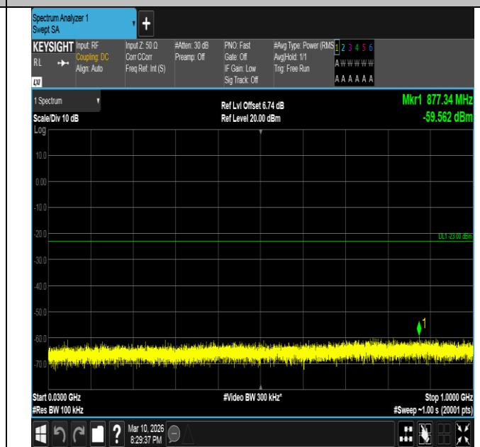
Band2-10MHz-QPSK-18900-1RB#49-30~1000-PASS
