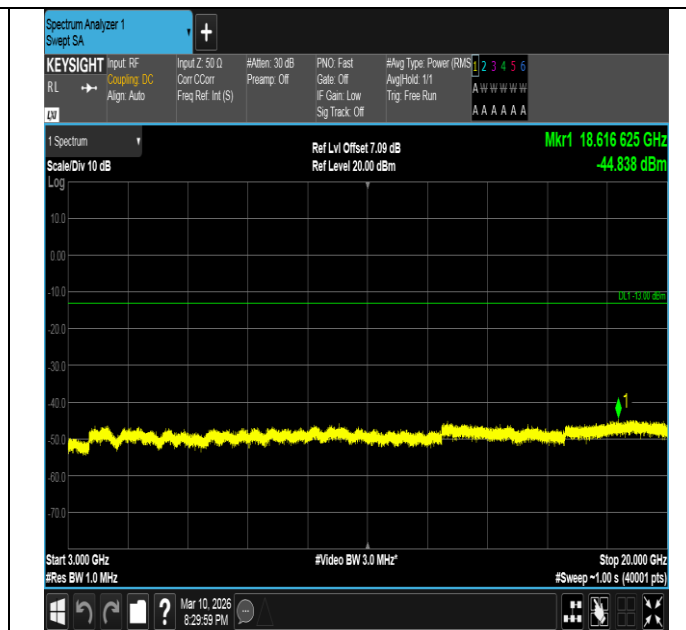
Band2-10MHz-QPSK-18900-1RB#49-3000~20000-PASS
