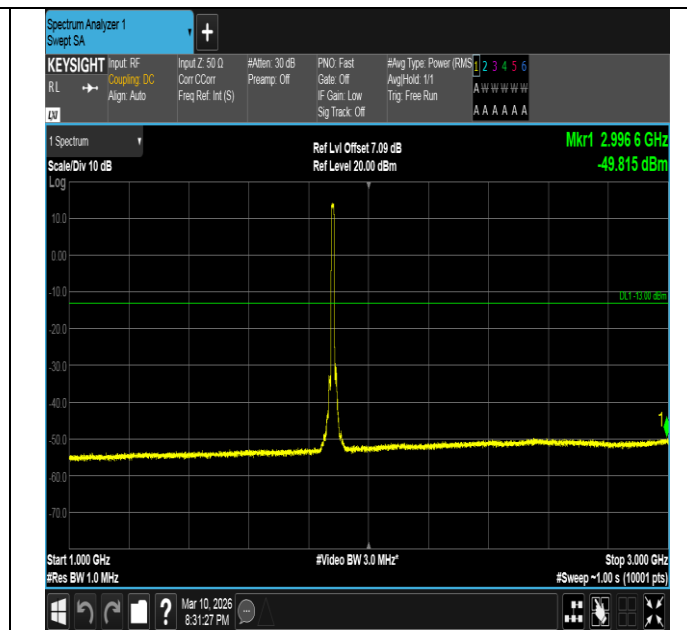
Band2-10MHz-QPSK-18900-50RB#0-1000~3000-PASS
