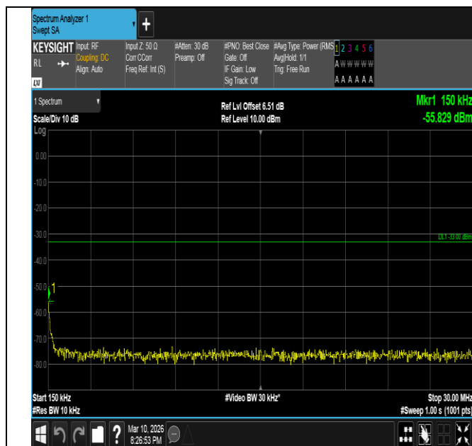
Band2-10MHz-16QAM-18650-50RB#0-0.15~30-PASS
