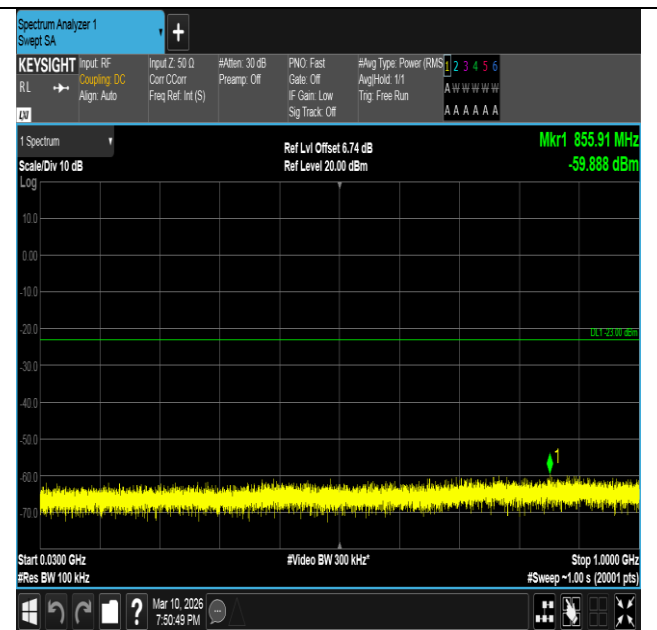
Band2-5MHz-16QAM-19175-1RB#0-30~1000-PASS
