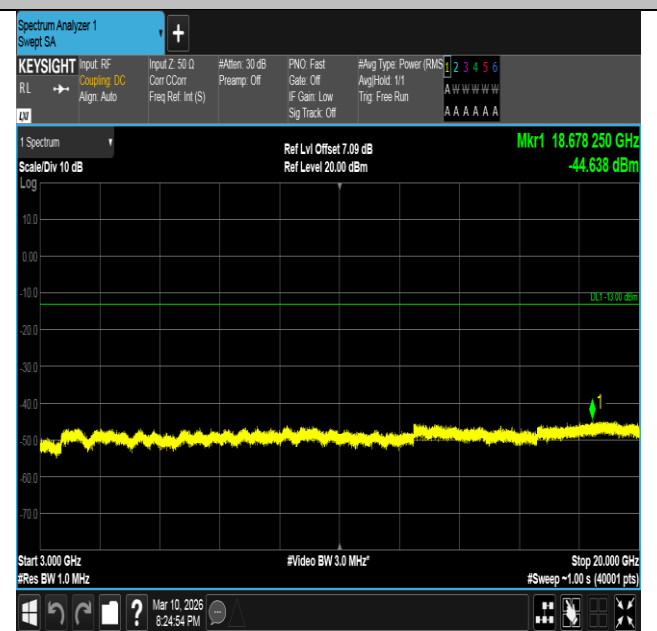
Band2-10MHz-QPSK-18650-1RB#49-3000~20000-PASS
