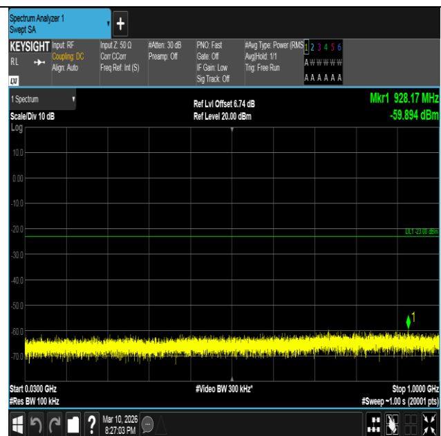
Band2-10MHz-16QAM-18650-50RB#0-30~1000-PASS
