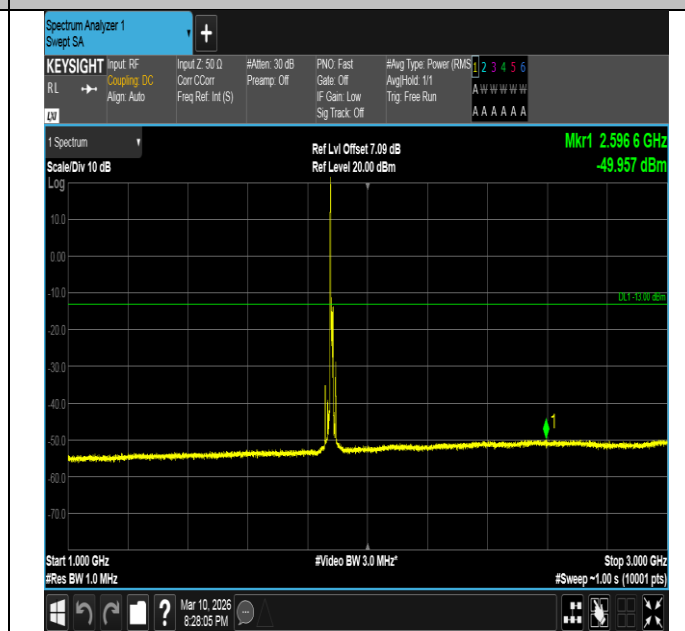
Band2-10MHz-QPSK-18900-1RB#0-1000~3000-PASS
