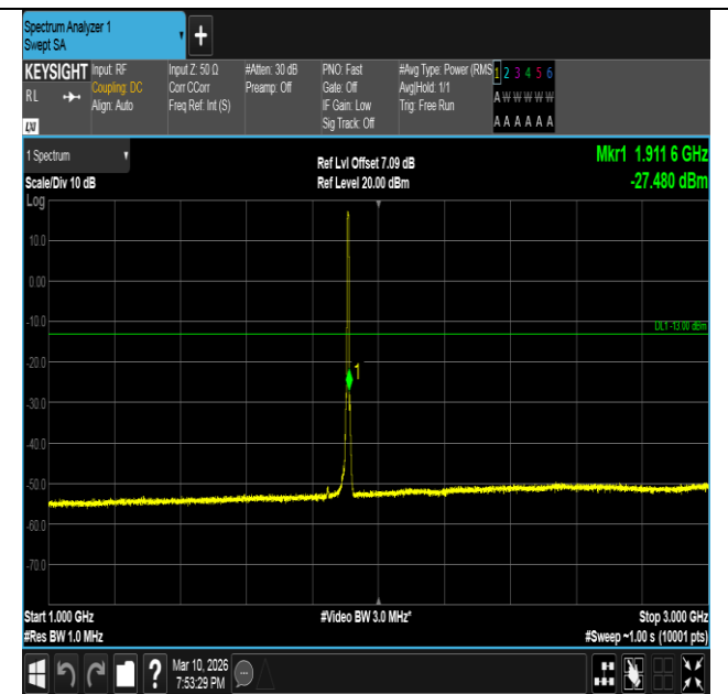
Band2-5MHz-QPSK-19175-25RB#0-1000~3000-PASS
