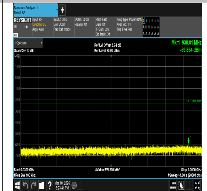
Band2-10MHz-16QAM-18650-1RB#0-30~1000-PASS
