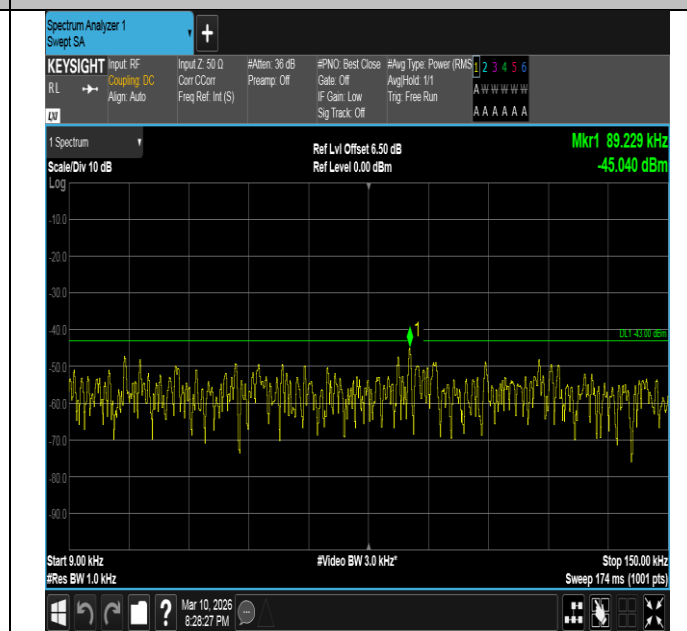
Band2-10MHz-16QAM-18900-1RB#0-0.009~0.15-PASS
