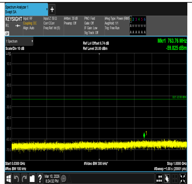
Band2-10MHz-QPSK-18650-1RB#49-30~1000-PASS
