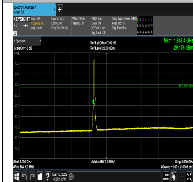
Band2-10MHz-16QAM-18650-50RB#0-1000~3000-PASS
