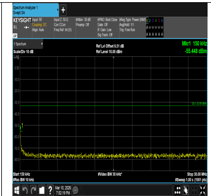
Band2-5MHz-16QAM-19175-1RB#24-0.15~30-PASS
