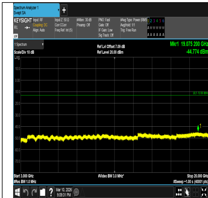
Band2-15MHz-16QAM-18675-1RB#74-3000~20000-PASS
