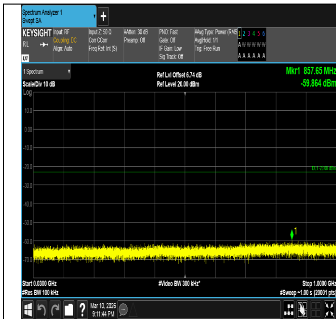
Band2-15MHz-QPSK-18900-1RB#0-30~1000-PASS
