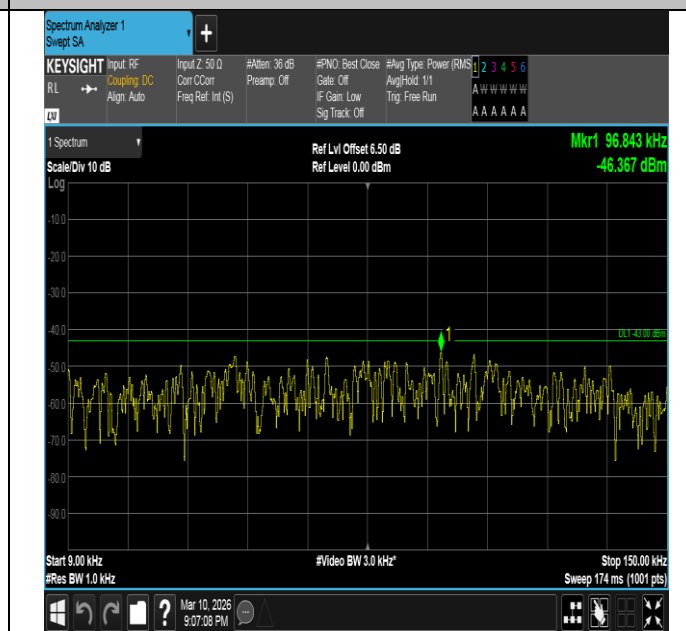
Band2-15MHz-16QAM-18675-1RB#0-0.009~0.15-PASS
