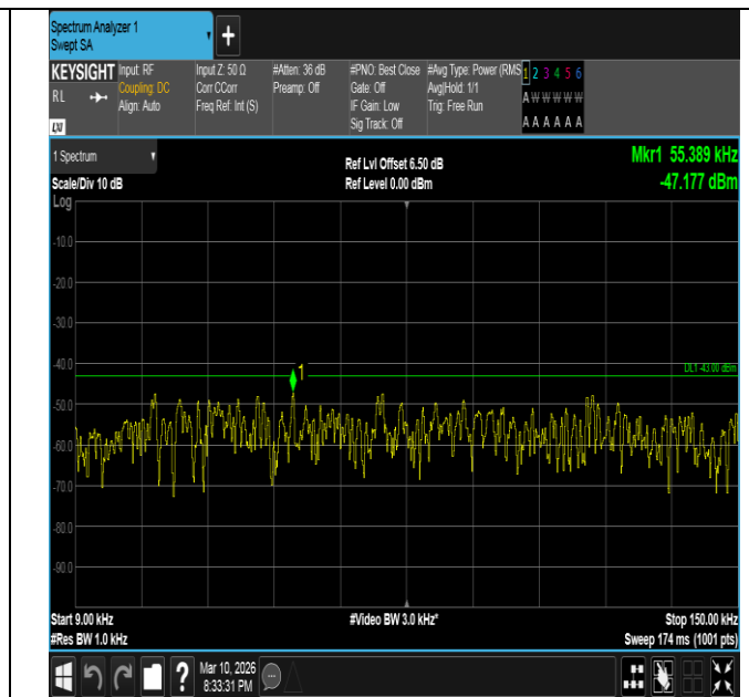
Band2-10MHz-16QAM-19150-1RB#0-0.009~0.15-PASS
