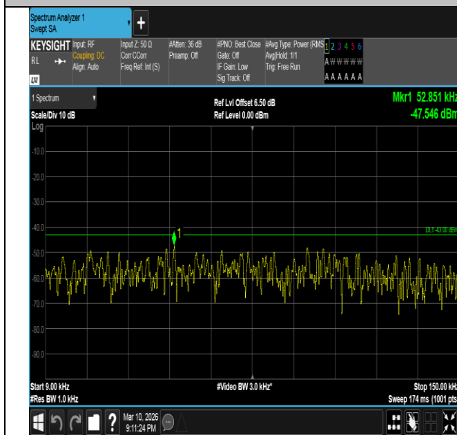
Band2-15MHz-QPSK-18900-1RB#0-0.009~0.15-PASS
