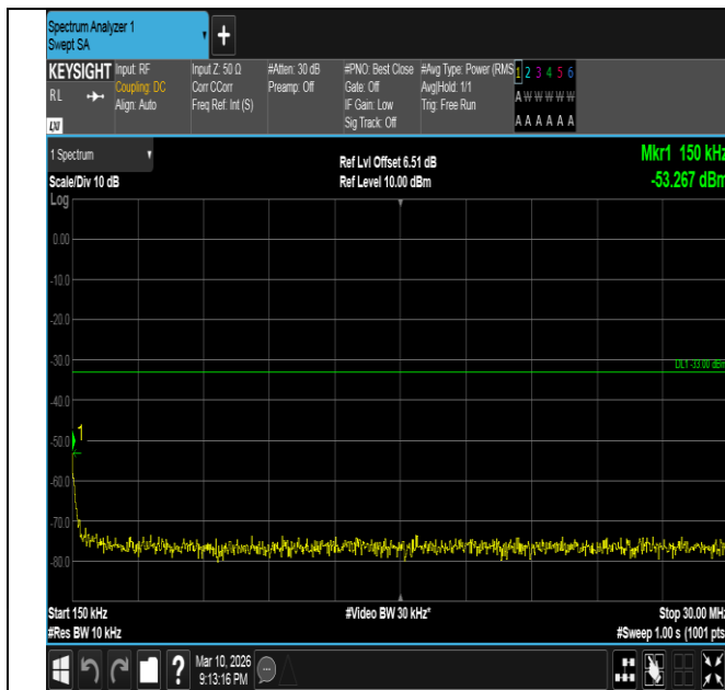
Band2-15MHz-QPSK-18900-1RB#74-0.15~30-PASS
