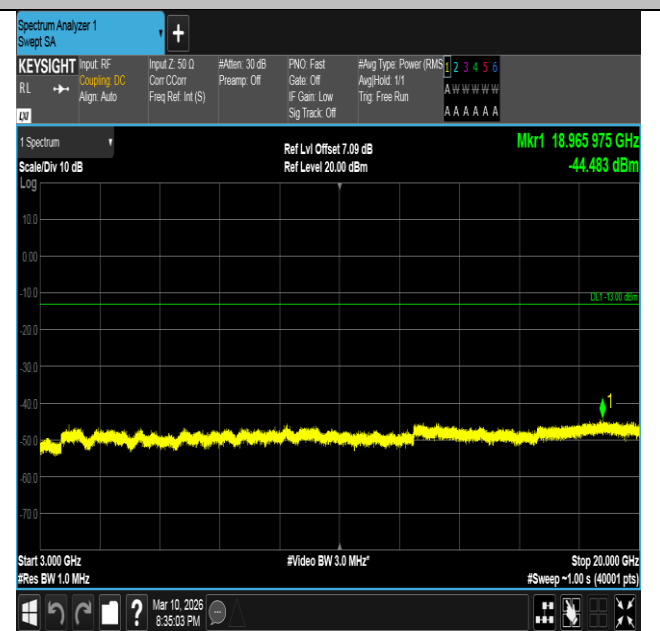
Band2-10MHz-QPSK-19150-1RB#49-3000~20000-PASS
