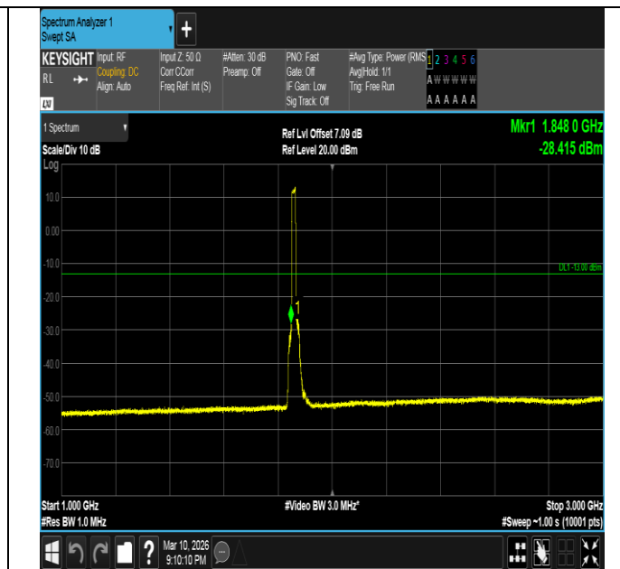
Band2-15MHz-QPSK-18675-75RB#0-1000~3000-PASS
