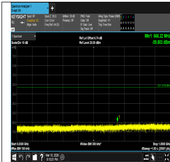
Band2-15MHz-QPSK-18675-75RB#0-30~1000-PASS
