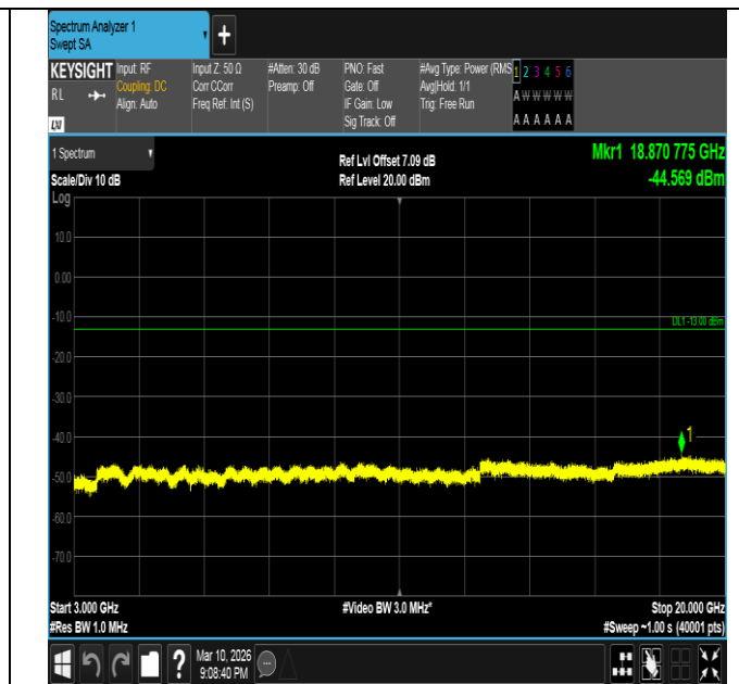
Band2-15MHz-QPSK-18675-1RB#74-3000~20000-PASS
