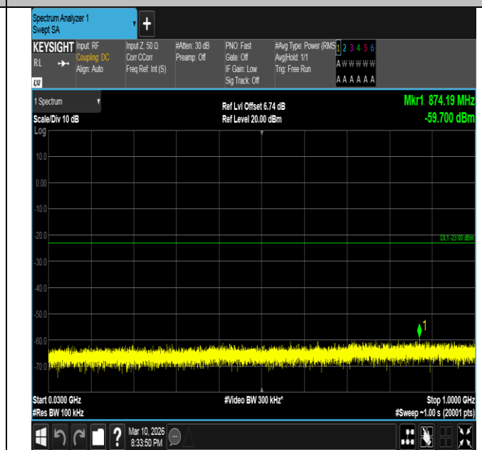
Band2-10MHz-16QAM-19150-1RB#0-30~1000-PASS
