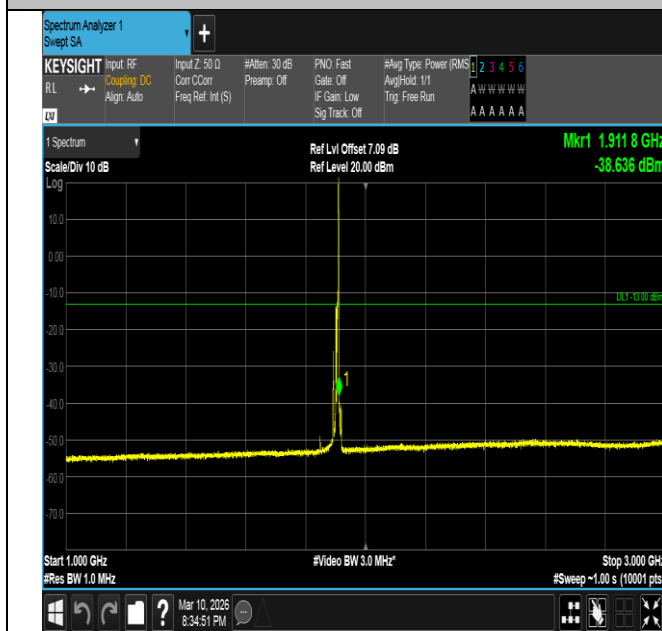
Band2-10MHz-QPSK-19150-1RB#49-1000~3000-PASS
