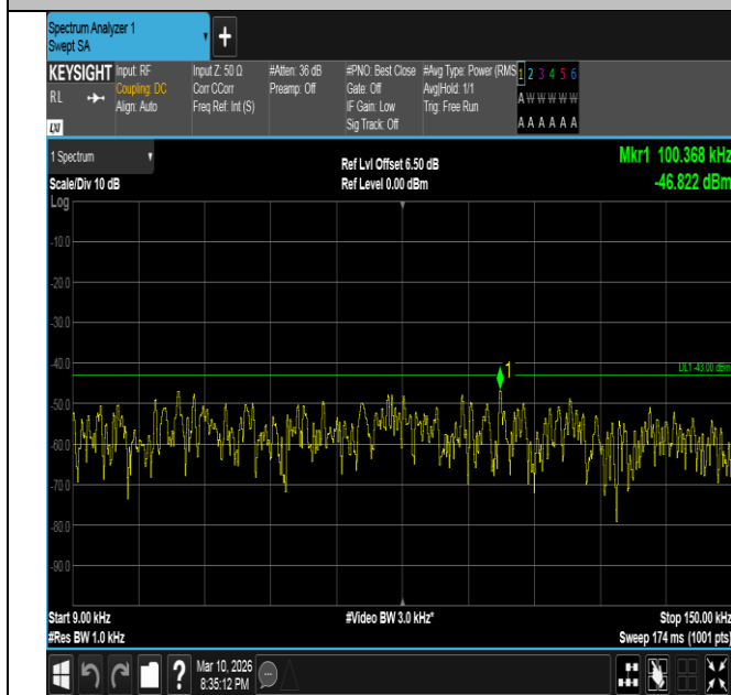
Band2-10MHz-16QAM-19150-1RB#49-0.009~0.15-PASS
