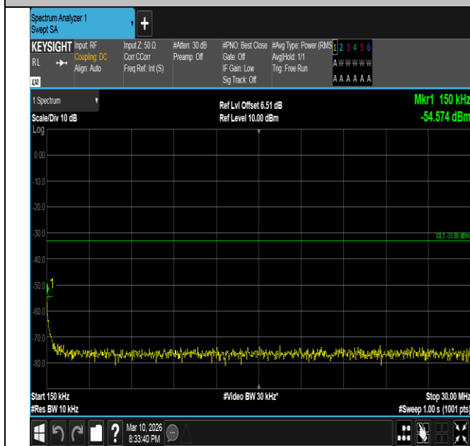
Band2-10MHz-16QAM-19150-1RB#0-0.15~30-PASS
