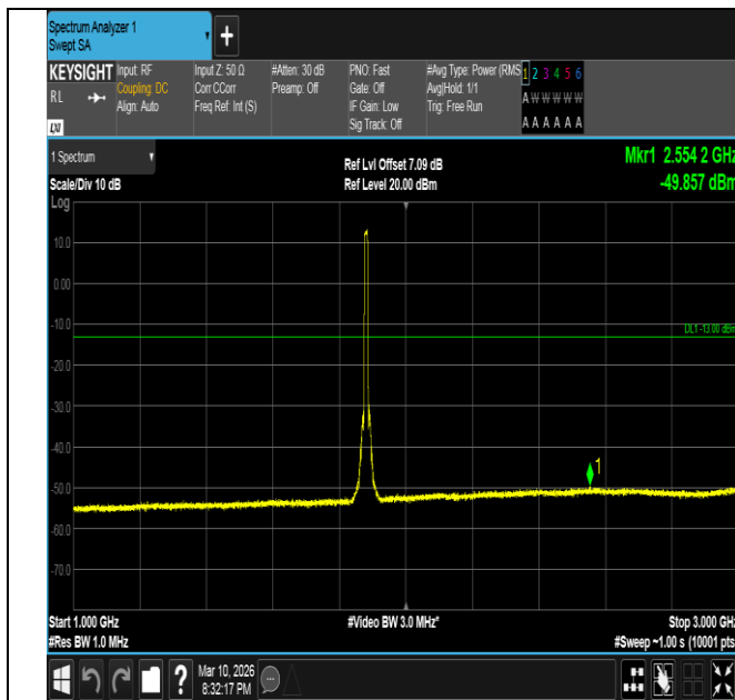
Band2-10MHz-16QAM-18900-50RB#0-1000~3000-PASS
