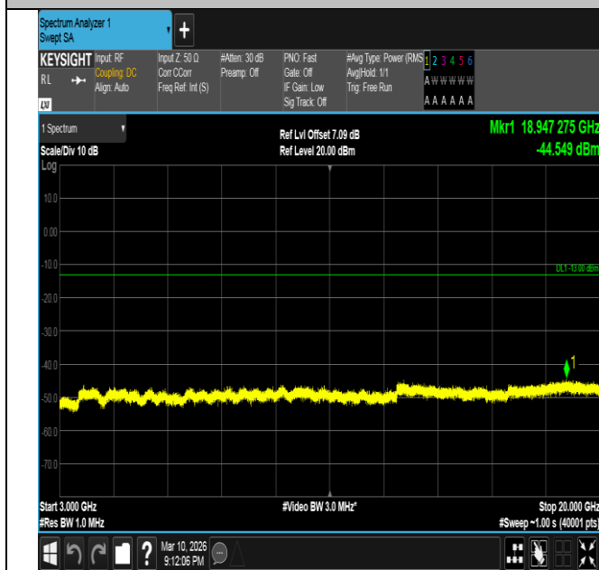
Band2-15MHz-QPSK-18900-1RB#0-3000~20000-PASS
