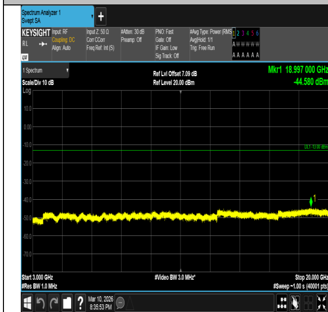
Band2-10MHz-16QAM-19150-1RB#49-3000~20000-PASS
