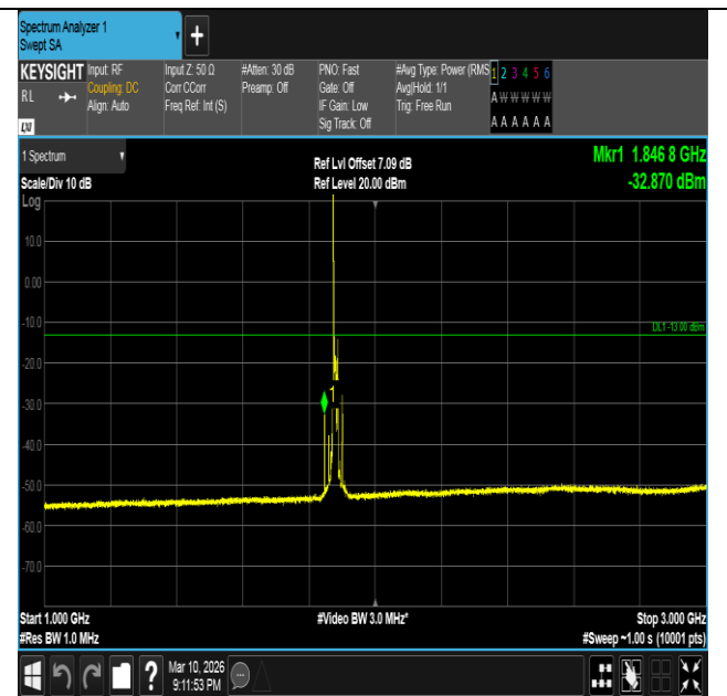
Band2-15MHz-QPSK-18900-1RB#0-1000~3000-PASS
