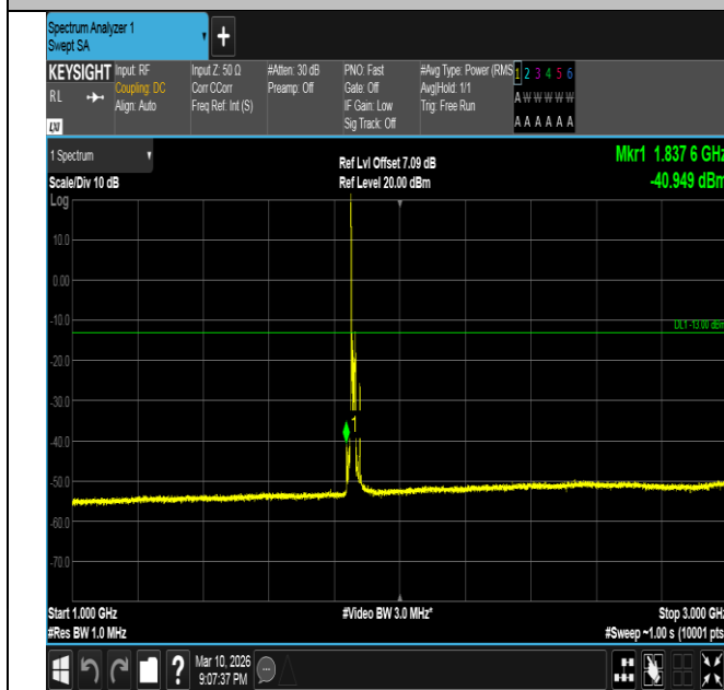
Band2-15MHz-16QAM-18675-1RB#0-1000~3000-PASS
