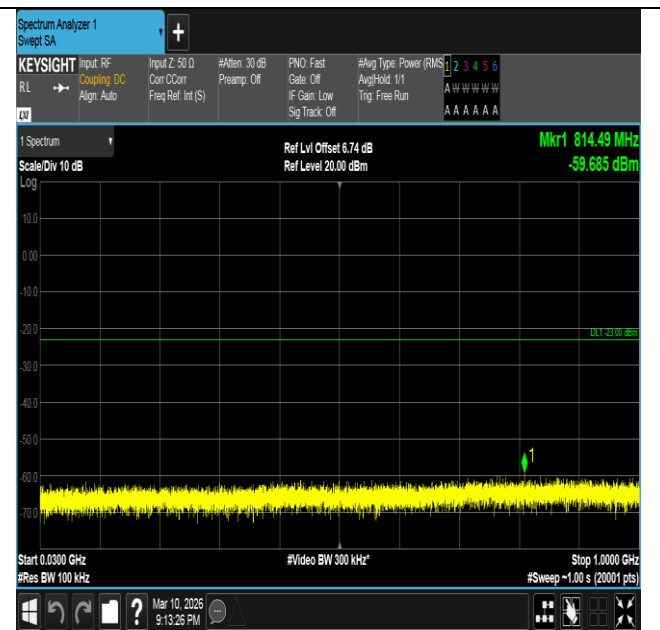
Band2-15MHz-QPSK-18900-1RB#74-30~1000-PASS
