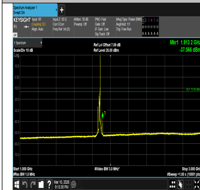
Band2-15MHz-QPSK-18900-1RB#74-1000~3000-PASS
