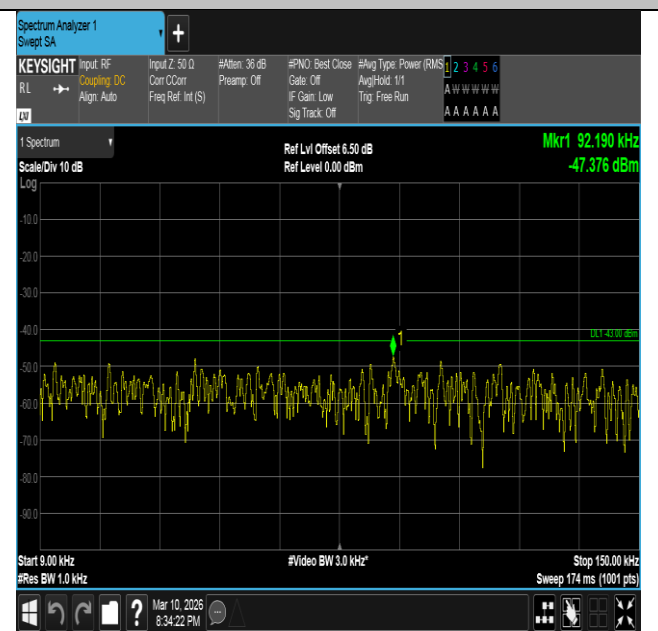
Band2-10MHz-QPSK-19150-1RB#49-0.009~0.15-PASS
