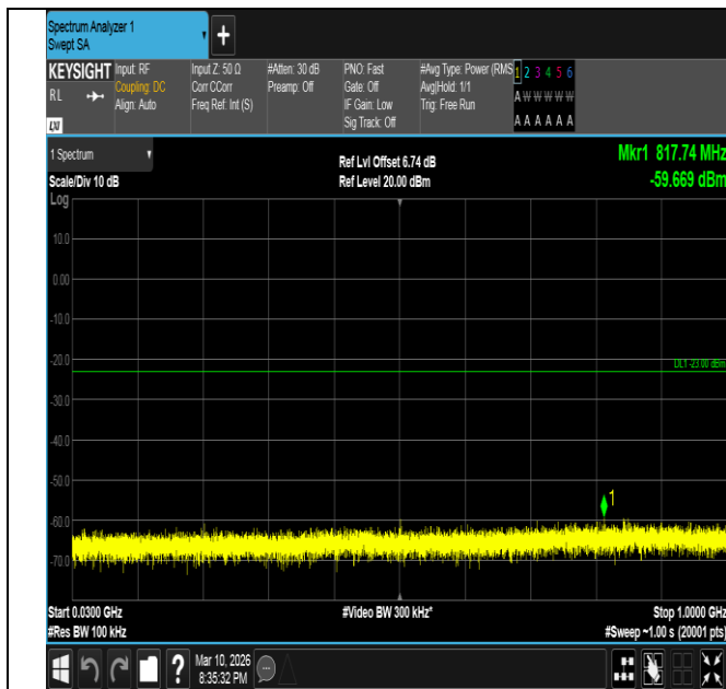
Band2-10MHz-16QAM-19150-1RB#49-30~1000-PASS
