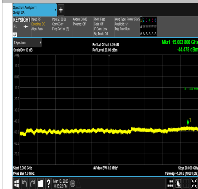
Band2-10MHz-QPSK-19150-1RB#0-3000~20000-PASS
