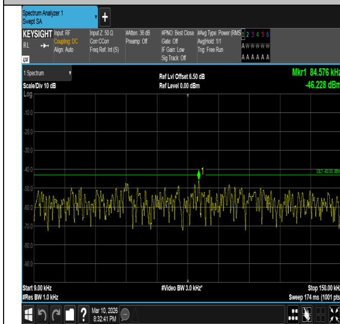
Band2-10MHz-QPSK-19150-1RB#0-0.009~0.15-PASS
