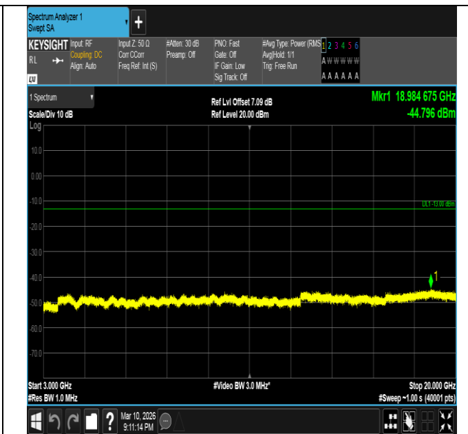
Band2-15MHz-16QAM-18675-75RB#0-3000~20000-PASS
