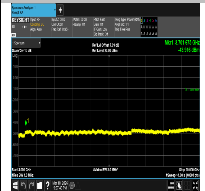
Band2-15MHz-16QAM-18675-1RB#0-3000~20000-PASS
