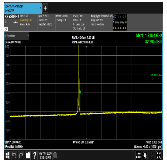
Band2-10MHz-QPSK-19150-1RB#0-1000~3000-PASS
