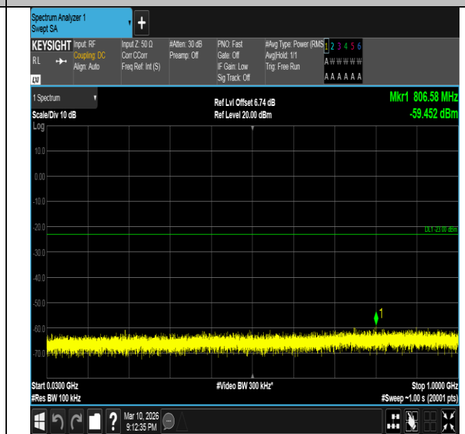
Band2-15MHz-16QAM-18900-1RB#0-30~1000-PASS
