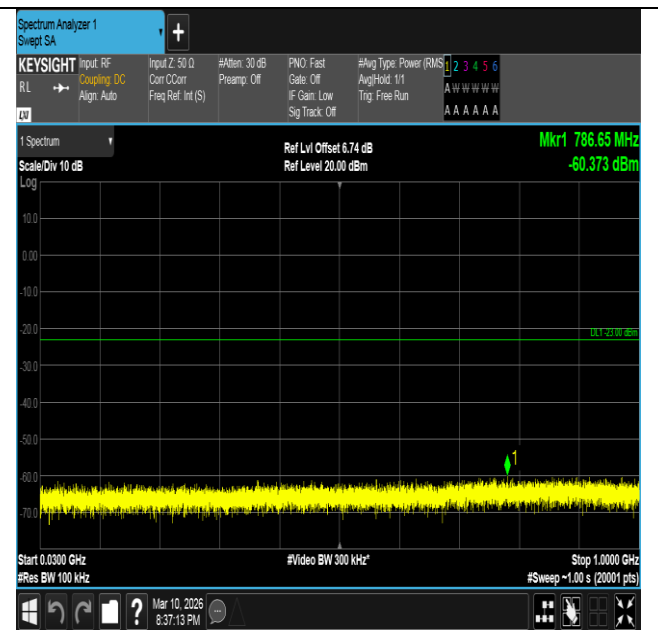
Band2-10MHz-16QAM-19150-50RB#0-30~1000-PASS
