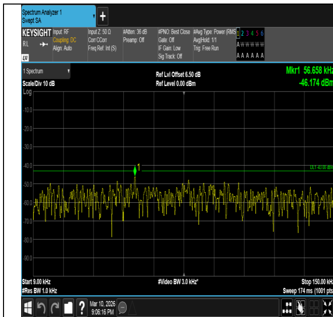
Band2-15MHz-QPSK-18675-1RB#0-0.009~0.15-PASS
