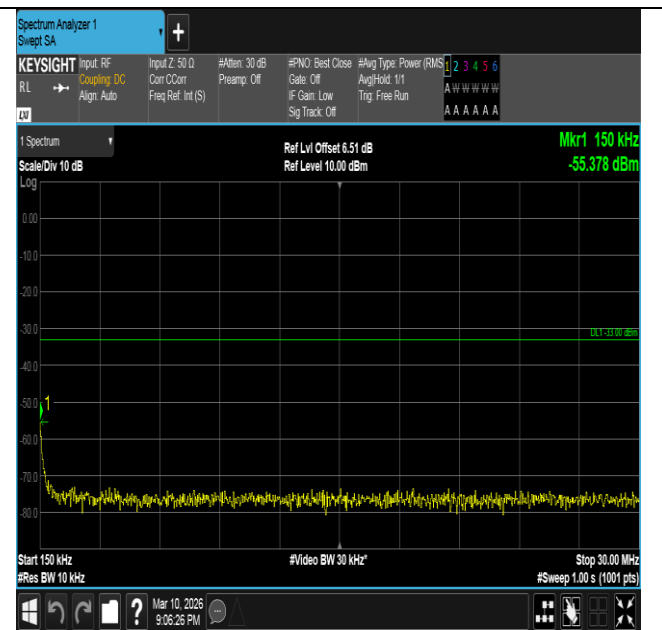
Band2-15MHz-QPSK-18675-1RB#0-0.15~30-PASS
