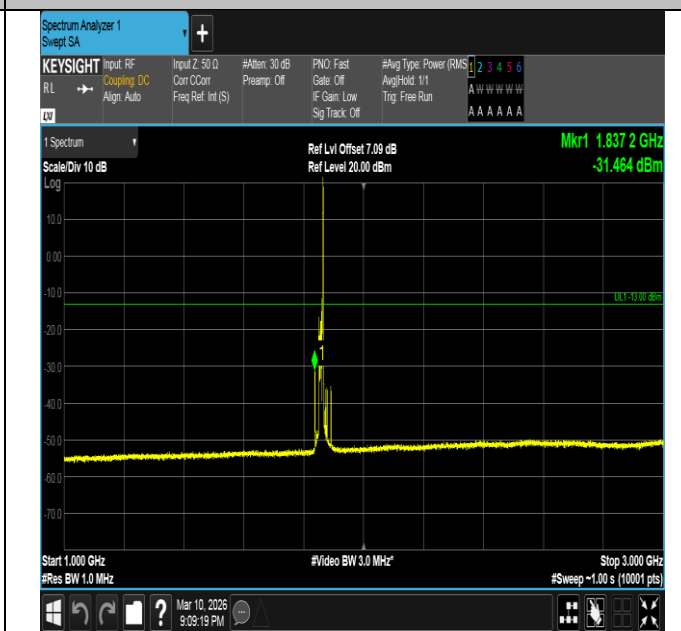
Band2-15MHz-16QAM-18675-1RB#74-1000~3000-PASS
