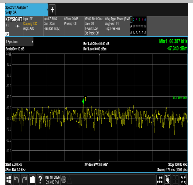
Band2-15MHz-QPSK-18900-1RB#74-0.009~0.15-PASS
