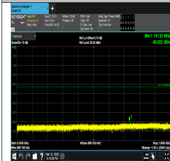
Band2-15MHz-QPSK-18900-75RB#0-30~1000-PASS
