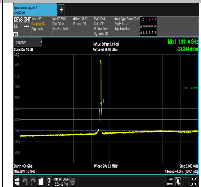
Band2-10MHz-QPSK-19150-50RB#0-1000~3000-PASS
