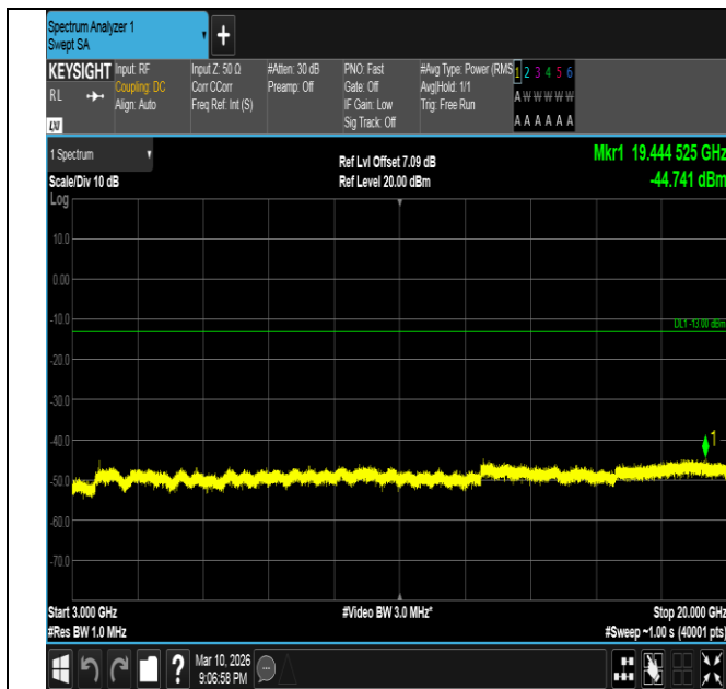
Band2-15MHz-QPSK-18675-1RB#0-3000~20000-PASS
