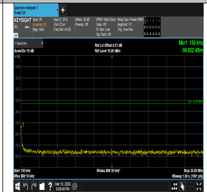
Band2-15MHz-QPSK-18675-75RB#0-0.15~30-PASS
