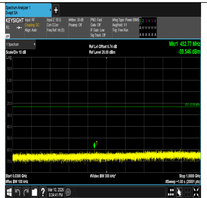
Band2-10MHz-QPSK-19150-1RB#49-30~1000-PASS
