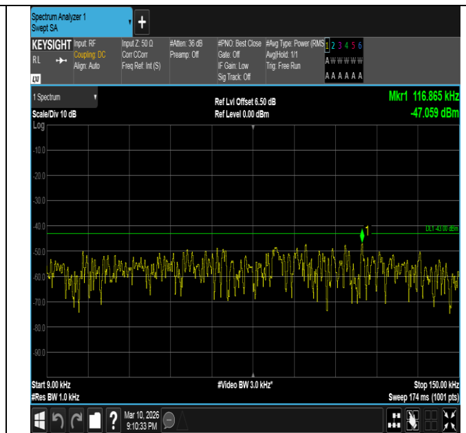
Band2-15MHz-16QAM-18675-75RB#0-0.009~0.15-PASS
