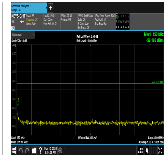
Band2-15MHz-QPSK-18900-75RB#0-0.15~30-PASS
