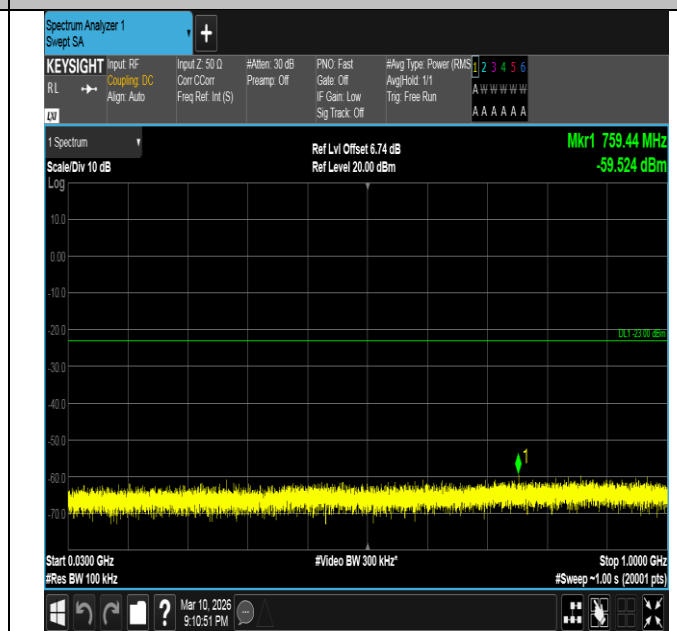
Band2-15MHz-16QAM-18675-75RB#0-30~1000-PASS
