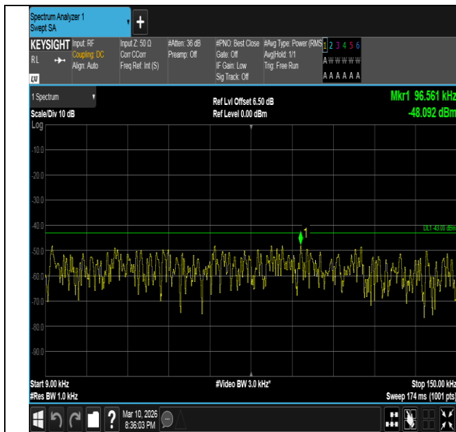
Band2-10MHz-QPSK-19150-50RB#0-0.009~0.15-PASS
