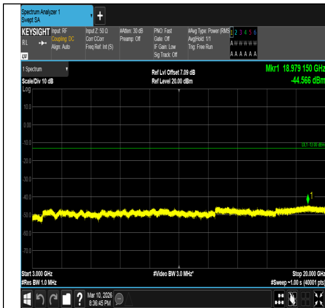
Band2-10MHz-QPSK-19150-50RB#0-3000~20000-PASS
