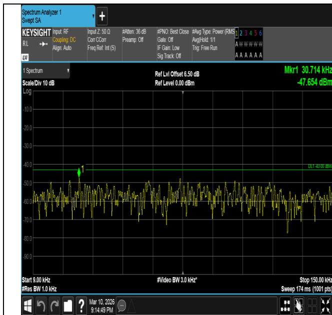
Band2-15MHz-QPSK-18900-75RB#0-0.009~0.15-PASS
