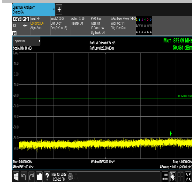
Band2-10MHz-QPSK-19150-50RB#0-30~1000-PASS
