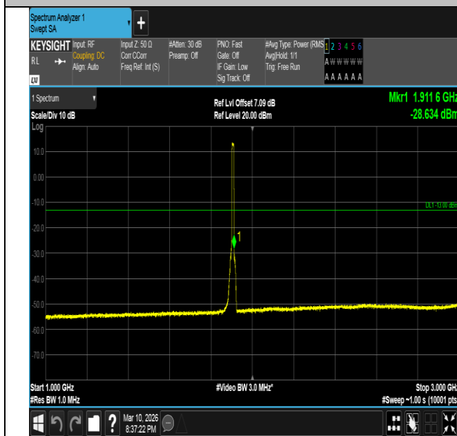
Band2-10MHz-16QAM-19150-50RB#0-1000~3000-PASS
