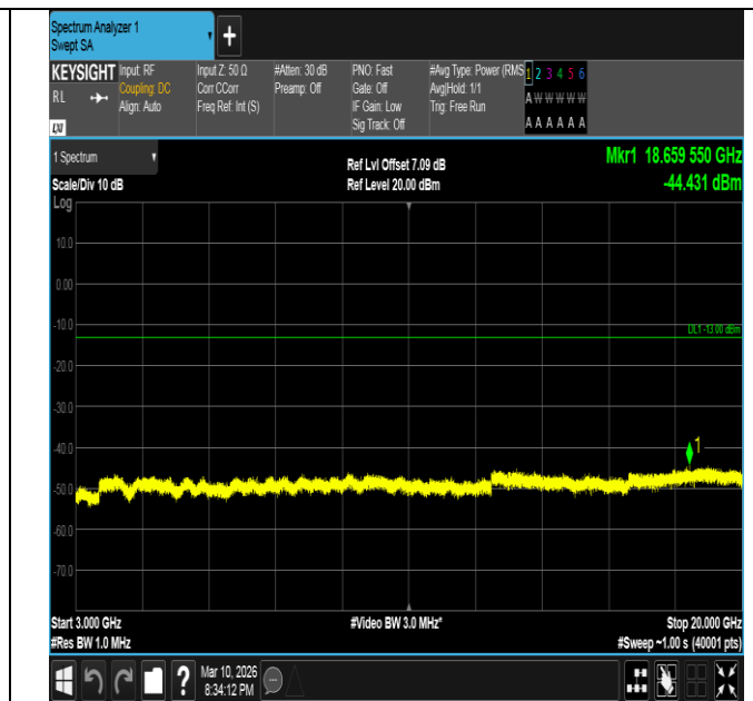
Band2-10MHz-16QAM-19150-1RB#0-3000~20000-PASS
