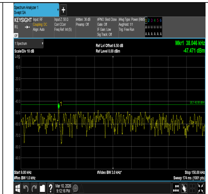
Band2-15MHz-16QAM-18900-1RB#0-0.009~0.15-PASS
