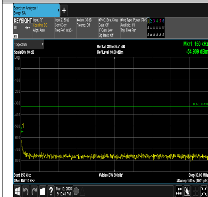
Band2-15MHz-16QAM-18675-75RB#0-0.15~30-PASS
