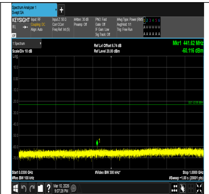
Band2-15MHz-16QAM-18675-1RB#0-30~1000-PASS
