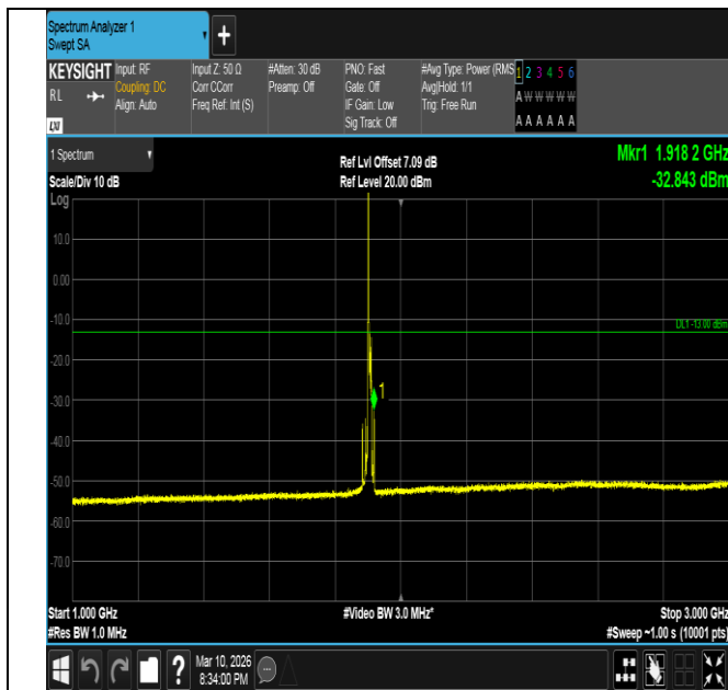
Band2-10MHz-16QAM-19150-1RB#0-1000~3000-PASS
