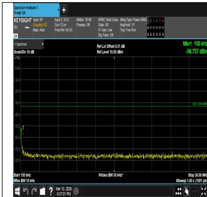
Band2-10MHz-16QAM-19150-50RB#0-0.15~30-PASS
