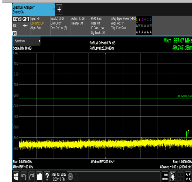
Band2-15MHz-16QAM-18675-1RB#74-30~1000-PASS
