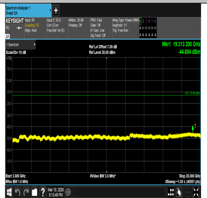
Band2-15MHz-QPSK-18900-1RB#74-3000~20000-PASS
