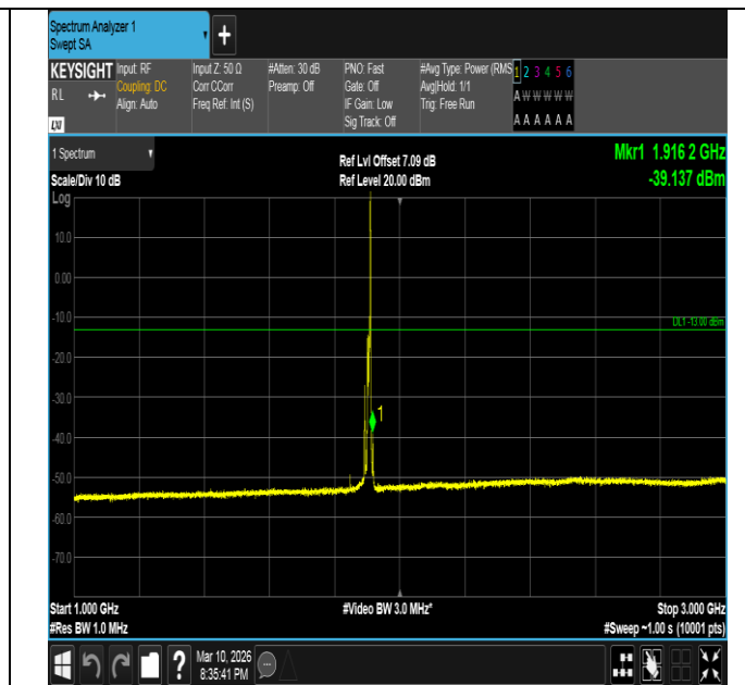
Band2-10MHz-16QAM-19150-1RB#49-1000~3000-PASS
