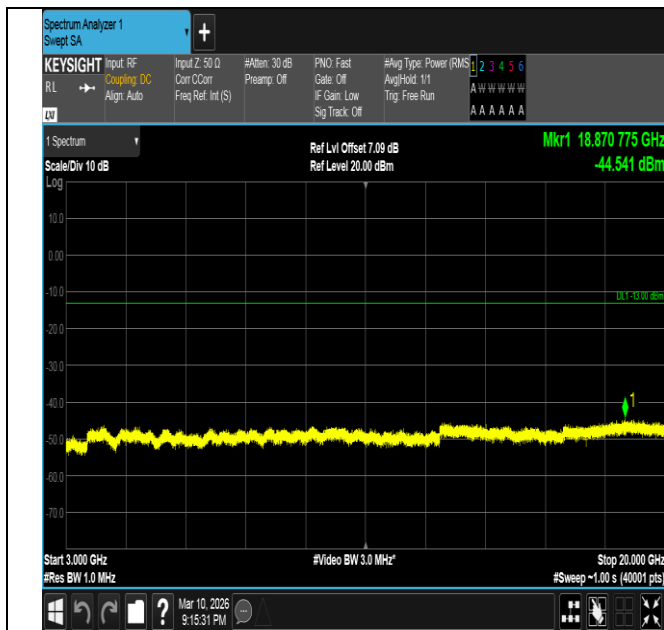
Band2-15MHz-QPSK-18900-75RB#0-3000~20000-PASS
