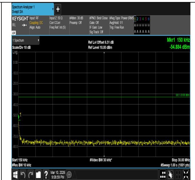
Band2-15MHz-16QAM-18675-1RB#74-0.15~30-PASS
