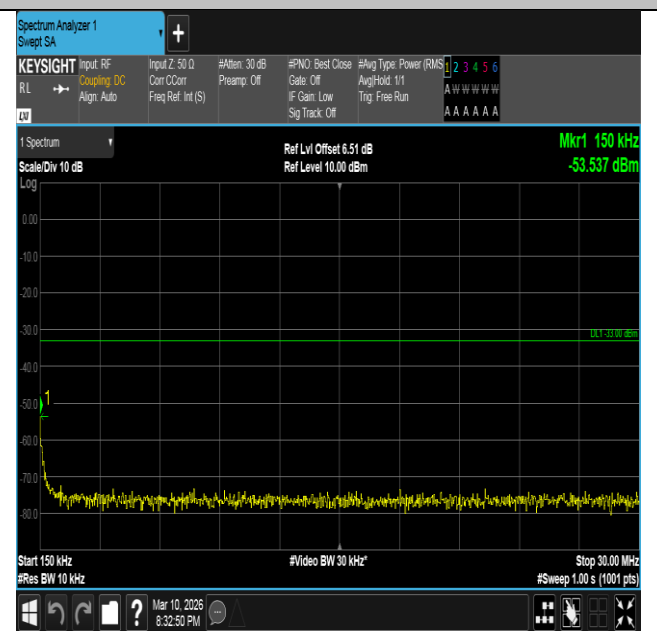
Band2-10MHz-QPSK-19150-1RB#0-0.15~30-PASS
