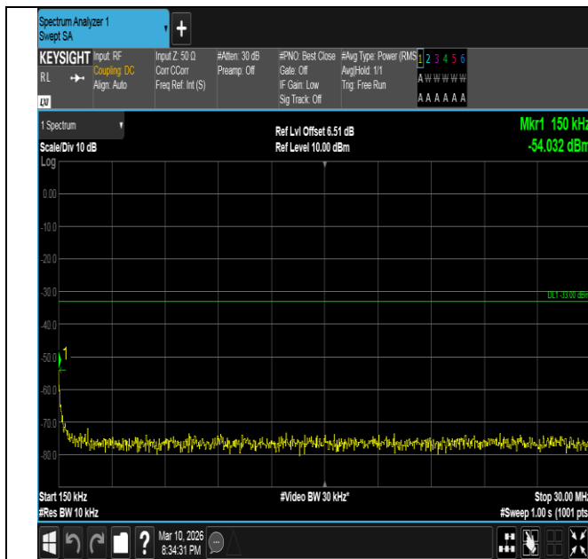
Band2-10MHz-QPSK-19150-1RB#49-0.15~30-PASS
