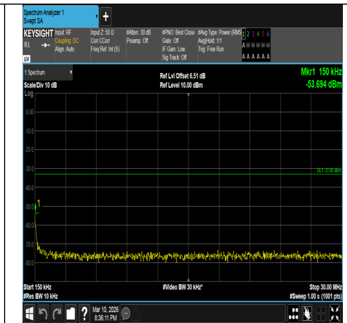
Band2-10MHz-QPSK-19150-50RB#0-0.15~30-PASS
