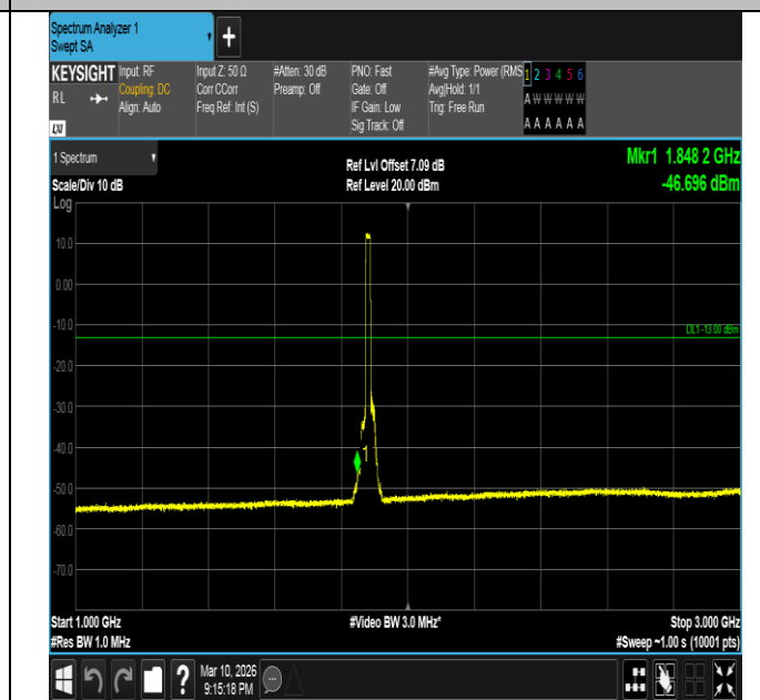
Band2-15MHz-QPSK-18900-75RB#0-1000~3000-PASS
