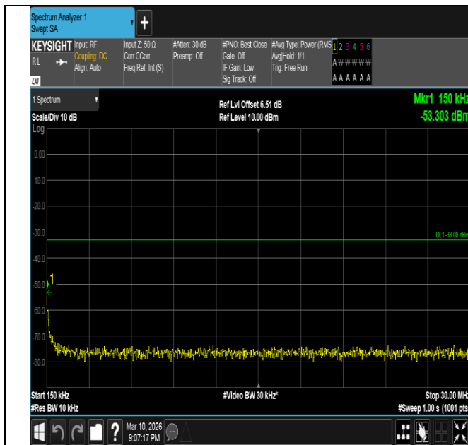
Band2-15MHz-16QAM-18675-1RB#0-0.15~30-PASS
