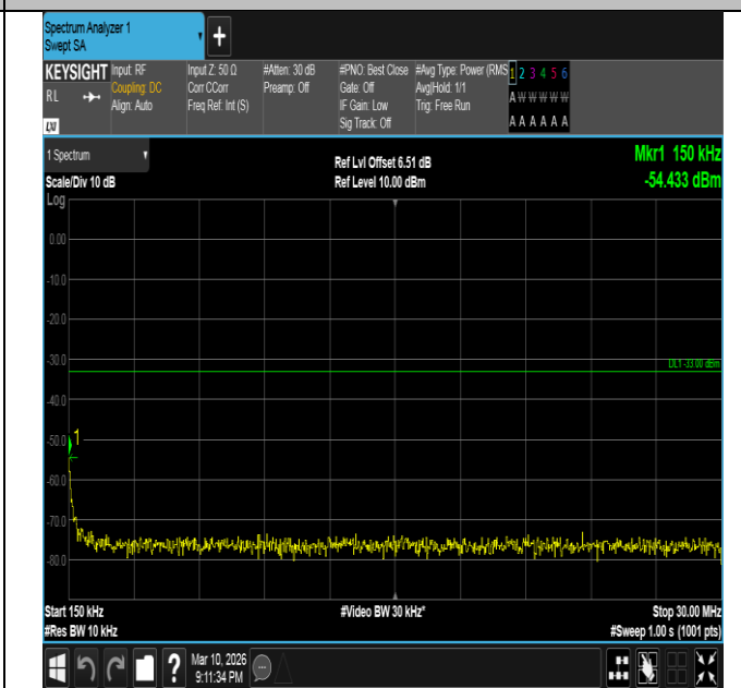
Band2-15MHz-QPSK-18900-1RB#0-0.15~30-PASS
