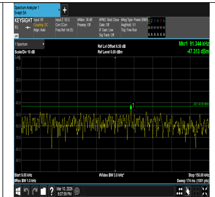
Band2-15MHz-QPSK-18675-1RB#74-0.009~0.15-PASS
