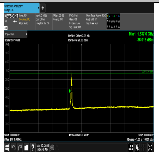
Band2-15MHz-QPSK-18675-1RB#0-1000~3000-PASS
