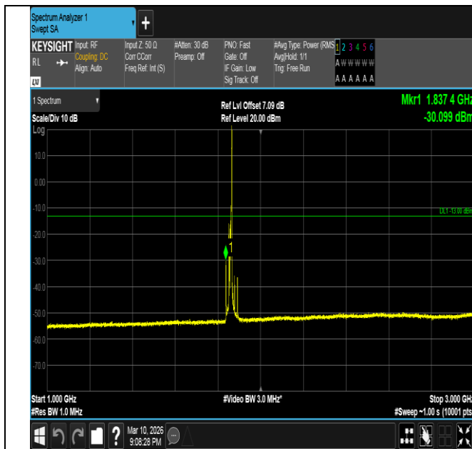
Band2-15MHz-QPSK-18675-1RB#74-1000~3000-PASS
