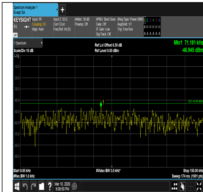
Band2-15MHz-16QAM-18675-1RB#74-0.009~0.15-PASS
