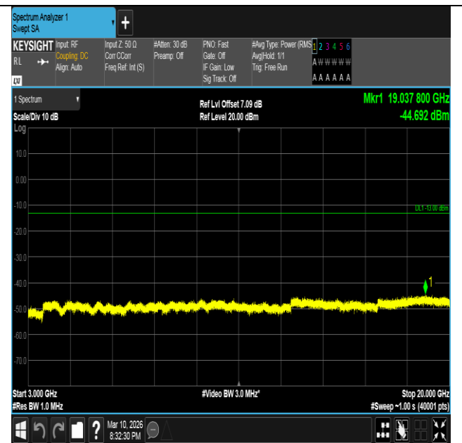
Band2-10MHz-16QAM-18900-50RB#0-3000~20000-PASS
