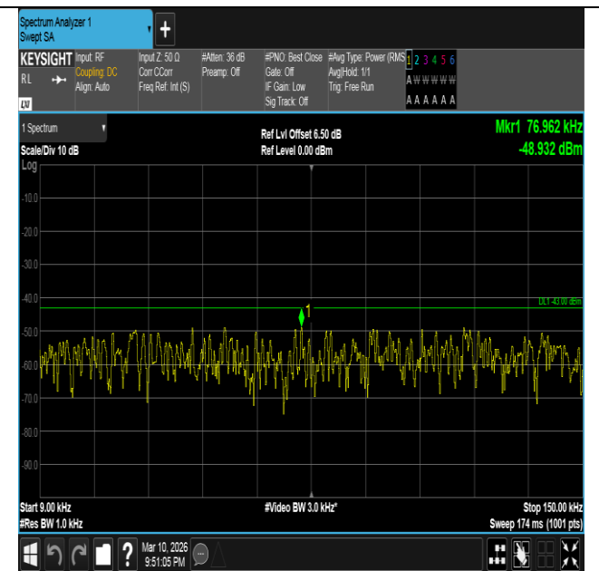
Band2-20MHz-16QAM-18700-1RB#0-0.009~0.15-PASS
