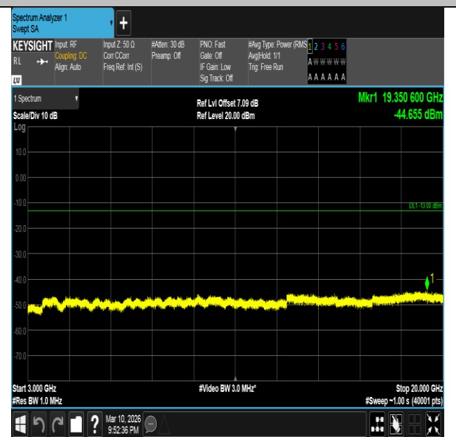
Band2-20MHz-QPSK-18700-1RB#99-3000~20000-PASS
