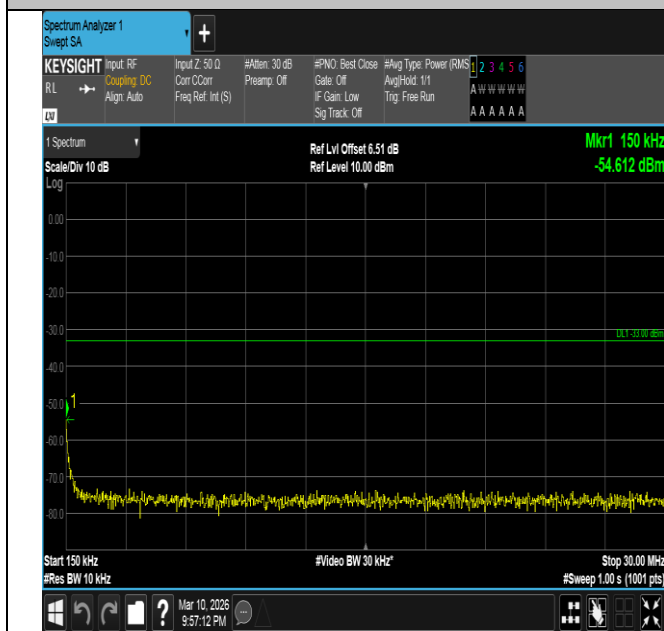
Band2-20MHz-QPSK-18900-1RB#99-0.15~30-PASS
