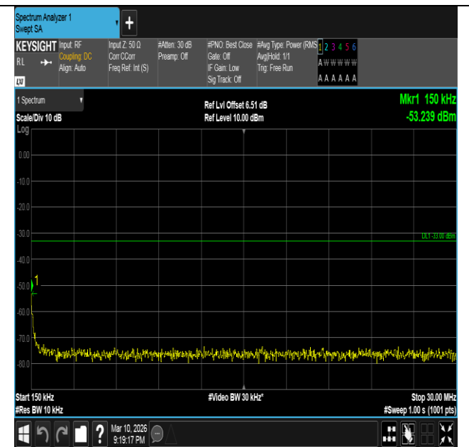
Band2-15MHz-16QAM-19125-1RB#74-0.15~30-PASS
