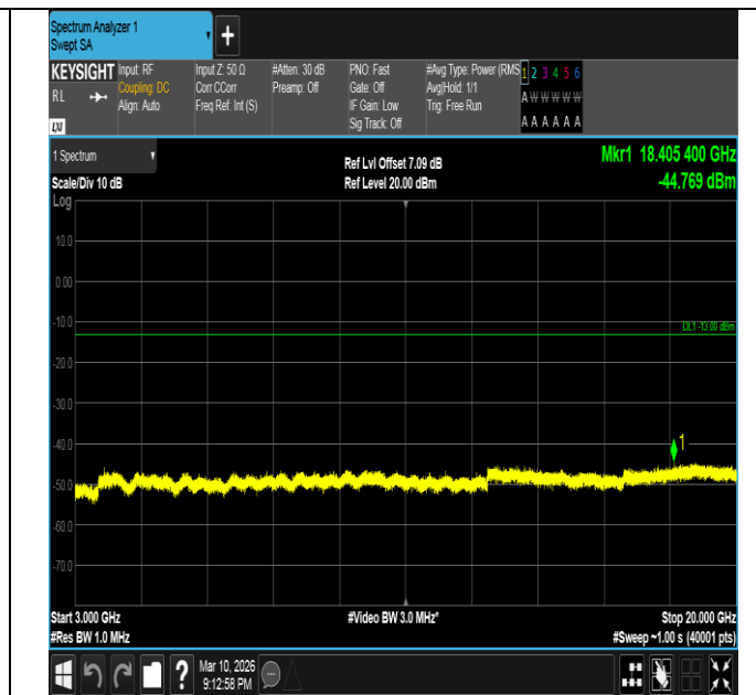
Band2-15MHz-16QAM-18900-1RB#0-3000~20000-PASS
