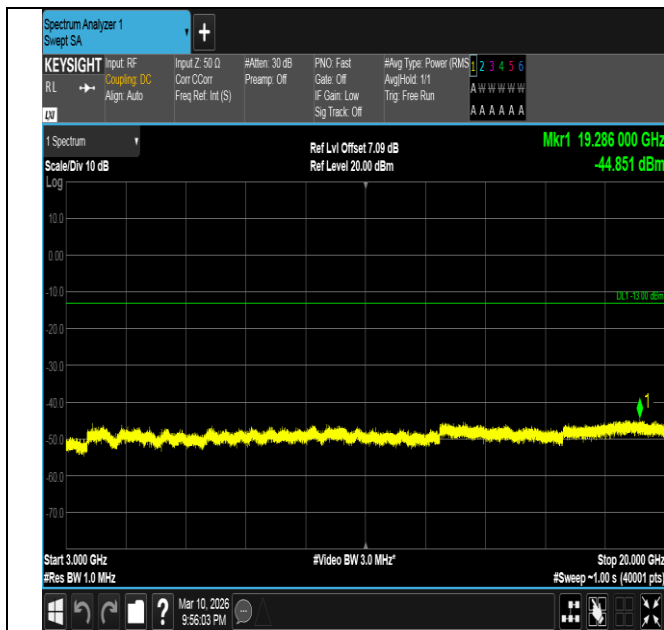
Band2-20MHz-QPSK-18900-1RB#0-3000~20000-PASS
