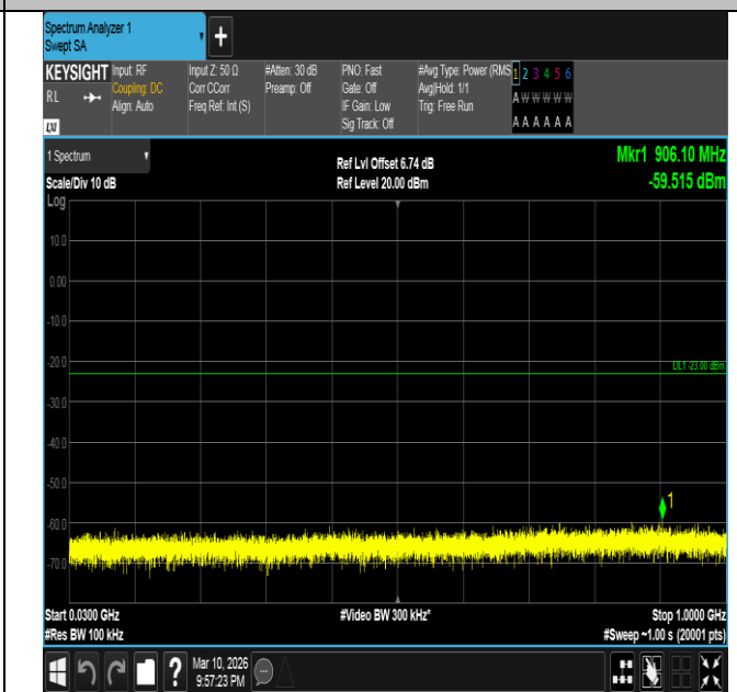
Band2-20MHz-QPSK-18900-1RB#99-30~1000-PASS
