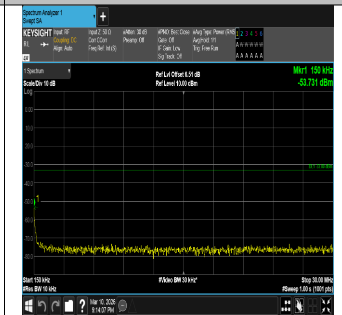
Band2-15MHz-16QAM-18900-1RB#74-0.15~30-PASS
