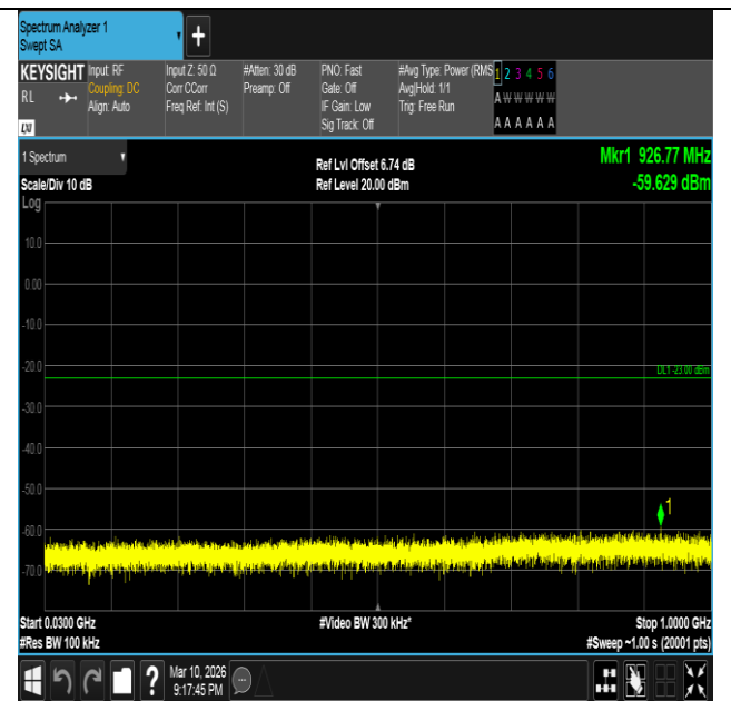
Band2-15MHz-16QAM-19125-1RB#0-30~1000-PASS
