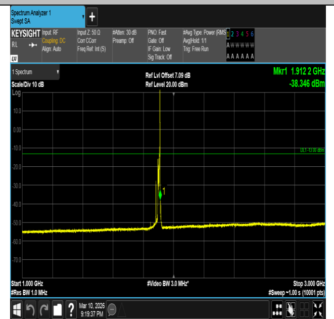
Band2-15MHz-16QAM-19125-1RB#74-1000~3000-PASS
