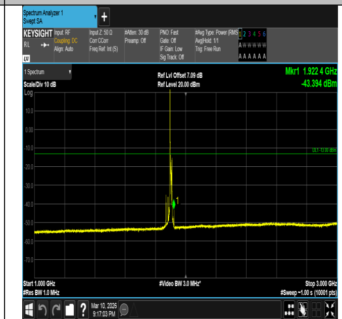
Band2-15MHz-QPSK-19125-1RB#0-1000~3000-PASS
