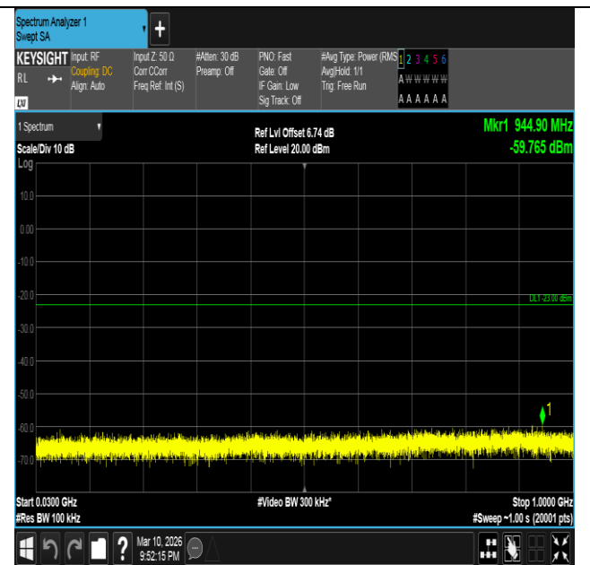
Band2-20MHz-QPSK-18700-1RB#99-30~1000-PASS
