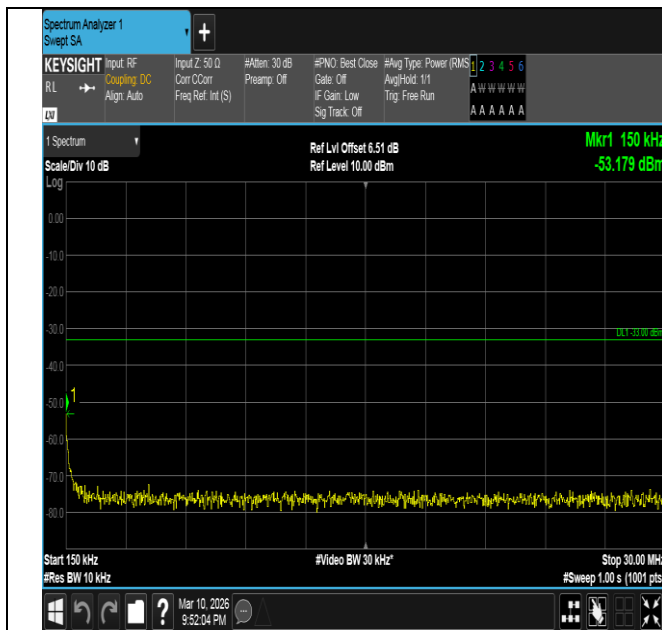
Band2-20MHz-QPSK-18700-1RB#99-0.15~30-PASS
