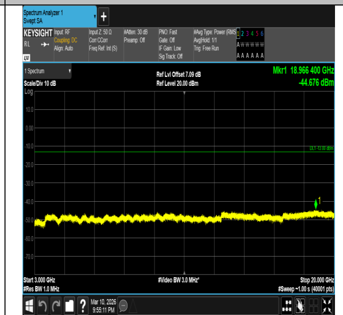
Band2-20MHz-16QAM-18700-100RB#0-3000~20000-PASS
