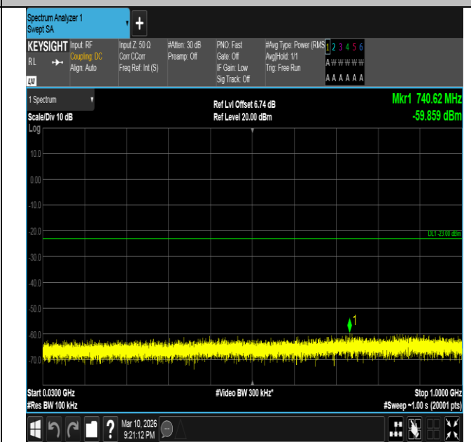
Band2-15MHz-16QAM-19125-75RB#0-30~1000-PASS
