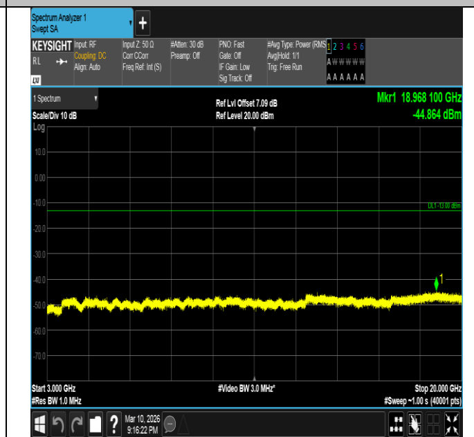
Band2-15MHz-16QAM-18900-75RB#0-3000~20000-PASS
