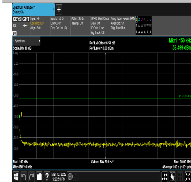
Band2-15MHz-16QAM-19125-75RB#0-0.15~30-PASS
