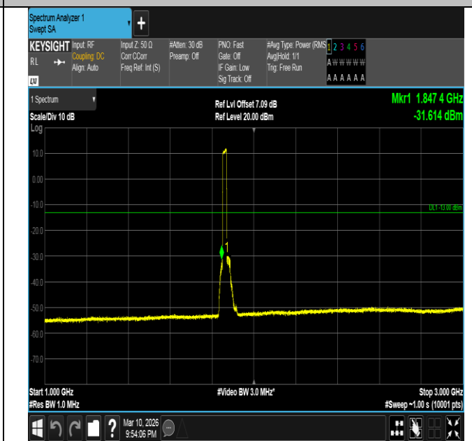
Band2-20MHz-QPSK-18700-100RB#0-1000~3000-PASS
