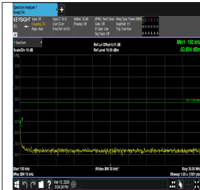
Band2-20MHz-16QAM-18700-100RB#0-0.15~30-PASS
