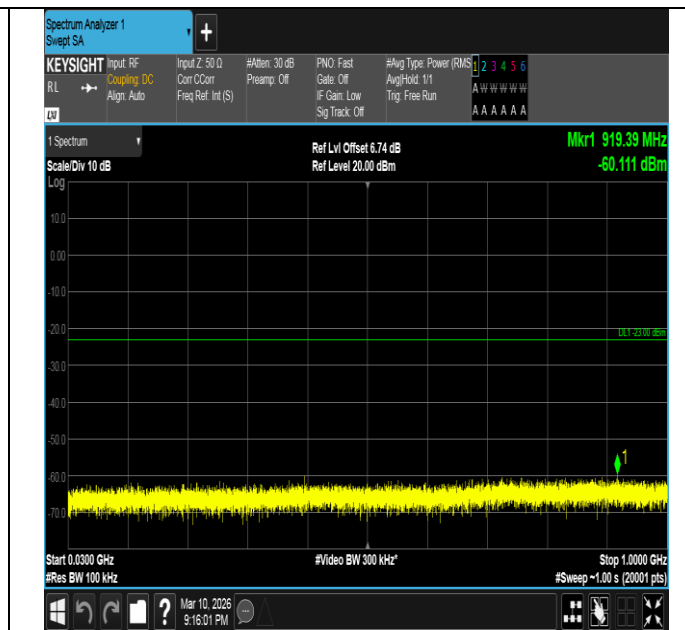
Band2-15MHz-16QAM-18900-75RB#0-30~1000-PASS
