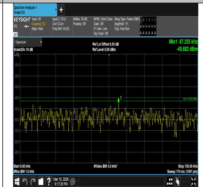
Band2-15MHz-16QAM-19125-1RB#0-0.009~0.15-PASS
