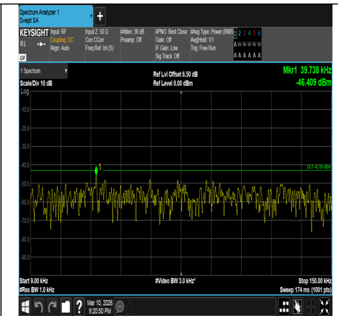
Band2-15MHz-16QAM-19125-75RB#0-0.009~0.15-PASS
