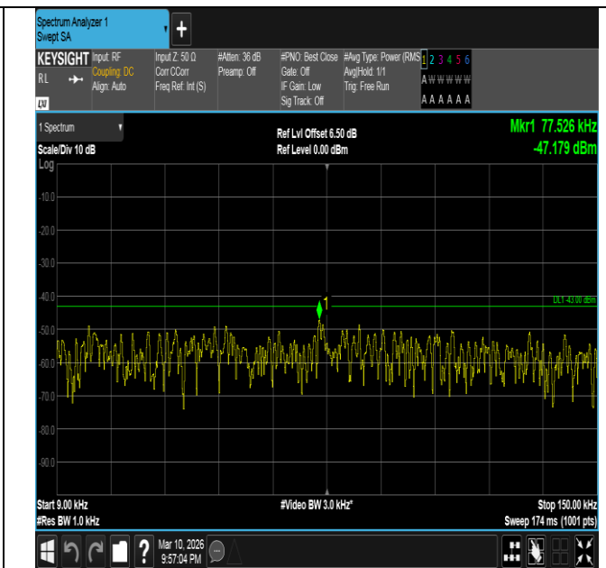
Band2-20MHz-QPSK-18900-1RB#99-0.009~0.15-PASS
