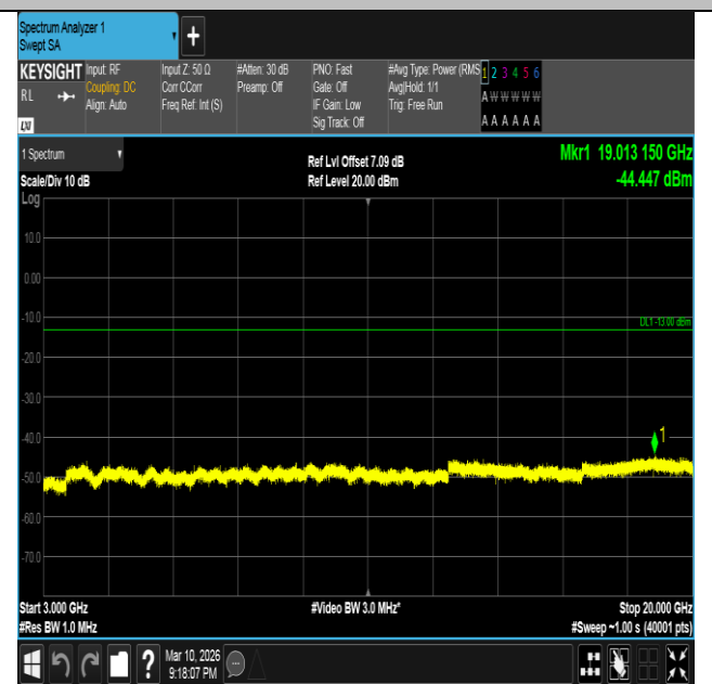
Band2-15MHz-16QAM-19125-1RB#0-3000~20000-PASS
