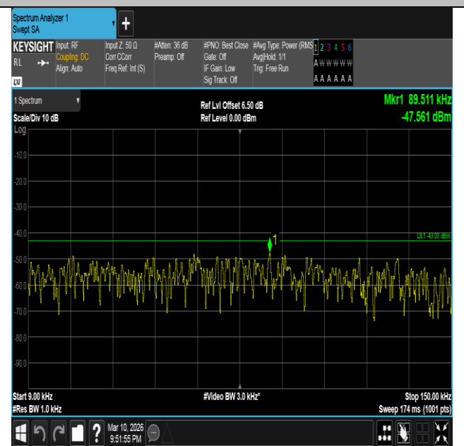
Band2-20MHz-QPSK-18700-1RB#99-0.009~0.15-PASS
