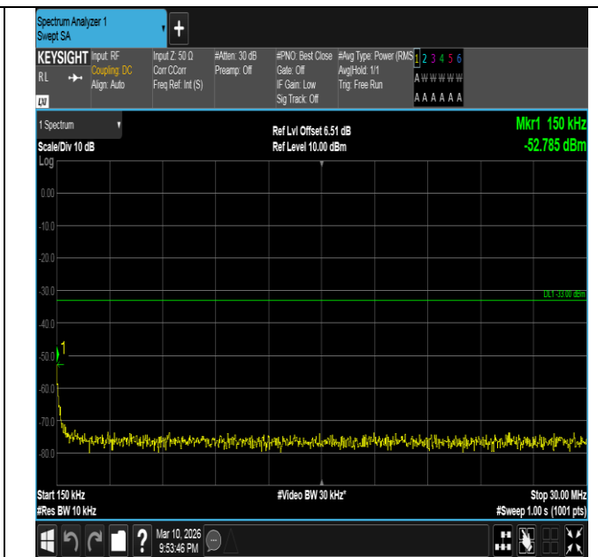
Band2-20MHz-QPSK-18700-100RB#0-0.15~30-PASS
