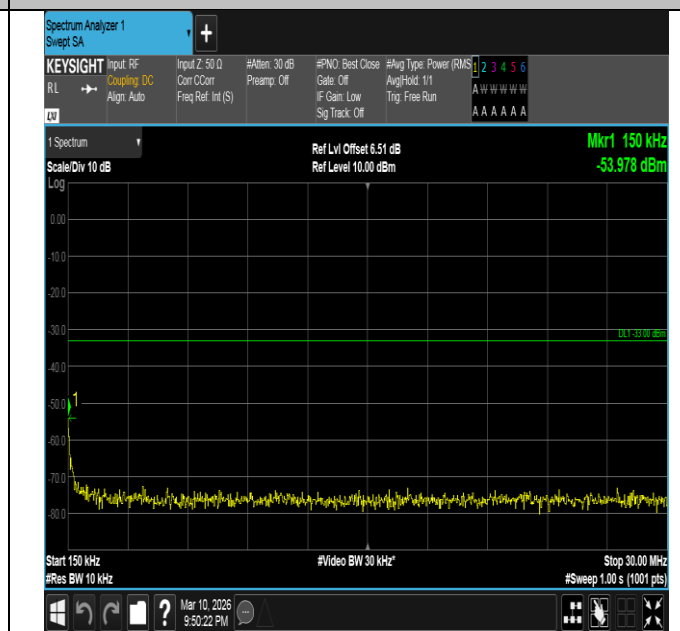
Band2-20MHz-QPSK-18700-1RB#0-0.15~30-PASS
