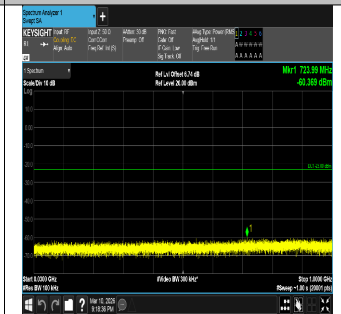
Band2-15MHz-QPSK-19125-1RB#74-30~1000-PASS
