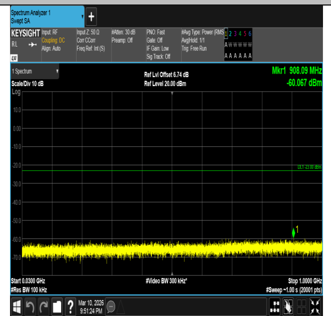
Band2-20MHz-16QAM-18700-1RB#0-30~1000-PASS
