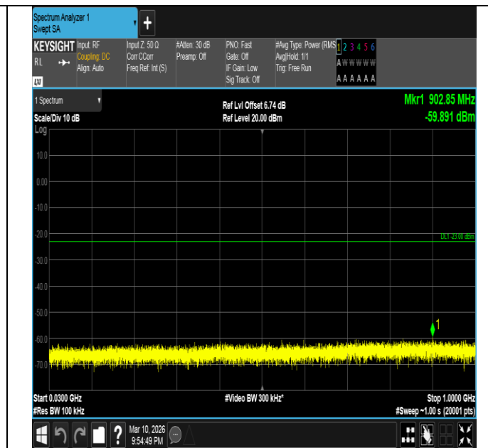
Band2-20MHz-16QAM-18700-100RB#0-30~1000-PASS
