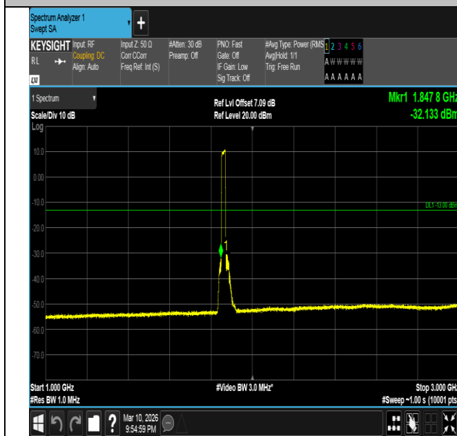
Band2-20MHz-16QAM-18700-100RB#0-1000~3000-PASS
