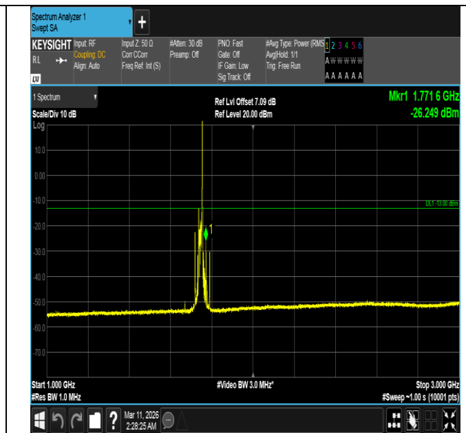
Band4-20MHz-16QAM-20300-1RB#99-1000~3000-PASS
