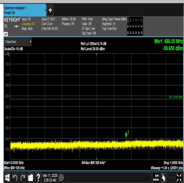
Band4-20MHz-16QAM-20300-1RB#0-30~1000-PASS
