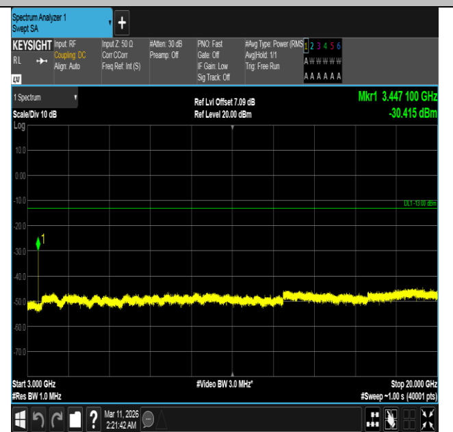
Band4-20MHz-16QAM-20175-1RB#0-3000~20000-PASS
