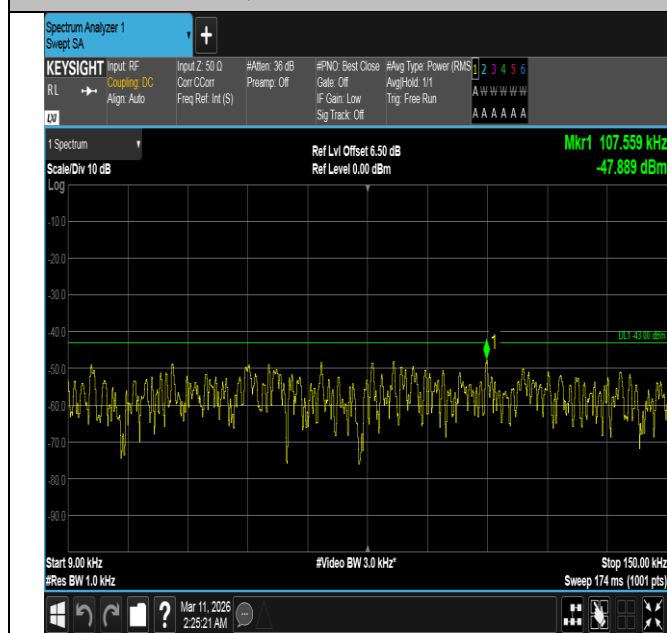
Band4-20MHz-QPSK-20300-1RB#0-0.009~0.15-PASS
