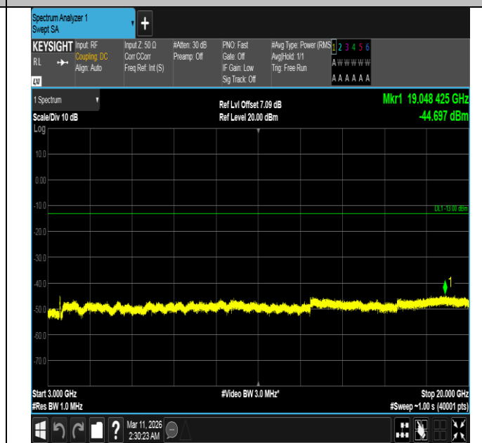
Band4-20MHz-16QAM-20300-100RB#0-3000~20000-PASS
