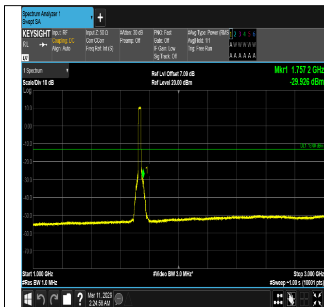
Band4-20MHz-16QAM-20175-100RB#0-1000~3000-PASS
