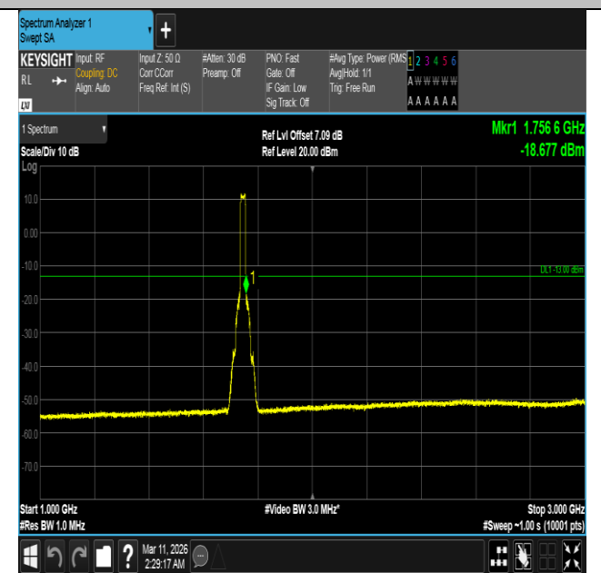
Band4-20MHz-QPSK-20300-100RB#0-1000~3000-PASS
