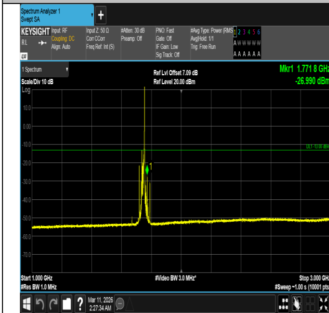
Band4-20MHz-QPSK-20300-1RB#99-1000~3000-PASS
