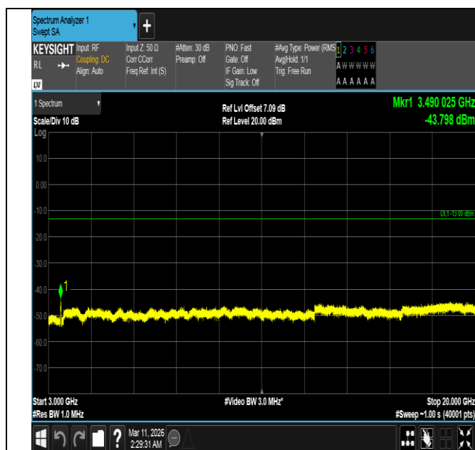
Band4-20MHz-QPSK-20300-100RB#0-3000~20000-PASS
