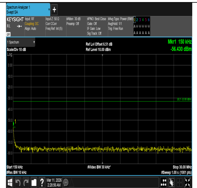
Band4-20MHz-QPSK-20300-100RB#0-0.15~30-PASS
