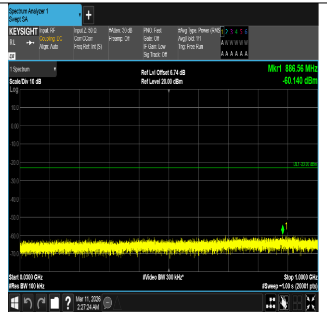
Band4-20MHz-QPSK-20300-1RB#99-30~1000-PASS
