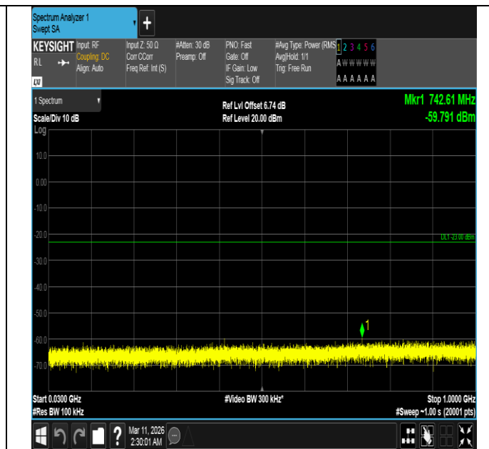
Band4-20MHz-16QAM-20300-100RB#0-30~1000-PASS
