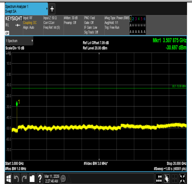
Band4-20MHz-QPSK-20300-1RB#99-3000~20000-PASS
