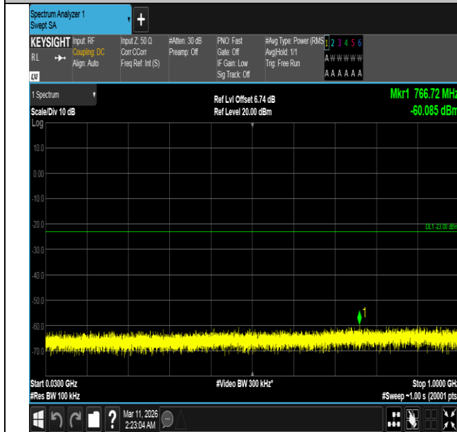
Band4-20MHz-16QAM-20175-1RB#99-30~1000-PASS
