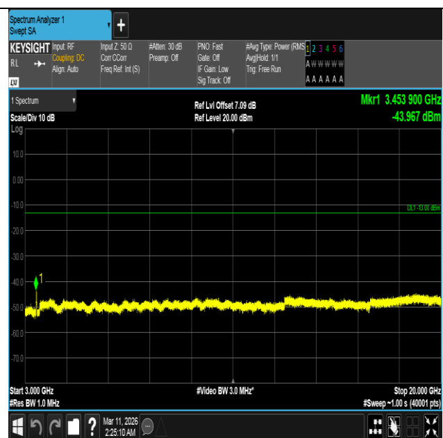
Band4-20MHz-16QAM-20175-100RB#0-3000~20000-PASS
