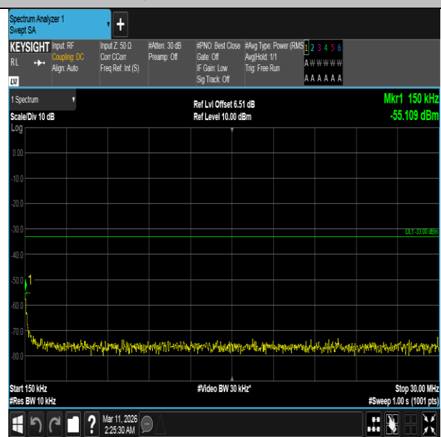
Band4-20MHz-QPSK-20300-1RB#0-0.15~30-PASS
