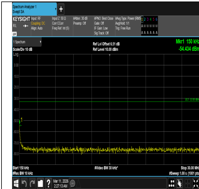
Band4-20MHz-QPSK-20300-1RB#99-0.15~30-PASS
