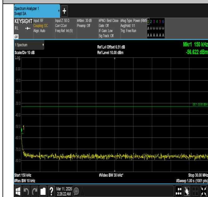
Band4-20MHz-16QAM-20300-1RB#0-0.15~30-PASS
