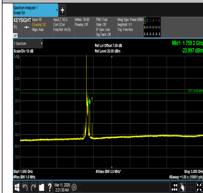
Band4-20MHz-16QAM-20175-1RB#0-1000~3000-PASS
